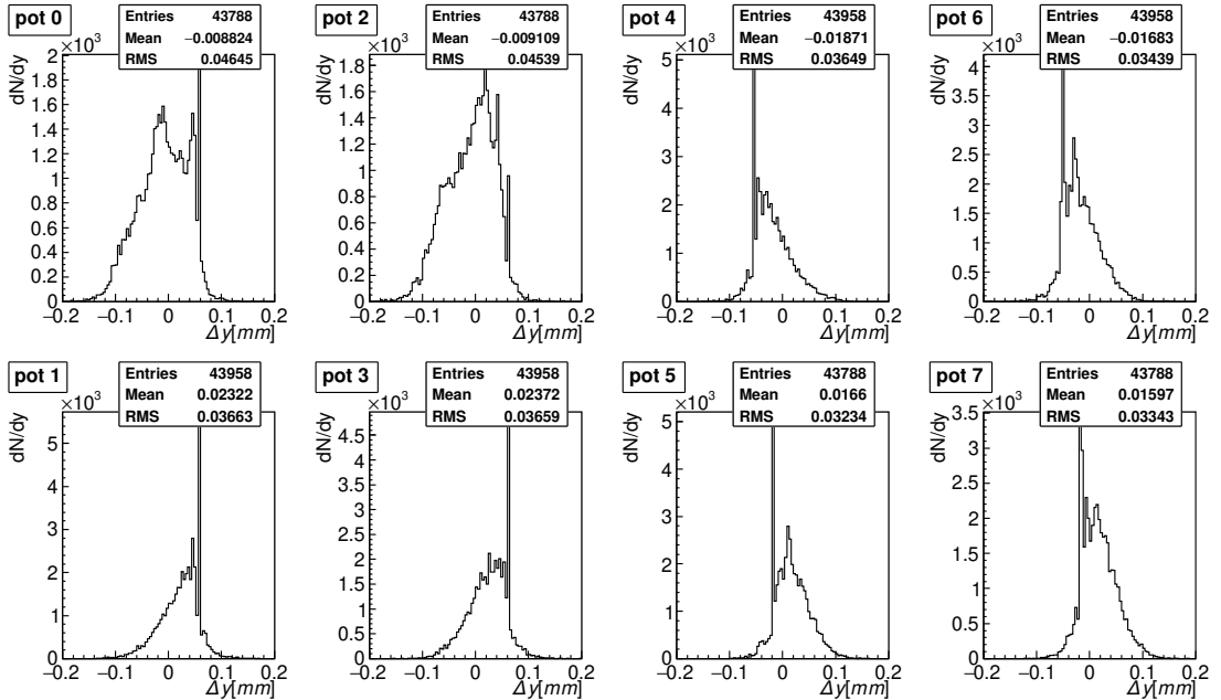
Event by event y difference for all pots: \Delta y = y_{\text{LHC\_fieldOff}} - y_{\text{LHC\_fieldOn}} ; golden elastic events.
