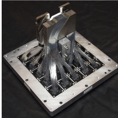
Figure 1.10: Left: Schematic view of the ALFA station instrumentation (copyright CERN, CC-BY-4.0 license). Right: Photograph of the ALFA detector assembly [P11].
