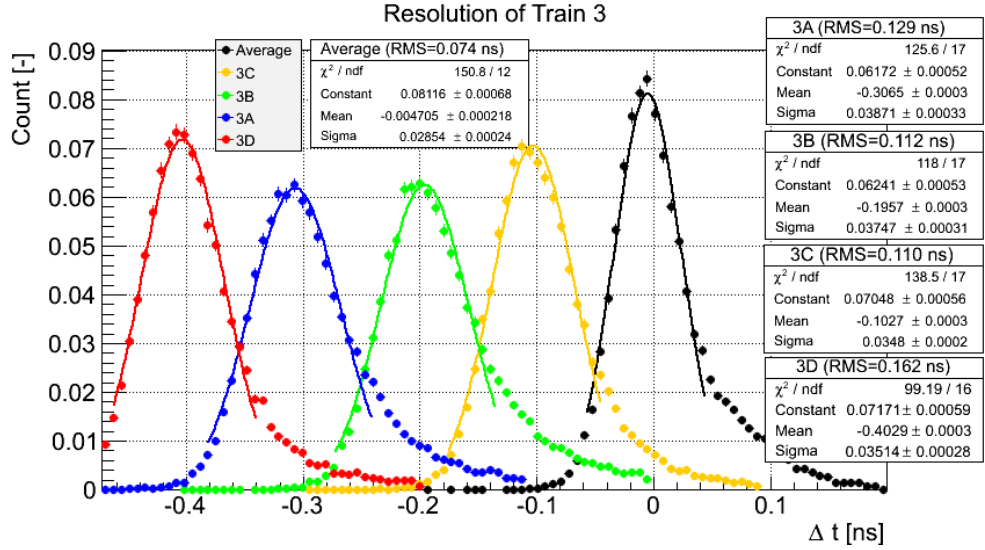
Figure 7.29: Time distributions of individual bars of train 3 and of the whole train (black) for the measurement at the edge, PMT 9002097. The mean values are shifted for clarity. The sigma values in the statistic boxes are not corrected for the SiPM contribution.
