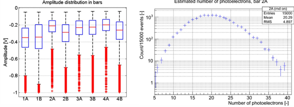
Figure 7.11: Left : Distribution of the amplitudes with the blue boxes representing the range from the 25 % to the 75 % quantile, the red line marking the mean value and the dotted line representing the distribution range excluding the outliers drawn as the red points. Right : Distribution of generated photoelectrons obtained from a Monte Carlo simulation [P3].
