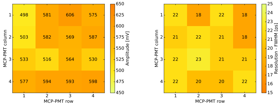
Figure 8.4: Uniformity of the MCP-PMT 9002053 response in terms of the output pulse amplitude ( left ) and the time resolution ( right ). The colormap is inverted between the two plots, as the resolution is expected to rise with decreasing amplitude.
