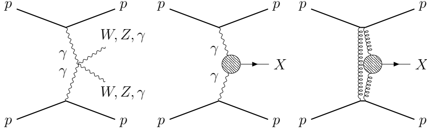
Figure 2.7: Feynman diagrams of processes with a potential to probe beyond the Standard Model physics. From left to right: diphoton production of diphoton, WW or ZZ ; diphoton production of an invisible particle X ; CEP of an invisible particle X .
