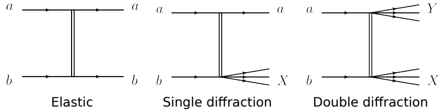
Figure 2.4: Illustration of elastic scattering, single and double diffractive dissociation [10].
