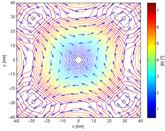
Figure 3.11: Visualization of the Q2 magnet field map. Contours show the value of the magnetic induction, arrows show the value and direction of the magnetic induction in the mesh points of the map.
