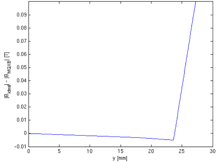
Figure 3.12: Difference between the magnetic induction value calculated by interpolating the field map and that of the ideal (analytical) quadrupole for x = 0 .
