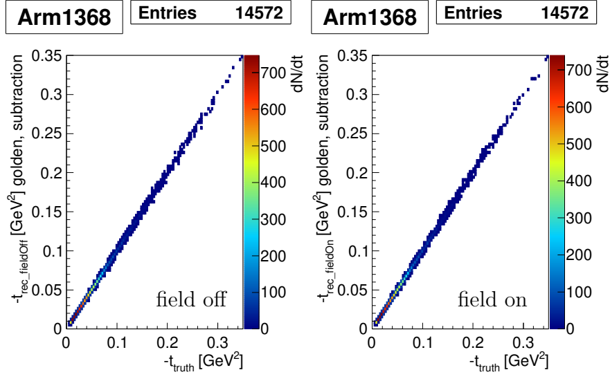
Figure 4.17: Migration between the true (generated) t values and the values reconstructed by the ALFA detectors for the two samples with the field off and on.
