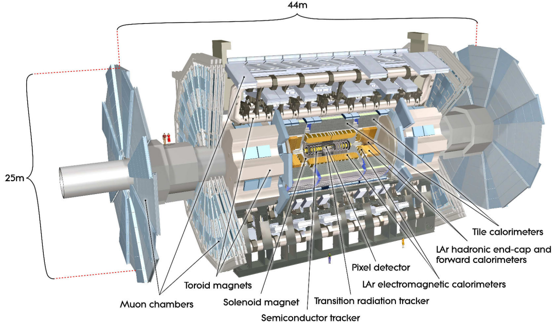
Figure 1.5: ATLAS experiment with a cut out part to see the inner composition of detector layers [1].
