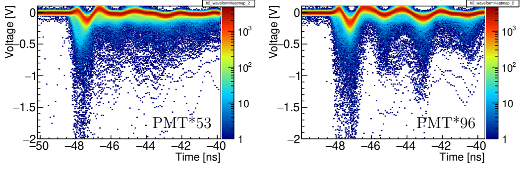
Figure 7.28: Raw crosstalk waveforms in bar 4B with signal in train 3 for MCP-PMT 9002053 ( left ) and 9002096 ( right ). There are 32768 waveforms overlaid in each plot and the color map shows the amount of overlaid waveform points.
