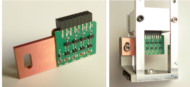
Figure 6.13: The first stage preamplifier (PAa) board with the heat sink (courtesy off Vladimír Urbášek).
