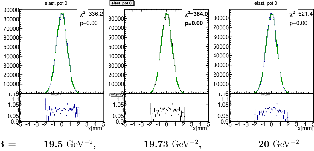
Figure 4.22: Effect of the B slope on the x distribution of hits in ALFA pot 0 in the MC sample (black) compared to the data sample (green). The bottom part of each histogram shows ratio of the counts in each bin for MC over data.
