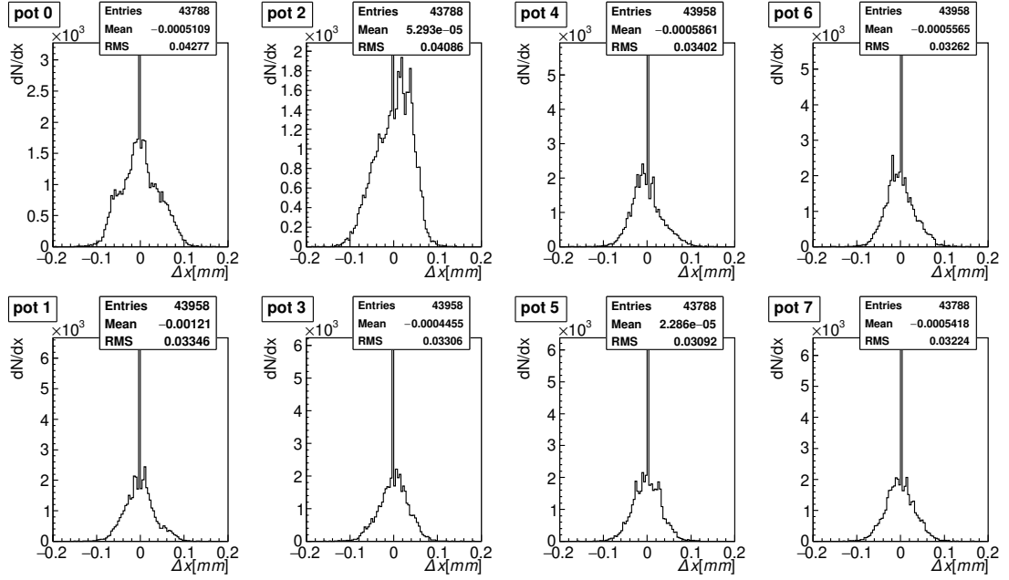
Event by event x difference for all pots: \Delta x = x_{\text{LHC\_fieldOff}} - x_{\text{LHC\_fieldOn}} ; golden elastic events.
