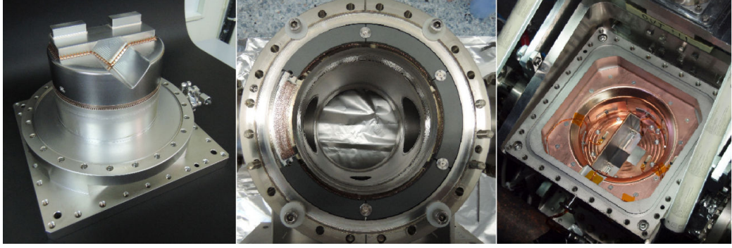
Figure 1.11: Modifications of the ALFA pot and station to lower RF heating. Left : RP filler placed on the original pot; middle : ferrite ring attached to the station flange; right : added copper inside the pot to improve heat transfer [P11].
