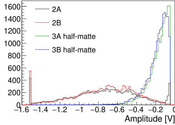
Figure 7.16: Signal amplitude distributions for bars of the train 2 (polished) and the train 3 (matte light guide). In both cases the HV was set to 1950 V. The negative polarity of the signal originates from the MCP-PMT output polarity.
