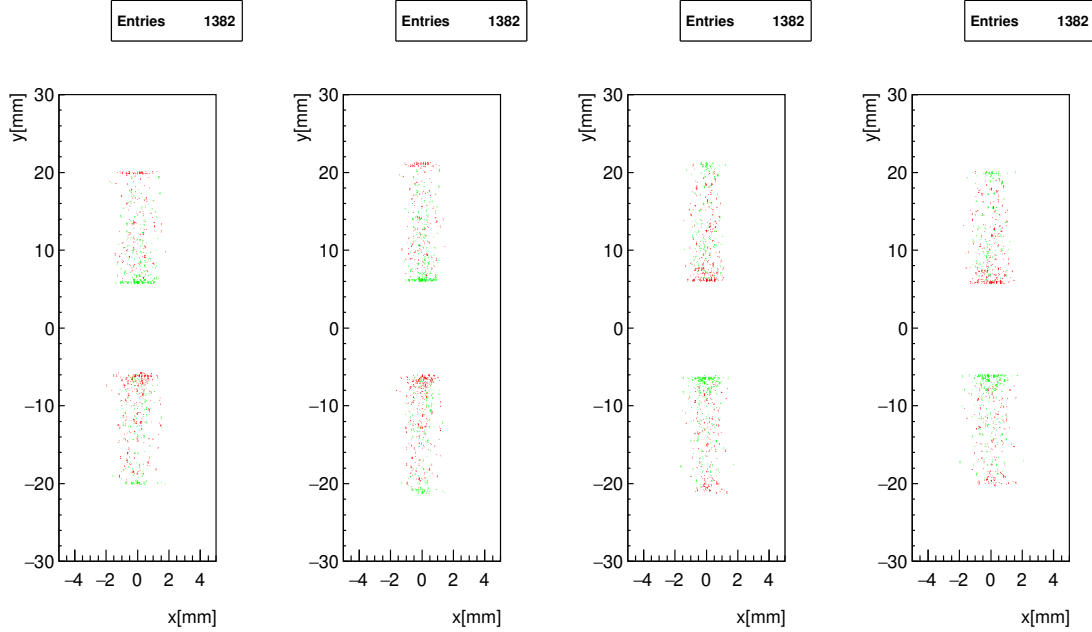
Figure 4.15: Positions of hits in events with a 4/4 track in the field off sample, but no 4/4 track in the field on sample (red), and in events with a 4/4 track in the field on sample, but no 4/4 track in the field ff sample (green).
