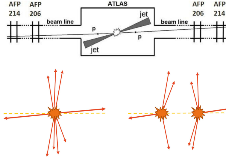
Figure 6.1: Illustration of a central diffraction event and two single diffraction events producing the same signature in AFP.
