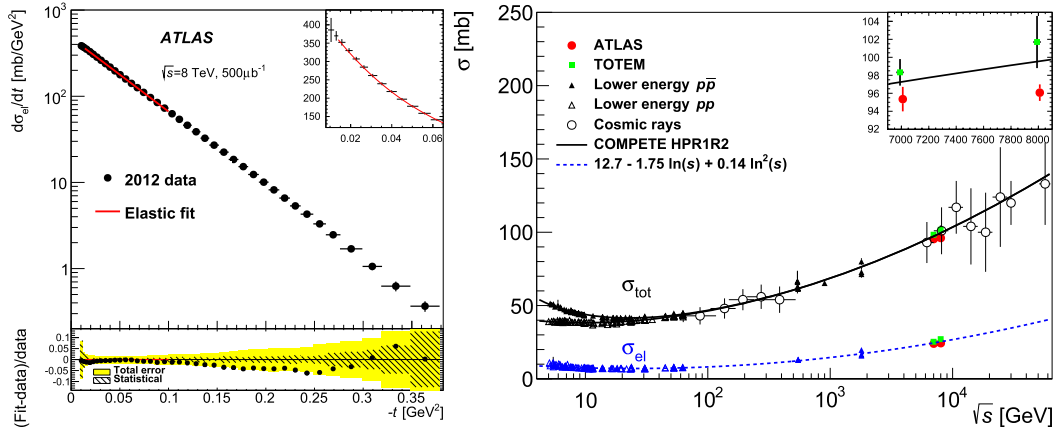
Figure 2.2: Left : Differential elastic cross section measured by ALFA with the fit using the theoretical prediction with free parameters \sigma_{\text{tot}} and B . The lower part shows the relative difference between the fit and the data with the yellow area representing the total uncertainty and the hatched area the statistical uncertainty. Right : Compilation of total and elastic cross section results as a function of the center-of-mass energy [P8].
