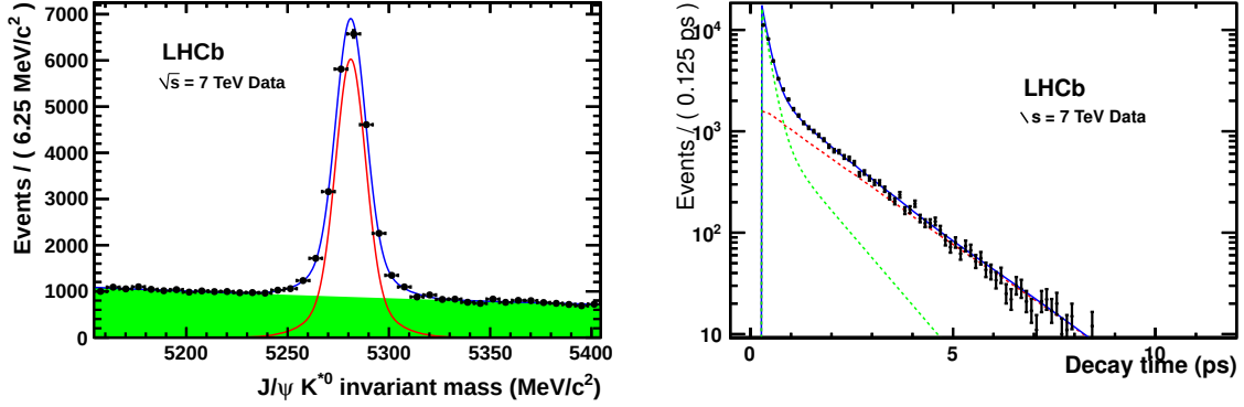
FIGURE A.7: Distribution of the reconstructed mass B^0 (left) and decay time (right) for the B^0 \rightarrow J/\psi K^{*0} channel for the events tagged by the OS. Black points are data, the blue curve is the fit result, red curve is the signal component, while the green line represents the sum of the two background components.
