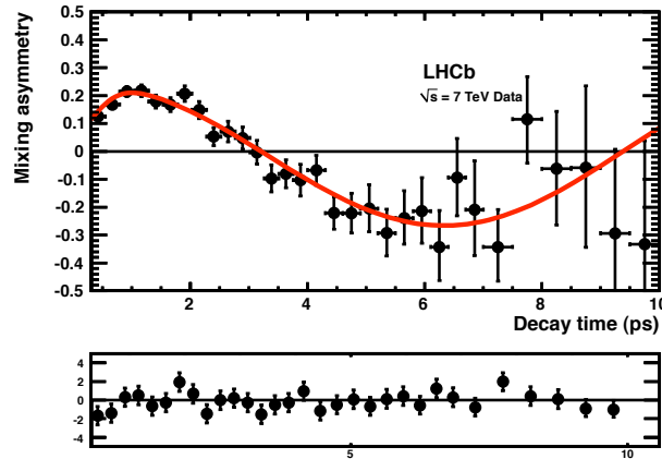
FIGURE A.8: Mixing asymmetry of the B^0 \rightarrow J/\psi K^{*0} events in the signal mass region, for all OS tagged events. Black points are data, red solid curve is the asymmetry of the fit function. The lower plot shows the pulls of the residuals with respect to the fitted function.
