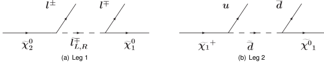
Figure 2.4: Possible decay chain in SU2 leading to jets and correlated opposite sign leptons.
