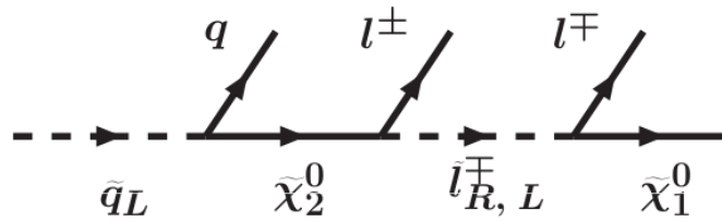
Figure 7.1: Signal decay chain for mass measurement of \tilde{\chi}_2^0
