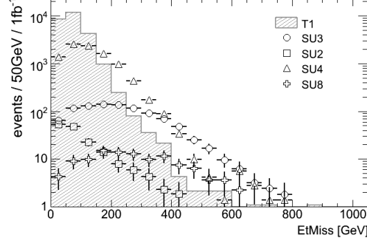
(a) Without extra generator-based cuts
