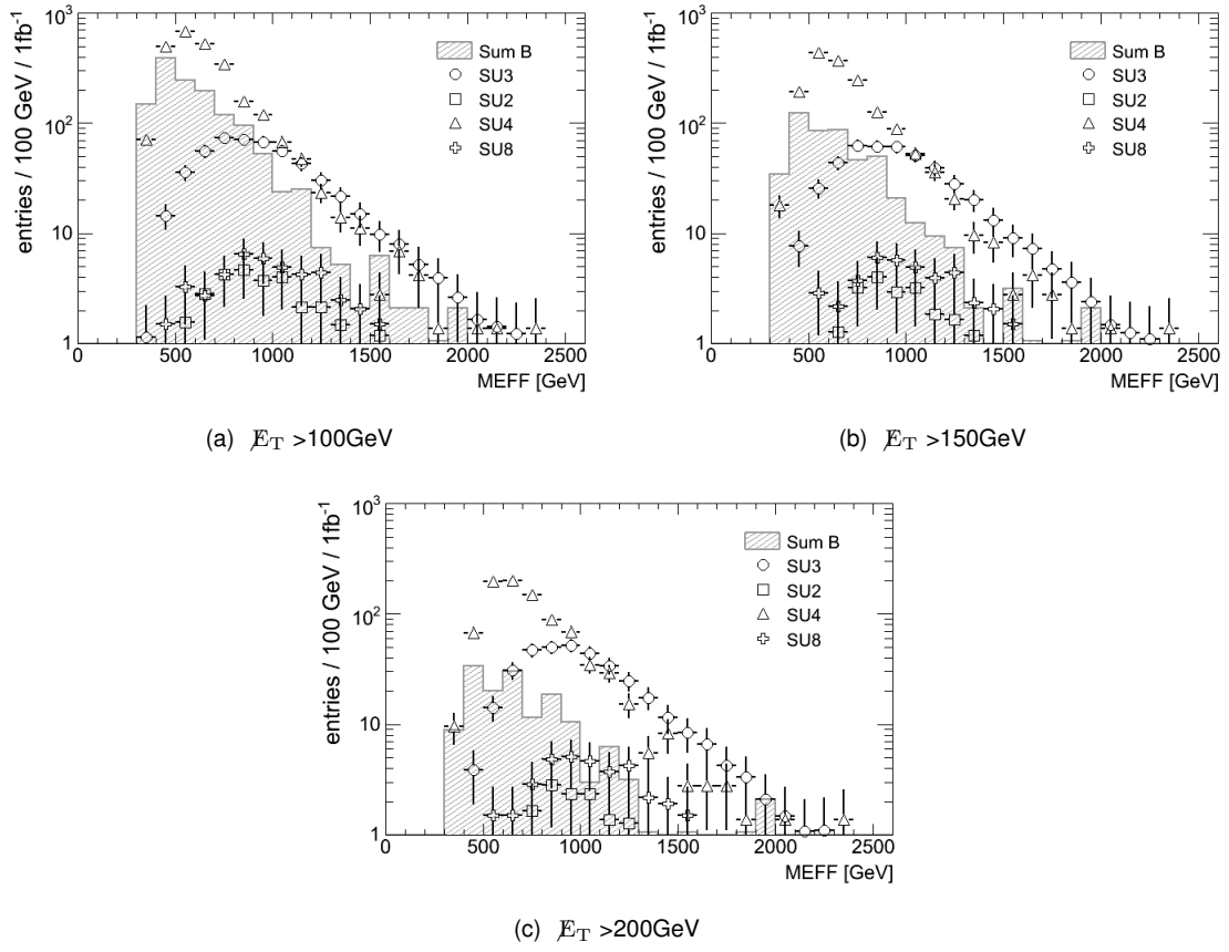
Figure 6.4: Effective mass when cutting on 3 values of \cancel{E}_T . 2 isolated leptons with opposite sign and extra generator-level cuts, a preselection of \cancel{E}_T > 100 \text{ GeV} , p_T^{jet1, jet2} > 100, 50 \text{ GeV} have been applied.
