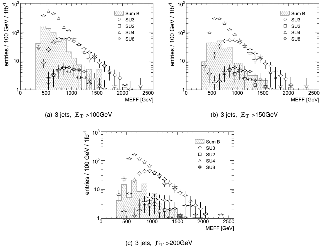
Figure 6.8: Effective mass distributions after 2 leptons of opposite sign have been required, and in addition 3 jets satisfying p_T^{JetAll} > 50 \text{ GeV} , p_T^{Jet1} > 100 \text{ GeV} . Plots show effect of \cancel{E}_T cut for \cancel{E}_T > (100, 150, 200) \text{ GeV}
