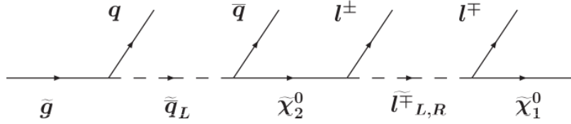
Figure 2.3: Decay of gluino through neutralino, leading to a finalstate with correlated opposite sign di-leptons.
