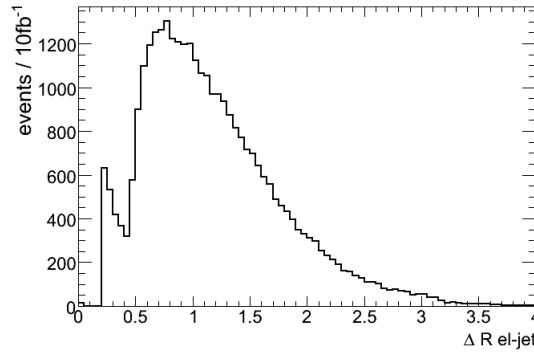
Figure 5.10: Angular distance \Delta R between the electron and the closest jet after electron-jet overlap removal but before lepton isolation.
