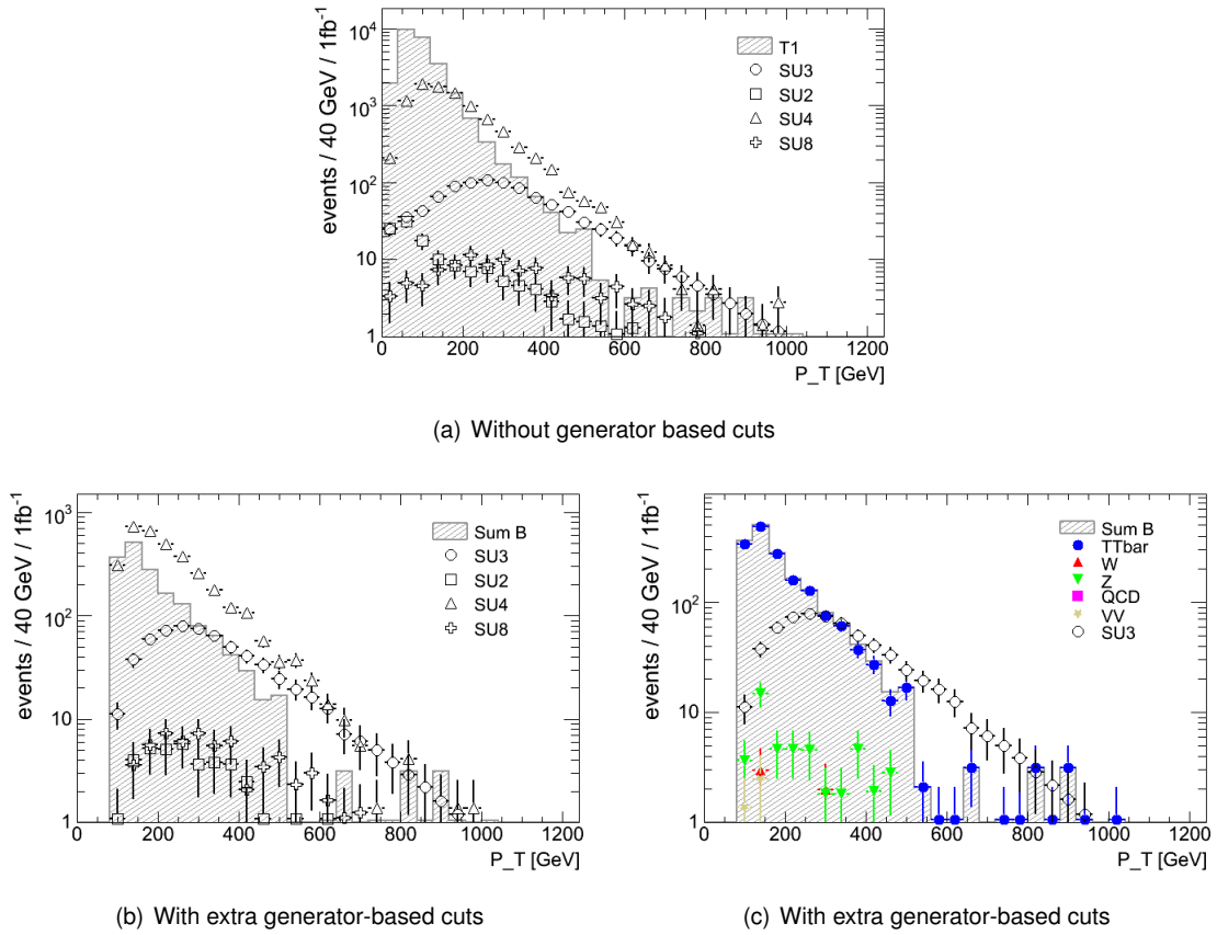
Figure 6.6: Transverse momentum p_T of the hardest jet in the event. Plot a) show SM (semi) leptonic t\bar{t} sample "T1" and for the various SUSY signal samples. Only requirement on event is at least 2 opposite signed well-defined leptons required. Plot b) shows various signal samples versus the sum of all backgrounds, plot b) shows the signal sample SU3 together with the sum of all backgrounds, and also each class of backgrounds separately. Event requirements for all 3 plots are at least 2 isolated opposite sign leptons, and for plot (b,c) additional generator-based cuts \cancel{E}_T > 100 GeV, p_T^{jet1, jet2} > 100, 50 GeV. SU1 and SU6 have similar distributions as SU3 and are therefore not shown.
