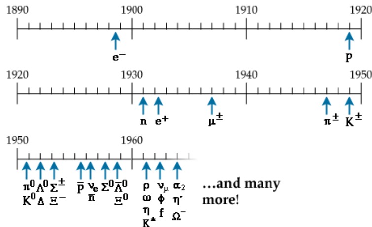
Figure 1.1: Particle Discoveries 1898-1964
