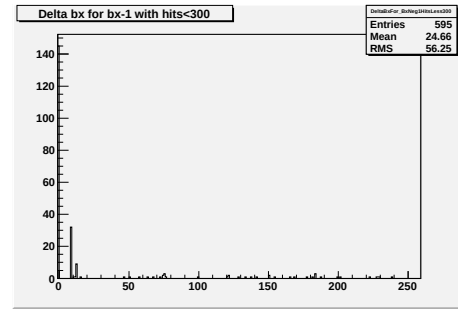
(b) Events with muons in bunch -1. "Normal" number of hits in DT. Small peak at small \Delta bx , but also plenty of events with large \Delta bx .
