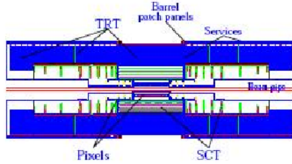
Figure 3.4: Layout of the inner detector showing the positioning of the pixel detector, the silicon strip detector (SCT) and the transition radiation tracker (TRT).
