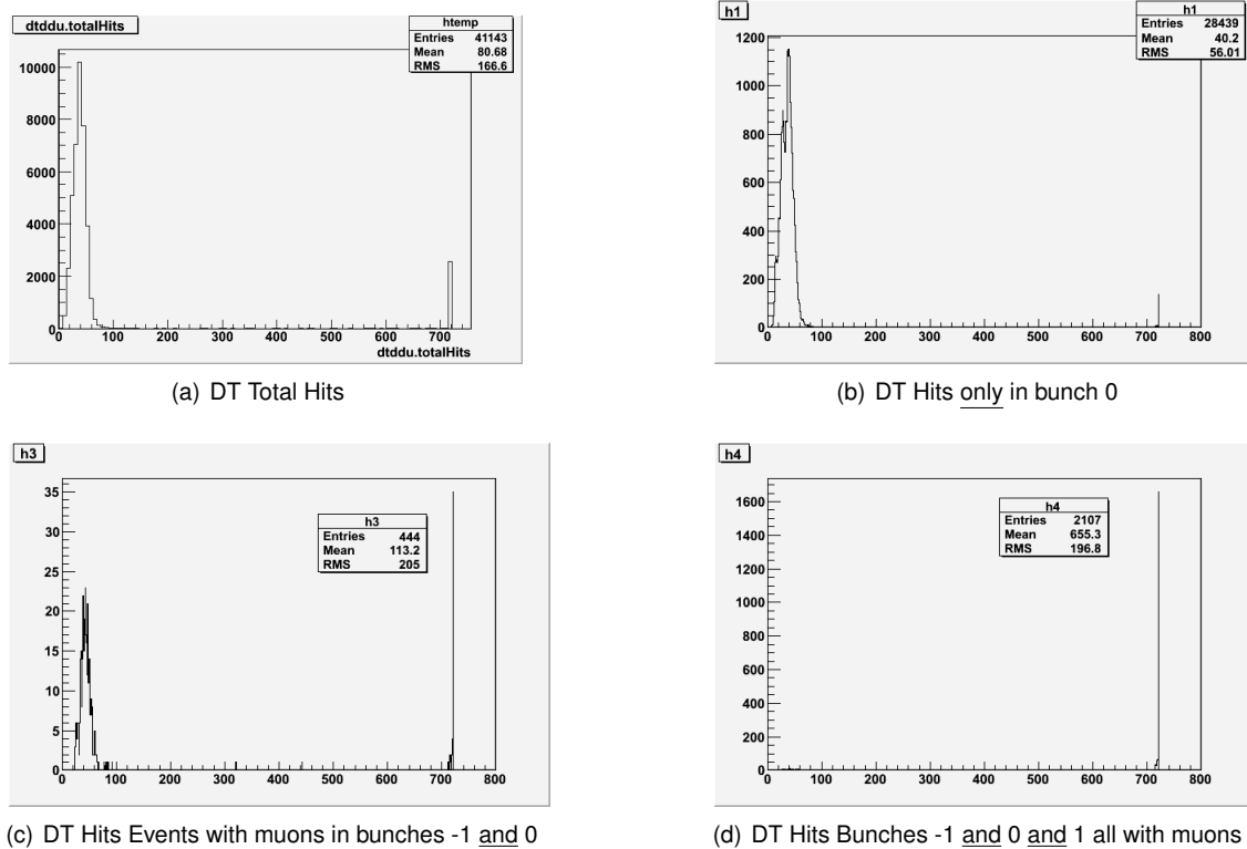
Figure A.4: Plots a-d show number of hits in the DT for the various classifications of events from July Run 14851. a) shows DT hits for all events. b) where only bunch 0 had events, notice the small number of noise-events with hits around 700. c) For events where there were muons in bunches -1 and 0 in the same event there was a large fraction of noise-events. It is still interesting that there were quite a number of events that were not obviously noise. d) shows DT hits for events that had muons in all bunches. The number of events that were not noise is vanishingly small.
