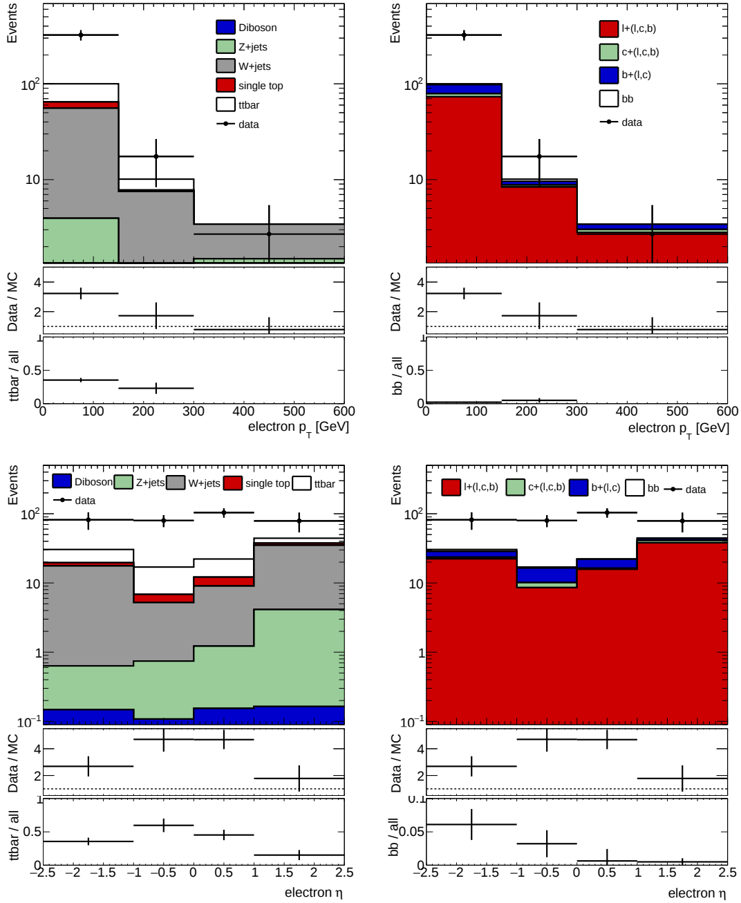
Figure A.2: The predicted distributions of the non-prompt electron p_T (top) and \eta (bottom) compared to ATLAS data from 2015 and 2016 in the SS region. Here, the simulated 0NPel component has been subtracted from both MC simulation and data. The remaining 1NPel prediction is split either by the contributing physics processes (left) or the contributing two jet flavour compositions (right). Correspondingly, the ratio plots show, in addition to the common data/MC ratio, either the amount of t\bar{t} events (left) or the amount of b\bar{b} events (right) compared to all simulated NPel events. Only statistical uncertainties from data and simulation are included in this comparison.
