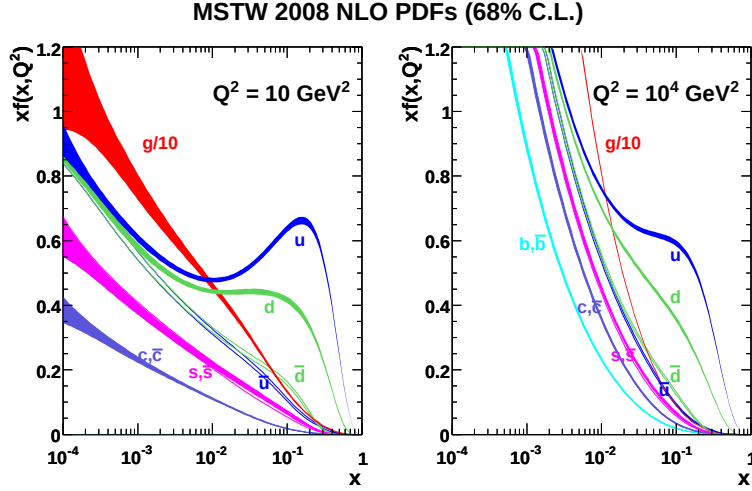
Figure 4.2: The momentum density xf of the parton is plotted as a function of its momentum fraction x . Here, the prediction of f is taken from [38] at a momentum transfer of Q^2 = 10 \text{ GeV}^2 (left) and Q^2 = 10^4 \text{ GeV}^2 (right) at NLO precision.
