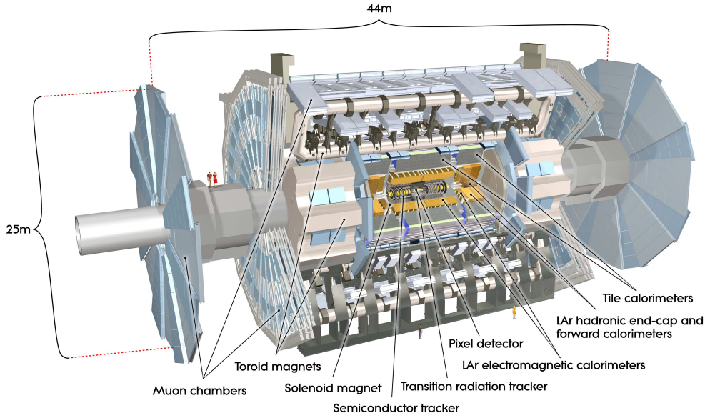
Figure 3.2: The different parts of the ATLAS detector at the LHC. © 2008-2019 CERN
