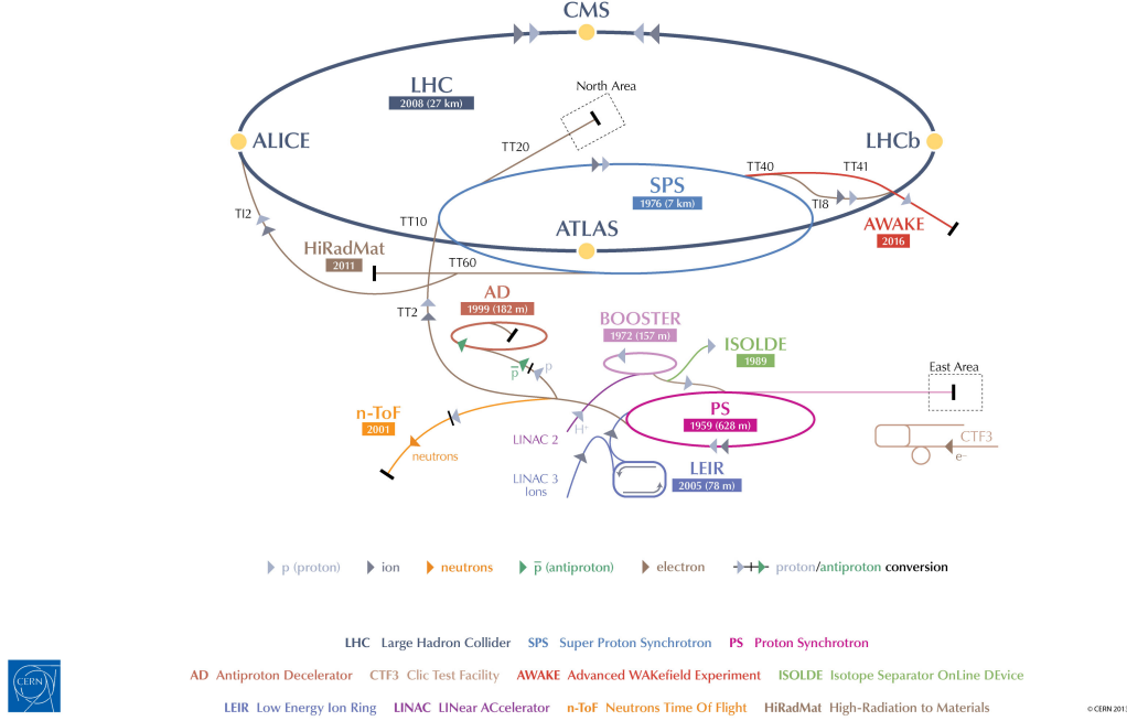
Figure 3.1: A sketch of the CERN accelerator complex at the France-Switzerland border near Geneva. Shown are the four interaction points of the LHC which mark the four main experiments at the LHC, namely ATLAS, CMS, ALICE and LHCb. Also shown are some of the other experiments at CERN as well as additional structures that pre-accelerate and feed the protons into the LHC tunnel. © 2013-2019 CERN.
