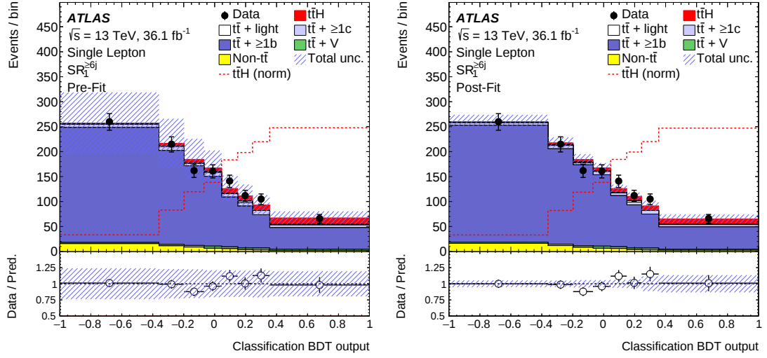
Figure 11.5: Comparison of the predicted event yields to the observed events in data as a function of the Classification BDT output in the single lepton \text{SR}_1^{\geq 6j} before (left) and after the combined fit (right). The filled red area represents the t\bar{t}H signal stacked on top of the background normalised to the SM cross-section before the fit and to the extracted \mu value after the fit. The dashed red line shows the t\bar{t}H signal separately, normalised to the total background prediction. The total uncertainty in the simulated yields is represented by the hatched area, while the histograms before the fit do not consider an uncertainty in the t\bar{t} + \geq 1b and t\bar{t} + \geq 1c normalisations.
