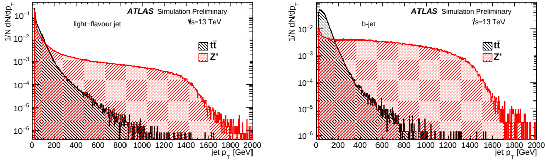
Figure 6.4: The normalised differential cross-section of the light-jet p_T (left) and b -jet p_T (right) spectra [68]. The simulated t\bar{t} sample contributes mostly to jets with p_T \leq 250 GeV (black). Therefore, an additional sample of simulated Z' decays is added to increase the number of jets with a higher p_T (red).
