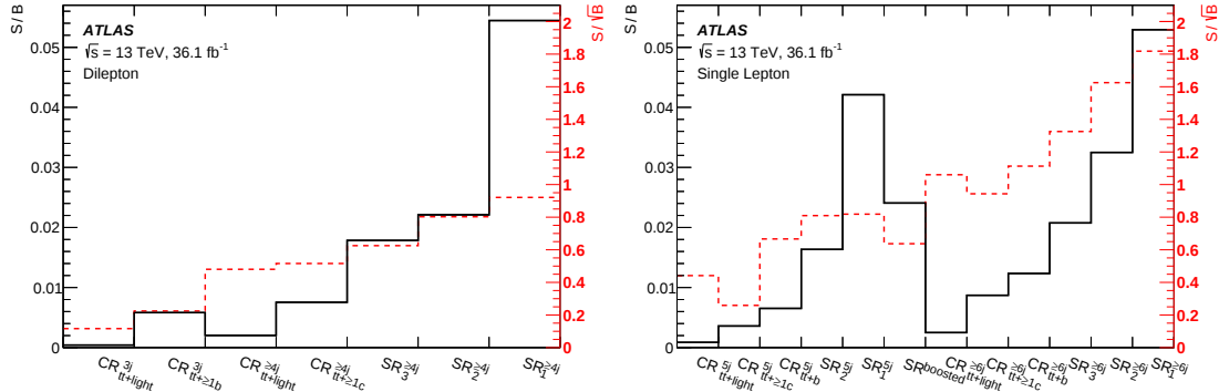
Figure 8.4: The signal-to-background ratio (solid black) and its significance (dotted red) are shown for each of the dilepton (left) and single lepton (right) regions.
