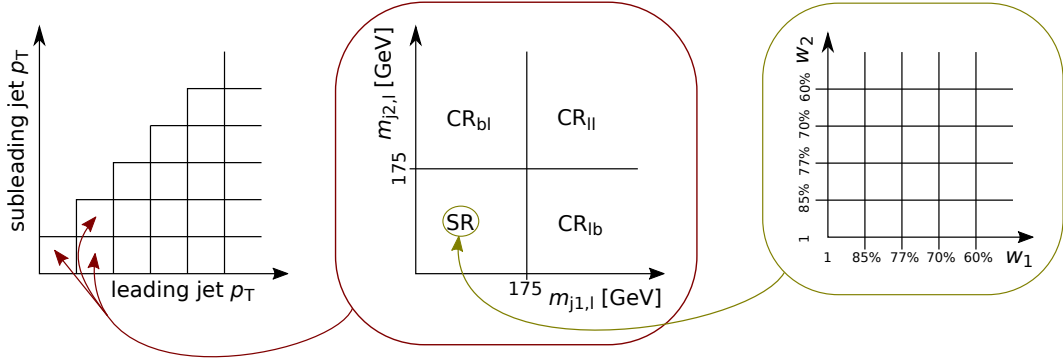
Figure 6.8: A schematic of how the various signal and control regions of each event are selected according to the leading and subleading jet and the corresponding m_{j,l} quantities. The b -tagging efficiencies are then extracted for leading and subleading jet from the SR for each WP. This schematic is included with the courtesy of Julian Schmoeckel (DESY).
