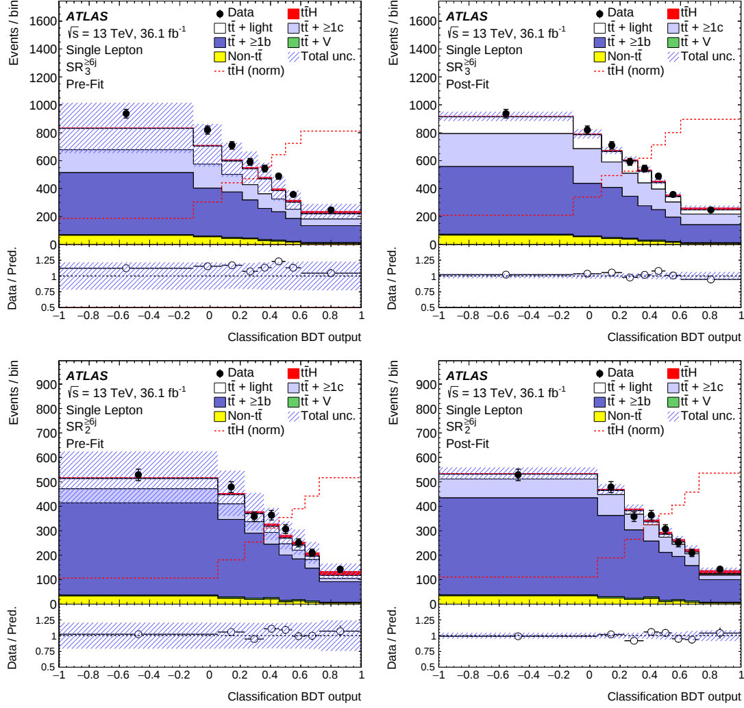
Figure 11.4: Comparison of the predicted event yields to the observed events in data as a function of the Classification BDT output in the single lepton \text{SR}_3^{\geq 6j} before (top left) and after the combined fit (top right) and in the single lepton \text{SR}_2^{\geq 6j} before (bottom left) and after the combined fit (bottom right). The filled red area represents the t\bar{t}H signal stacked on top of the background normalised to the SM cross-section before the fit and to the extracted \mu value after the fit. The dashed red line shows the t\bar{t}H signal separately, normalised to the total background prediction. The total uncertainty in the simulated yields is represented by the hatched area, while the histograms before the fit do not consider an uncertainty in the t\bar{t} + \geq 1b and t\bar{t} + \geq 1c normalisations.
