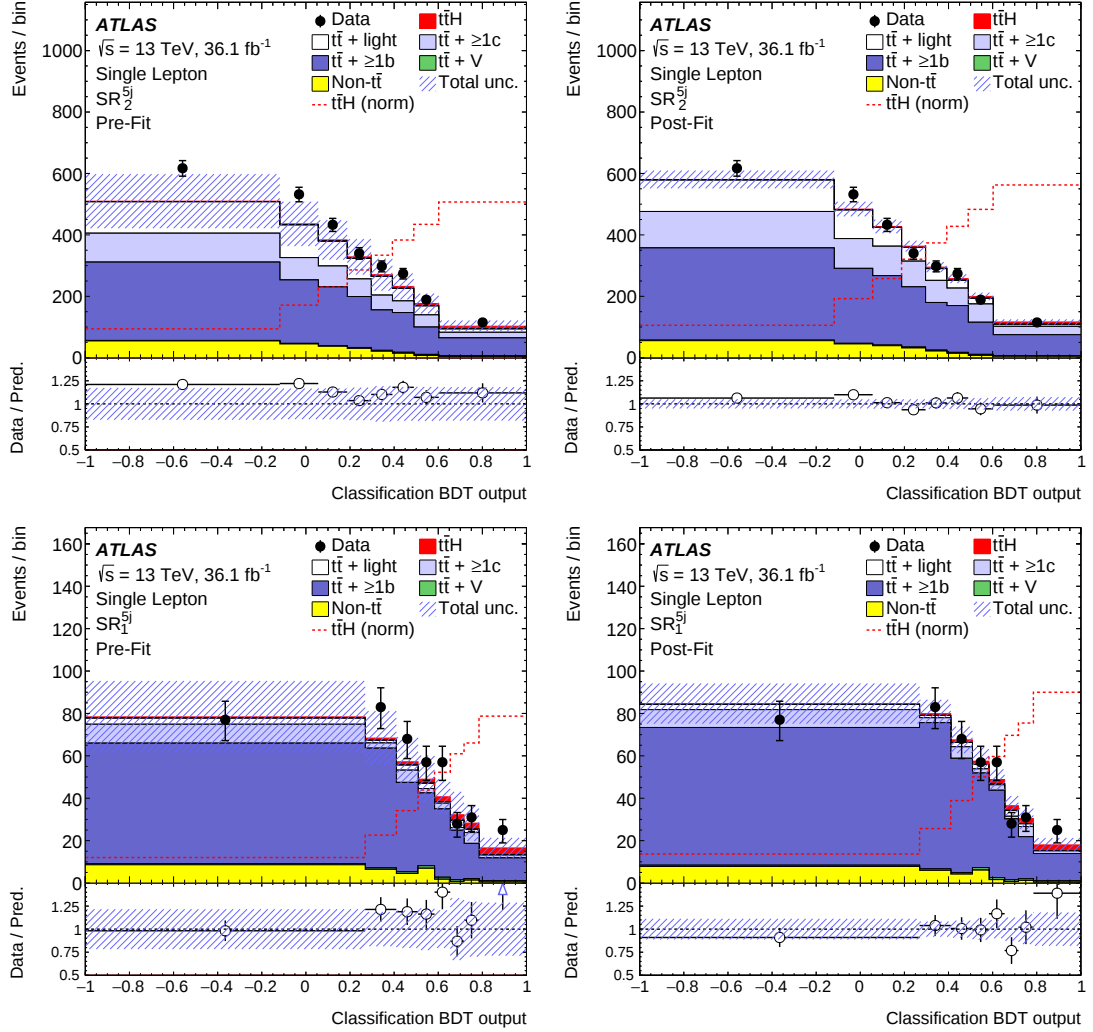
Figure 11.3: Comparison of the predicted event yields to the observed events in data as a function of the Classification BDT output in the single lepton SR_2^{5j} before (top left) and after the combined fit (top right) and in the single lepton SR_1^{5j} before (bottom left) and after the combined fit (bottom right). The filled red area represents the t\bar{t}H signal stacked on top of the background normalised to the SM cross-section before the fit and to the extracted \mu value after the fit. The dashed red line shows the t\bar{t}H signal separately, normalised to the total background prediction. The total uncertainty in the simulated yields is represented by the hatched area, while the histograms before the fit do not consider an uncertainty in the t\bar{t} + \geq 1b and t\bar{t} + \geq 1c normalisations.
