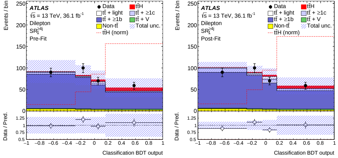
Figure 11.7: Comparison of the predicted event yields to the observed events in data as a function of the Classification BDT output in the dilepton \text{SR}_1^{\geq 4j} before (left) and after the combined fit (right). The filled red area represents the t\bar{t}H signal stacked on top of the background normalised to the SM cross-section before the fit and to the extracted \mu value after the fit. The dashed red line shows the t\bar{t}H signal separately, normalised to the total background prediction. The total uncertainty in the simulated yields is represented by the hatched area, while the histograms before the fit do not consider an uncertainty in the t\bar{t} + \geq 1b and t\bar{t} + \geq 1c normalisations.
