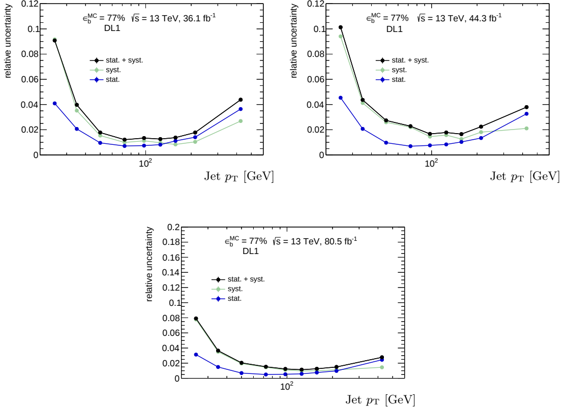
Figure C.3: The uncertainty components relative to the extracted b -tagging efficiency as a function of the jet p_T from the LH fit method to data for the DL1 algorithm at the 77% WP. Shown are the statistical uncertainty from data (blue), the total systematic uncertainty (green) and their sum in quadrature (black). The uncertainty estimations are based on the fit to ATLAS data from the years 2015 and 2016 (top left), 2017 (top right) and all three years combined (bottom).
