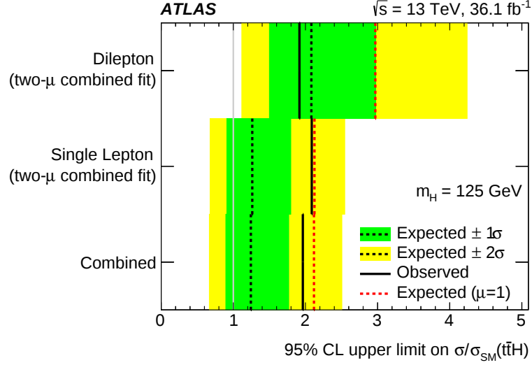
Figure 11.11: Shown are the upper limits on the signal strength at 95% CL for the individual channels and the combined result [4]. The individual limits are derived using the same approach as the quoted \mu values in Equation 11.3. The black solid line represents the observed limits, while the black (red) dotted line shows the expected limits for the background-only (signal-plus-background) hypothesis. The green (yellow) area depicts the 1\sigma ( 2\sigma ) uncertainty range on the expected limits for the background-only hypothesis.
