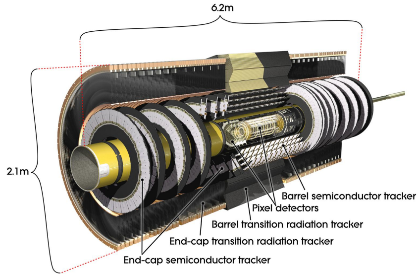
Figure 3.6: Cutaway view of the ATLAS inner detector, showing the layout of the pixel detector, SCT and TRT [59].
