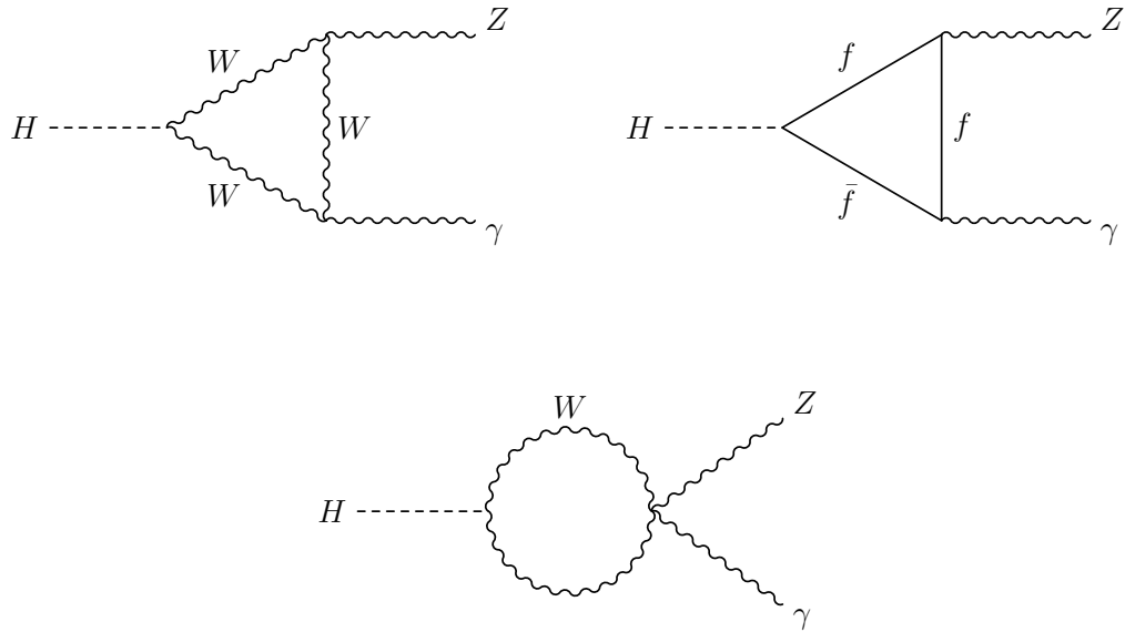
Figure 2.6: Summary of the H \rightarrow Z\gamma decay process.
