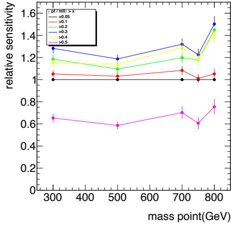
Figure 7.7: Relative variation in \varepsilon_S/\sqrt{\varepsilon_B} as a function of the resonance mass for given p_T^\gamma/m_{\ell\ell\gamma} cut values [119].
