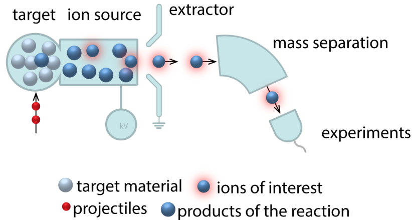
Figure 2.1: Schematic drawing of the processes needed to product the RIB via the ISOL method. In the target the projectiles create the primary products, which are then ionized, extracted and mass separated. The experimental chambers are reached at the end.
