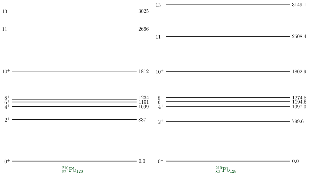
Figure 4.12: Experimentally deduced level scheme for the ^{210}\text{Pb} (right), compared with ( g_{9/2} , i_{11/2} , d_{3/2} , d_{5/2} , g_{7/2} , s_{1/2} , j_{15/2} ) shell-model calculations with the Kuo-Herling interaction (left).
