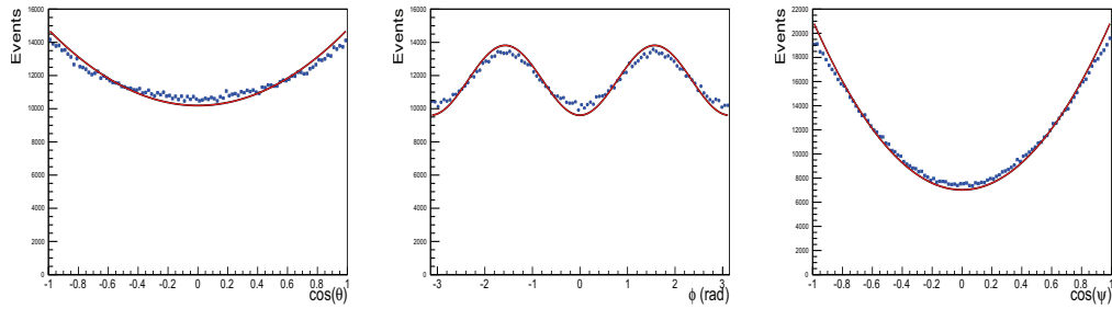
Figure 3.16: Distribution of angular variables, from left to right \cos(\theta) , \phi and \cos(\psi) . The red line is the projection of the theoretical differential decay rate, where the data points are the reconstructed angular variables (MC10).
