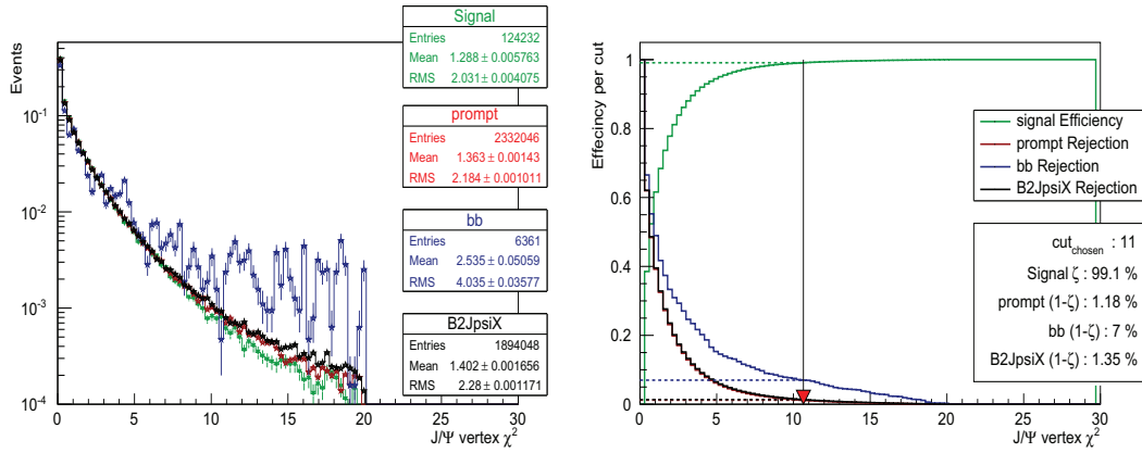
Figure 3.4: Left: J/\psi vertex \chi^2/\text{nDoF} distribution for B_s^0 \rightarrow J/\psi\phi signal candidates (green), b\bar{b} inclusive candidates (blue), B_{u,d,s} \rightarrow J/\psi X candidates (black), and prompt inclusive J/\psi candidates. Right: signal efficiency and individual background rejection ratios per cut. the best cut chosen is, \chi^2_{\text{vertex}}/\text{nDoF} < 11 .
