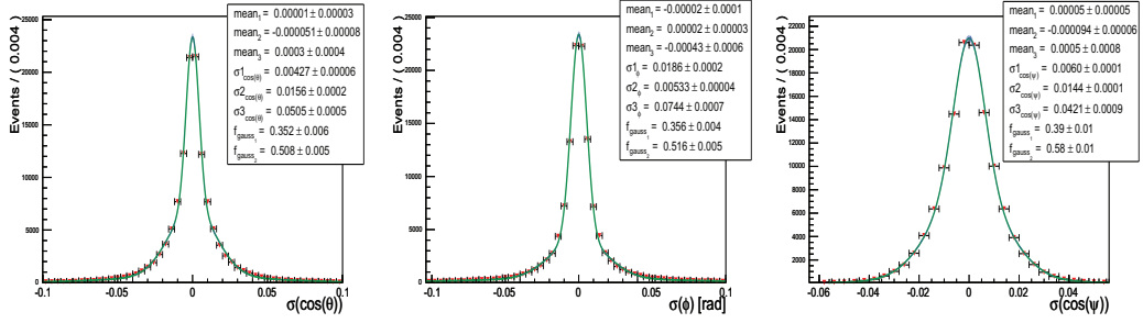
Figure 3.18: Distributions of angular variables resolution, Left: distribution of \cos(\theta) resolution where \langle \sigma_{\cos(\theta)} \rangle = 0.022 . Center: distribution of \phi resolution, where \langle \sigma_{\phi} \rangle = 0.029 rad. Right: distribution of \cos(\psi) resolution where \langle \sigma_{\cos(\psi)} \rangle = 0.014 (MC10).
