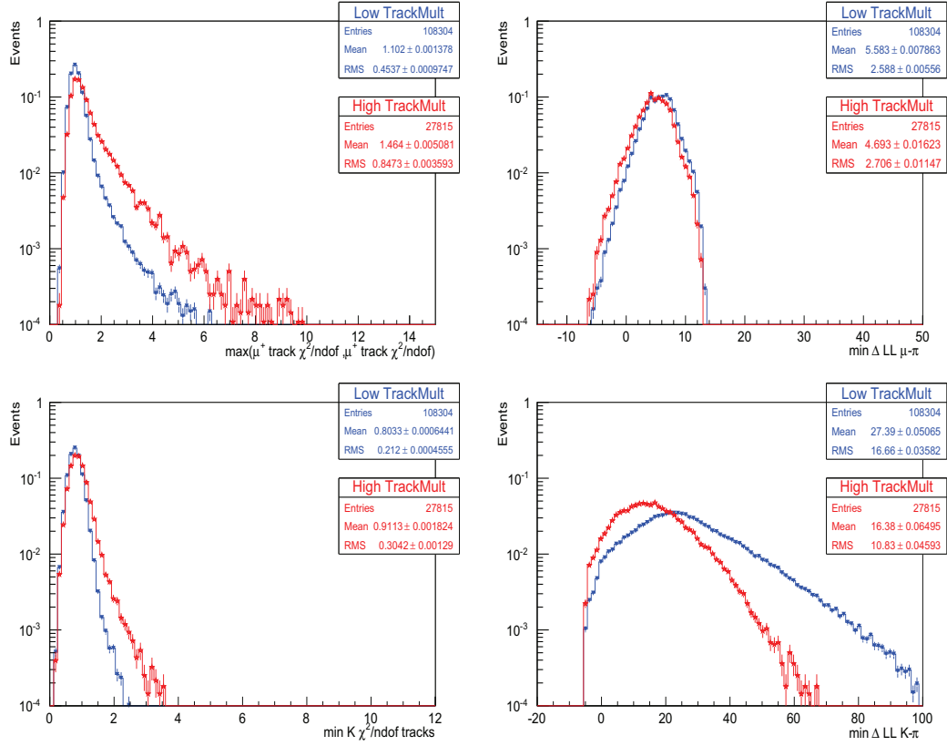
Figure 3.24: Maximum of \chi^2_{\text{track}}/\text{nDoF} distribution (left). Minimum of muons \Delta \ln \mathcal{L}_{\mu\pi} distribution (right). The top row is for muons and the bottom for kaon. High multiplicity variable distributions in red, low multiplicity distribution in blue (MC2010).
