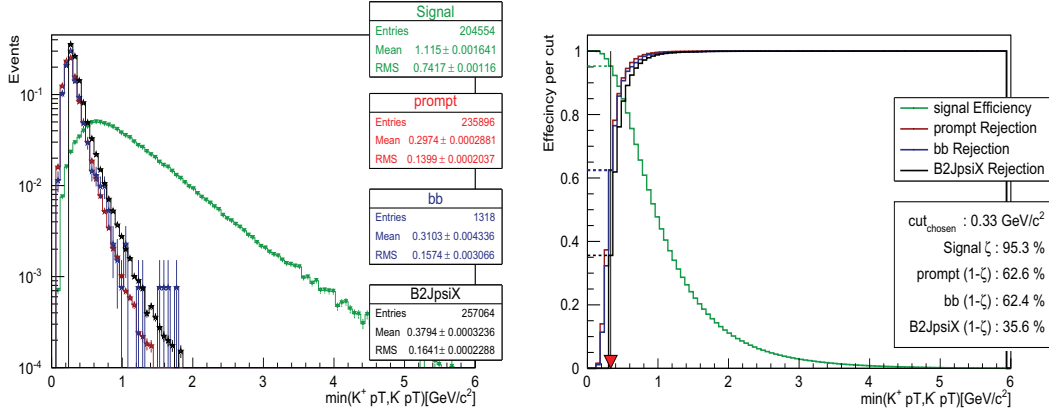
Figure 3.29: Left: distribution of the minimum kaons' p_T for B_s^0 \rightarrow J/\psi \phi signal candidates (green), b\bar{b} inclusive candidates (blue), B_{u,d,s} \rightarrow J/\psi X candidates (black), and prompt inclusive J/\psi candidates. Right: signal efficiency and individual background rejection rates per cut.
