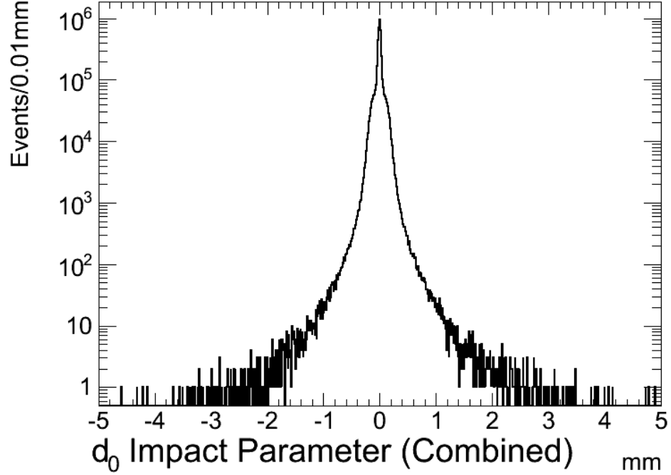
Figure 6.8: Transverse impact parameter distribution for Combined muons.
