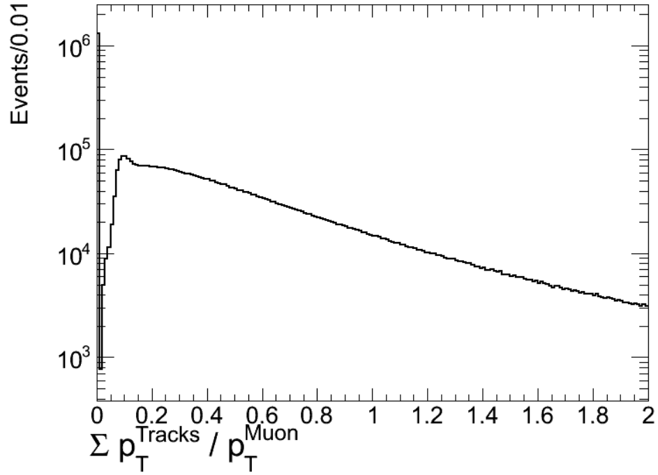
Figure 6.10: Distribution of the isolation variable. This follows the application of the previous cuts up to the Combined quality on muons.
