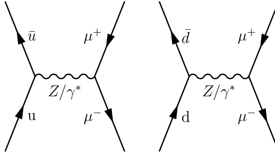
Figure 2.4: Muon pair production through mediation of both Z bosons and photons. (The \gamma^* notation indicates that the photon is produced off the mass shell.) The two processes also produce an interference term.
