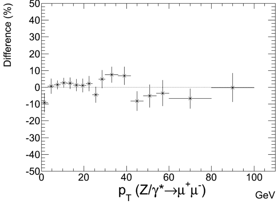
Figure 7.6: Percent difference between reference study and PYTHIA. \frac{\text{PYTHIA} - \text{ATLAS}}{\text{PYTHIA}} plotted as a function of the transverse momentum with the ATLAS study errors applied as symmetric uncertainties.
