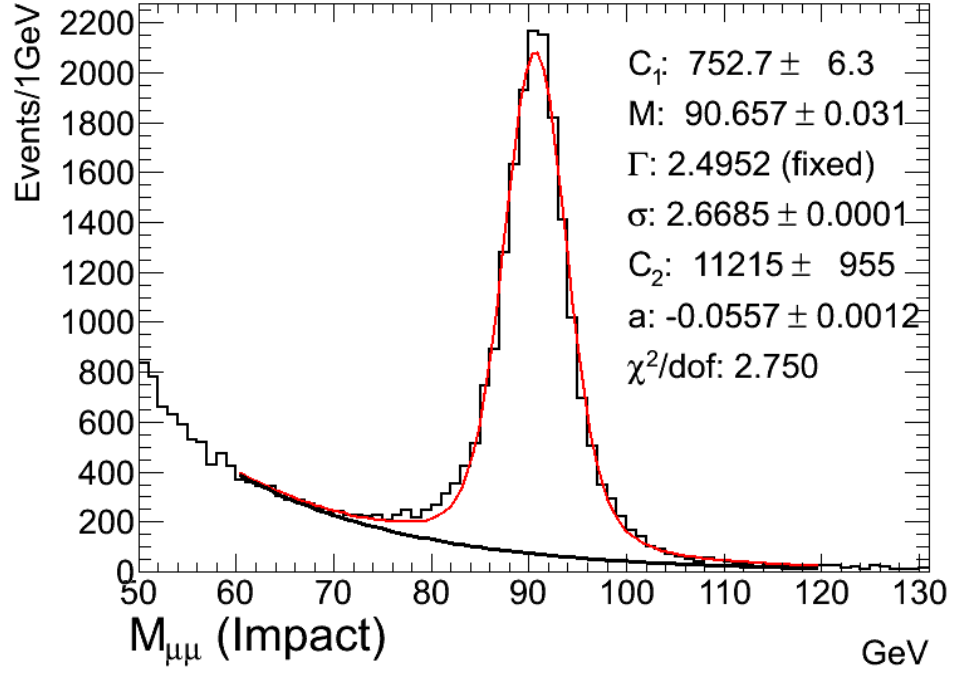
Figure 6.7: Dimuon invariant mass after an impact parameter requirement. Both muons are required to satisfy |d_0| < 1 \text{ mm} and |z_0| < 5 \text{ mm} . In the region 60 < M_{\mu\mu} < 120 \text{ GeV} there are 6865 events classified as background leaving 18515 events as signal.
