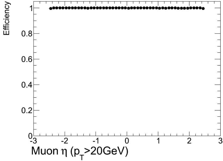
Figure 6.23: Inner detector efficiency as a function of muon pseudorapidity.
