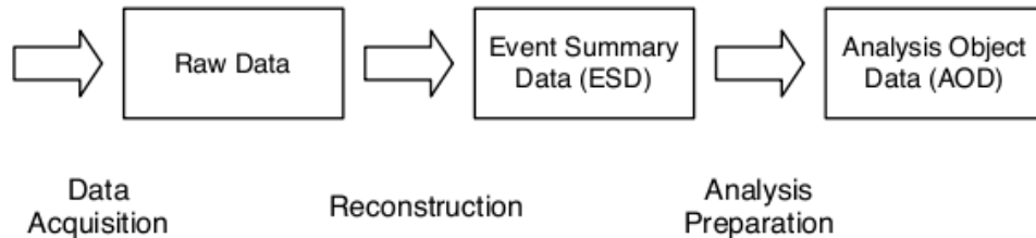
Figure 4.6: Flow of data file production [41].
