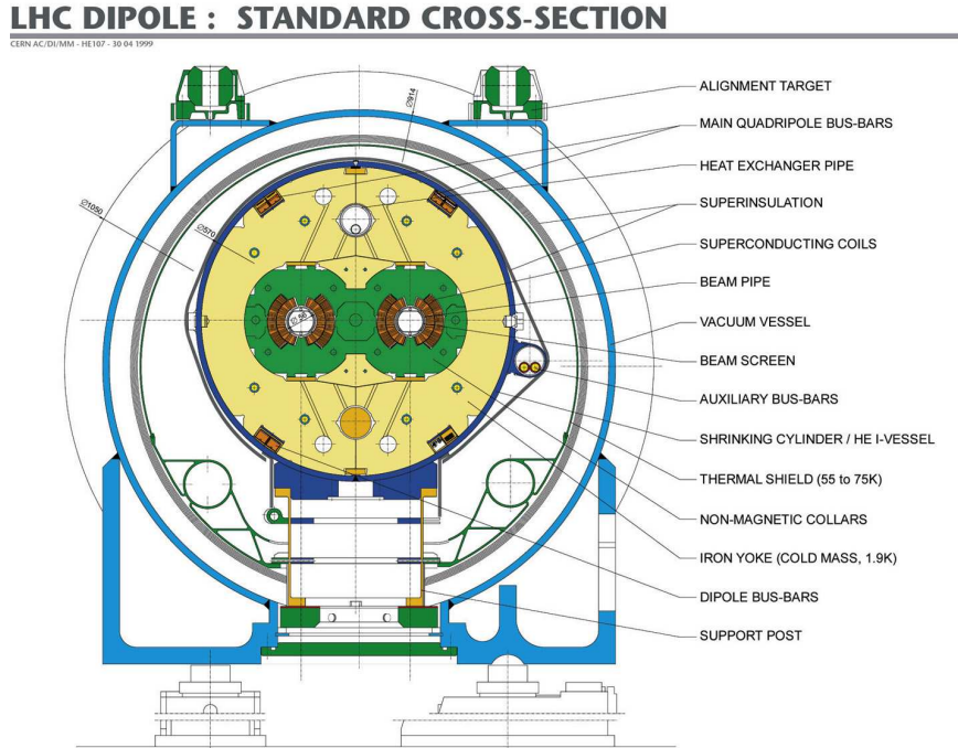
Figure 3.3: LHC superconducting dipole magnet [15].
