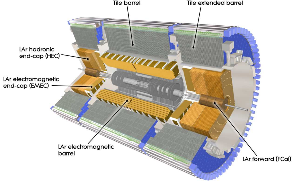
Figure 4.2: ATLAS calorimeters [27].
