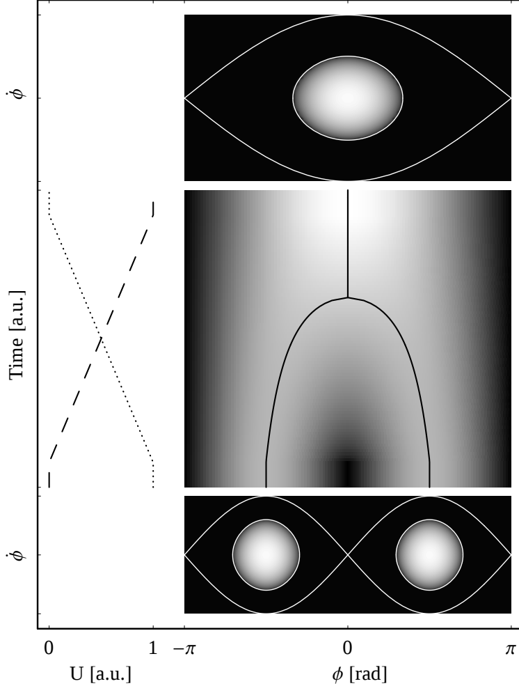
Fig. 3.3: Evolution of RF amplitudes (left, dashed and dotted), separatrix function and bucket center position (continuous) with time during bunch pair merging (time goes from bottom to top) or bunch pair splitting (time goes from top to bottom). The gray level is proportional to the height of the separatrix function \dot{\phi}(\phi) .
