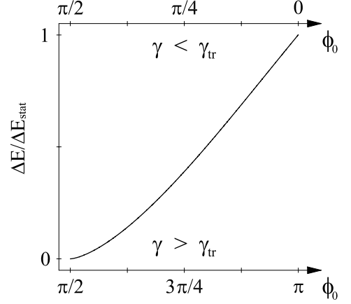
Fig. 2.4: Relative bucket height versus synchronous phase \phi_0 .
