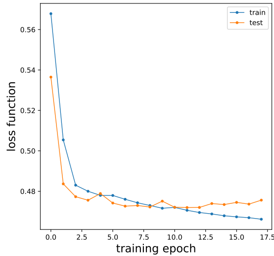
Figure 6.8: The loss function of the final optimisation of the model. The loss on the training set is shown in blue, the validation set in orange. In general, we see a relatively good convergence of the model after approximately 10-15 optimisation epochs. There is a small amount of over-training present after ten epochs, as visible from the increasing loss function on the test set.
