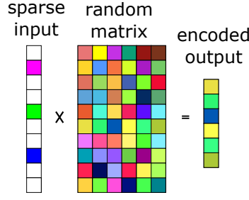
Figure 6.5: An illustration of the sparse coding technique using random projections. In this example, we encode a 3-sparse 10-dimensional signal to a 6-dimensional space using a matrix of Gaussian distributed weights.
