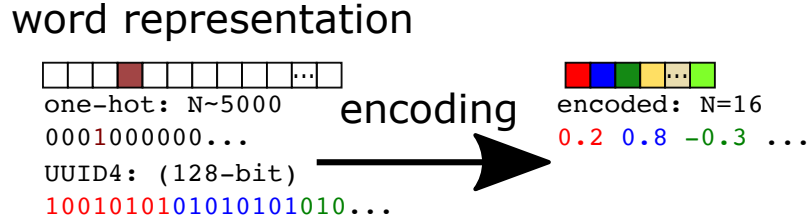
Figure 6.6: The word embedding scheme, where we use the 128-bit unique UUID4 representation to construct an encoded representation of 16 8-bit floats in the range [-1, +1] . The actual bit strings and floating point values are illustrative.
