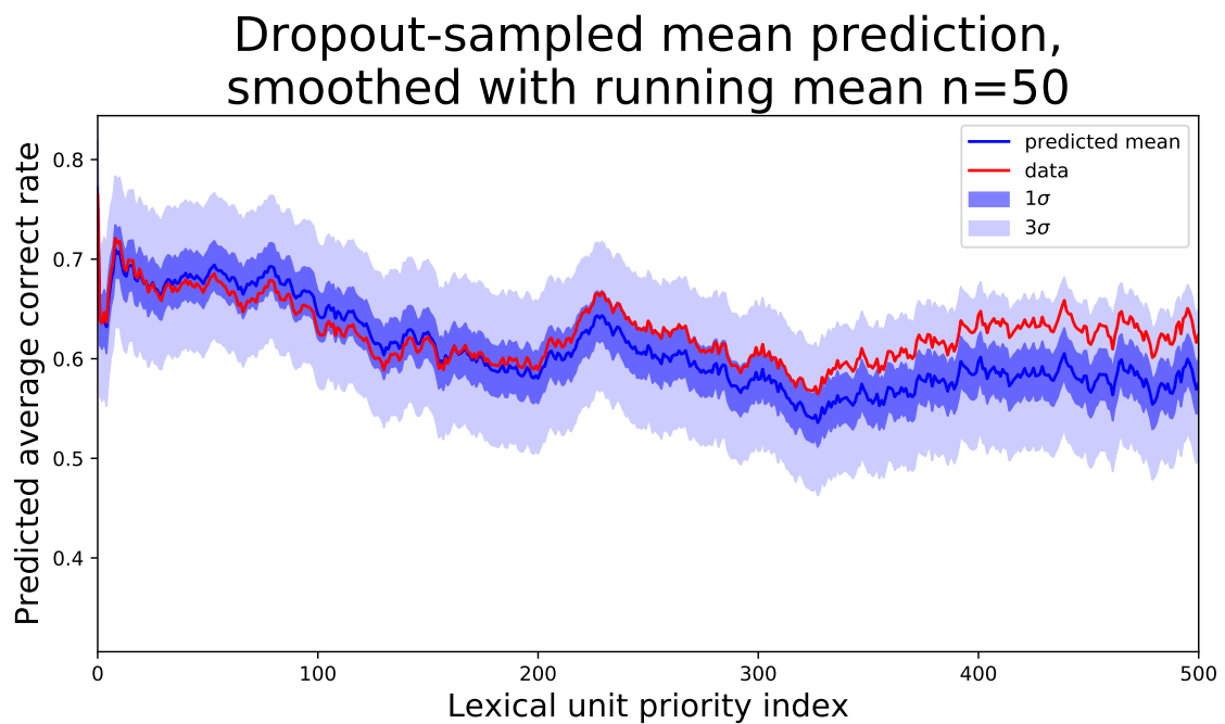
Figure 6.15: The predicted (blue) and true (red) guess probability as a function of LU priority index for the first 500 LUs. We see that the prediction is generally sufficiently close to the true mean correct rate, but trends somewhat lower than the data.
