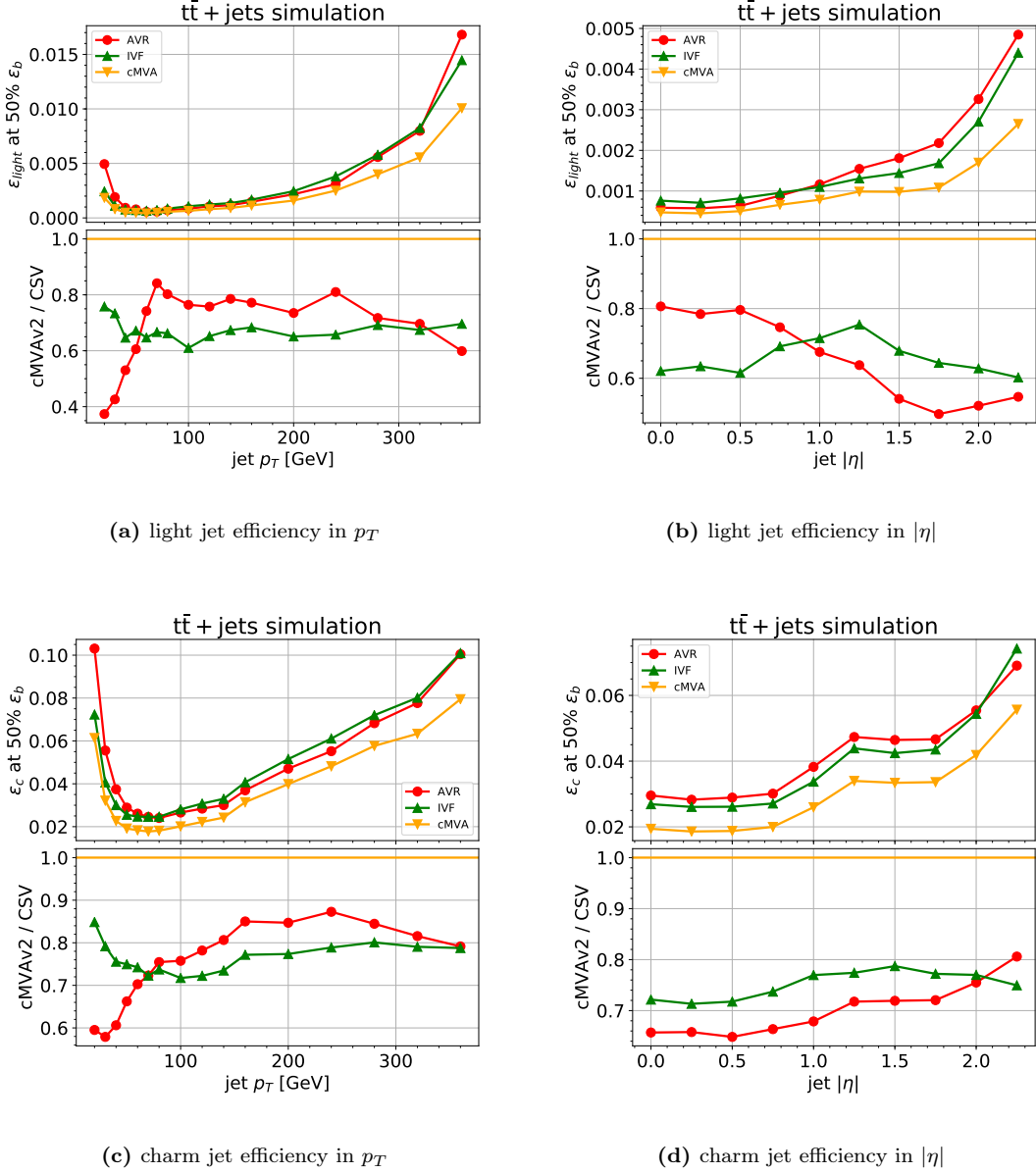
Figure 3.10: The p_T and |\eta| -dependent mistagging efficiency \epsilon_{\text{light}} , \epsilon_c at a fixed b-jet efficiency \epsilon_b in t\bar{t} + jets simulation. We compare the cMVA v2 discriminator to the CSV IVF and AVR discriminators in terms of the light jet and charm jet efficiency (mistagging) at the working point with 50% b jet efficiency. We see that the cMVA v2 discriminator performs well over a wide p_T and |\eta| range, with \epsilon_{\text{light}} in the forward region being around 40% lower than for the CSV algorithm. While the efficiency of the discriminator overall still depends on jet kinematics due to the inherent correlation between the kinematics and the underlying variables sensitive to b tagging, the dependence is somewhat lower for cMVA v2 than for CSV.
