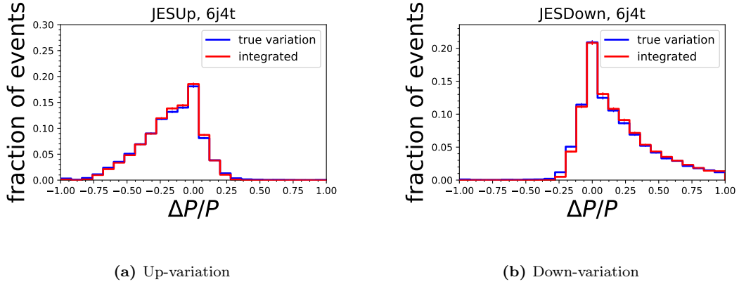
Figure 4.6: The effect of JES up and down variations on the MEM signal probability P_{\text{t}\bar{\text{t}}\text{H}(\rightarrow\text{b}\bar{\text{b}})} for the signal hypothesis with the full computation (blue) and with the vector integration approximation method. We see that both the up and down shifts have the correct direction and magnitude. This estimation is done on \text{t}\bar{\text{t}}\text{H}(\rightarrow\text{b}\bar{\text{b}}) simulation with exactly six jets and exactly four b tags, requiring that the jet variations do not change the jet multiplicity in the final state.
