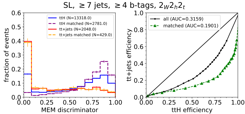
Figure 4.18: The MEM discriminator with the interpretation 2_W2_h2_t , i.e. the fully reconstructed interpretation, in the single-leptonic category with at least seven jets, at least four of which must be b tagged. In order to interpret the light jets as quarks, we sum over all possibilities of choosing two light quarks from the three light jets most compatible with a W-boson decay according to invariant mass. We see that in the presence of an additional jet, the fully-reconstructed MEM interpretation is still able to distinguish between signal and background at an acceptable level.
