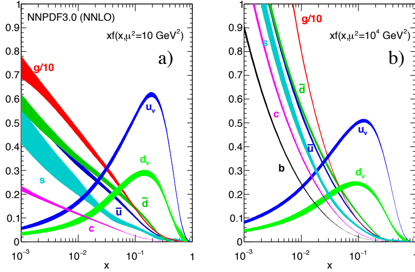
Figure 1.5: The parton distribution functions for protons at \mu_F^2 = 10 \text{ GeV}^2 (left) and \mu_F^2 = 10^4 \text{ GeV}^2 . We see that at higher momenta \mu_F and low x , the proton consists almost entirely out of gluons. Figure from [33].
