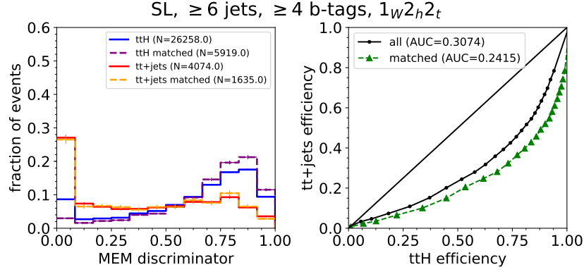
Figure 4.17: The MEM discriminator with the interpretation 1_W2_h2_t in the single-leptonic category with at least six jets, at least four of which must be b tagged. In comparison to fig. 4.15, we have integrated over the momentum of one of the light jets, assuming that only one of the two light jets corresponds to a quark from the W-boson decay. We see a slightly improved performance compared to the fully reconstructed hypothesis in the case of all events (black), and a slight decrease for events that are fully matched. This is consistent with the performance of the MEM being strongly dependent on whether the objects in the final state correspond to the hard scattering process.
