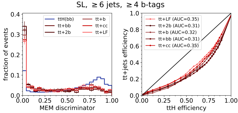
Figure 4.16: The performance of the MEM for different t\bar{t}+jets subprocesses, introduced in section 5.1.1, in the semileptonic \geq 6 -jet, \geq 4 -b tag category. In general, we see that the discrimination is best against t\bar{t}+b\bar{b} and t\bar{t}+2b , followed by t\bar{t}+b . This arises from the use of the t\bar{t}+b\bar{b} diagram as the representative diagram for the computation of the background amplitude.
