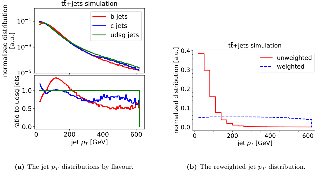
Figure 3.6: Comparison of jet kinematics by associated MC flavour before and after the kinematic reweighting. On (a), we compare the jet p_T distributions for bottom, charm and light jets. We see that b jets have a momentum distribution that is narrower and peaks around 100 GeV. On (b), we show the jet p_T distribution before and after applying the kinematic reweighting w(p_T, |\eta|, \text{flavor}) . We see that the reweighted distribution is roughly uniform, with small differences caused by simulation statistics in the derivation of the weight. These distributions are derived using t\bar{t} +jets simulation.
