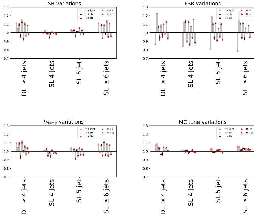
Figure 5.12: The t\bar{t} +jets ISR, FSR, h_{damp} and MC tune uncertainties in terms of a scale factor that depends on jet multiplicity. We extract this scale factor by comparing the yield predicted by the MC simulation with varied parameter values to the nominal, adding the statistical uncertainty on this prediction. Generally, these scale factors are symmetric around the nominal and change the yield by < 15\% , with the most significant effects on the t\bar{t} + LF process.
