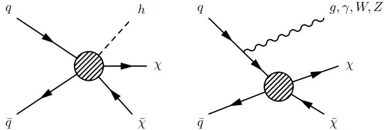
Figure 3.5: Feynman diagrams showing DM production in association with an ISR gluon, photon, Z , W or a Higgs boson.
