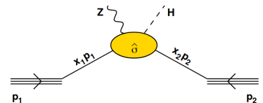
Figure 5.1: Schematic illustration of a hadron-hadron collision modelled using PDFs with pp \rightarrow Z + h [65].
