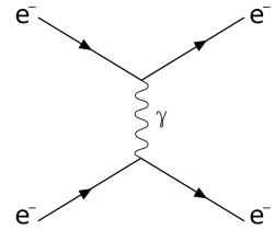
Figure 2.1: Feynman diagram of electron-electron scattering.
