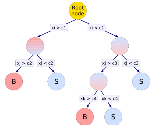
Figure 8.6: Schematic representation of a decision tree with three variables, taken from [76].
