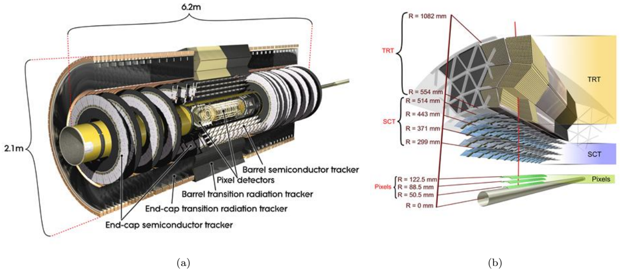
Figure 4.4: An illustration of the ATLAS ID (a), and a cross sectional view of the barrel region(b), showing the Pixel Detector, SCT and TRT. Taken from [31].
