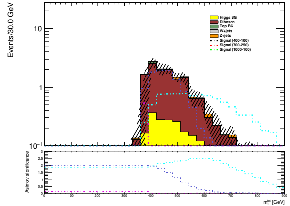
(c) m_T^{tot} SR_High
