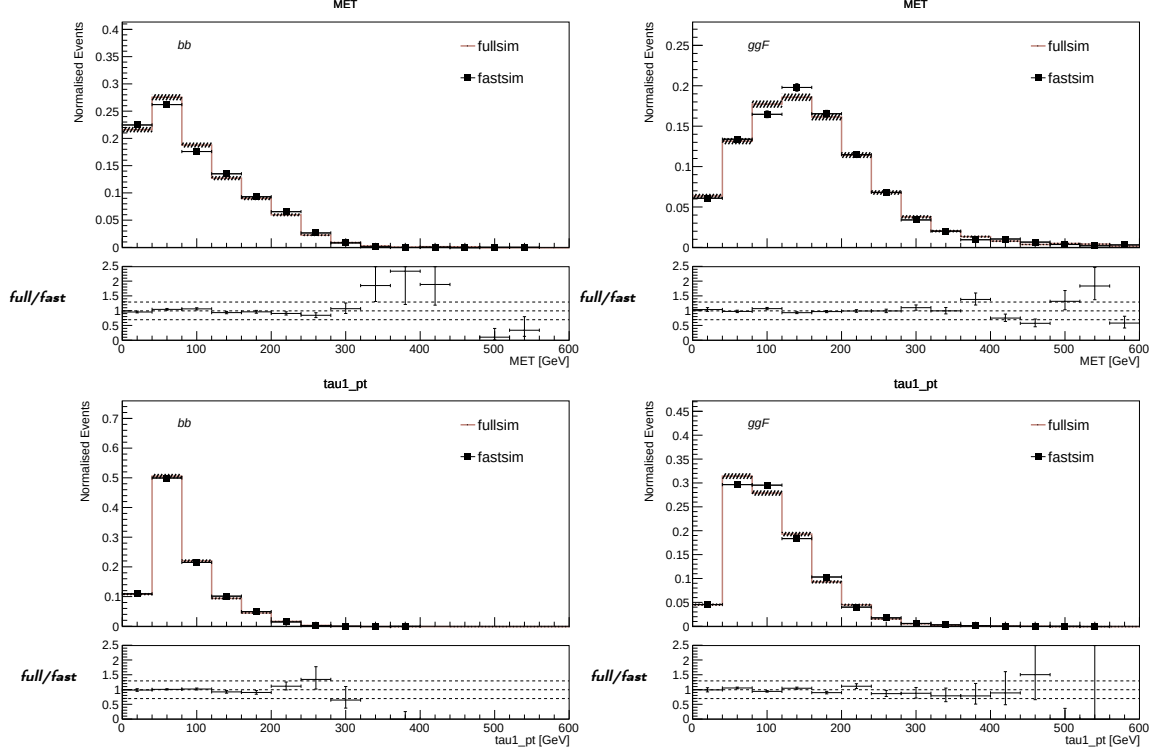
Figure 7.3: Comparison of the ATLFast II and full detector simulation of the 2HDM+a signal. The upper plots show the E_T^{miss} distributions while the lower plots shows the leading \tau p_T distributions. The red lines with shaded uncertainty show the full detector simulation and the black dots the ATLFast II detector simulation.
