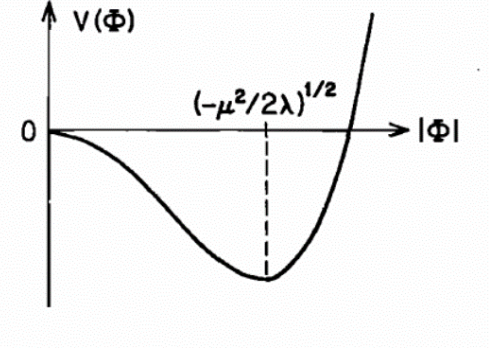
Figure 2.2: Potential of a scalar field with \mu < 0 . Taken from [7].
