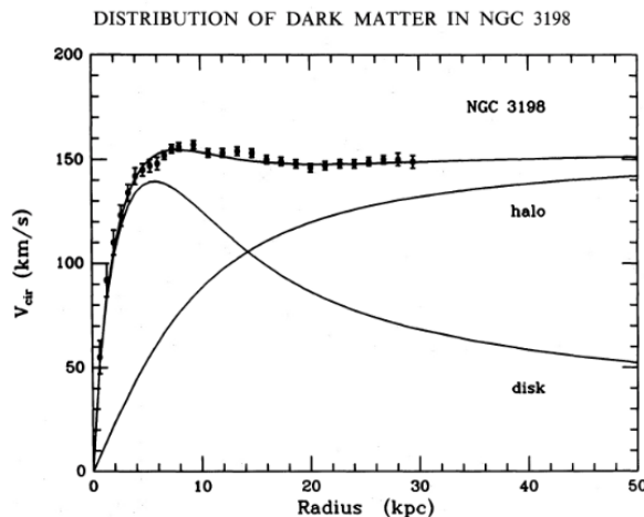
Figure 3.1: Rotation curve of NGC 3198 showing agreement between data and combined fit from velocity distributions of visible matter ("disk") and Dark Matter ("halo") [15] .
