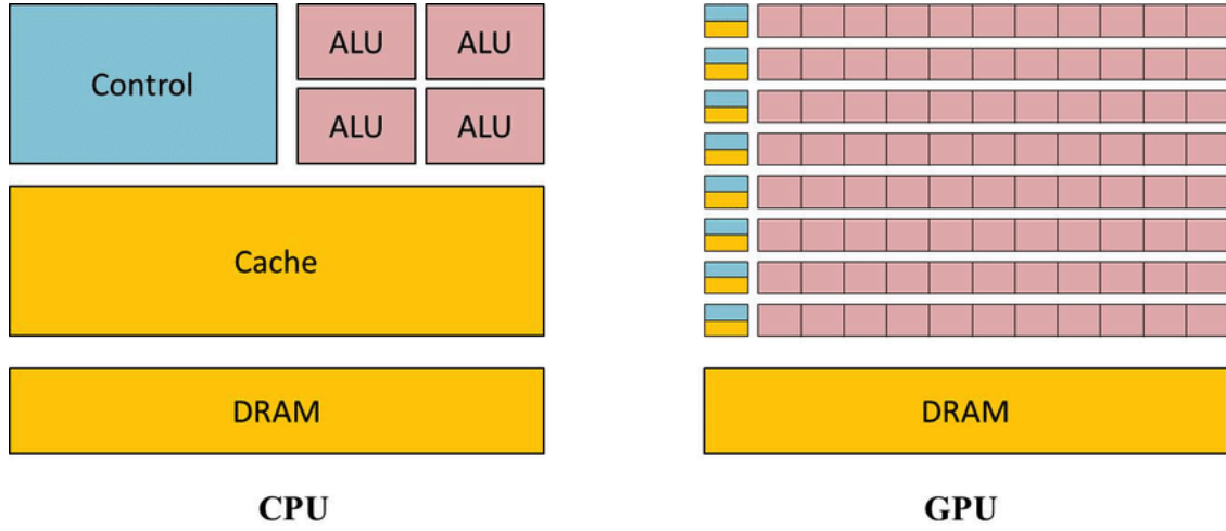
Figure 3.1: Comparison between CPU and modern GPUs structures. The Control Units (CUs) are reported in light blue. The yellow boxes represent the DRAMs and the caches and the ALU/FPU are shown as pink boxes. It is relevant the different proportions of dedicated resources in the two devices.
