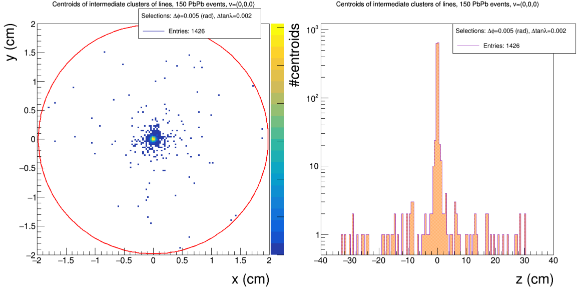
(a) Distribution of transverse position belonging to the centroids of lines clusters. It resembles the distribution of the combinatorial centroids, a part from apart for the narrower core. Red circle is the beampipe cross section border.
