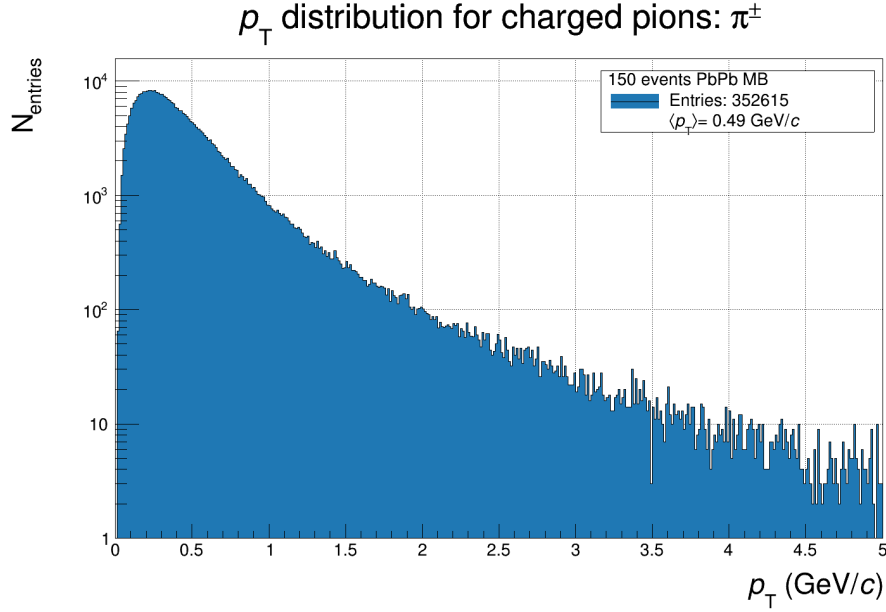
Figure 4.3: The p_T distribution for charged primary pions detected for simulated events. The \langle p_T \rangle = 0.49 GeV/ c is similar to the aforementioned measured value on real data by ALICE detector.
