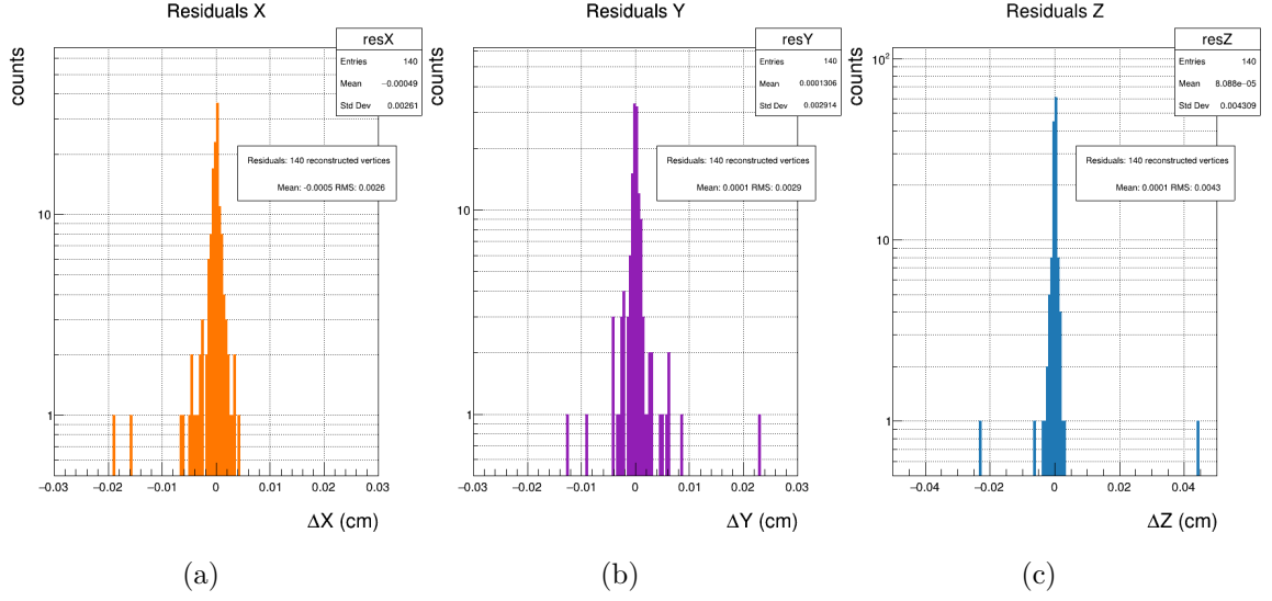
Figure 5.16: Residuals distributions of reconstructed vertices.
