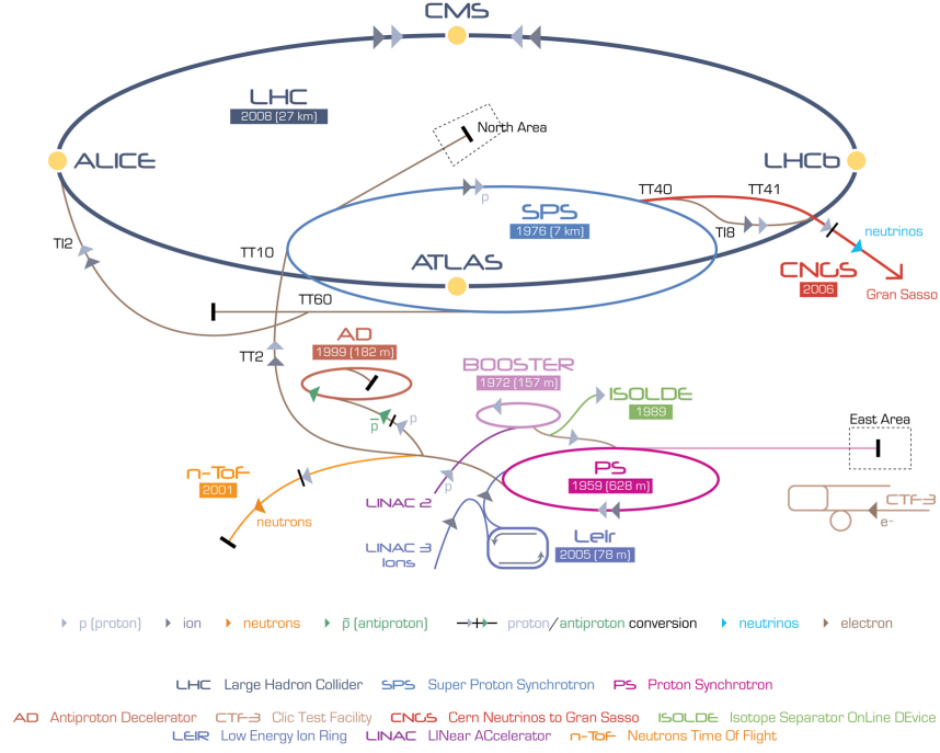
Figure 1.3: LHC experiments
