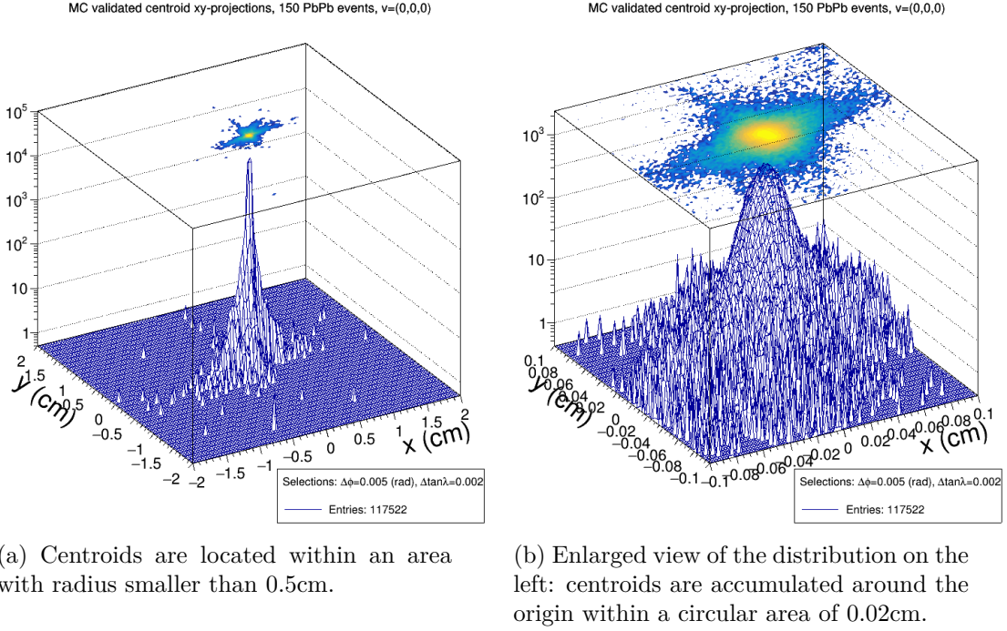
Figure 5.10: On the left: Distribution of the transverse position of the centroids for every combination of Monte Carlo validated lines. Figure on the right is an enlargement of the plot on the left to better visualise the accumulation of centroids around the origin. Events are generated with vertex fixed in the origin of the transverse plane. The amplitude of the distribution is proportional to the amplitude of the distribution of DCAs, since centroids are medium point of DCA vectors.
