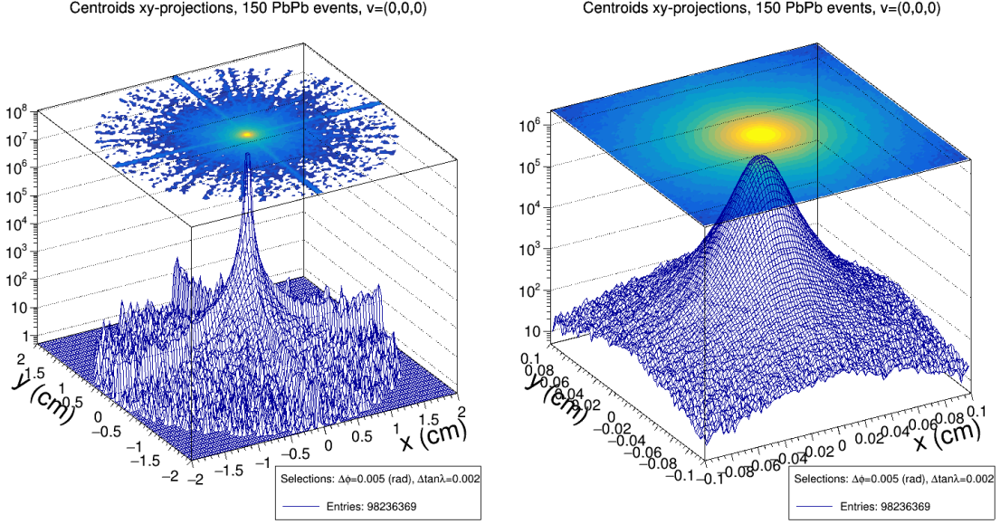
(a) Centroids transverse positions are more spread across the beampipe cross-section compared to the ones from Monte Carlo validated lines. It is interesting to observe the regular patterns shaped as multiple overlapped crosses in the tails of the distribution, caused by matches of tracklets reconstructed multiple times in the angular intervals corresponding to overlaps of staves in single layers.
