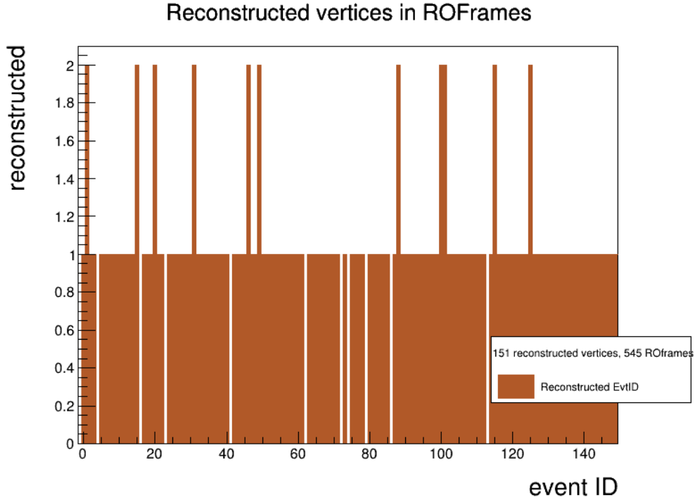
Figure 5.15: The histogram reports the IDs of reconstructed vertices spread across 545 readout frames. Indices are assigned using the Boyer-Moore voting routine. When more than one entry is present for the same ID, it means that the event is shared across at least two frames. White gaps represent missing IDs, hence vertices not reconstructed. No fake vertices (ID= -1) have been reconstructed in this dataset.
