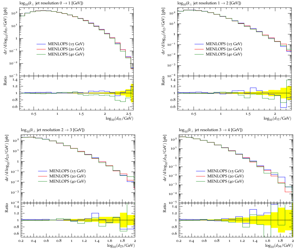
Figure 3.20: Differential jet rates d_{n+1} for three different merging cuts, Q_{\text{cut}} , in Drell-Yan lepton-pair production at the Tevatron at \sqrt{s} = 1.96 TeV.
