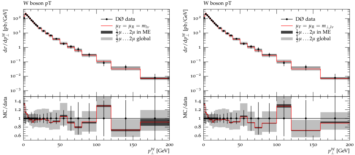
Figure 3.19: Transverse momentum of the W boson in W +jets production at the Tevatron compared to data from the DØ experiment [111]. Scale variations of the POWHEG prediction by factors of 1/2 and 2 are displayed for two different scale schemes, \mu_F = \mu_R = m_{l\nu} (left) and \mu_F = \mu_R = m_{\perp,l\nu} (right). The inner (dark) band displays the variations associated with redefining the scales for matrix elements alone, while the outer (light) band also takes variations in the running coupling of the parton shower evolution into account.
