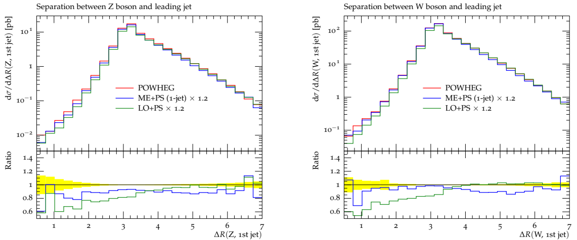
Figure 3.6: Separation between vector boson and leading jet in Z/\gamma^* (left) and W (right) boson production at the Tevatron.
