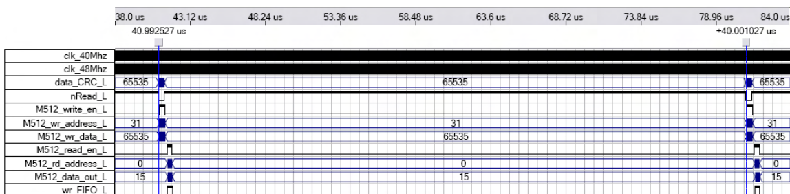
Figure 3.5.: Postsynthesis simulation of dual clock memory: Every 40\mu s data are available. This data are converted to the 48 MHz clock system and stored in the FIFO before new data arrives.
