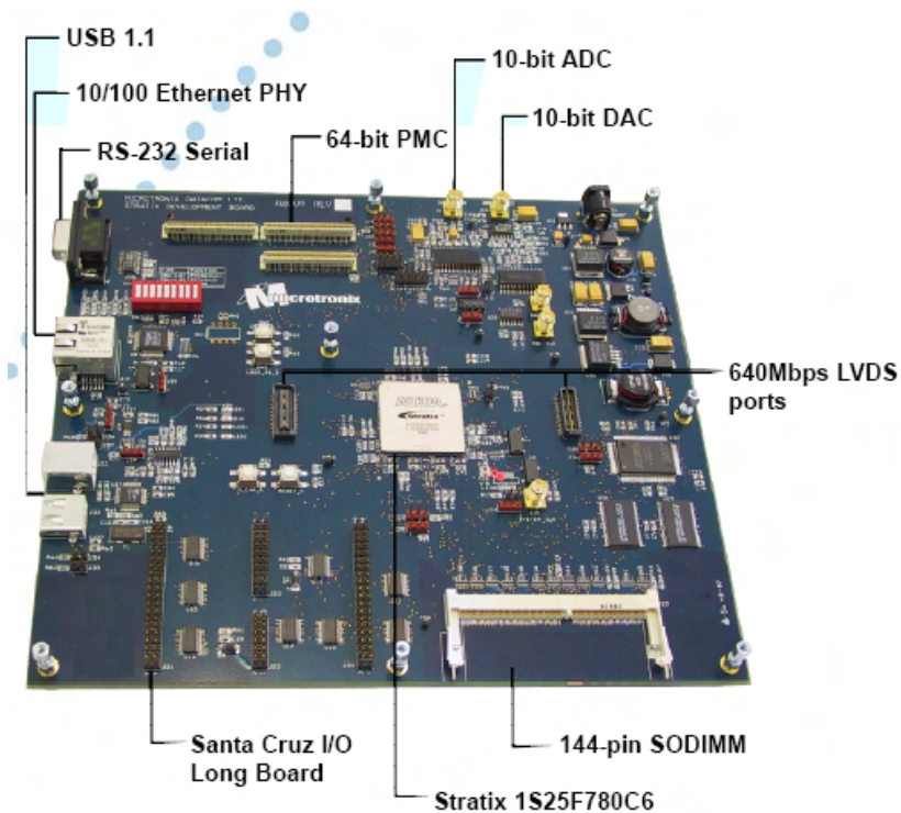
Figure 3.1.: FPGA Development board. [7]
