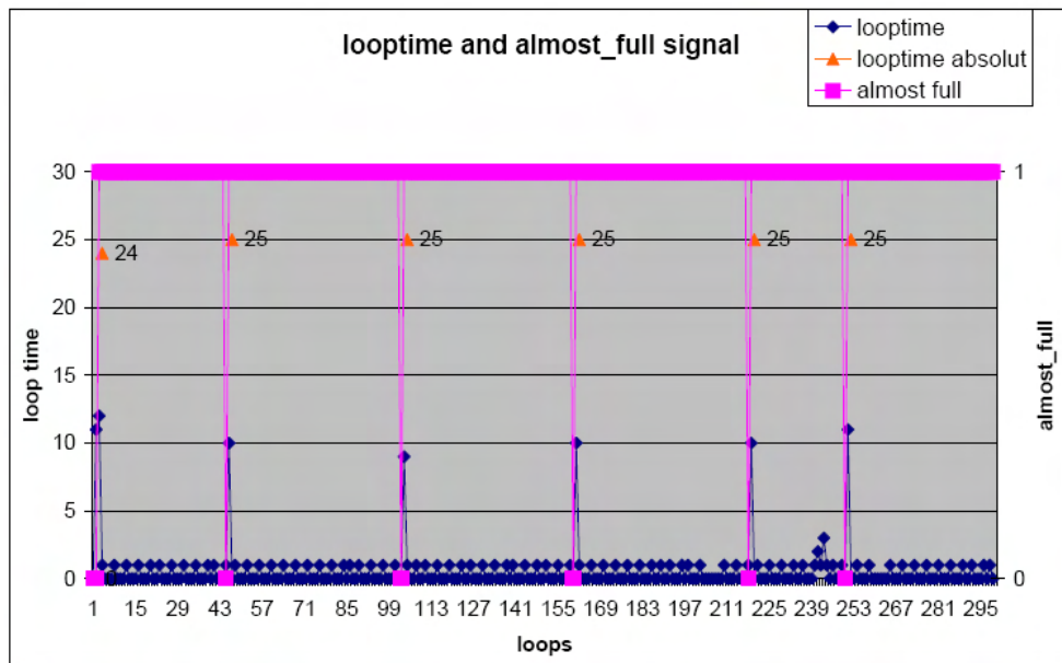
Figure 6.7.: Read out cycle loop time as function of the loop index. In this test the displays were deactivated to increase read out speed. The timing of the program can be estimated using the time of the loops.
