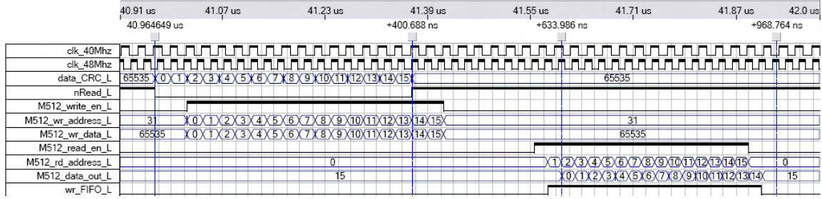
Figure 3.6.: Postsynthesis simulation of dual clock memory 2: After writing data to the memory, it is read using the other clock in the system, and passed to the FIFO.
