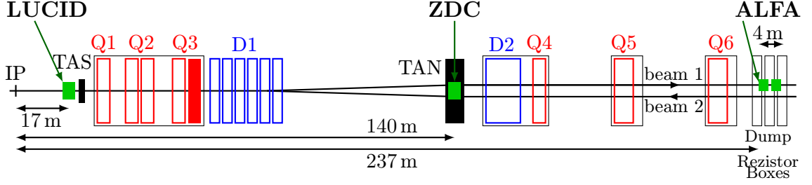
Figure 5.9: The placement of the ATLAS forward detectors with respect to IP1 [51].
