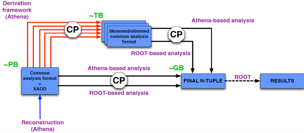
Figure 6.1: The ATLAS Run 2 analysis model consists of a new EDM (xAOD) and a centralized data-reduction framework (Derivation Framework)[60].
