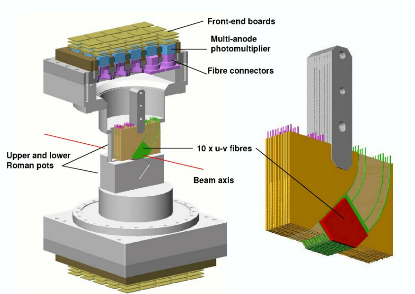
Figure 5.10: Schematics of ALFA detector and special retractable devices called Roman pots [56].
