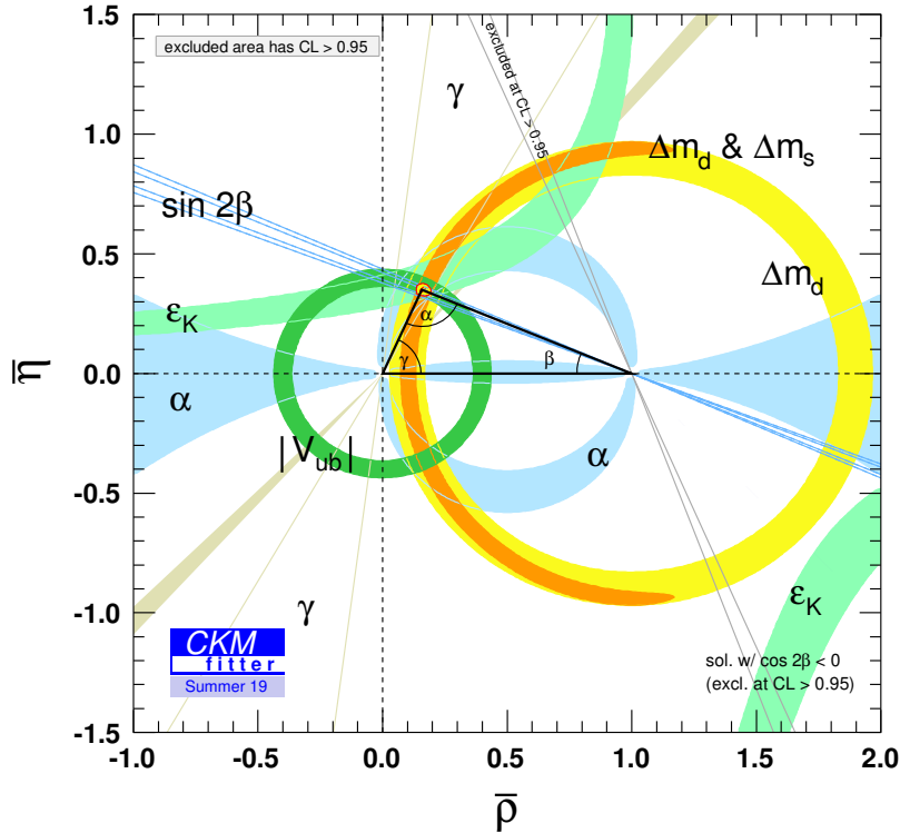
Figure 2.4: Constraints of CP -violation parameters on the \bar{\rho} , \bar{\eta} plane [22].
