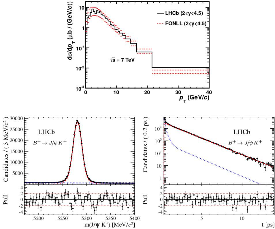
Figure 7.5: Differential production cross-section as a function of the B^+ transverse momentum measured by LHCb experiment at \sqrt{s} = 7 \text{ TeV} compared with FNLLO calculation (Top). Distributions of the mass (bottom-left) and decay time (bottom-right) of B^+ \rightarrow J/\psi K^+ candidates and their associated residual uncertainties [74, 75].
