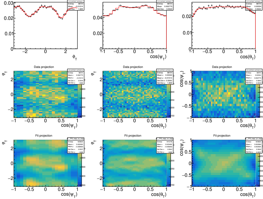
Figure 8.10: 1D projections (top) and 2D projections (middle and bottom) of the fitted transversity angular distributions for \Lambda_b \rightarrow J/\psi p K^- .
