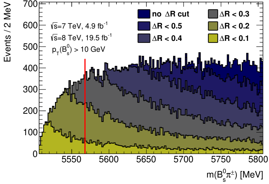
Figure 10.3: The study of the background shape behavior under the cut on \Delta R parameter. The red line represents the central invariant mass value of the resonance X(5568) reported by the D\emptyset collaboration.
