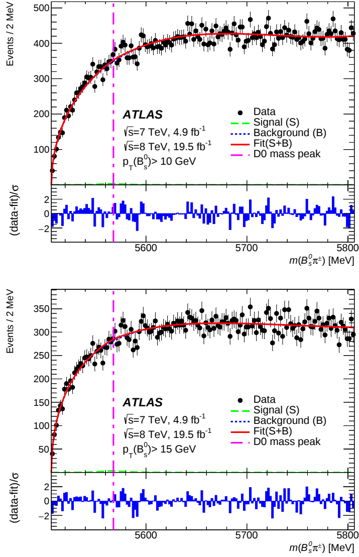
Figure 10.4: Results of the fit to the B_s^0\pi^\pm mass distribution for candidates with p_T(B_s^0) > 10 \text{ GeV} (top) p_T(B_s^0) > 15 \text{ GeV} and (bottom). The bottom panels show the difference between each data point and the fit divided by the statistical uncertainty of that point [110].
