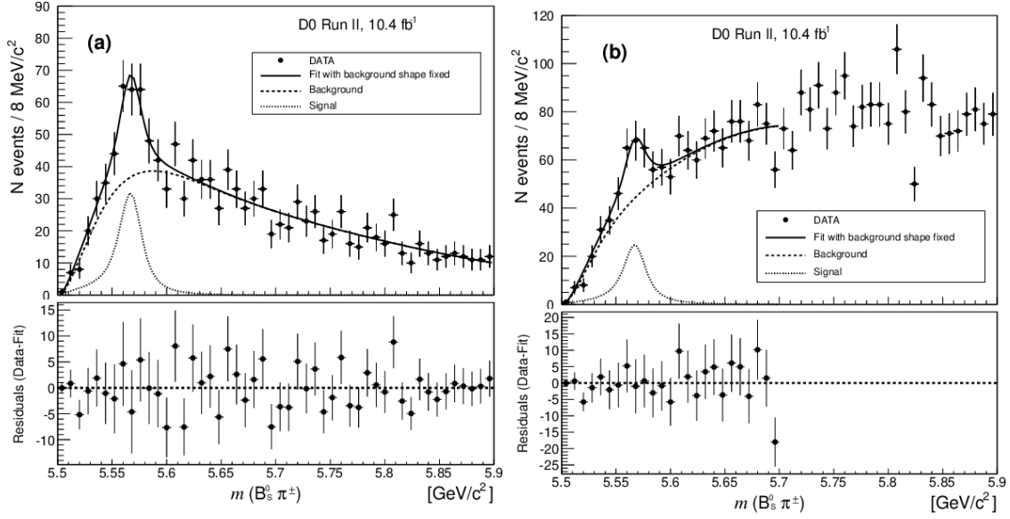
Figure 10.1: The m(B_s^0\pi^\pm) distribution together with the background distribution and the fit results (a) after applying the \Delta R < 0.3 cone cut and (b) without the cone cut obtained by DØ experiment [105].
