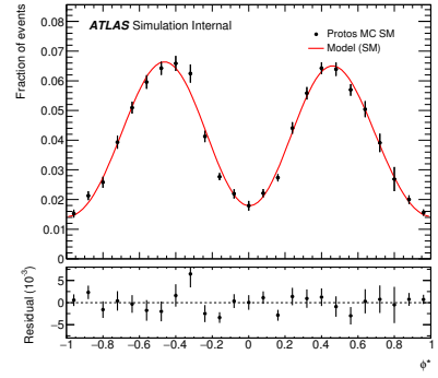
(f) \phi^*
