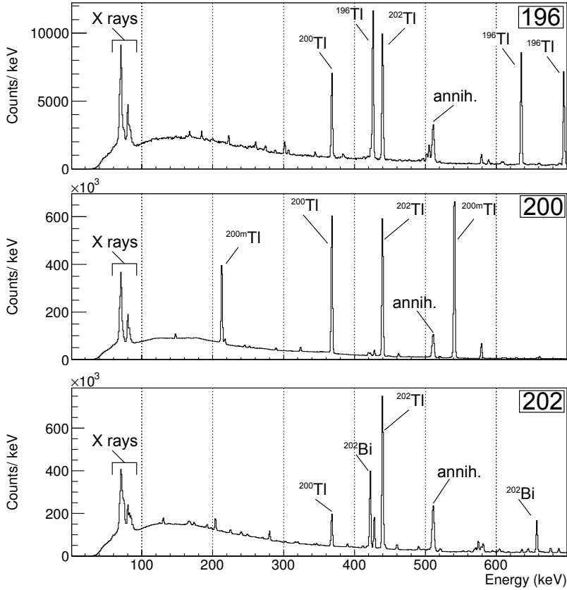
Figure 4.1: Gamma spectra recorded by detector Ge 1 during the IS466-III run when measuring at masses 196, 200 and 202. The most prominent lines were identified as originating from Tl contaminants. The presence of non-isobaric Tl in the spectra is due to earlier measurements on other masses. In the case of ^{200}\text{Tl} , also a short-living (34 ms) isomeric state was implanted in the carbon foil. Therefore, \gamma rays emitted in the internal decay of this state are also observed in the spectra at mass 200. Also \gamma photons followed by the \beta^+/\text{EC} decay of ^{202}\text{Bi} were detected. As indicated in Table 4.1, no \gamma spectra at mass 194 were recorded.
