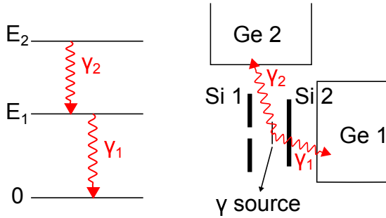
Figure 3.9: (In color) Schematic illustration of the coincidence method to determine the efficiencies of the HPGe detectors Ge 1 and Ge 2 in the WM setup (see Figure 3.7). A cascade of two \gamma rays, denoted by \gamma_1 and \gamma_2 are emitted from a \gamma source placed at the foil position.
