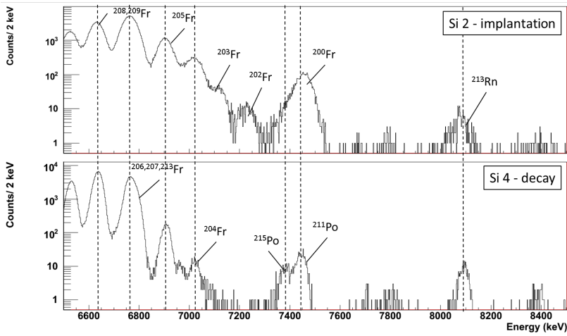
Figure 4.7: A comparison of measured \alpha spectra of Si 2 and Si 4 at mass 200 during the IS534 run. Observed \alpha lines in the decay detector reveal the presence of ^{211,215}\text{Po} \alpha -decay lines at energies close to 7.4 MeV, which is close to the energy of the main ^{200}\text{Fr} \alpha peak.
