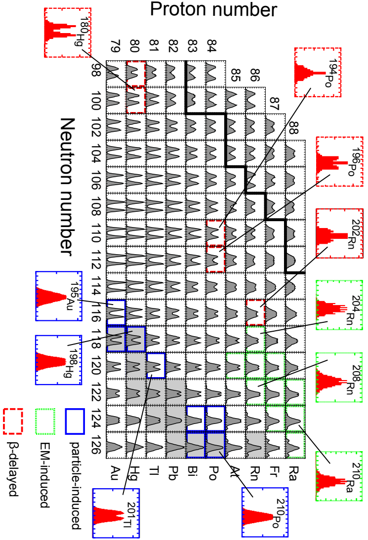
Figure 5.1: (In color) Calculated MDs (gray), with fission-fragment masses on the horizontal and their relative yields on the vertical axis, for even- N neutron-deficient isotopes between gold and radium at excitation energies slightly above the theoretical fission-barrier heights B_{f,th} [71]. The calculated yields are compared with selected experimental MDs (red) from particle-induced [36, 37], \beta -delayed ([3, 4], this work) and EM-induced fission [5, 6]. The border of the lightest known isotopes is shown by the thick solid line, \beta -stable nuclei are shown on a gray background.
