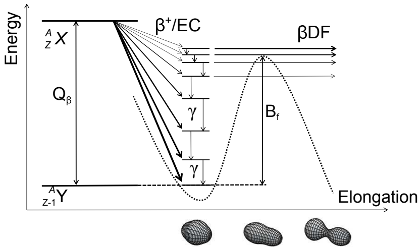
Figure 2.4: Schematic representation of \beta DF on the neutron-deficient side of the nuclear chart. The curved dotted line indicates the potential energy of the daughter nucleus with respect to nuclear elongation, displaying also the fission barrier.
