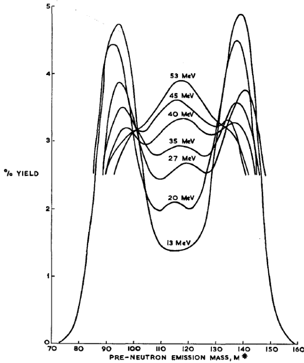
Figure 2.2: Pre-neutron emission FF mass distributions, recorded after the bombardment of a ^{232}\text{Th} target with protons. The beam energies are given as labels to the curves. Figure taken from [35].
