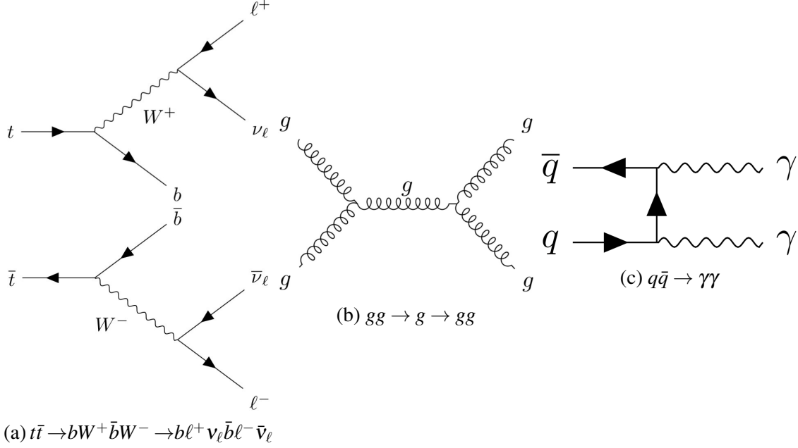
Figure 4: Examples of Feynman diagrams for t\bar{t} , gluon–gluon scattering and non-resonant diphoton production, which may appear as backgrounds to W , Z and Higgs analyses.
