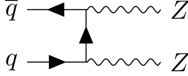
Figure 3: Example Feynman diagram for ZZ diboson production.
