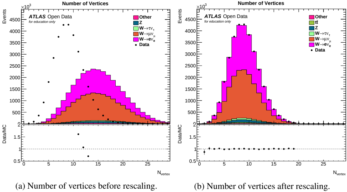
Figure 8: Stacked histograms showing the difference in the number of vertices between data and Monte Carlo, before and after rescaling, for a 13 TeV ATLAS Open Data W analysis. Rescaling makes Data/MC closer to 1. “Other” includes backgrounds for low-mass Drell-Yan, single top and dibosons in both (a) and (b), as well as t\bar{t} in (a). W \rightarrow \tau\nu_\tau and Z are also backgrounds.
