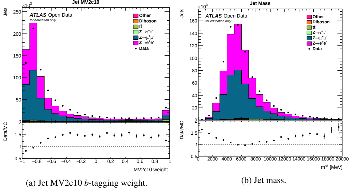
Figure 12: Stacked histograms of further jet variables for a 13 TeV ATLAS Open Data Z analysis. The signal Monte Carlo samples are Z \rightarrow e^+ e^- and Z \rightarrow \mu^+ \mu^- . “Other” includes backgrounds for W , low-mass Drell-Yan and single top. Z \rightarrow \tau\tau , t\bar{t} and diboson are also backgrounds.
