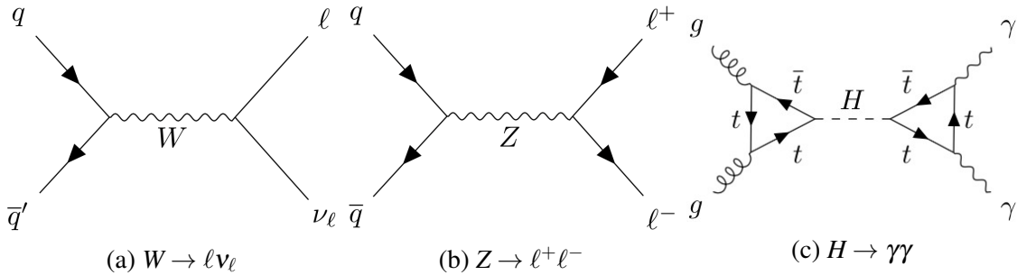
Figure 2: Examples of Feynman diagrams for the processes W \rightarrow \ell \nu_\ell , Z \rightarrow \ell^+ \ell^- and H \rightarrow \gamma\gamma . \bar{q}' denotes an antiquark of different flavour to quark q . g denotes a gluon. Other symbols are defined in Section 2.1. No arrows are drawn when a particle could be a fermion or an antifermion.
