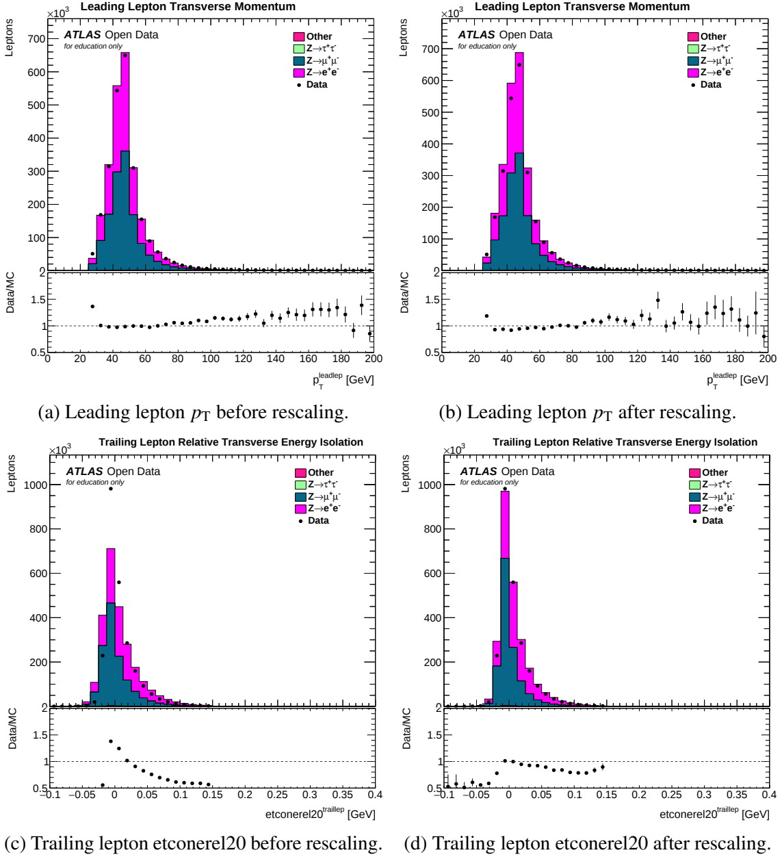
Figure 9: Stacked histograms showing the difference in selected lepton variables between data and Monte Carlo, before and after rescaling the number of vertices, for an ATLAS Open Data Z analysis. etconerel20 is defined as the etcone selection requirement in Table 3. “Other” includes backgrounds for dibosons, low-mass Drell-Yan, W , single top and t\bar{t} . Z \rightarrow \tau\tau is also background.
