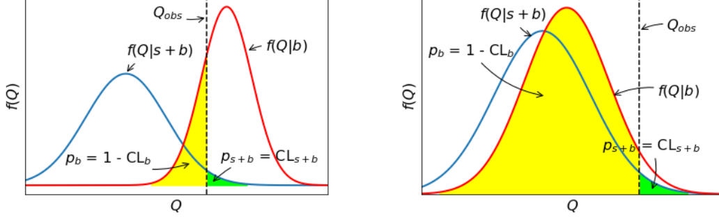
Figure B.6: Left: The \text{CL}_S technique applied to H_0 and H_1 distributed in the test statistic Q , where a reasonable sensitivity under Q gives well separated distributions. Right: The \text{CL}_S technique for low sensitivity under Q , leading to a large overlap and hence a small p_0 in the B -only hypothesis.
