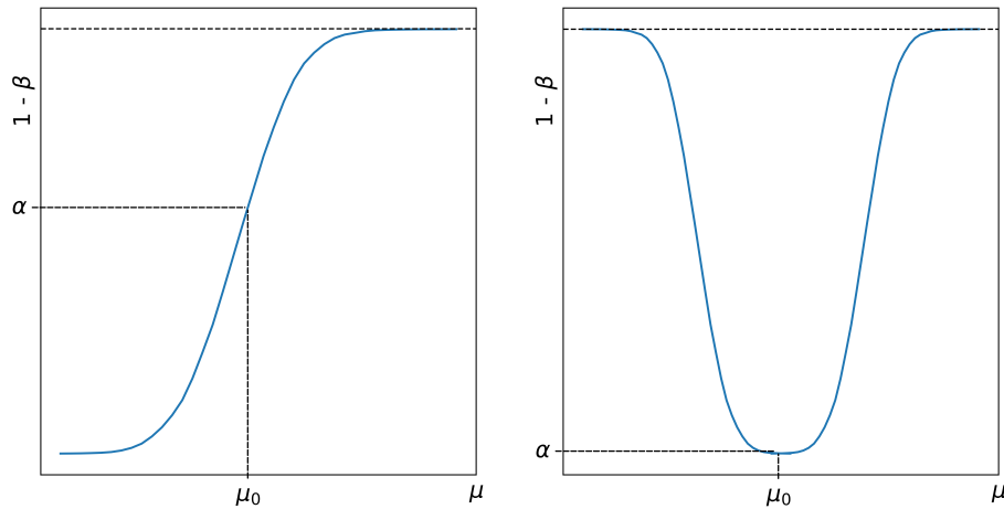
Figure B.2: Visual representations of the possible hypothesis tests, demonstrating the one-tailed (left) and two-tailed tests (right) distributed in \mu . The two-tailed test improves on the statistical test of an alternative hypothesis for \mu < \mu_0 , but loses power versus the one-tailed test in the region for which \mu > \mu_0 . This is a case where no single test can achieve maximal power.
