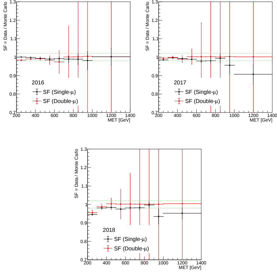
Figure 5.4: Trigger efficiency correction factors, or scale factors ( SF = \text{Data}/\text{Monte Carlo} ) for 2016 (top left), 2017 (top right), and 2018 (bottom). A green band demarcates the 2% uncertainty attributed to the trigger efficiency as measured in the ratio across all p_T^{\text{miss}} intervals.
