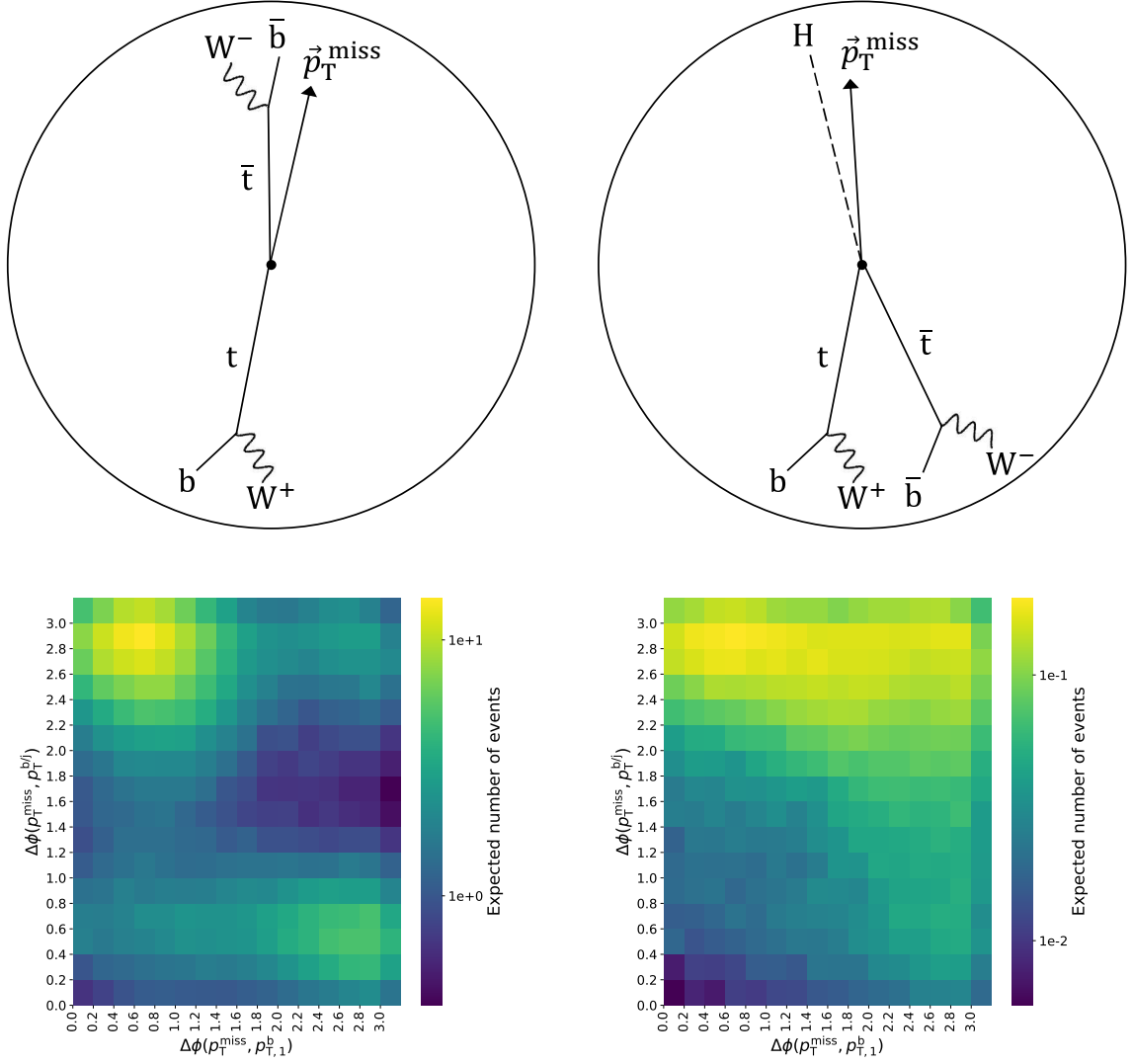
Figure 5.5: Upper: The topology of the t\bar{t} and t\bar{t}H system in the transverse plane of the detector, where the \vec{p}_T^{\text{recoil}} , denoted by a solid arrow, is typically aligned with the leading or subleading b-jet direction in t\bar{t} events, and aligned with the invisibly decaying Higgs boson in t\bar{t}H events. Lower: The distribution of t\bar{t} and t\bar{t}H processes in |\Delta\phi(\vec{p}_T^{\text{recoil}}, \vec{p}_{T,1}^b)| and either |\Delta\phi(\vec{p}_T^{\text{recoil}}, \vec{p}_{T,1}^j)| (for the 5/6j1b subcategories) or |\Delta\phi(\vec{p}_T^{\text{recoil}}, \vec{p}_{T,2}^b)| (for the 5/6j2b subcategories), demonstrating the alignment or anti-alignment of \vec{p}_T^{\text{recoil}} commonly with the lead b jet for t\bar{t} processes, and the lack of correlation with the presence of the invisibly decaying Higgs boson in t\bar{t}H processes.
