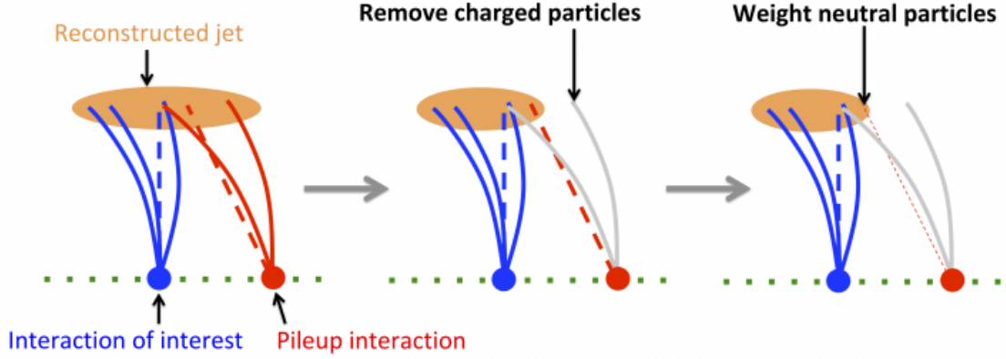
Figure 3.3: The PUPPI technique of identifying vertices based on the charged particle distribution, rejecting those coming from pileup vertices. The neutral particles are weighted based on the distribution of charged particles in its vicinity.
