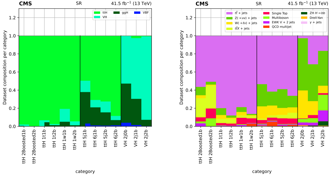
Figure 5.10: The fractional SR composition of signal (left) and background (right) processes for each subcategory using simulated 2017 CMS samples.
