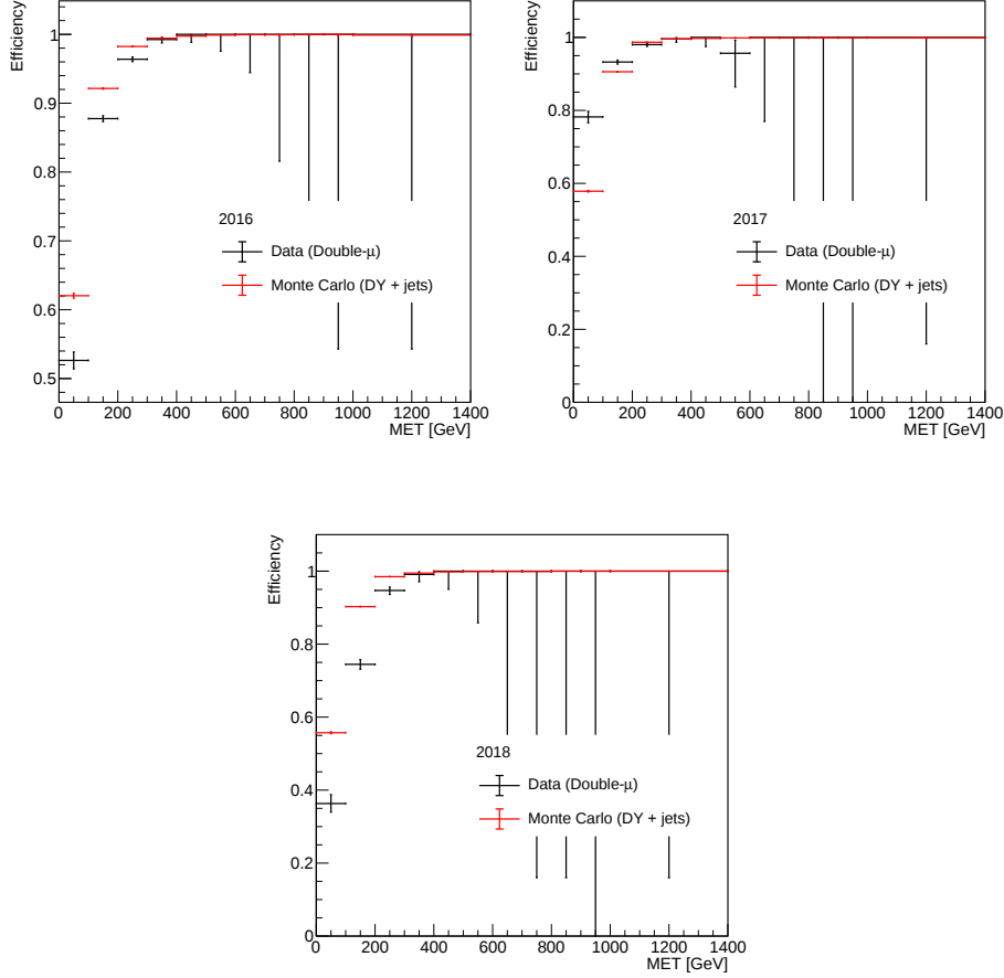
Figure 5.3: Combined PF p_T^{\text{miss}} and PF H_T^{\text{miss}} trigger efficiency in dimuon data and DY + jets MC samples for 2016 (top left), 2017 (top right), and 2018 (bottom).
