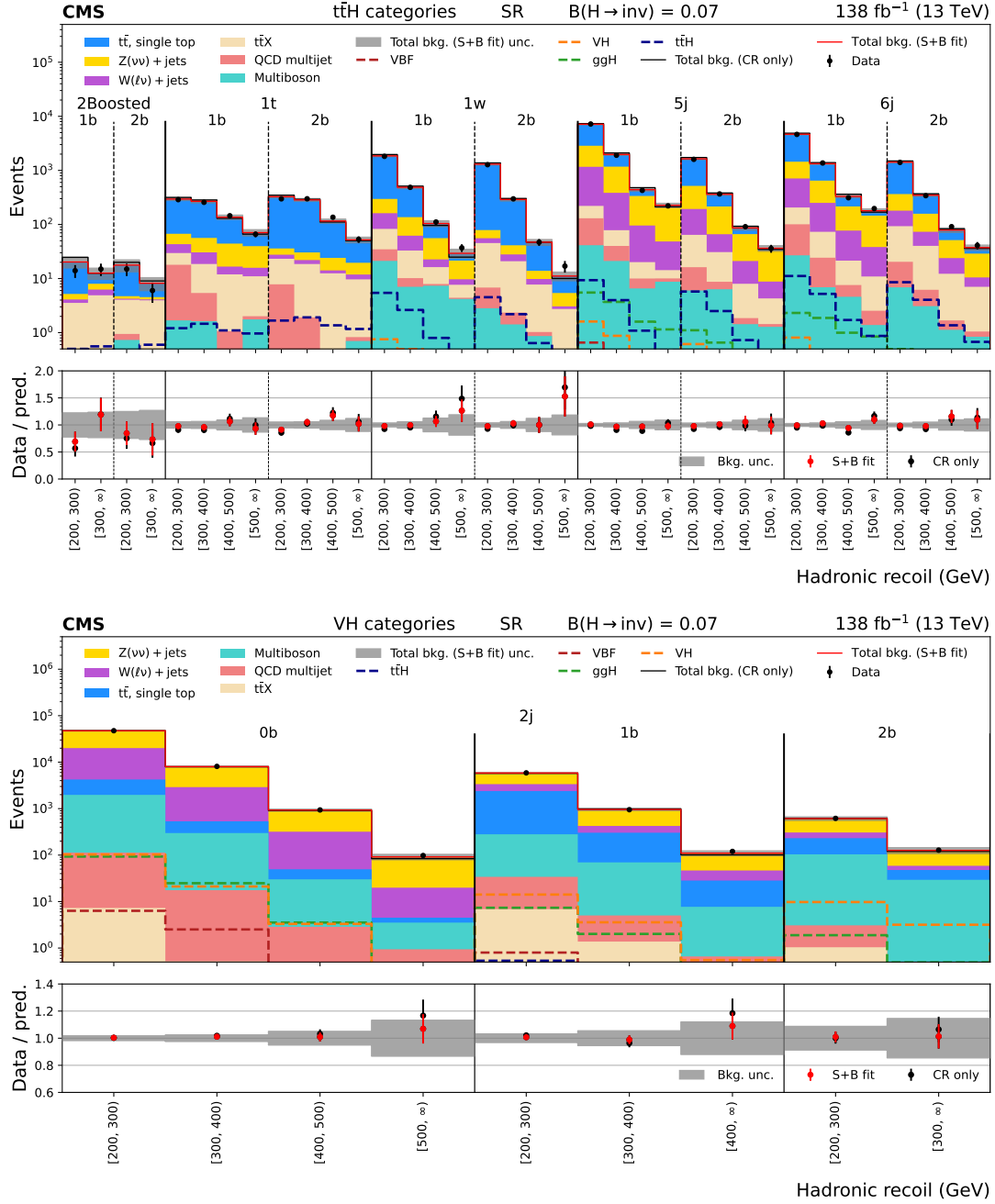
Figure 7.4: Distributions of hadronic recoil in the t\bar{t}H (upper) and VH (lower) categories for the SR, showing the signal contributions from t\bar{t}H , VH , ggH , and VBF weighted by B(H \rightarrow \text{inv}) = 0.07 . The black histogram shows the total background (bkg.) prediction from a CR only, B -only fit, while the red histogram shows the yields from a CR+SR S+B fit.
