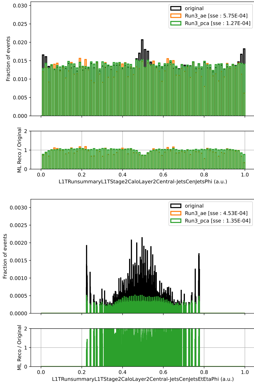
Figure 3.16: Reconstructions of CenJets \phi and \eta - \phi - p_T distributions from the AE (orange) and PCA (green), taken from bad run 356709 in which a significant amount of L1 pre-firing has occurred, and overlaid on the original histogram for that run. The SSE is an effective \chi^2 measurement between the original and reconstructed histograms.
