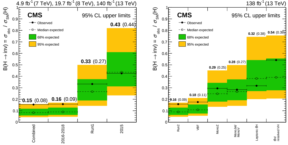
Figure 8.2: Left: Observed and expected limits at 95% CL for the combination, broken down by data-taking period. Right: Observed and expected limits at 95% CL for the combination, broken down by analysis.
