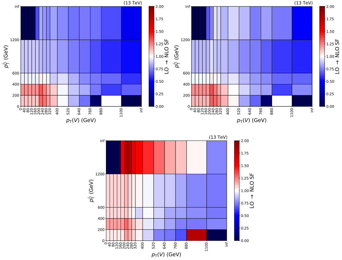
Figure 6.1: The QCD-derived K-factors applied to LO QCD simulations of DY + jets (top left), Z( \nu\bar{\nu} ) + jets (top right), and W( \ell\nu ) + jets (bottom) derived differentially as functions of p_T^V and p_{T,1}^j from NLO QCD DY + jets (top) and W + jets (bottom) samples.
