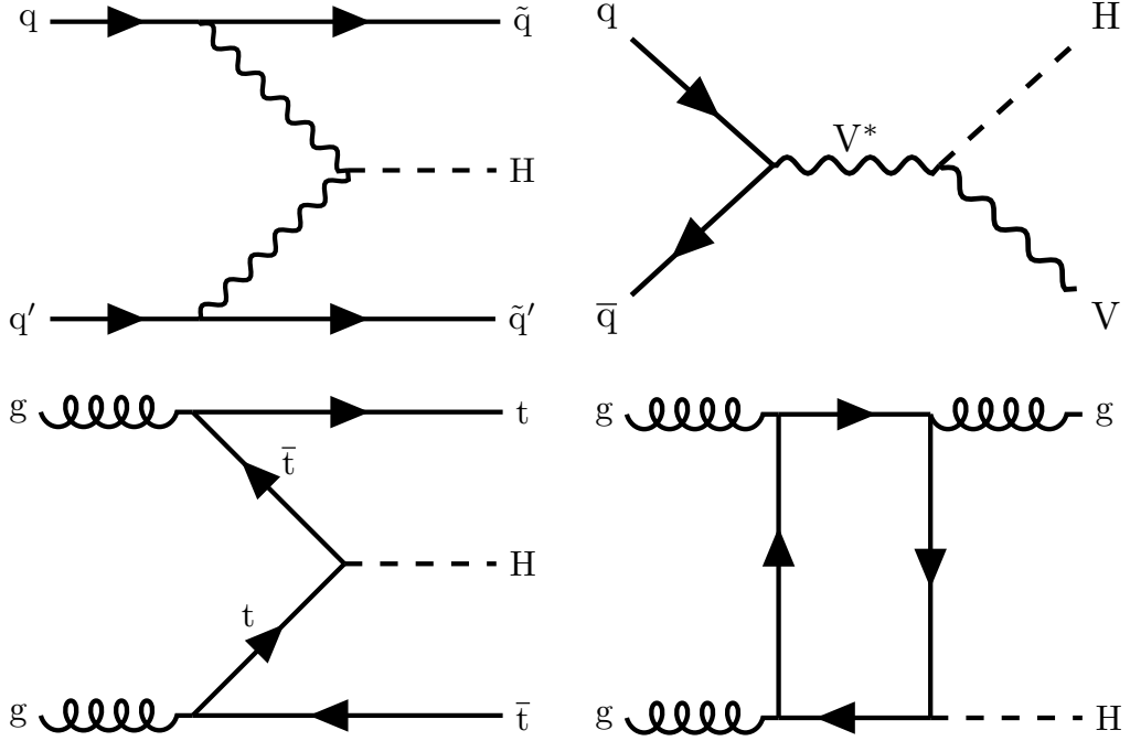
Figure 1.1: Representative tree level diagrams of the four Higgs production channels, (clockwise) VBF, VH, ggH, and t\bar{t}H , in which H \rightarrow \text{inv} searches are performed by the CMS Collaboration.
