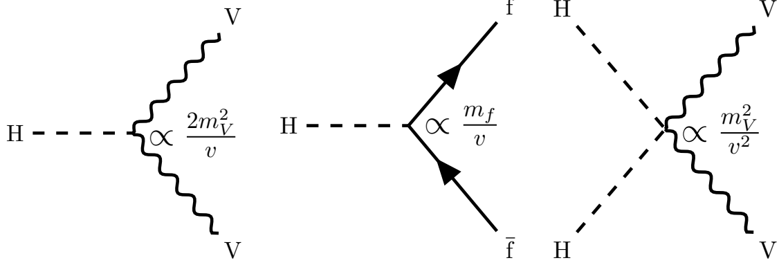
Figure 2.4: The set of Higgs boson interactions with SM fermions and bosons, with their accompanying coupling strengths in proportions of m_V or m_f , and the VEV, v . The quartic coupling term has not been observed experimentally.
