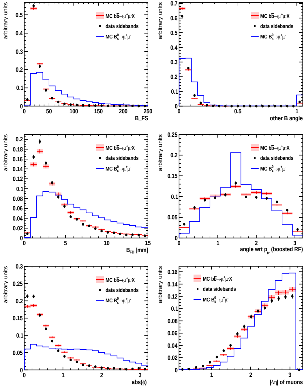
Figure 5.20: Variables included in the optimization of the BDT classifier. All the samples have a \text{BDTS} > 0.05 requirement.
