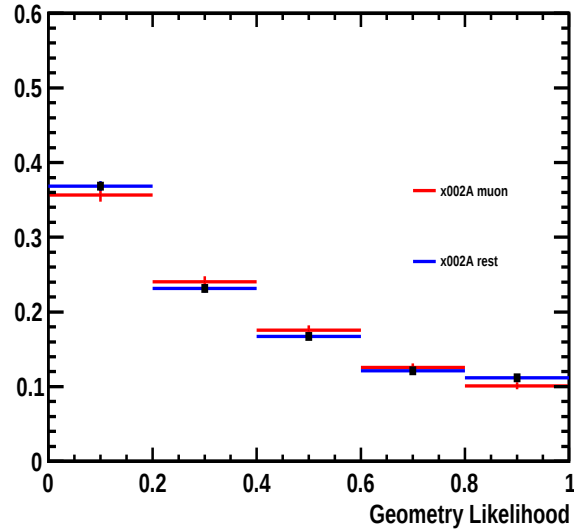
Figure 4.9: Signal GL distributions obtained from D^0 \rightarrow K\pi events triggered with the configuration TCK=x002A that are triggered unbiased for muonic lines (red) and for the rest of lines (blue with black squares).
