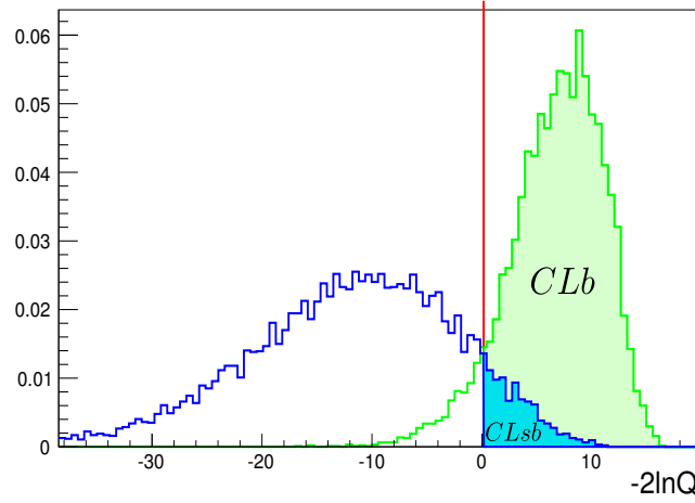
Figure 7.5: Distribution of the test statistics for a set of generated pseudo-experiments with a background only hypothesis (green) and signal plus background hypothesis (blue) for an assumed \mathcal{B}(B_s^0 \rightarrow \mu^+ \mu^-) . The vertical line corresponds to the value of the test statistic for a certain data sample; the green area is the CL_b and the blue area CL_{s+b} [52].
