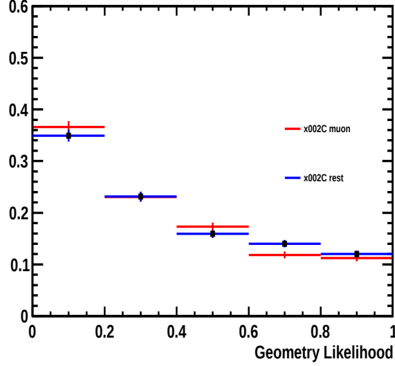
Figure 4.10: Signal GL distributions obtained from D^0 \rightarrow K\pi events triggered with the configuration TCK=x002C that are triggered unbiased for muonic lines (red) and for the rest of lines (blue with black squares).
