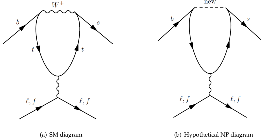
Figure 1.3: Penguin diagrams contributing to b \rightarrow s \ell \bar{\ell} involving observed particles (a) and hypothetical particles (b).
