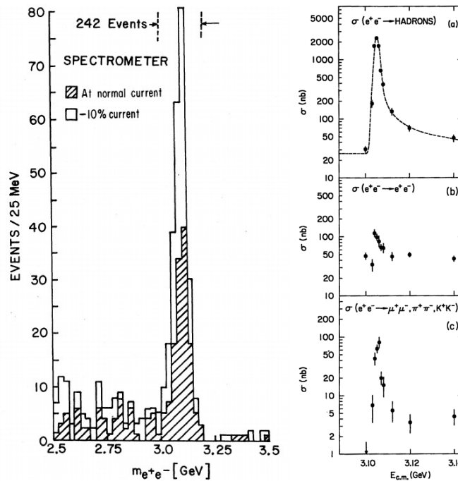
Figure 1.7.: Discovery of the J/\psi . Left: Invariant mass distribution of dielectrons pairs, measured in p-Be collisions. Figure taken from [57]. Right: Cross section of electron-positron annihilation as a function of center-of-mass energy in hadronic channel (top), dielectron channel (middle), and dimuon, dipion, dikaon channel (bottom). Figure taken from [58].
