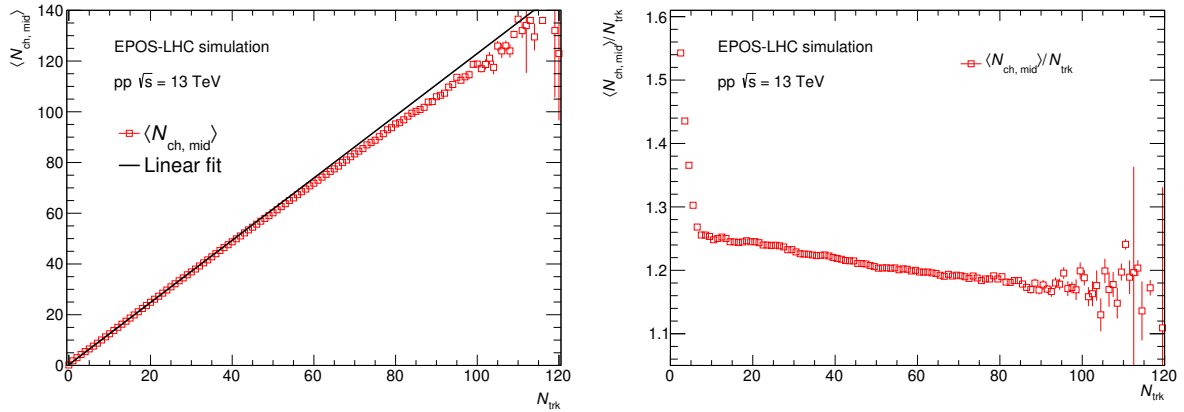
Figure 4.6.: Correlation between charged-particle multiplicity at mid-rapidity N_{\text{ch,mid}} and number of SPD tracklets in |\eta| < 1 from Monte Carlo simulation. Left: Mean N_{\text{ch,mid}} in events selected according to N_{\text{trk}} as a function of N_{\text{trk}} . Right: Mean ratio of N_{\text{ch,mid}} and number N_{\text{trk}} ( \alpha factor) as a function of N_{\text{trk}} .
