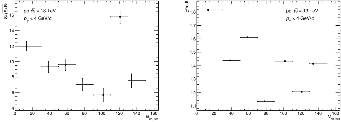
Figure A.9.: Performance of the signal extraction at low p_T as a function of N_{ch, fwd} . Left: Significance of the extracted signal; Right: \chi^2/ndf between the extracted signal and the scaled line shape from Monte Carlo simulations.
