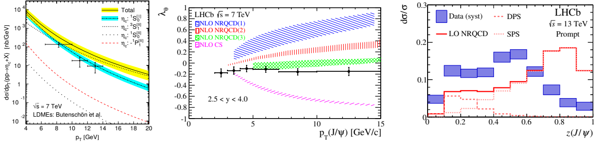
Figure 1.14.: Disagreement between predictions from NRQCD and experimental results of charmonium production in pp collisions from the LHCb experiment. Left: \eta_c cross section as a function of p_T at \sqrt{s} = 7 TeV, compared to NLO NRQCD. Also shown is the color-singlet contribution to the cross section. Middle: J/\psi polarization at \sqrt{s} = 7 TeV, compared to NLO NRQCD. Also shown is the prediction from the CSM model. Right: J/\psi production inside jets at \sqrt{s} = 13 TeV, compared to LO NRQCD. Figures taken from [97], [98], [99].
