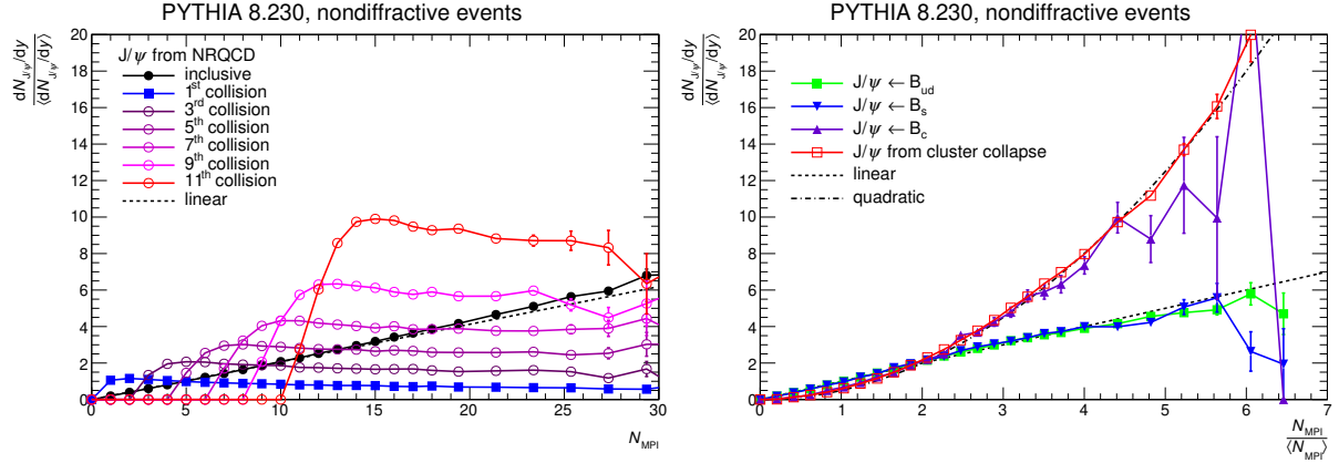
Figure 7.12.: Explanation for the linear and quadratic scaling of J/\psi production as a function of N_{MPI} . Left: Prompt J/\psi produced from NRQCD split according to in which PI it was produced. Right: J/\psi from coalescence and B decay, split into B , B_s and B_c .
