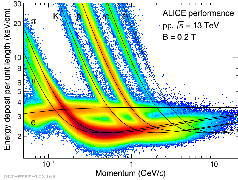
Figure 3.4.: Specific energy loss ( dE/dx ) in the TPC versus particle momentum in pp collisions at \sqrt{s} = 13 \text{ TeV} . The lines show the parametrizations of the expected mean energy loss for different particle species. Figure taken from [171].
