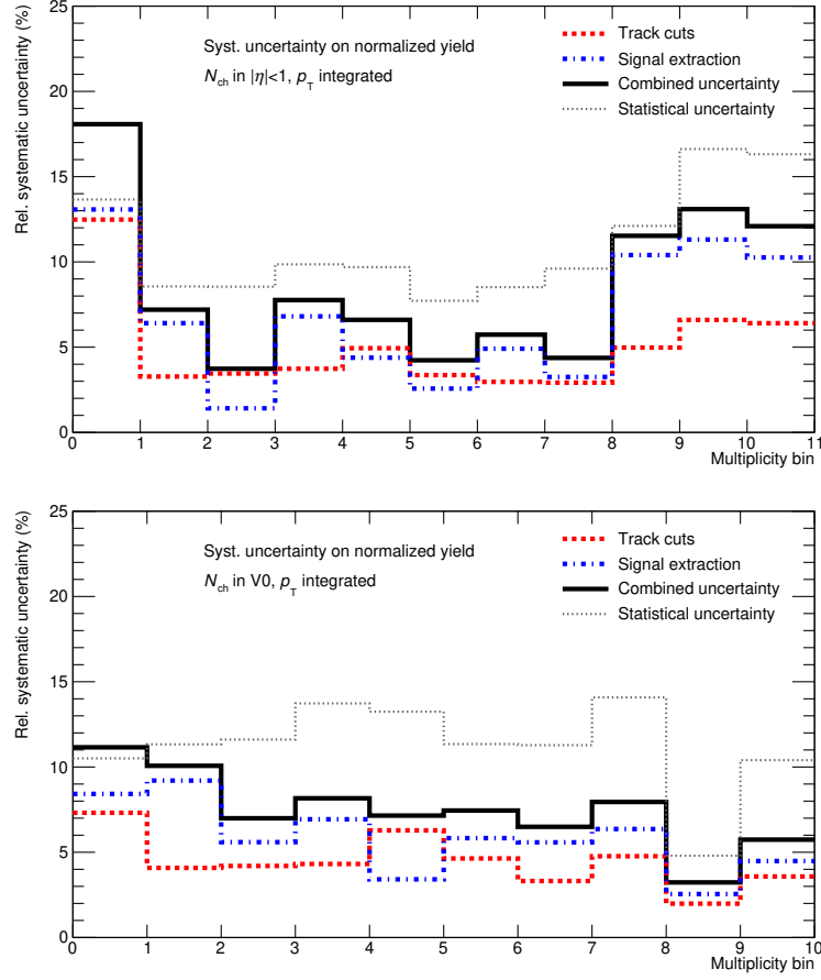
Figure 5.6.: Relative systematic uncertainty on the self-normalized J/\psi yield as a function of the multiplicity interval at mid-rapidity (top) and at forward rapidity (bottom). Uncertainty due to the track selection, the signal extraction, and the total systematic uncertainty as combination of the two. Statistical uncertainty shown for comparison.
