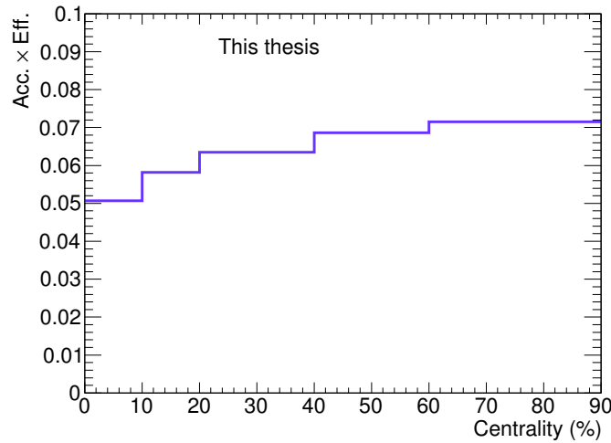
Figure 4.21: J/\psi Acc. \times Eff. integrated over p_T for the different centrality classes.
