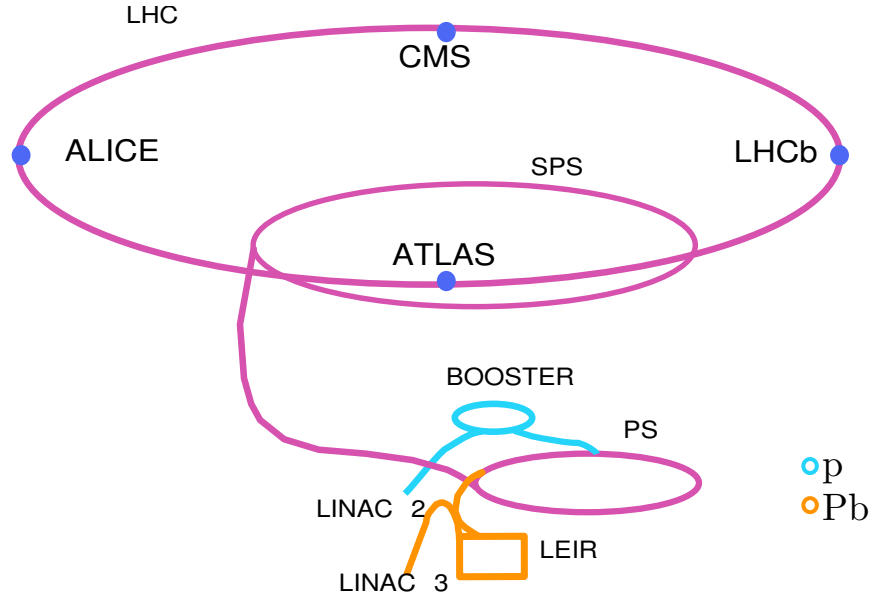
Figure 3.1: CERN accelerator chain. The different injection and acceleration chain for protons are ions are indicated with different colors. The steps after the injection in SPS is analogous for both. Details on the acceleration process are explained in the text.
