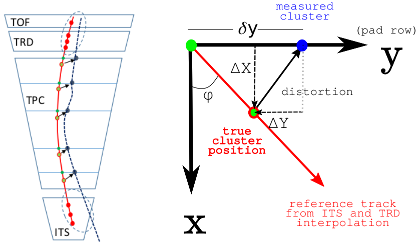
Figure 3.9: TPC sector coordinate frame, y-axis parallel to the pad rows and z-axis along the beamline. ITS, TRD and TOF clusters (red) with the corresponding expected track on the TPC. TPC measured clusters (blue). Figure adapted from [100].
