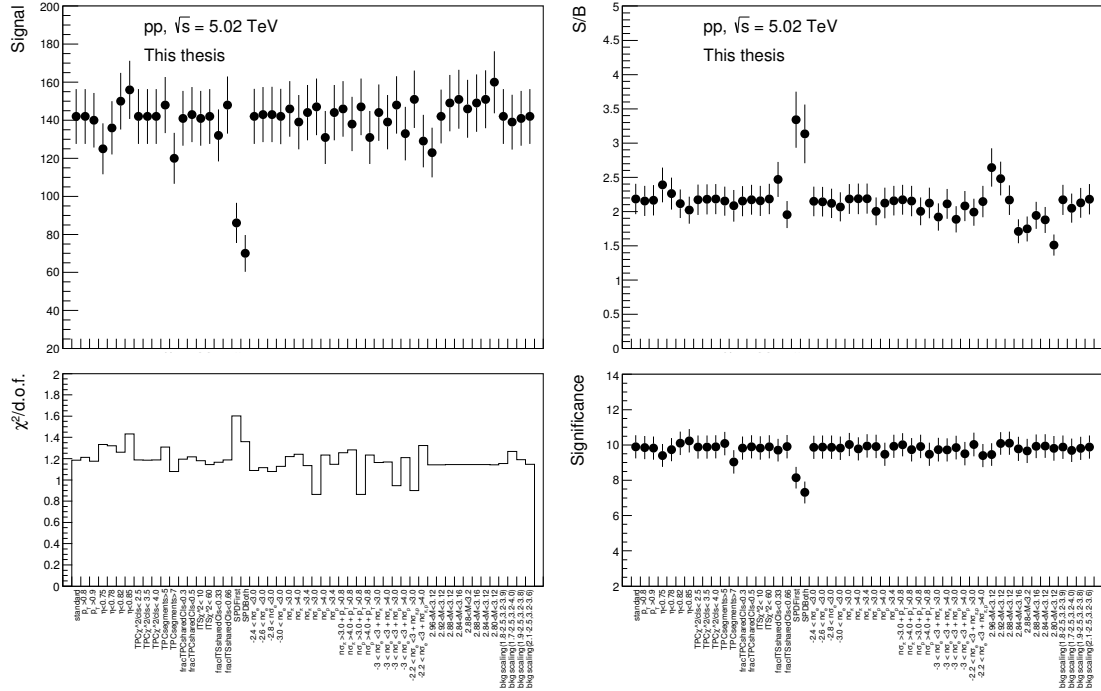
Figure A.5: Summary of the signal extraction parameters. Signal, S/B, significance and \chi^2/d.o.f. for the different track, PID and signal extraction variations.
