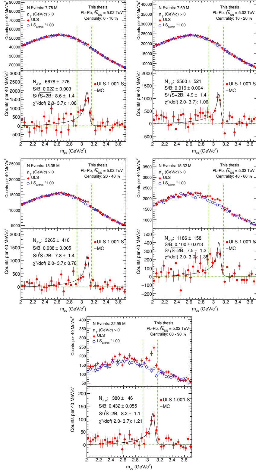
Figure 4.8: Signal extraction performed with the like-sign (LS arithm ) arithmetic method for five different centrality classes. Top left: 0-10 %, top right: 10-20 %, middle left: 20-40 %, middle right: 40-60 %, bottom: 60-90 %.
