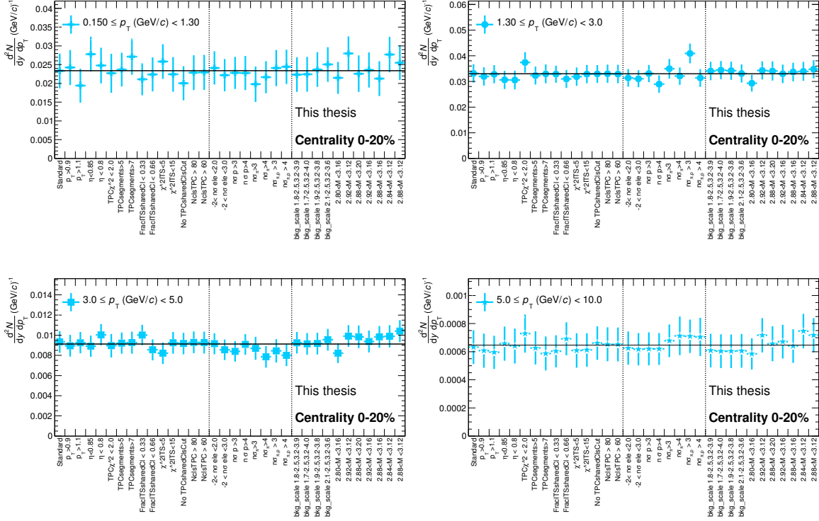
Figure 5.6: Corrected p_T -differential inclusive J/\psi yield obtained for each of the selection criteria variations in the centrality class 0–20%. Each panel corresponds to a different p_T bin. Discussion is given in the text.
