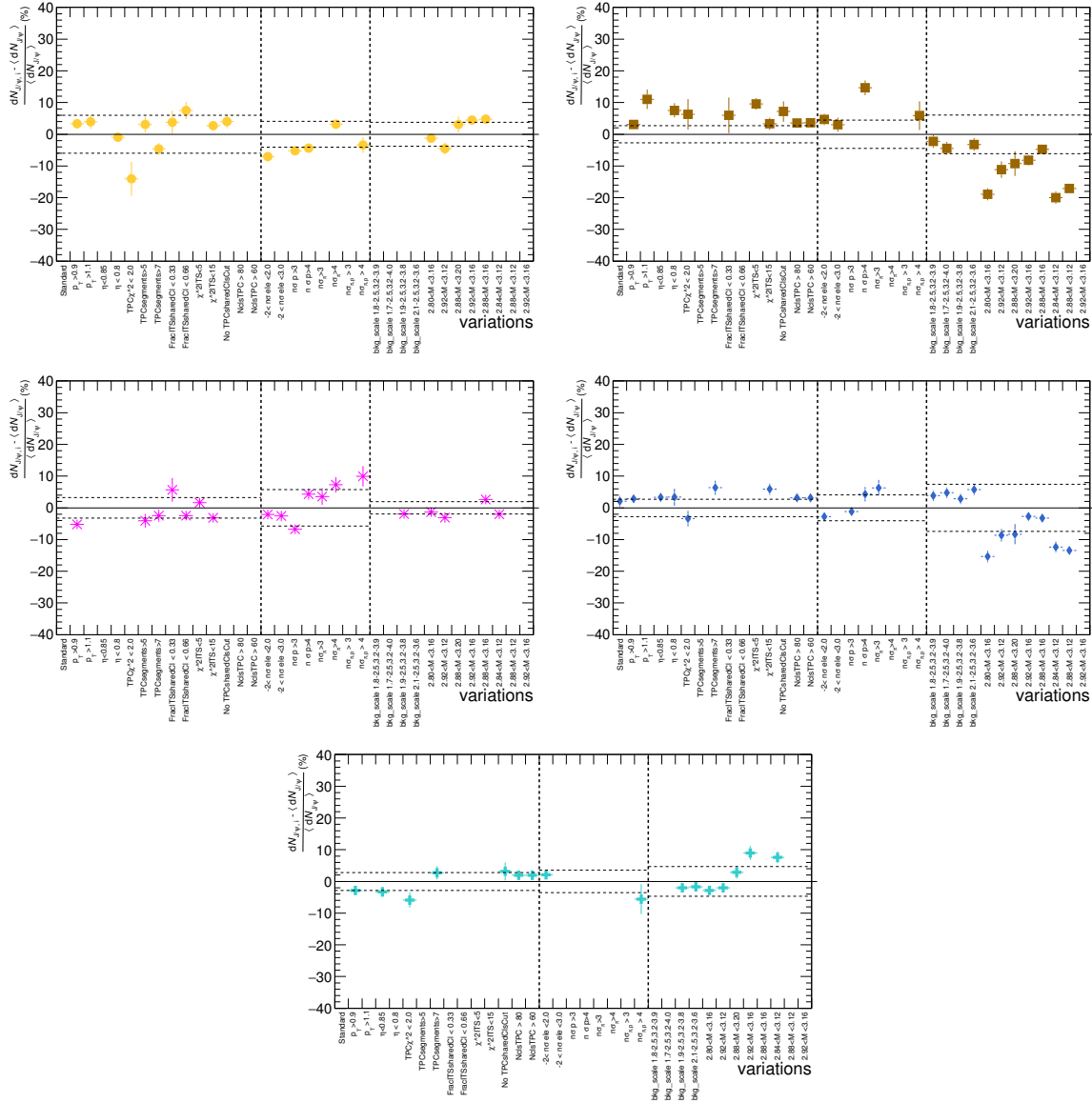
Figure 5.10: Difference with respect to the mean for each of the variations. Only the variation after applying Barlow's are shown. The corresponding RMS of each of contribution: tracking, PID and signal extraction is indicated with a band in the corresponding variations region.
