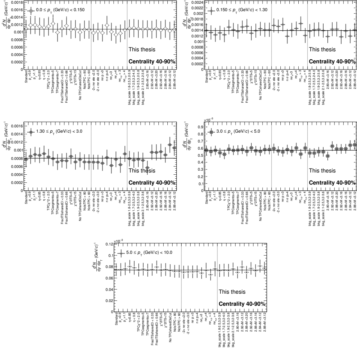
Figure 5.8: Corrected p_T -differential inclusive J/\psi yield obtained for each of the selection criteria variations in the centrality class 40 – 90%. Each panel corresponds to a different p_T bin. Discussion is given in the text.
