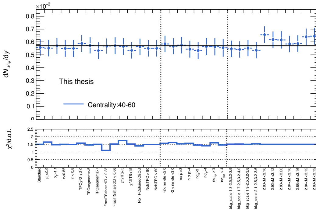
Figure 5.4: Corrected J/\psi yield calculated for each selection criteria variation in the centrality class 40 - 60\% . The horizontal black line corresponds to the mean value of all the variations. The vertical lines divide the different selection criteria in tracking, PID and signal extraction.
