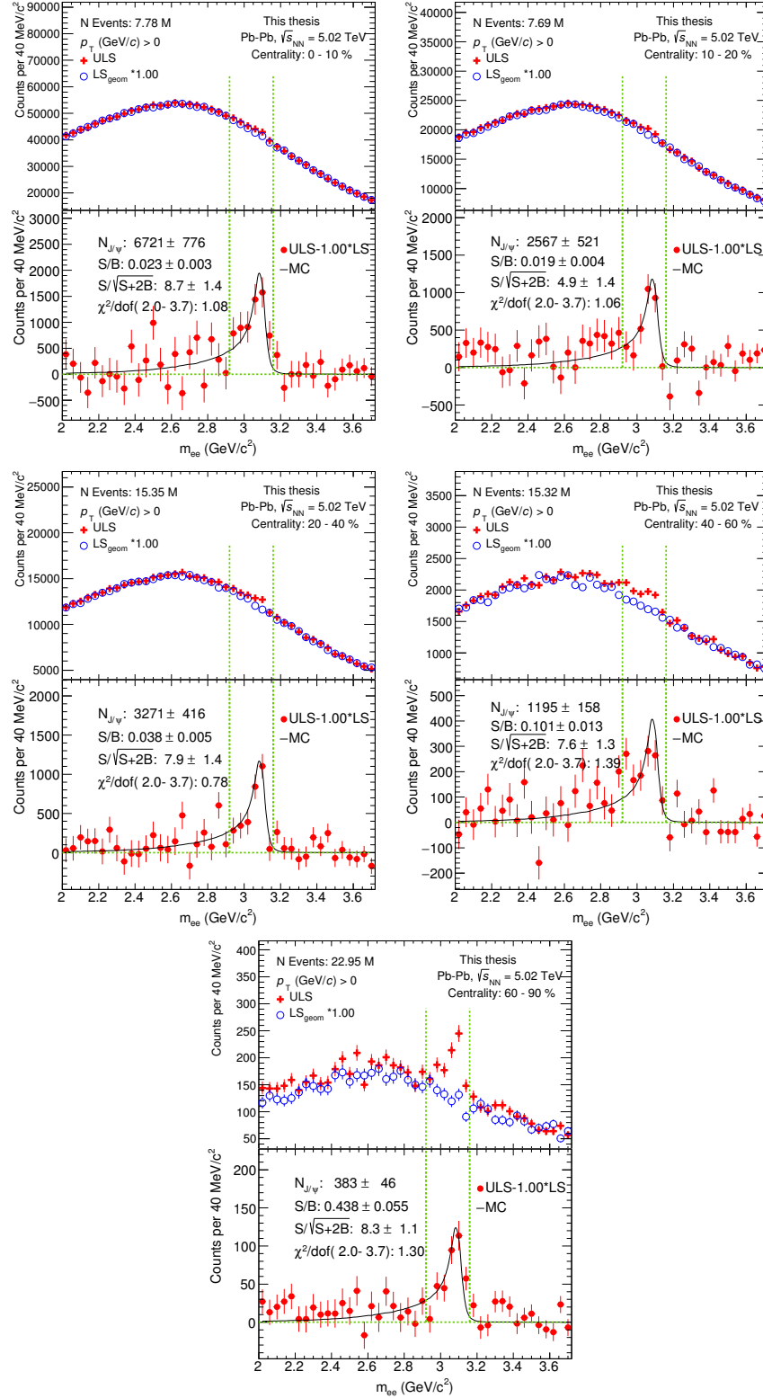
Figure 4.7: Signal extraction performed with the like-sign (LS geom ) geometric method for five different centrality classes. Top left: 0-10 %, top right: 10-20 %, middle left: 20-40 %, middle right: 40-60 %, bottom: 60-90 %.
