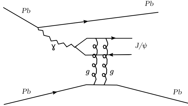
Figure 2.10: Lowest order Feynman diagram for J/\psi photo-production.
