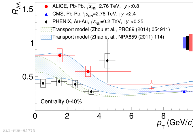
Figure 2.16: J/\psi R_{AA} measured at mid-rapidity as a function of p_T in central collisions (0-40%) by ALICE, PHENIX and CMS. The ALICE open marker corresponds to 0-50% centrality. Predictions by Transport models are shown. Figure from [84].
