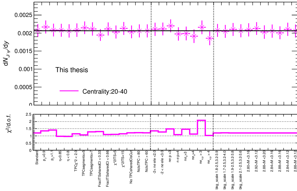
Figure 5.3: Corrected J/\psi yield calculated for each selection criteria variation in the centrality class 20 - 40\% . The horizontal black line corresponds to the mean value of all the variations. The vertical lines divide the different selection criteria in tracking, PID and signal extraction.
