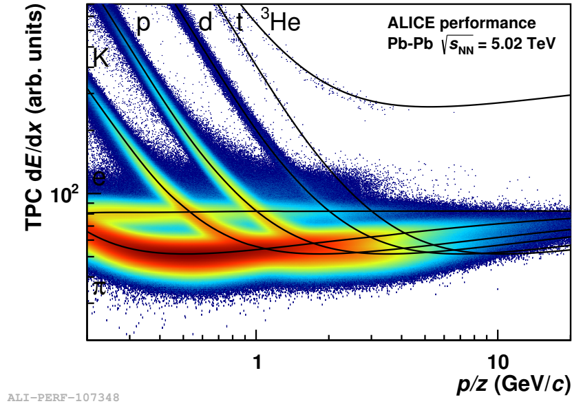
Figure 3.5: TPC- dE/dx distribution as a function of momentum for charged particles in Pb-Pb collisions at \sqrt{s_{\text{NN}}} = 5.02 TeV. The solid lines correspond to the calculated value of the Bethe-Bloch parametrization. Figure taken from [103].
