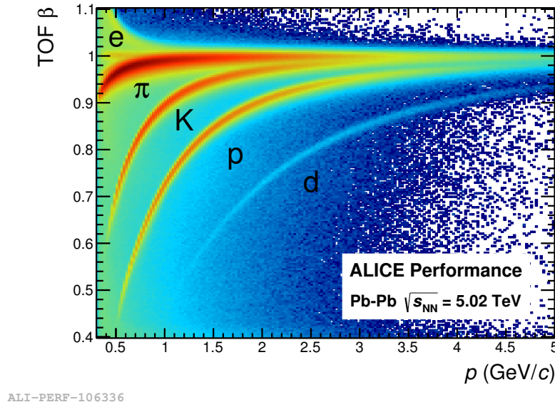
Figure 3.7: Velocity distribution measured by the TOF detector as a function of momentum for charged particles in Pb-Pb collisions at \sqrt{s_{NN}} = 5.02 TeV. Figure taken from [103].
