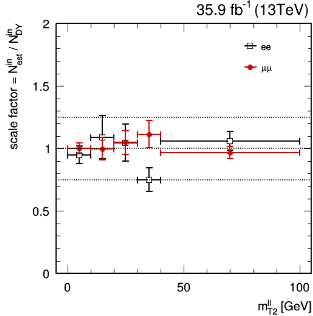
Figure 6.5: Scale factor obtained from the data-driven method applied to the Drell-Yan process as a function of M_{T2}(\ell\ell) for the same flavour channels, where its contribution is significant. Uncertainties are statistical only.
