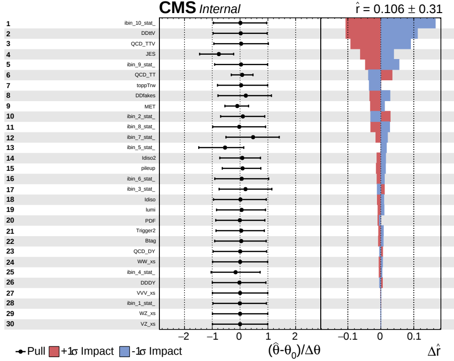
Figure 7.2: An illustrative example of the pulls and impacts plot (the chosen signal point is the 100 GeV scalar mediator). Impacts are shown on the right side by solid blue and red bars. They drive the ordering of the list. Nuisance names (according to the datacard nomenclature) and numbers are displayed on the left side. As it can be seen, only the first thirty are listed. Pulls come in the middle by dots and bars. The \hat{r} value at the top right-hand corner is the maximum-likelihood estimator of \mu , i.e. \hat{r} \equiv \hat{\mu} . The label “ (\hat{\theta} - \theta_0)/\Delta\theta ” might be confusing. What it actually means is “ (\hat{\theta} - \tilde{\theta})/\tilde{\theta} ”. All the fourteen plots are given in appendix B.
