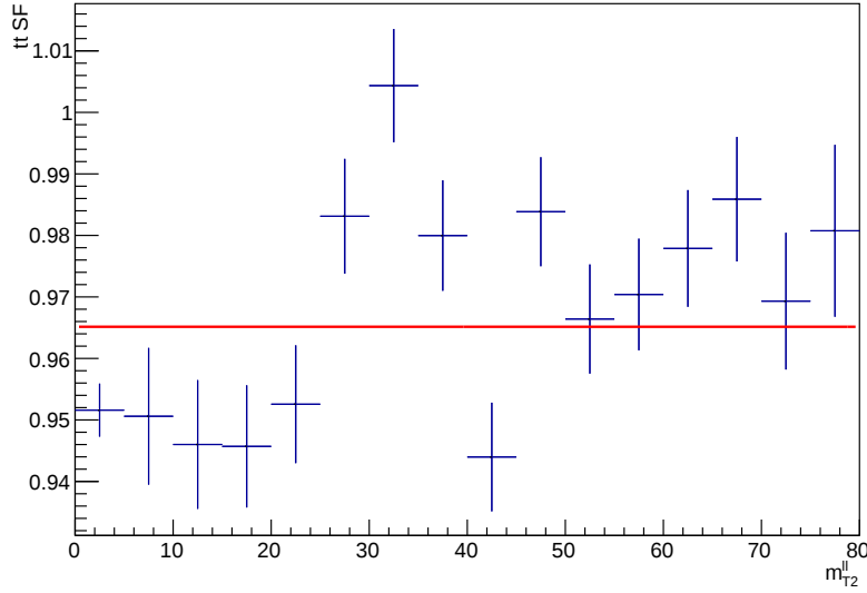
Figure 6.1: SF_{t\bar{t}} per bin of M_{T2}(\ell\ell) . In red, their fit to a constant. Notice the vertical axis starting at 0.93.
