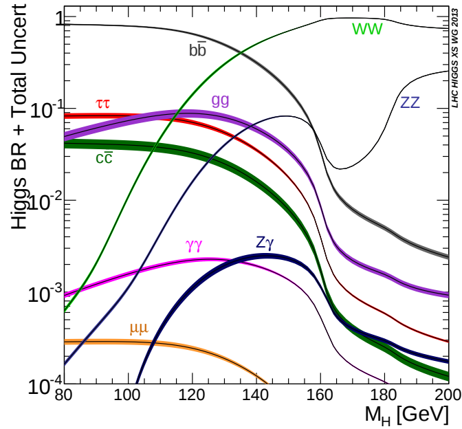
Figure 2.3: Relative decay rates for the SM Higgs as a function of its mass, unknown until 2012.
