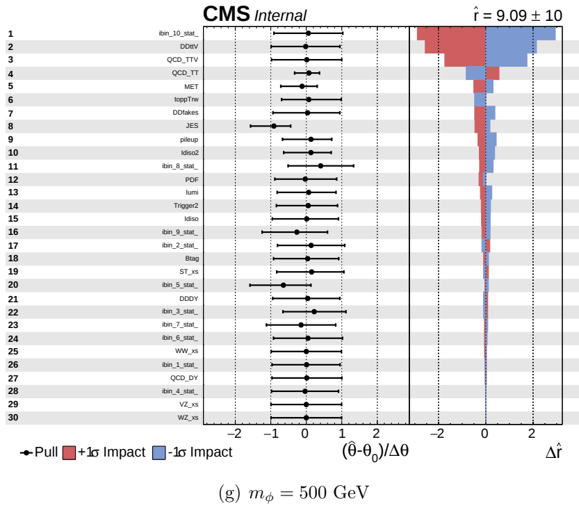
Figure B.2: Pulls (center) and impacts (right) for different pseudoscalar models. Nuisances are identified by their datacard names (left) (cont.)
