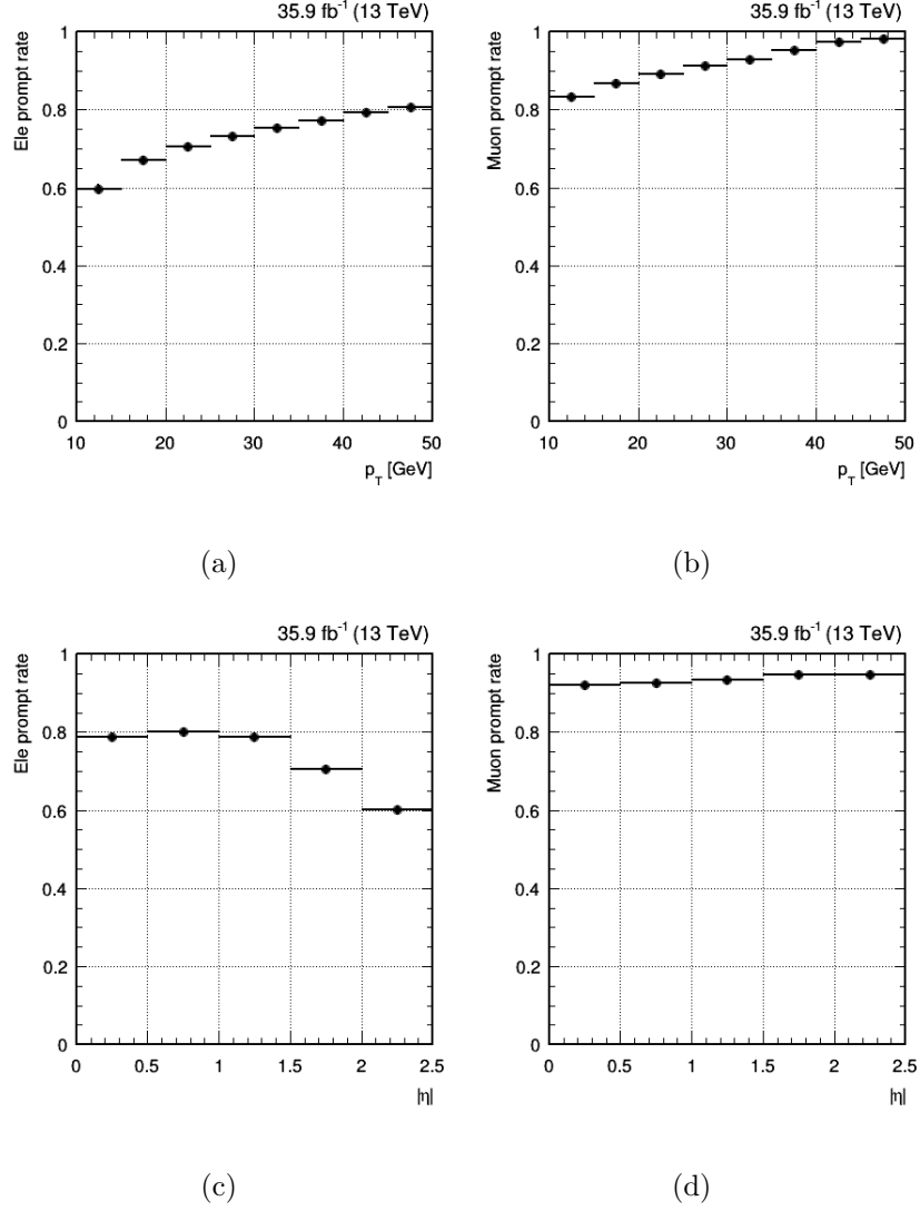
Figure 6.3: PRs obtained by applying a general tag and probe method within a Z enriched region for both electrons (left) and muons (right), with respect to the lepton p_T (top) and |\eta| (bottom).
