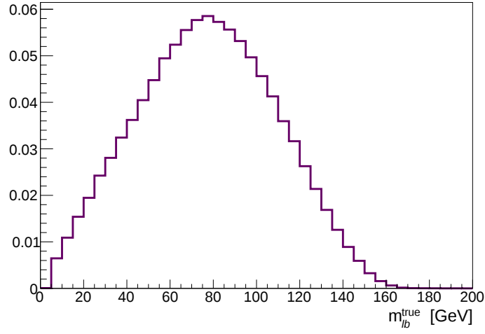
Figure 5.2: Normalised distribution of m_{\ell b} from simulated events, i.e. not suffering from inefficiencies from the reconstruction.
