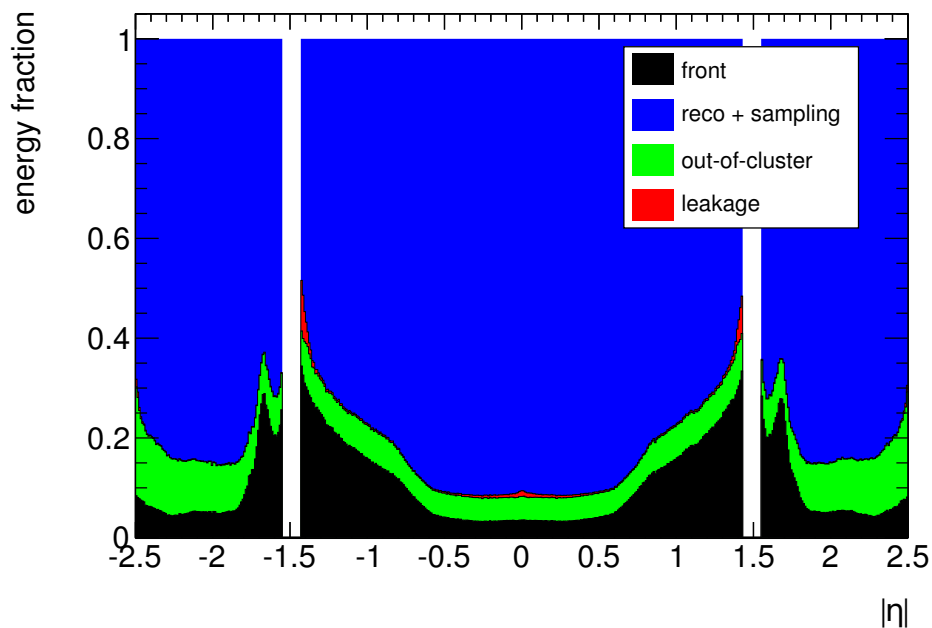
Figure 4.2: Energy decomposition for 50 GeV electrons.
