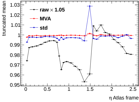
(f) pseudorapidity in the Atlas frame
