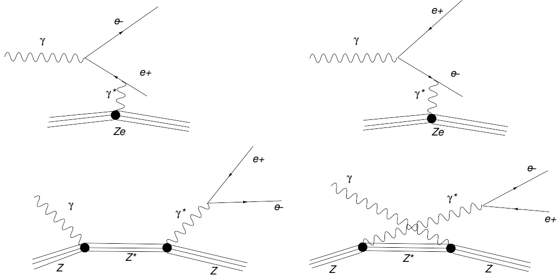
Figure 3.17: Leading-order Feynman diagrams for photon conversions.
