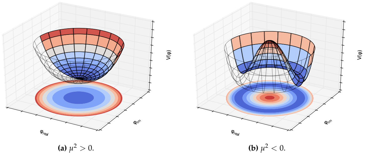
Figure 1.1: Illustration of the Higgs potential for a scalar field \Phi = \phi_{\text{real}} + i\phi_{\text{im}} with \mu^2 > 0 and \mu^2 < 0 .
