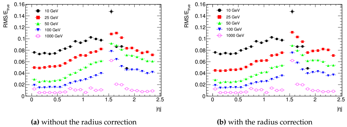
Figure 4.43: RMS for converted photons (a) without and (b) with the tool without pileup.
