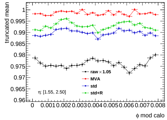
(k) \phi electrode modulation (endcap)
