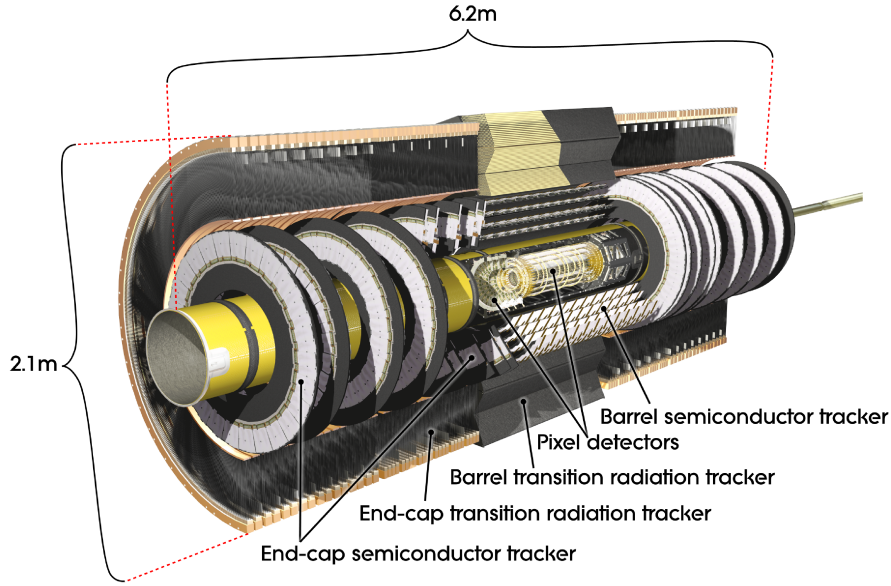
Figure 3.3: Cut-away view of the ATLAS Inner Detector.
