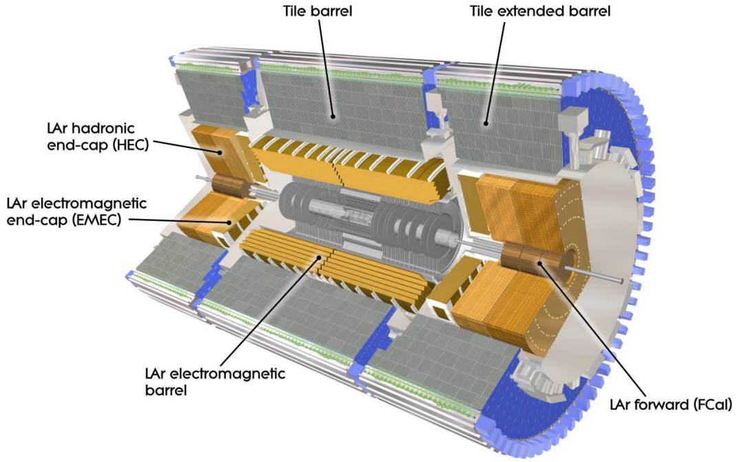
Figure 3.9: Cut-away view of the ATLAS calorimeter system.
