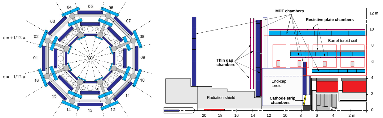
(a) R - \phi view of the barrel Muon Spectrometer, illustrating large sectors (dark blue), small sectors (light blue) and the magnet coils (dark grey).
