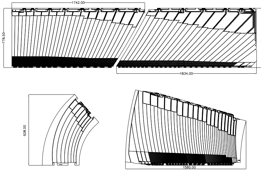
Figure 3.11: The four types of electrodes of the electromagnetic calorimeter. The two top ones correspond to barrel electrodes: |\eta| < 0.8 (left) and |\eta| > 0.8 (right). The bottom left is an endcap inner wheel electrode and the bottom right is the outer wheel. Dimensions are in mm.
