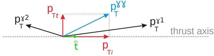
Figure 6.4: Illustration of the p_{Tt} quantity.
