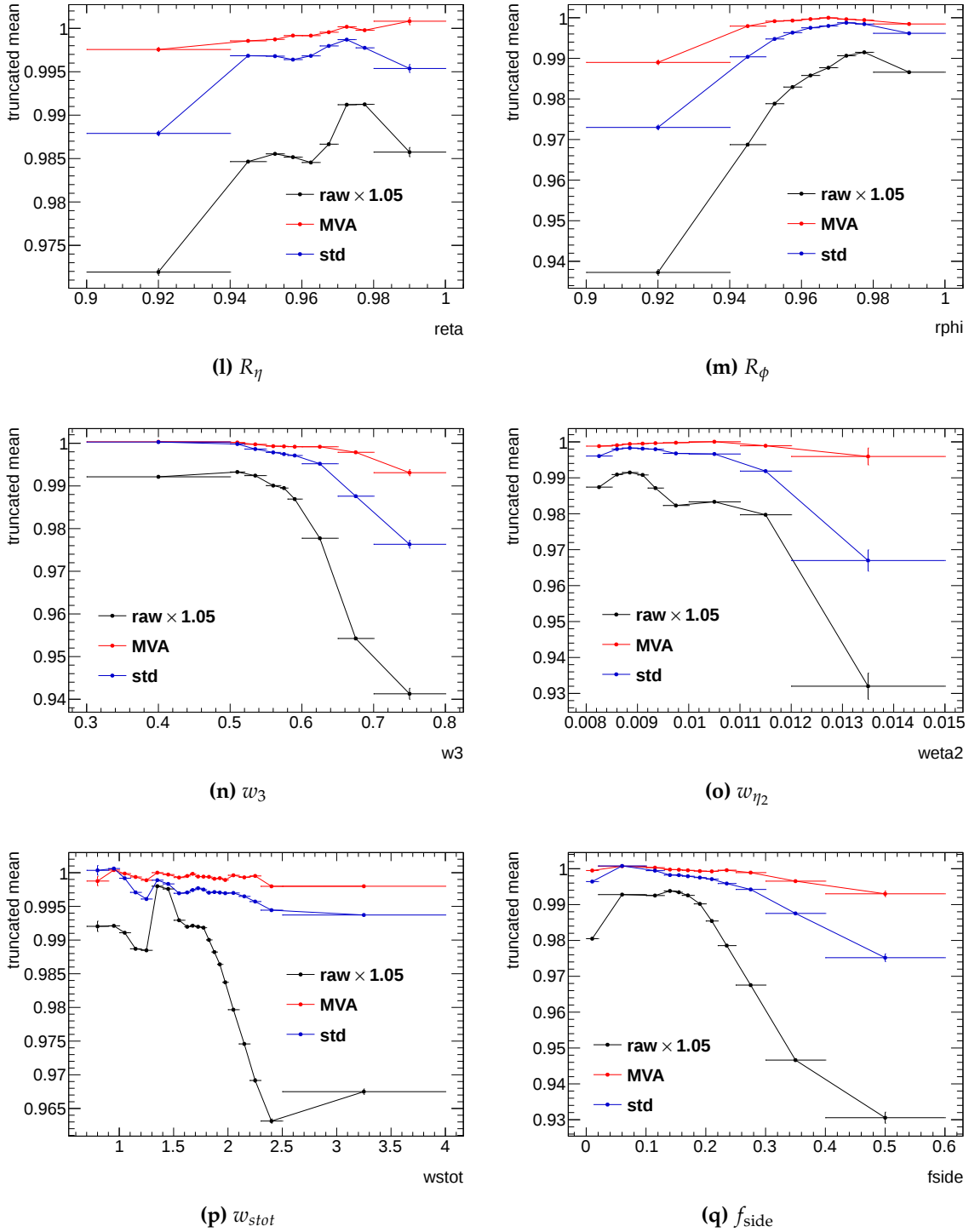
Continued Figure 5.4: The correlation between several variables and the truncated mean of the E/E_{\text{true}} before the calibration (black), after the standard calibration (blue) and after the MVA calibration described in section 5.6 (red) for unconverted photons. The point for the raw-energy are scaled by a factor 1.05. If not specified the whole test sample is used 7 \text{ GeV} < E_{T,\text{true}} < 500 \text{ GeV} and 0 < |\eta| < 2.5 .
