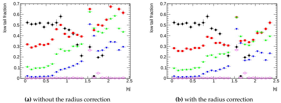
Figure 4.44: fraction of event in the low tail for converted photons (a) without and (b) with the tool without pileup.
