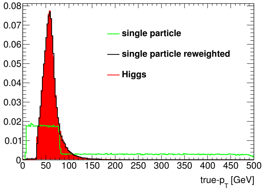
Figure 5.27: Reweighting of the single particle sample to match the photon p_T^{\text{true}} distribution from the Higgs decay.
