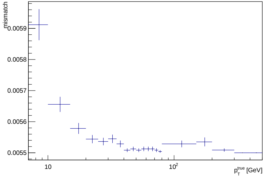
Figure 5.3: mismatch for electron versus the true p_T .
