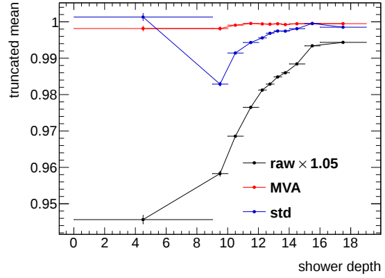
(g) shower depth
