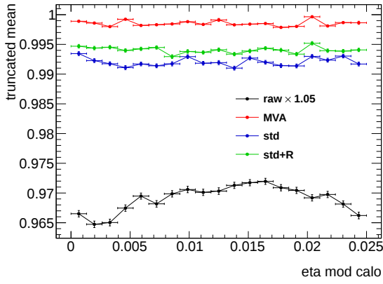
(h) \eta modulation
