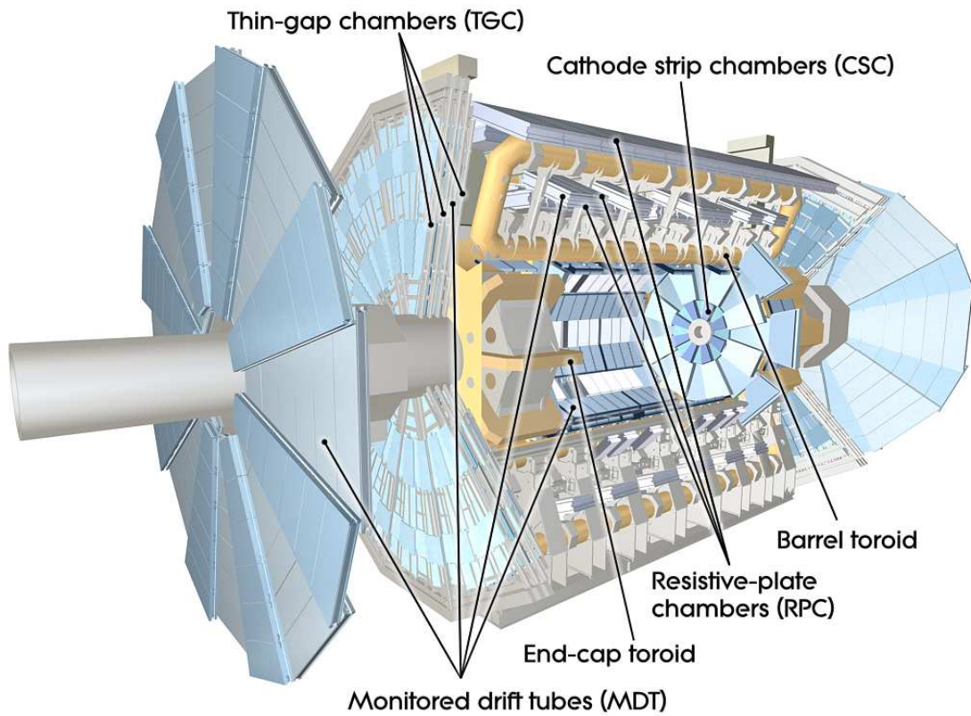
Figure 3.20: Cut-away view of the ATLAS muon system.
