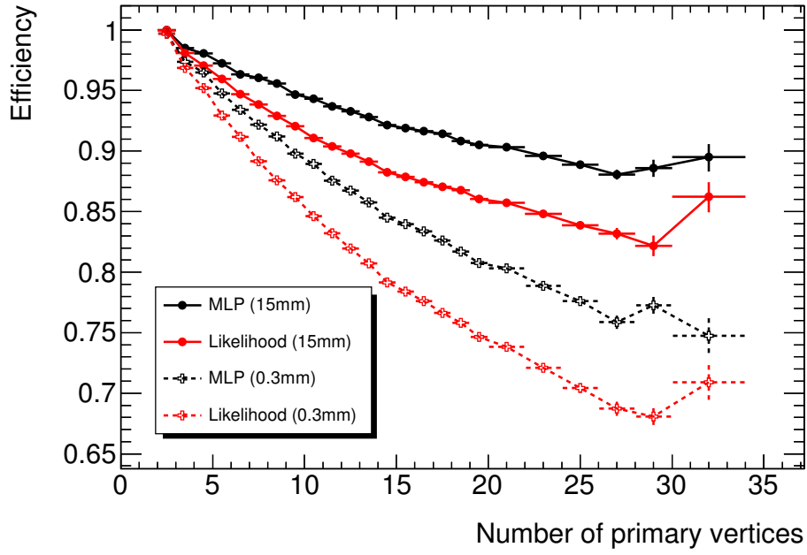
Figure 6.2: Efficiency to select a primary vertex close to the position of the Higgs production along the z-axis inside a window of 15 mm or 0.3 mm as a function of the number of reconstructed vertices.
