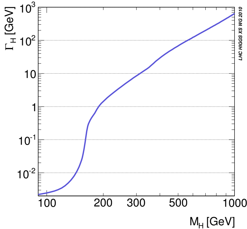
Figure 1.11: Total width of the SM Higgs boson as a function of its mass. Extracted from ref. [34].
