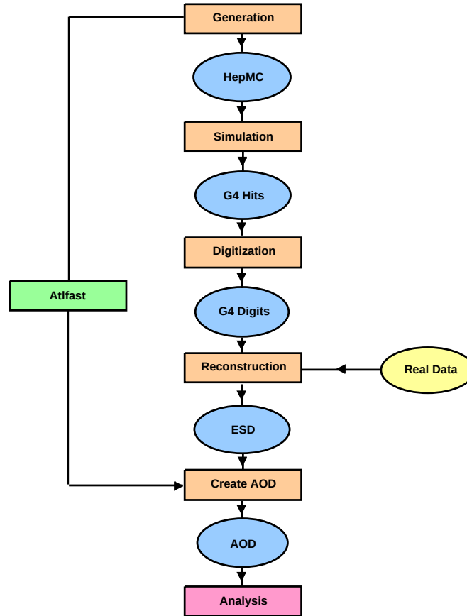
Figure 3.30: Schematic representation of the generation / simulation / reconstruction chain for Monte Carlo and real data in ATLAS. Extracted from ref. [84].
