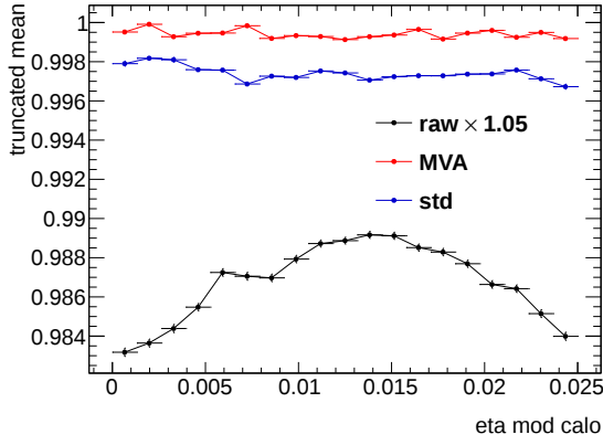
(h) \eta modulation
