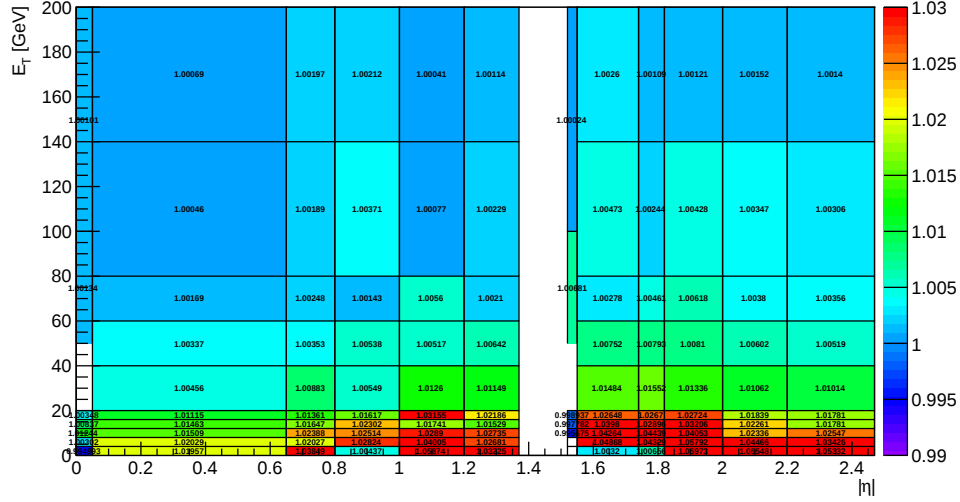
Figure 5.12: Peak position of the E_{\text{MVA}}/E_{\text{true}} distribution for electrons using the mean of the event inside the smallest range containing 10% of the statistics.
