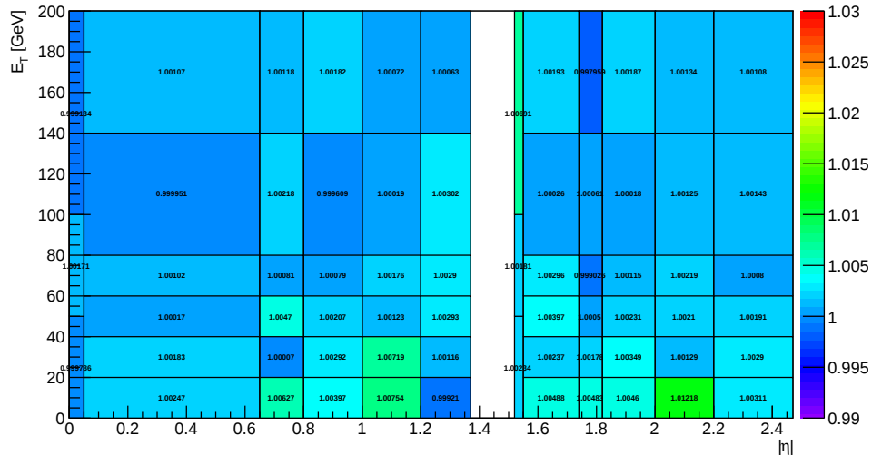
Figure 5.13: Peak position of the E_{\text{MVA}}/E_{\text{true}} distribution for converted photons using the mean of the event inside the smallest range containing 10% of the statistics.
