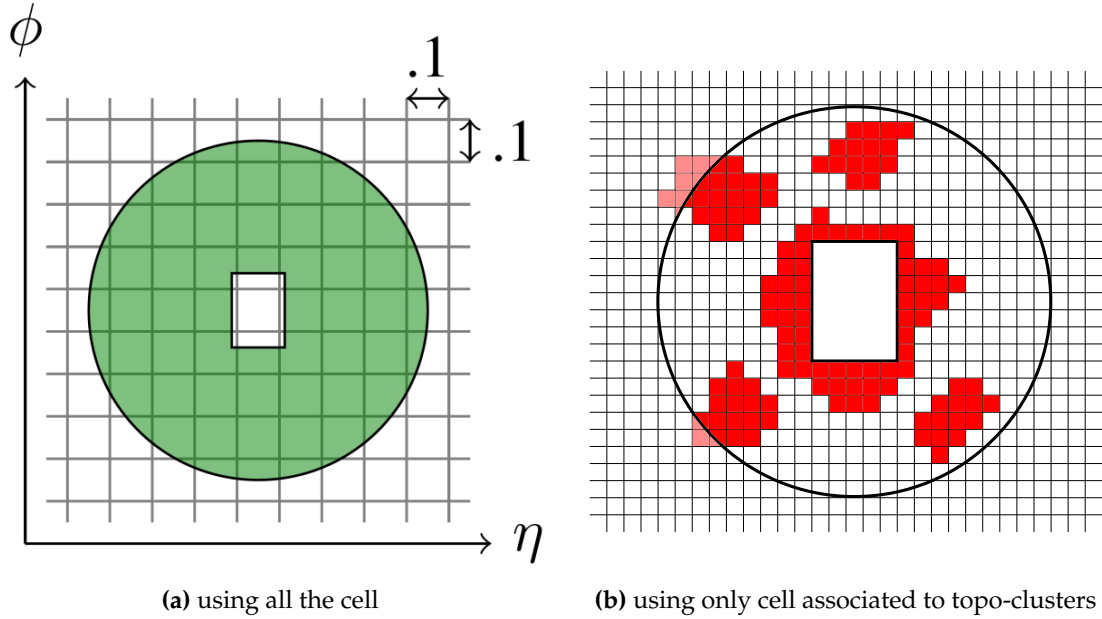
Figure 3.18: An illustration of the calculation of the isolation variable in ATLAS. A circle is drawn around the photon in \eta \times \phi space, and the energy from (a) all calorimeter cells (b) calorimeter cell associated to topocluster inside of that circle are summed. The energy in a central rectangle of the cone is excluded, in an attempt to remove the electron or photon shower.
