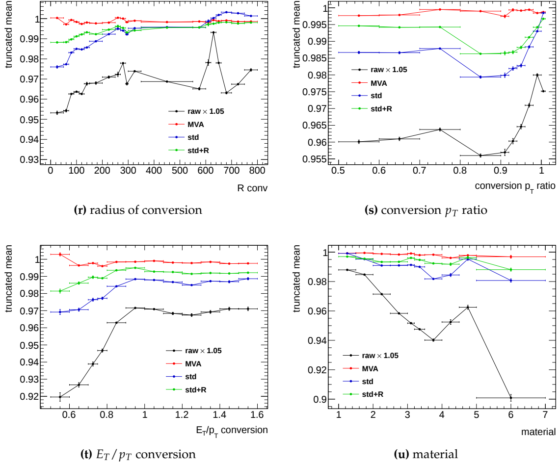
Continued Figure 5.5: The correlation between several variables and the truncated mean of the E/E_{\text{true}} before the calibration (black), after the standard calibration (blue), after the standard calibration corrected using the radius of conversion (green) and after the MVA calibration described in section 5.6 (red) for converted photons. The point for the raw-energy are scaled by a factor 1.05. If not specified the whole test sample is used 7\text{ GeV} < E_{T,\text{true}} < 500\text{ GeV} and 0 < |\eta| < 2.5 .
