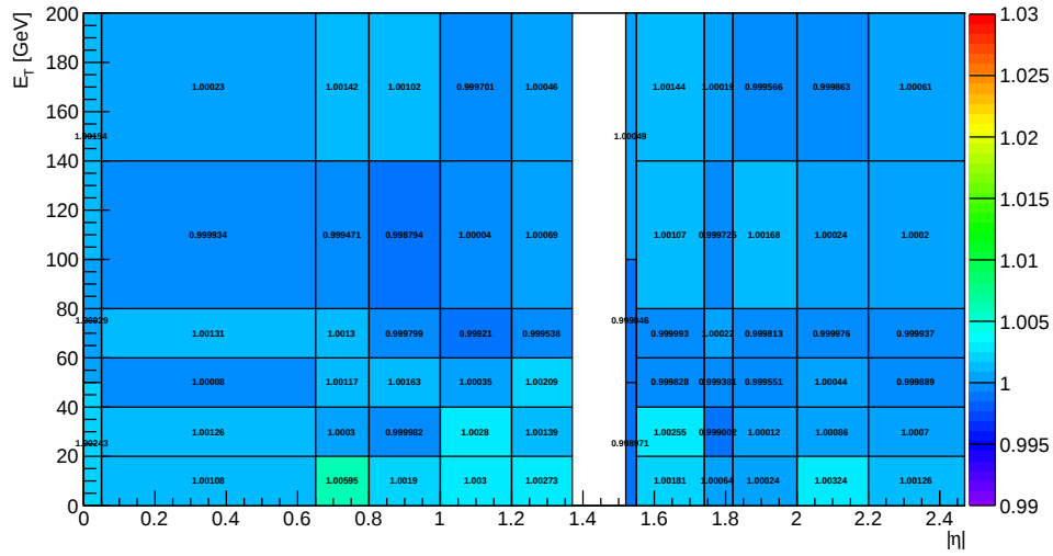
Figure 5.14: Peak position of the E_{\text{MVA}}/E_{\text{true}} distribution for unconverted photons using the mean of the event inside the smallest range containing 10% of the statistics.
