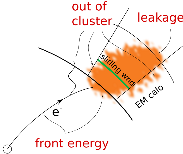
Figure 4.1: Sketch of the various components of the energy loss affecting the linearity and the resolution of the final energy measurement.
