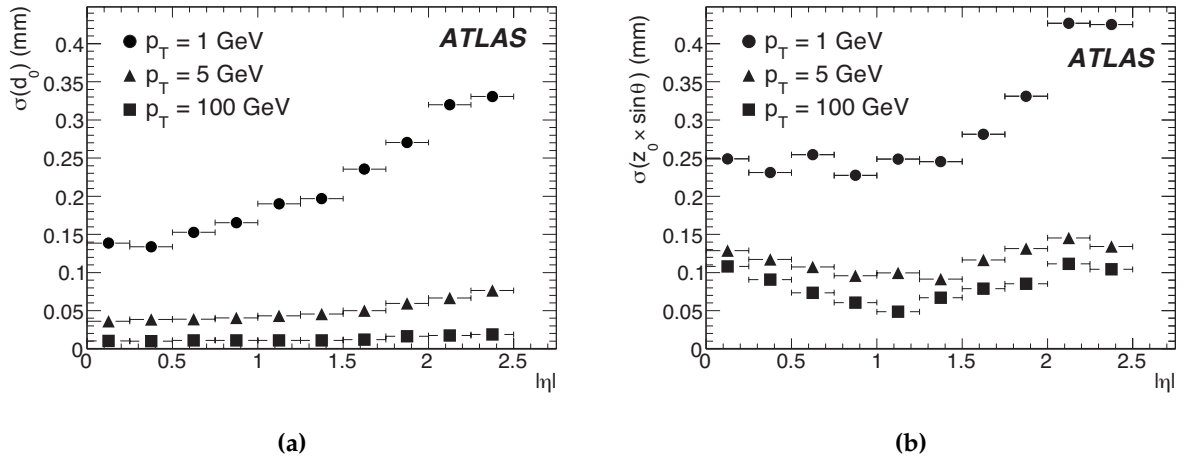
Figure 3.8: Expected resolution on (a) transverse and (b) modified longitudinal impact parameters ( d_0 and z_0 \times \sin \theta , respectively) as a function of |\eta| for pions of p_T = 1 GeV, 5 GeV and 100 GeV.
