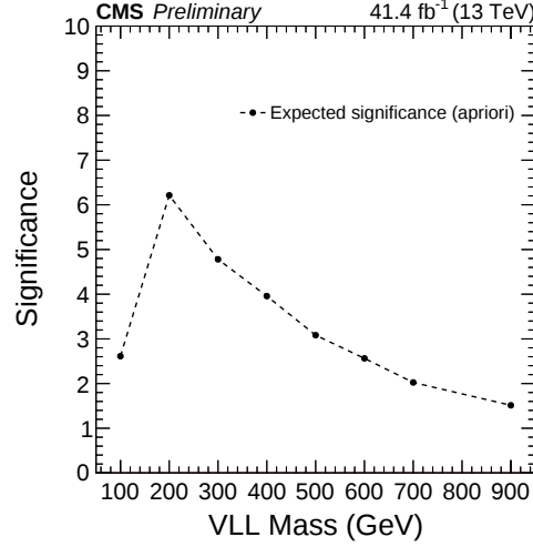
FIGURE 6.8: The expected signal significance as a function of VLL mass after statistically combining all the 3L, 4L and 2L1T channels in the analysis.
