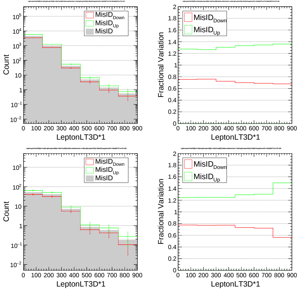
FIGURE 5.19: Impact of varying tau rates rates on L_T distribution in two leptons of opposite charge + hadronic tau channels in low p_T^{\text{miss}} (upper plots) and high p_T^{\text{miss}} (bottom plots).
