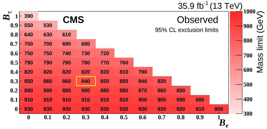
FIGURE 7.12: Two dimensional electron-tau branching ratio dependent observed exclusion limits at 95% CL on the production cross-section of \Sigma pairs, as calculated with the asymptotic CLs mode of the Higgs Combination Tool.
