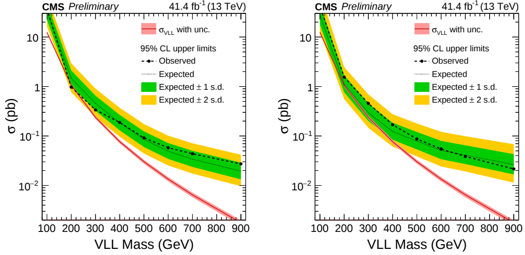
FIGURE 6.4: The 95% confidence level upper limits on the cross section for production of VLL pairs ( \tau'^+\tau'^- , \tau'^\pm\nu' and \nu'\nu' ). Left in 3L channel, right in 4L channels. Also shown is the theoretical prediction for the section of the VLL pair production.
