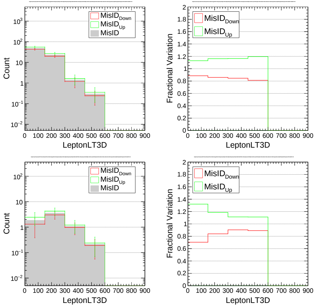
FIGURE 5.22: Impact of varying light lepton rates rates on L_T distribution in two leptons of same charge + hadronic tau channels in low p_T^{\text{miss}} (upper plots) and high p_T^{\text{miss}} (bottom plots).
