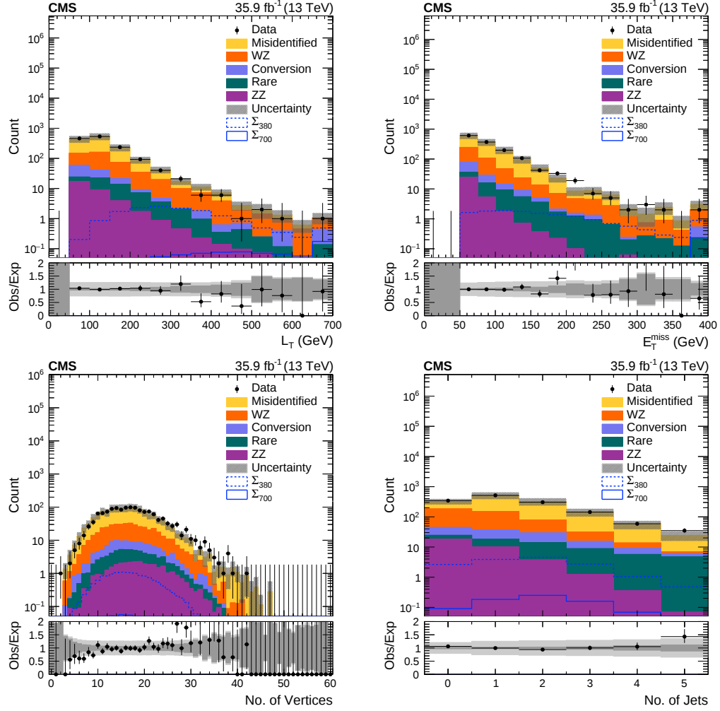
FIGURE 7.6: L_T (upper left), p_T^{\text{miss}} (upper right), primary vertex multiplicity (lower left), and jet multiplicity (lower right) distributions for the 3 lepton, below-Z signal region as defined in Table 7.2. The expected yields of the Seesaw signal model with M_\Sigma = 380 GeV and M_\Sigma = 700 GeV are overlaid. The last bins include overflow events, and the uncertainty bands in the ratio plots include statistical (dark) and systematic (light) uncertainties.
