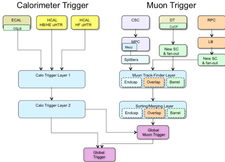
FIGURE 3.10: A schematic diagram of the L1 trigger logic is shown.
