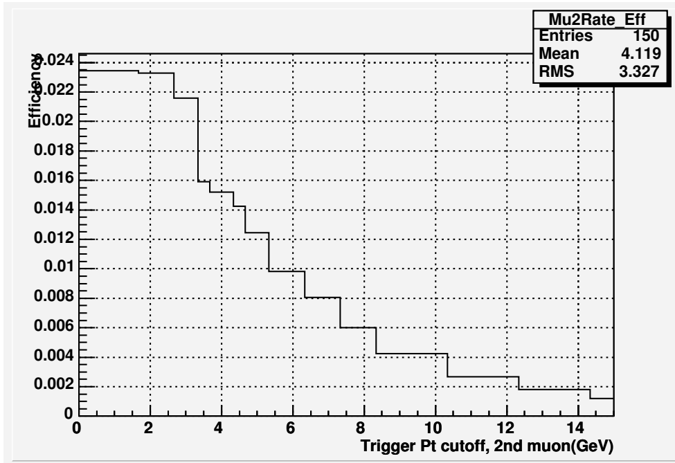
Figure 4.13: Signal efficiency for the 2\mu trigger for diffractive Higgs events for a Higgs with a mass of 120 GeV. The Higgs sample was generated with ExHuME.
