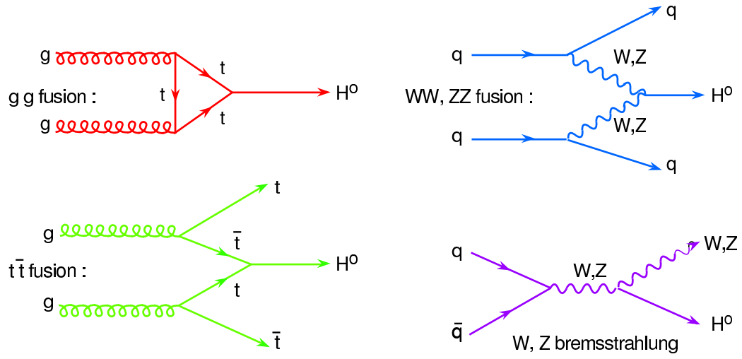
Figure 2.1: Higgs production Feynman diagrams at hadron colliders, from Ref. [22]
