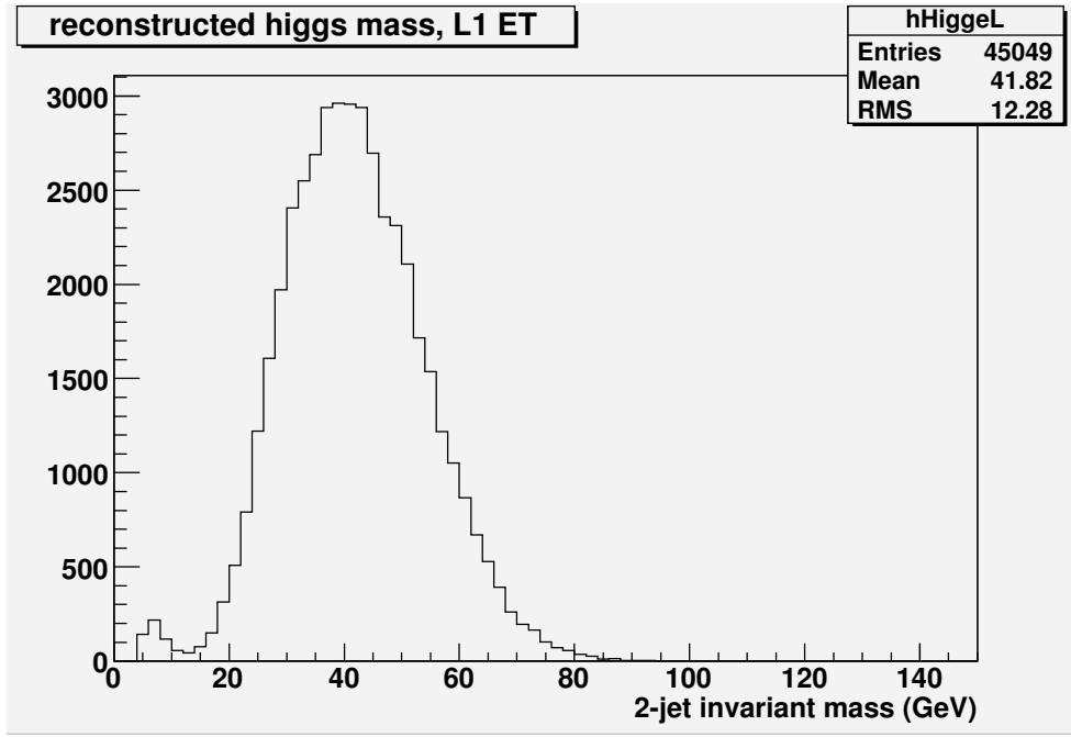
Figure 4.6: Invariant mass of two L1 jets reconstructed from the measured L1 jet E_T for events with exactly two L1 jets for a Higgs with a mass of 120 GeV, including detector effects.
