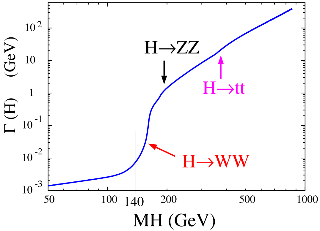
Figure 2.4: Decay width of SM Higgs, as a function of Higgs mass, from Ref. [23]
