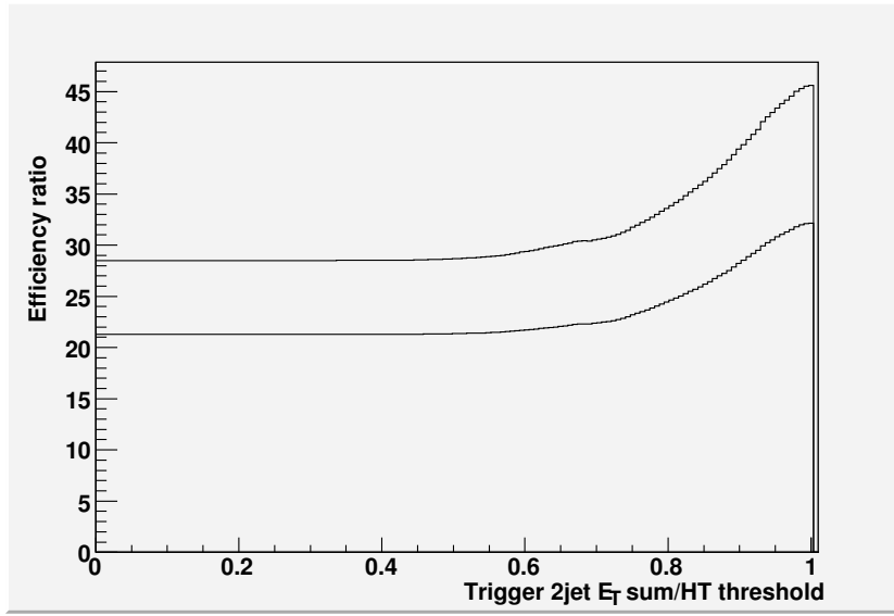
Figure 4.17: Efficiency ratio as a function of a 2-jet E_T sum/ H_T threshold requirement. H_T is the sum of the E_T 's of all L1 jets. The calibrated jet E_T is used. The upper curve is for central jets and the lower for all jets.
