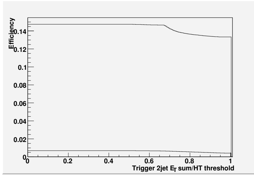
Figure 4.15: Efficiency for a 2-jet E_T sum/ H_T requirement at L1. H_T is the sum of the E'_T s of all L1 jets, not just the 12 jets available as L1 trigger objects. The calibrated jet E_T is used. The upper curve is for the EDDE Higgs sample and the lower for the QCD background.
