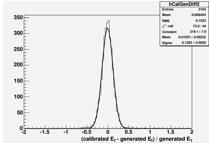
Figure A.3: Fractional deviation of the calibrated E_T from the generated E_T for an independent QCD sample ( 170 \text{ GeV} < \hat{p}_T < 230 \text{ GeV} ). The measured L1 E_T was required to be within the domain of validity of the calibration.
