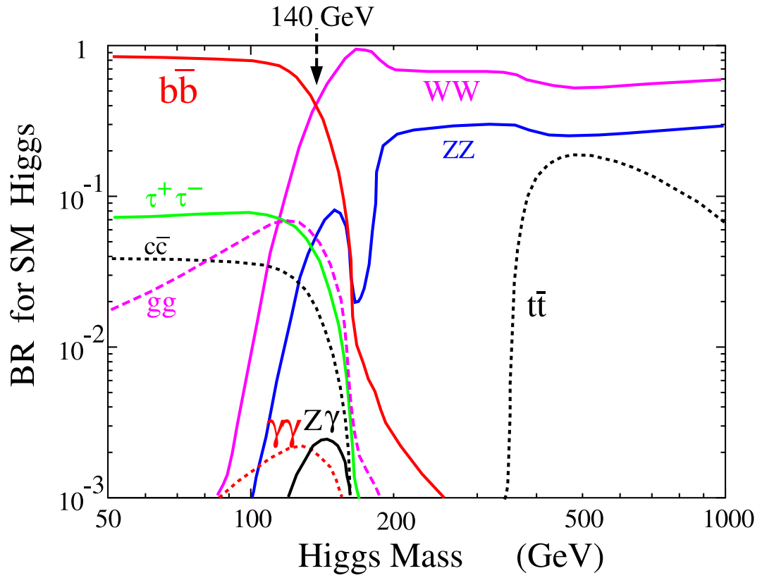
Figure 2.3: Branching ratio of various Higgs decay modes, as a function of Higgs mass, from Ref. [23]
