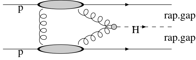
Figure 2.5: Feynman diagram of diffractive Higgs production at LHC
