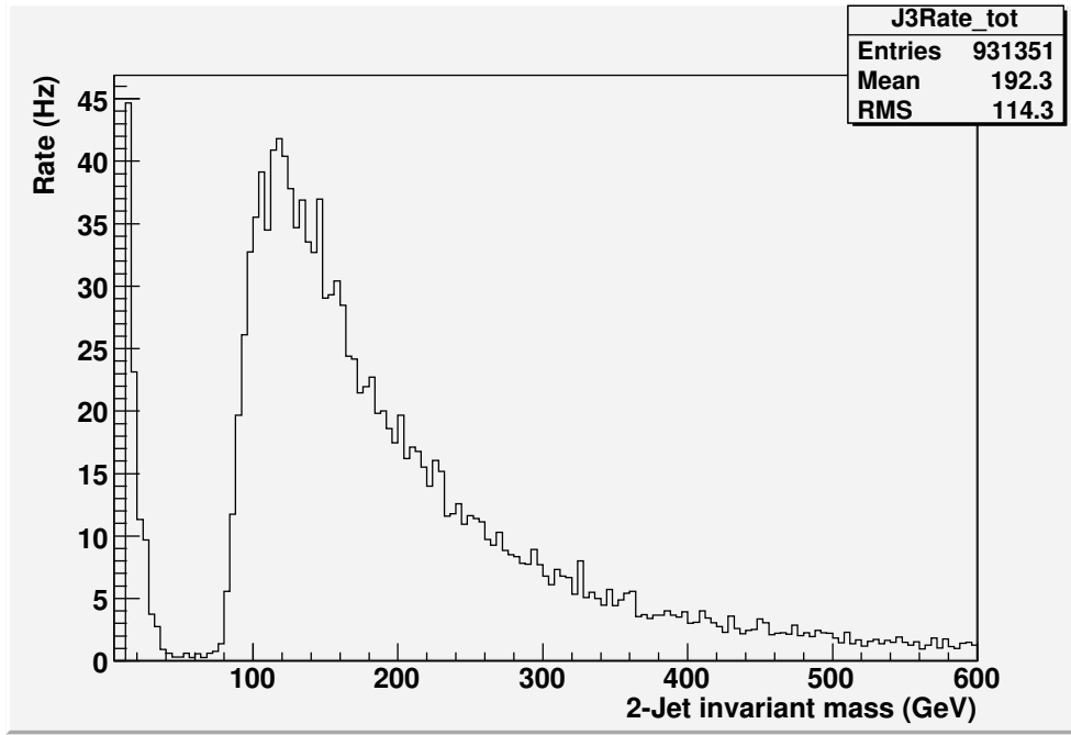
Figure 4.8: Rate of 2-jet invariant mass of calibrated jets for the QCD background sample for a luminosity of 10^{32} \text{ cm}^{-2} \text{ s}^{-1} . Only events with at least two calibrated L1 jets with an E_T above 40 GeV were considered.
