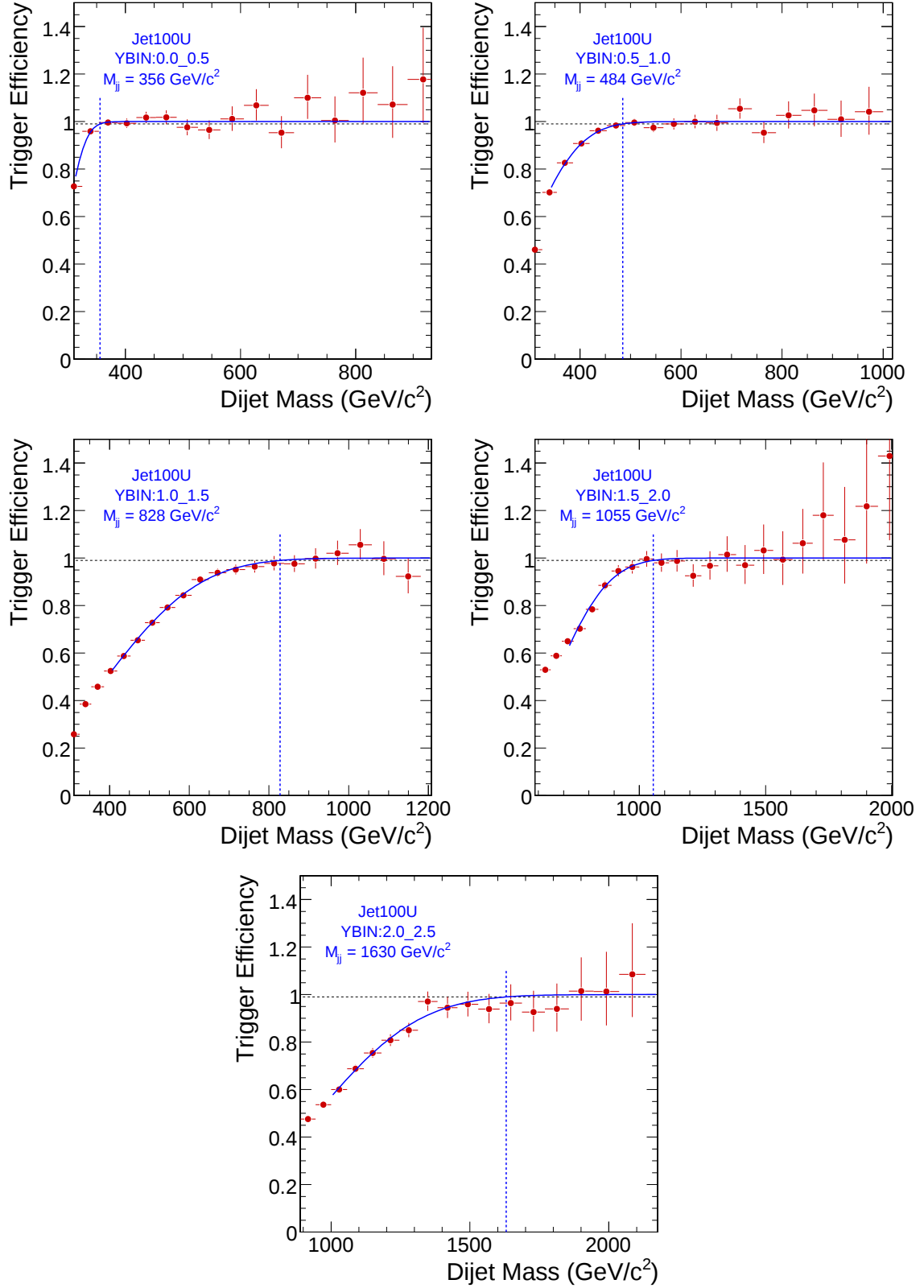
Figure B.3. Relative trigger efficiencies as a function of dijet mass for the five different |y|_{\max} bins and for the HLT_Jet100U trigger. The 100% efficiency point is determined by performing a fit with an error function.
