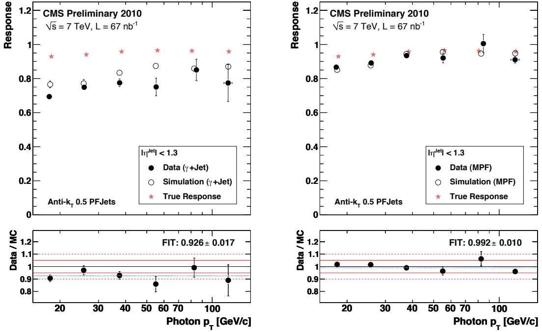
Figure 5.20. Response of \langle p_T/p_\gamma \rangle (left) and MPF response (right) as a function of photon p_T from data and simulation [36].
