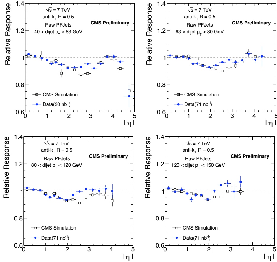
Figure 5.19. Relative jet response for PF jets as a function of \eta , for various p_T^{dijet} bins [36].
