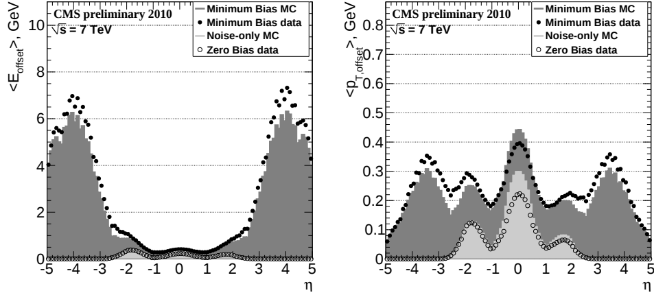
Figure 5.18. Offset contribution from the noise only and noise+one pile-up as function of \eta in energy (left) and transverse momentum (right) [36].
