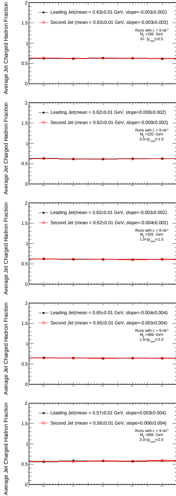
Figure C.2. The charged hadron fraction of the leading and second jet for the five different y_{\text{max}} bins and for the HLT_Jet30U trigger as a function of time (run number), fitted with a first degree polynomial.
