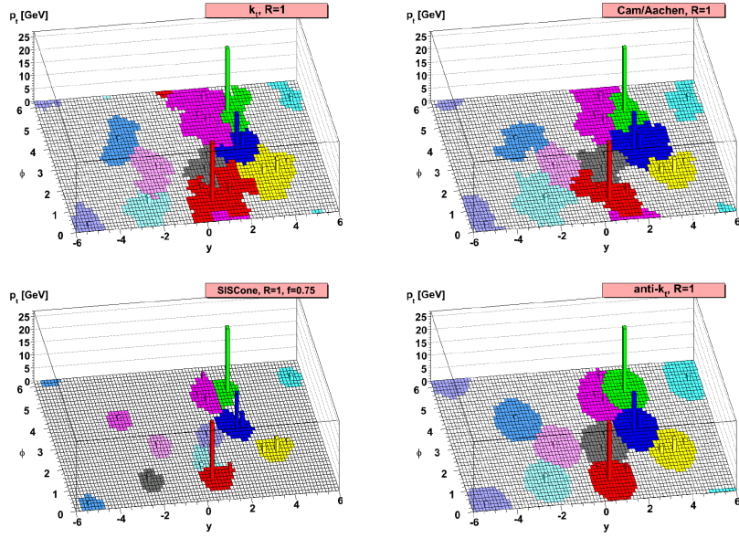
Figure 4.5. Illustration of different jet algorithms in parton level [28].
