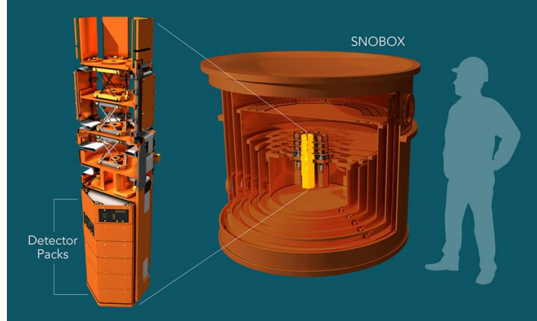
Figure 4.4: Detector setup of the SuperCDMS direct detection experiment at SNOLAB, in Sudbury, Canada [42]. The experiment uses cryogenic bolometer technology for dark matter detection.
