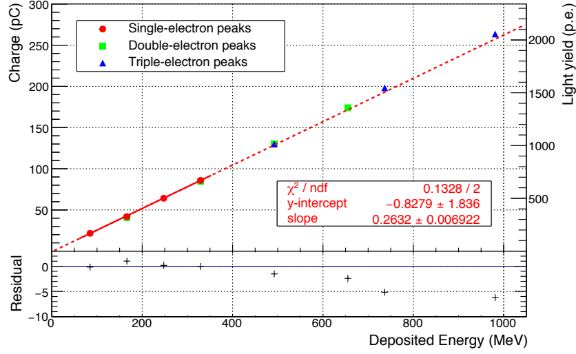
Figure 14.13: Detector linearity as a function of deposited energy (corrected for average leakage energy, see Figure 14.10). Only single-electron peaks are fit. The residuals are also shown, demonstrating good linearity up to at least 400 MeV. A bias in the linearity is introduced for multiple-electron peaks due to the nature of our threshold setting and the after-pulse ringing, but does not affect the resolution since only single-electron peaks are used. The light yield is shown on the right, assuming a gain of 8 \times 10^5 for a PMT operating voltage of 1,600 V [133]. The obtained light yield is 2.05 p.e./MeV.
