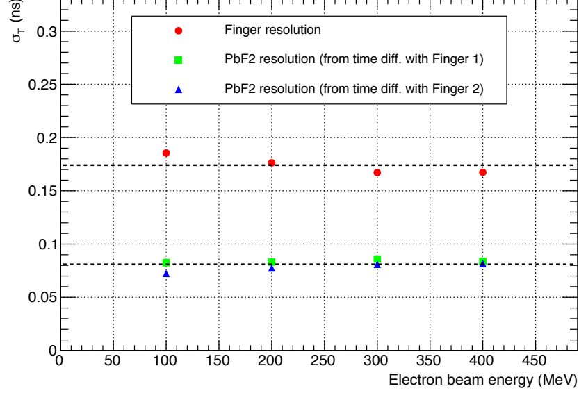
Figure 14.16: PbF 2 and finger timing resolutions, calculated from the difference in rise time between the different channels. The SAC timing resolution of roughly 80 ps meets PADME’s requirements. Note that timing resolution is not significantly affected by beam energy due to our method of estimating the arrival time. This method relies on calculating the slope of the rising pulse, whose midpoint does not vary much with amplitude.
