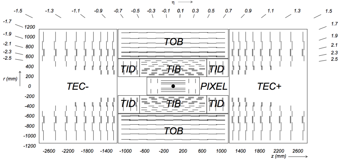
Figure 6.6: Layout of CMS's tracker [68]. Both inner and outer tracker layers are shown in this r - z projection.
