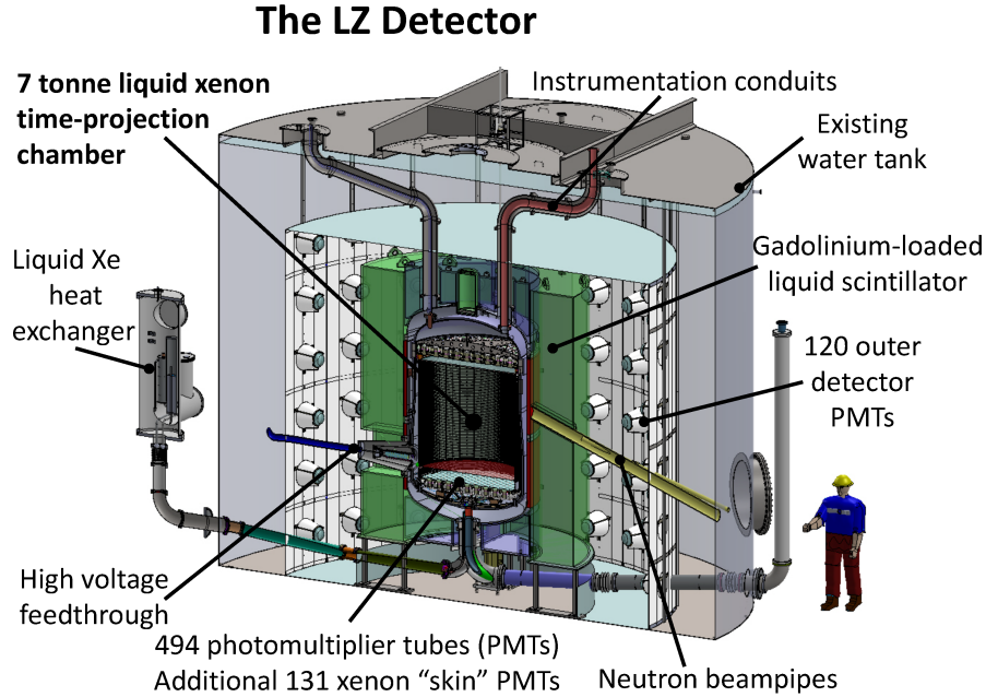
Figure 4.3: The LZ direct detection experiment under construction at the Sanford Underground Research Facility in Lead, South Dakota [41]. The detector uses liquid xenon as active medium.
