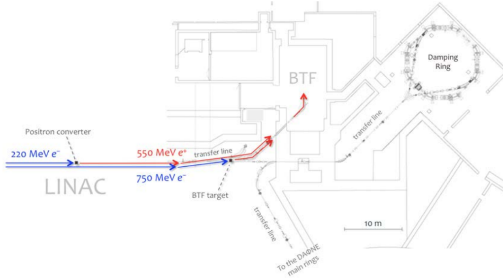
Figure 13.5: Primary and secondary positron beams delivered to the BTF line from the LINAC for injection into PADME [120].
