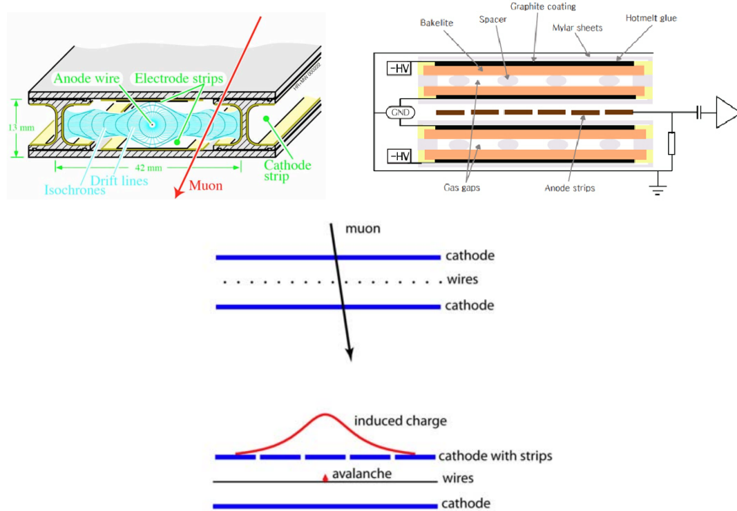
Figure 6.12: Comparison of different muon detector technologies employed at CMS [68, 86]. DT is shown on the upper left, RPC on the upper right, and CSC on the lower center.
