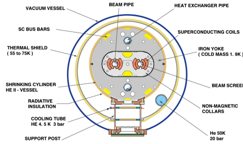
CROSS SECTION OF LHC DIPOLE
