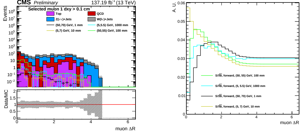
Figure 9.5: N-1 distributions of dimuon dR for signal and background simulated samples, and corresponding backward cumulative distributions (right). The optimal threshold is near dR < 1 .
