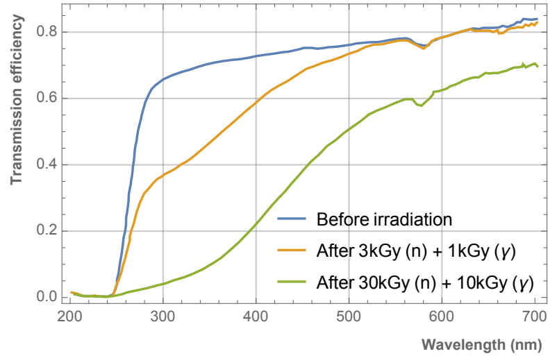
Figure 14.5: Transmission efficiency data before and after 4 kGy and 40 kGy of irradiation with neutrons and gamma rays [138], for a 1\text{ cm}^3 \text{PbF}_2 cube. Comparing with our expected radiation doses (Figure 14.4), the transmission loss for PADME crystals should be negligible.
