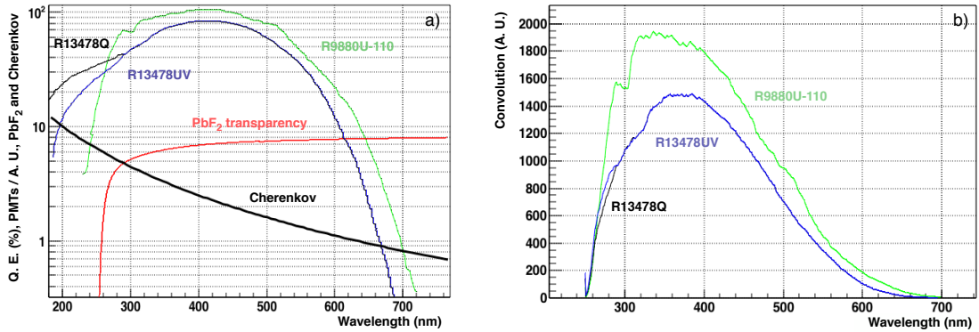
Figure 14.2: (a) Quantum efficiency (QE) curves for three different PMTs: R13478Q (black), R13478UV (purple), and R9880U-110 (green) [133, 134]. The Cherenkov spectrum (bold black) and \text{PbF}_2 transparency (red, [132]) are also plotted for comparison. (b) Convolution of each QE curve with \text{PbF}_2 transparency and Cherenkov spectrum. Due to the drop in transparency below 250 nm there is effectively no difference between the two R13478 PMT models. The R9880U-110 PMT has about 30% better performance over the entire spectrum.
