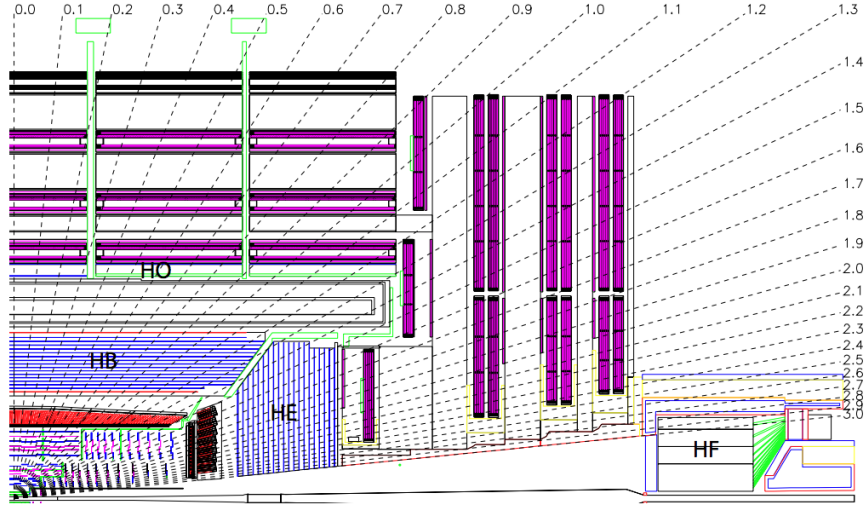
Figure 6.10: Layout of CMS's hadronic calorimeter [68]. All components are shown in this r - z projection. The coverage of the hadronic calorimeter is roughly |\eta| < 4 .
