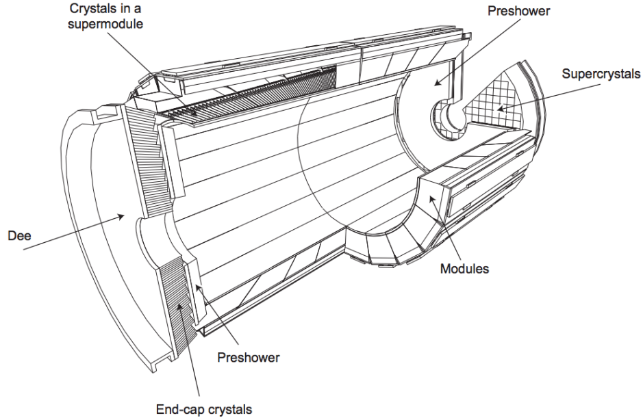
Figure 6.9: Layout of CMS's electromagnetic calorimeter [68]. The barrel, pre-shower, and endcap components together cover a pseudorapidity range of 0 to 4.
