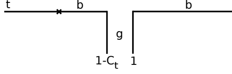
Figure 3.16: The probabilities of radiation from the colour lines of a gluon undergoing secondary radiation of a gluon whilst colour connected to a top and bottom in this example.
