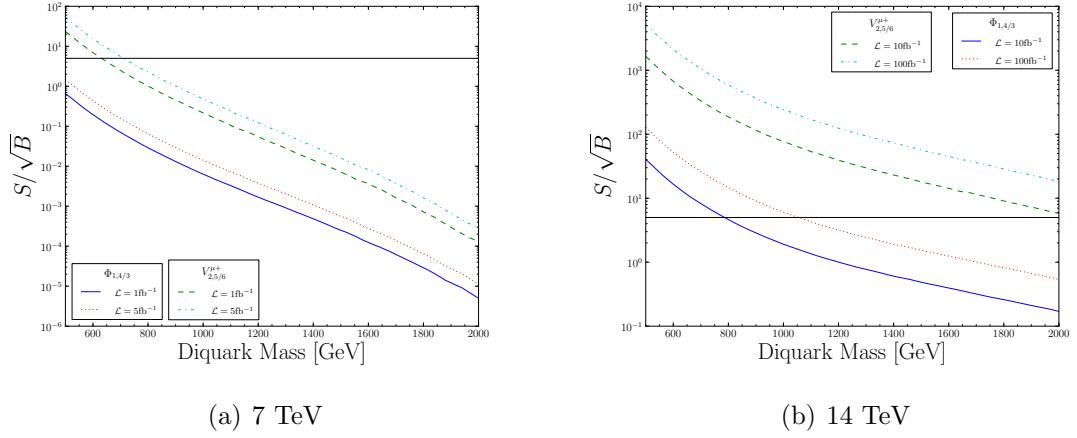
Figure 4.14: \frac{S}{\sqrt{B}} for the scalar and vector diquark at luminosities of \mathcal{L} = 1 \text{ fb}^{-1} and \mathcal{L} = 5 \text{ fb}^{-1} at \sqrt{s} = 7 \text{ TeV} and \mathcal{L} = 10 \text{ fb}^{-1} and \mathcal{L} = 100 \text{ fb}^{-1} at \sqrt{s} = 14 \text{ TeV} . The black horizontal line shows \frac{S}{\sqrt{B}} = 5 .
