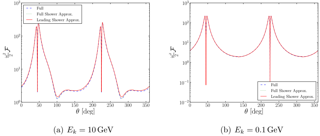
Figure 3.11: The radiation pattern for single gluon emission from e^+e^- collisions. We show the full radiation pattern, the shower approximation to the full radiation pattern and shower approximation with the interference terms neglected. These interference terms are so small, that this line lies on top of the shower approximation line.
