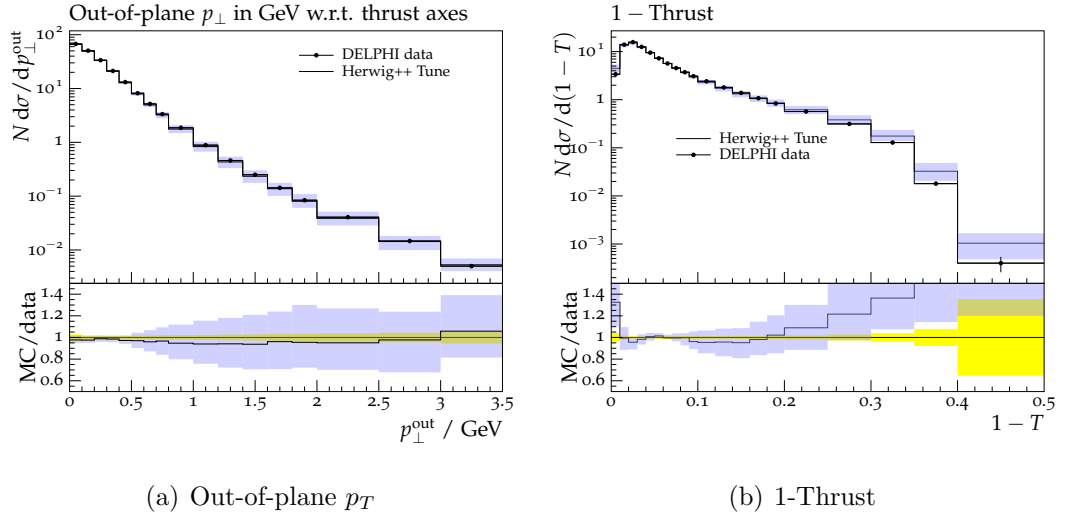
Figure 2.5: Results from the DELPHI [2] analysis of out-of-plane p_T with-respect-to the thrust axis and 1-thrust showing the new tune and the envelopes corresponding to a change in \Delta\chi'^2/N_{\text{df}} = 5 .
