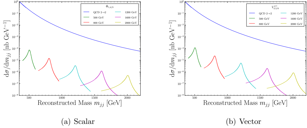
Figure 4.10: The dijet mass spectrum at \sqrt{s} = 14 TeV for 500 GeV, 800 GeV, 1200 GeV, 1600 GeV and 2000 GeV diquark masses with the couplings given in the text.
