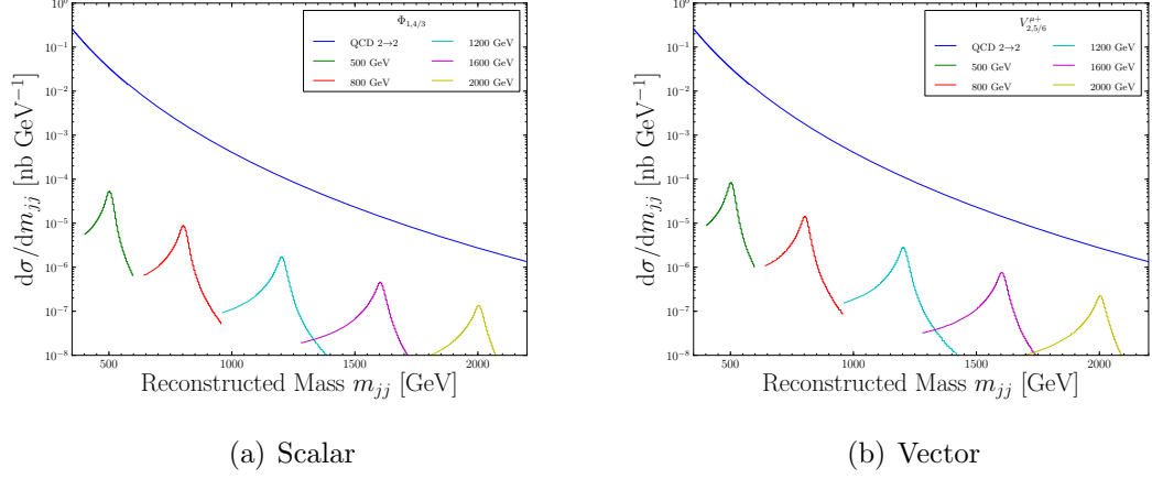
Figure 4.9: The dijet mass spectrum at \sqrt{s} = 7 TeV for 500 GeV, 800 GeV, 1200 GeV, 1600 GeV and 2000 GeV diquark masses with the couplings given in the text.
