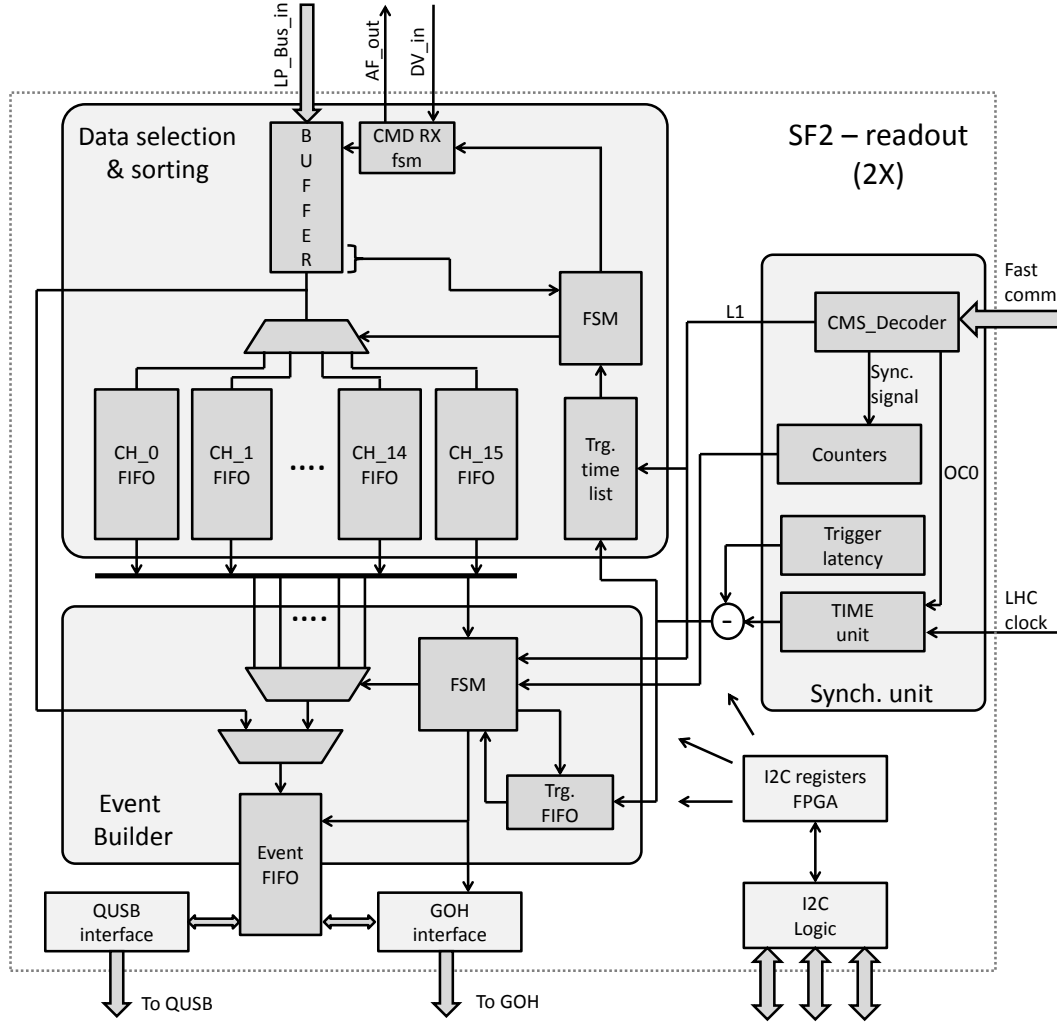
Figure 7.3: Scheme of the firmware readout path. The I 2 C registers are controlled through the control path.
