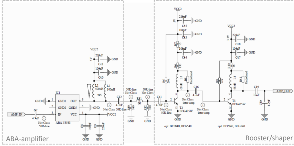
Figure 5.11: Scheme of the amplifier and shaper integrated by TOTEM. Component values may differ from the final one.
