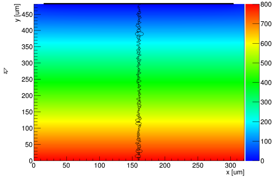
Figure 4.10: Charge release for MIP particle (Landau distribution) in a diamond detector. The applied field is also shown.
