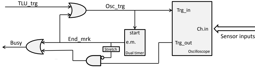
Figure 5.16: Scheme of the TLU/oscilloscope trigger handshake. Additional delay units have been used but not reported. TTL to NIM voltage translators have been used when needed.
