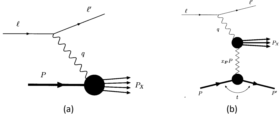
Figure 1.13: Deep inelastic scattering (a) and diffractive deep inelastic scattering (b) diagrams.
