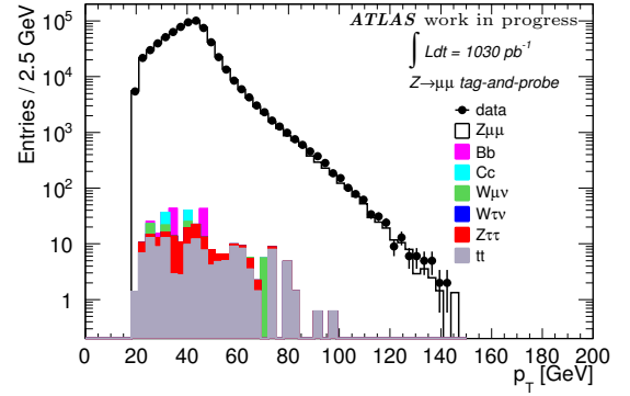
Figure 6.3: Transverse momentum distributions of MS probe muons.
