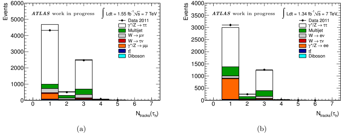
Figure 7.6: Number of tracks of the hadronic \tau decay candidates (a) in the \tau_\mu\tau_h channel and (b) in the \tau_e\tau_h channel.
