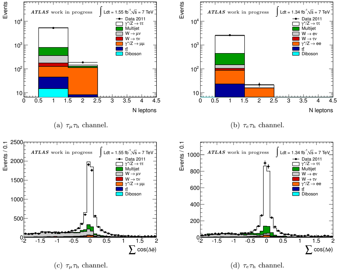
Figure 7.13: Selection variable distributions after all cuts except the one in the variable shown. The shape of the multi-jet background is estimated from the control region obtained by inversion of charge product sign requirement. It is normalized to the signal region expectation (see section 7.6.3).
