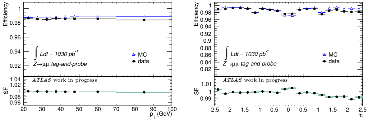
(a) Data and Monte Carlo efficiency as a function of the muon p_T .
