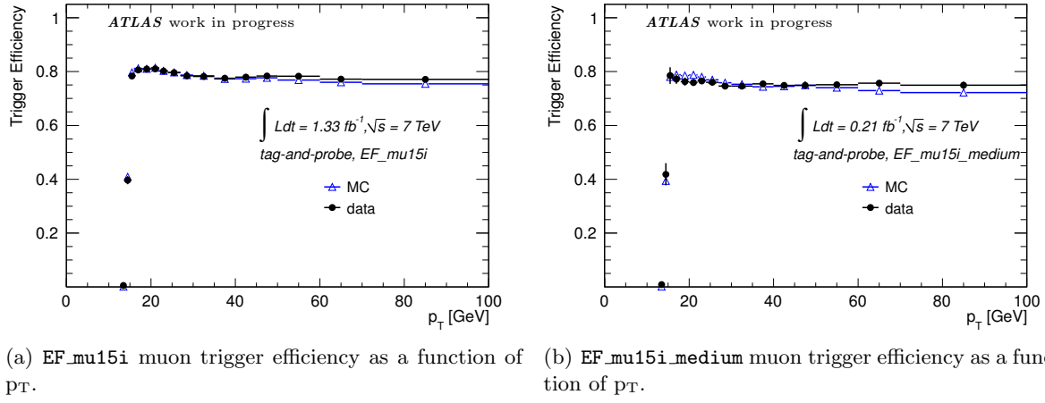
Figure 6.12: Trigger efficiency as a function of the muon transverse momentum for the Monte Carlo simulation (blue triangles) and the data (black dots). The efficiency is determined with respect to reconstructed and isolated muons.
