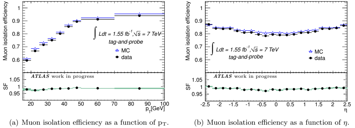
Figure 6.9: Measured isolation efficiencies of reconstructed muons from Monte Carlo simulation (blue triangles) and data (black dots). Muons are isolated in this example if \sum_i p_{T,i} (\Delta R = 0.4) / p_T < 0.03 and \sum_i E_{T,i} (\Delta R = 0.3) / p_T < 0.04 .
