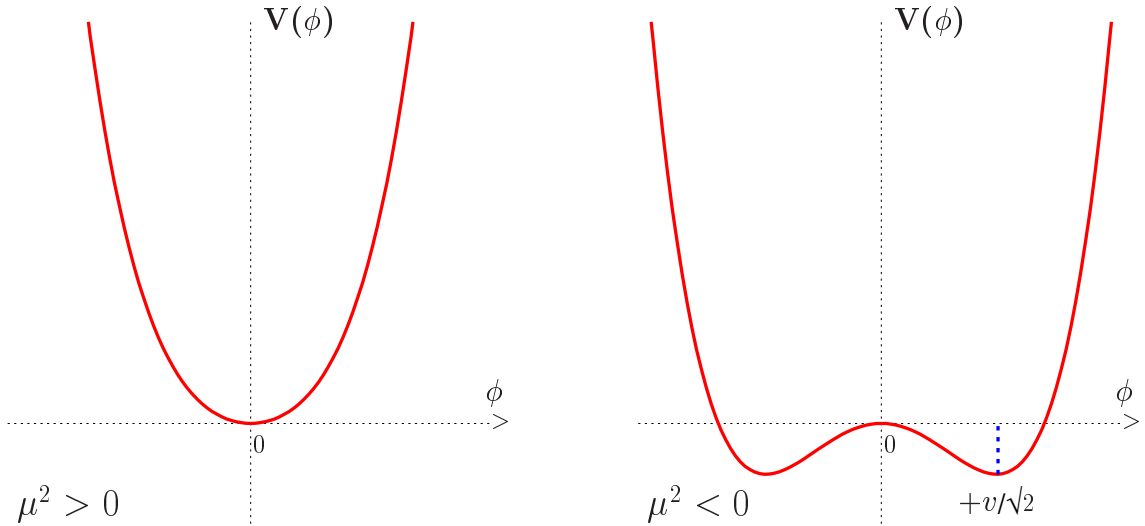
Figure 2.1: The Higgs potential for \mu^2 > 0 (left) and \mu^2 < 0 (right) [9]. In the latter case, the selection of a particular ground state breaks the electroweak gauge symmetry of the Lagrangian.
