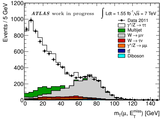
(a) \tau_\mu\tau_h channel.
