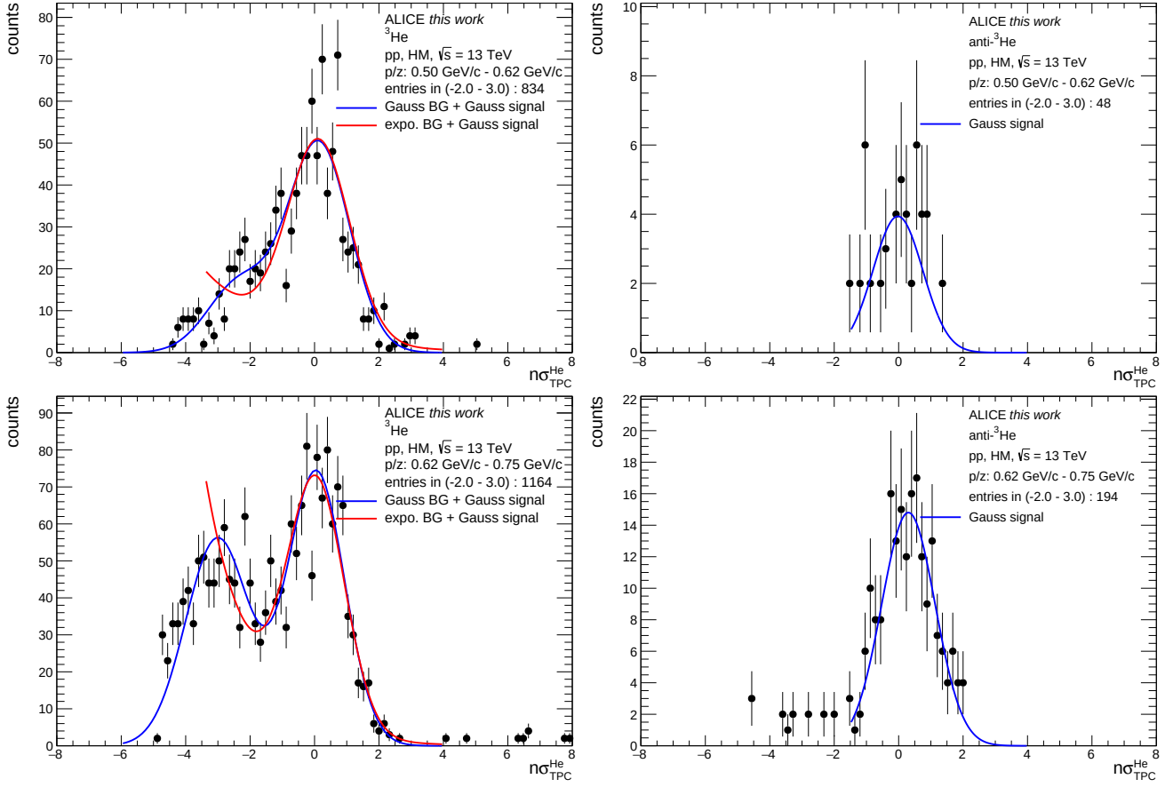
Figure B.4: TPC signal extraction for {}^3\text{He} (left) and anti- {}^3\text{He} (right) for the integrated high multiplicity triggered event class in the 0.5-0.625 GeV/c (top) and 0.625-0.75 GeV/c (bottom) rigidity intervals, with a signal plus background interpolation. The interpolation is not used for anti- {}^3\text{He} .
