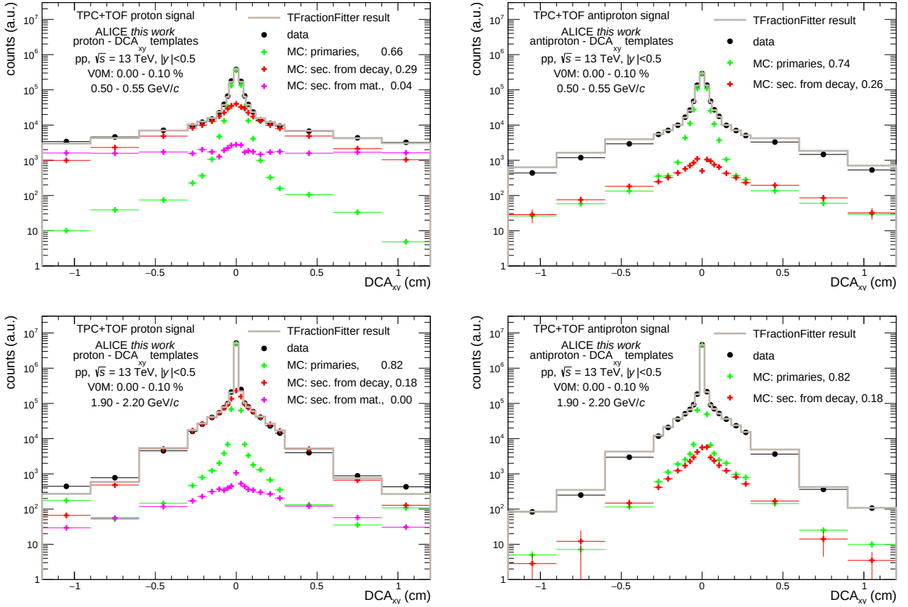
Figure 3.17: DCA_{xy} template fits for protons (left) and antiprotons (right) in the V0M multiplicity class 0-0.1%. The DCA_{xy} bin granularity is 31.
