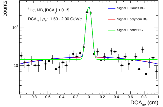
Figure 3.22: DCA_{xy} distribution of ^3\text{He} candidates with a required |DCA_z| < 0.15 cm. The data is interpolated with three different background shapes to estimate the secondary-particle contamination.
