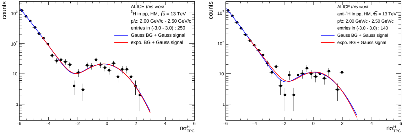
Figure B.7: Expected TPC triton signal after applying a TOF preselection ( |n\sigma_{\text{TOF}}^{3\text{H}}| < 3 ) for the momentum bin 2 < p < 2.5 GeV/c in the high multiplicity triggered event class. The left side shows particle while the right one shows anti-particle.
