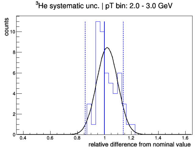
Figure 3.47: The track selection criteria for ^3\text{He} were varied fifty times and the resulting differences from the nominal value are filled into the distribution in the 2 < p_T < 3 GeV/ c range and the integrated MB data sample. The distribution is interpolated with a Gaussian and the width is taken as track selection systematic uncertainty. The dashed lines show the statistical uncertainty in the corresponding p_T bin.
