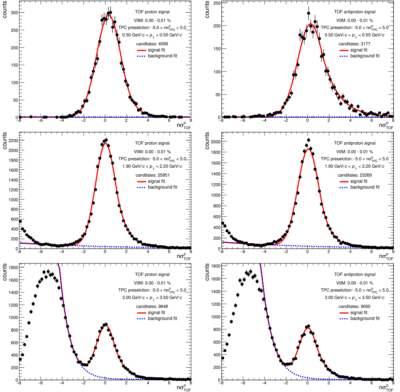
Figure B.1: Proton TOF signal extraction for the integrated multiplicity class ( VOM: 0-0.01\% ). Protons on the left side and antiprotons on the right. The displayed momentum bins are from top to bottom 0.5 \leq p_T < 0.55\ GeV/c , 1.9 \leq p_T < 2.2\ GeV/c , and 3.0 \leq p_T < 3.5\ GeV/c .
