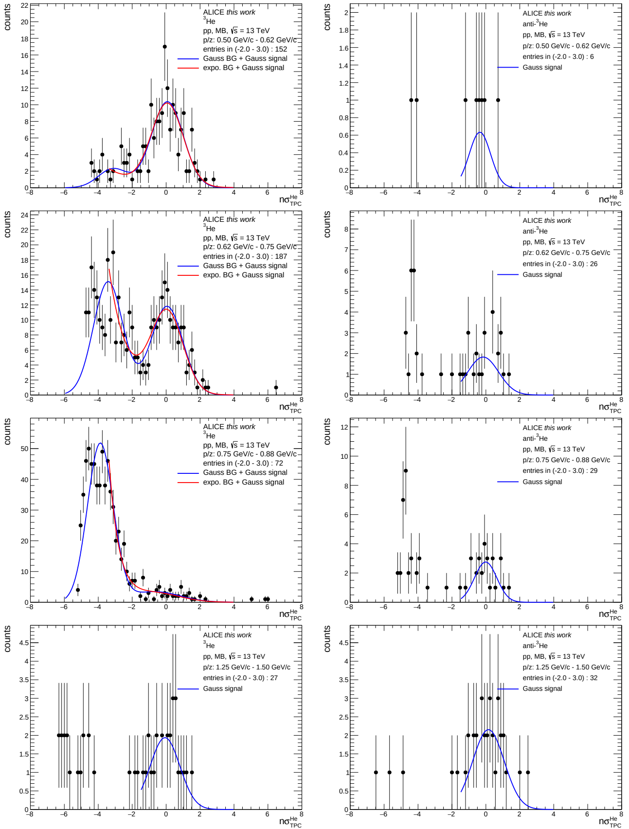
Figure 3.13: TPC signal extraction for {}^3\text{He} (left) and \text{anti-}{}^3\text{He} (right) for the integrated minimum bias event class, with a signal plus background interpolation. The interpolation is not used for \text{anti-}{}^3\text{He} .
