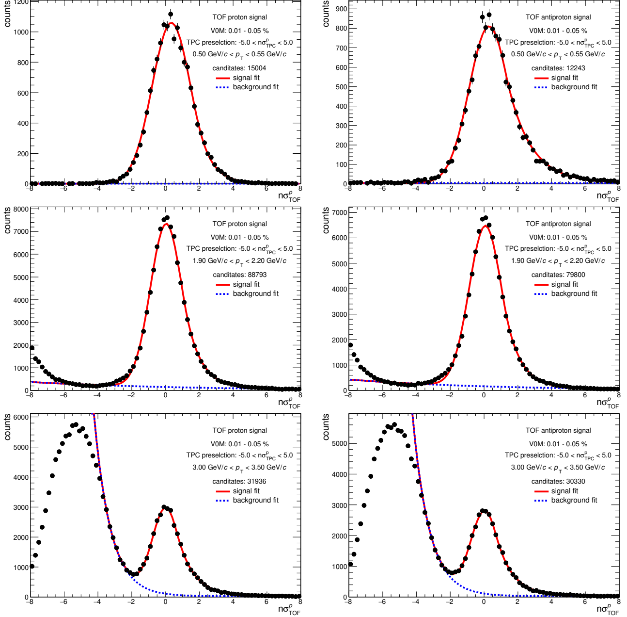
Figure B.2: Proton TOF signal extraction for the integrated multiplicity class (V0M: 0.01-0.05%). Protons on the left side and antiprotons on the right. The displayed momentum bins are from top to bottom 0.5 \leq p_T < 0.55 \text{ GeV}/c , 1.9 \leq p_T < 2.2 \text{ GeV}/c , and 3.0 \leq p_T < 3.5 \text{ GeV}/c .
