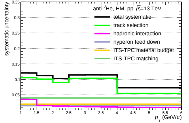
Figure B.12: Total systematic uncertainty with the individual contributions of the \text{anti-}{}^3\text{He} p_T spectra in the HM event class.
