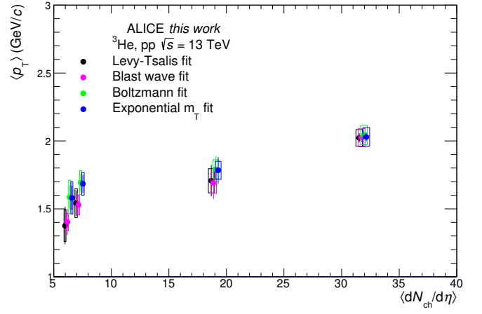
Figure 4.4: Mean p_T of (anti-) 3 He nuclei obtained with the different models for extrapolation. The data points are slightly shifted along the x-axis for better visibility.
