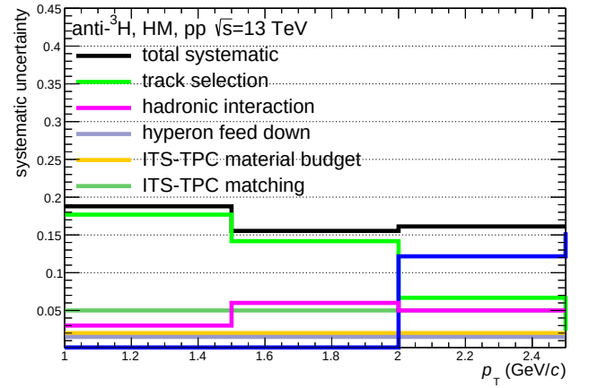
Figure B.14: Total systematic uncertainty with the individual contributions of the \text{anti-}{}^3\text{H} p_T spectra in the HM event class.
