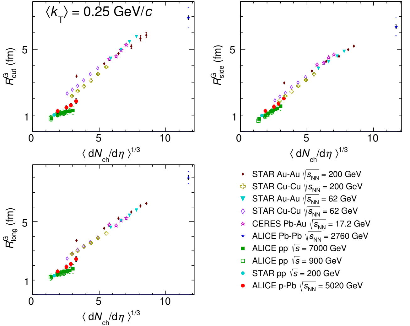
Figure 1.14: Different source radii obtained with femtoscopy techniques, as a function of charged-particle multiplicity density, measured for a wide range of collision systems and center of mass energies. The figure is taken from reference [98].
