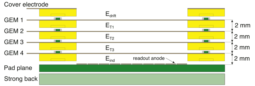
Figure 5.3: Set up of the GEM-based ALICE TPC readout chambers. Each GEM foil is glued onto a 2 mm thick support frame defining the gap between the four different GEM foils. The drift field E_{\text{drift}} , transfer fields E_{T_i} , and induction field E_{\text{ind}} are shown as well [164].
