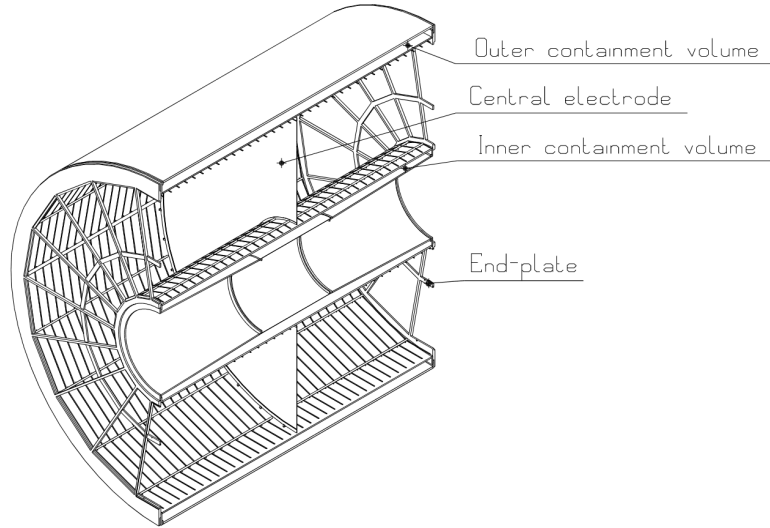
Figure 2.3: Schematic view of the ALICE TPC field cage without readout chambers [121].
