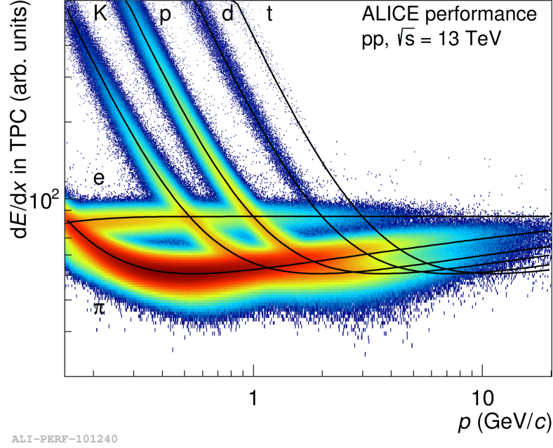
Figure 2.4: Performance plot of the ALICE TPC particle identification capabilities in pp collisions at \sqrt{s} = 13 TeV. The specific energy loss ( dE/dx ) vs. p is shown. The lines indicated the expected signal for the different particle species.
