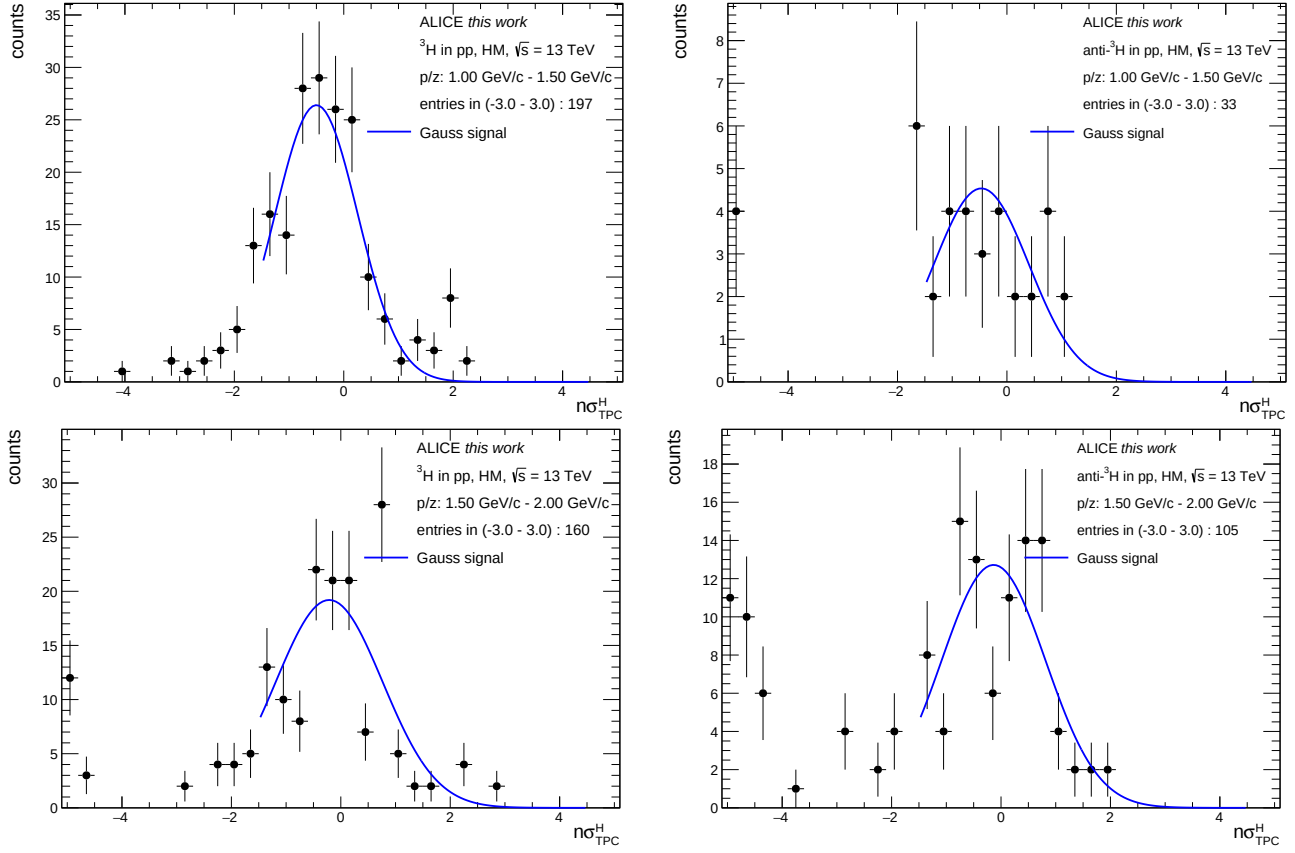
Figure B.6: TPC only signal extraction for triton candidates with low momentum ( p \leq 2 GeV/c) in the high multiplicity triggered event class. The left side shows particle while the right one shows anti-particle.
