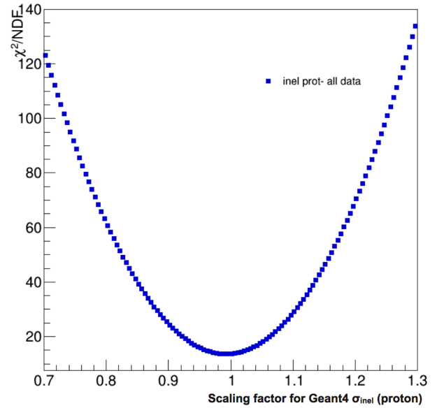
Figure 3.31: The \chi^2/\text{NDF} as a function of the combined fits rescaling factor.
