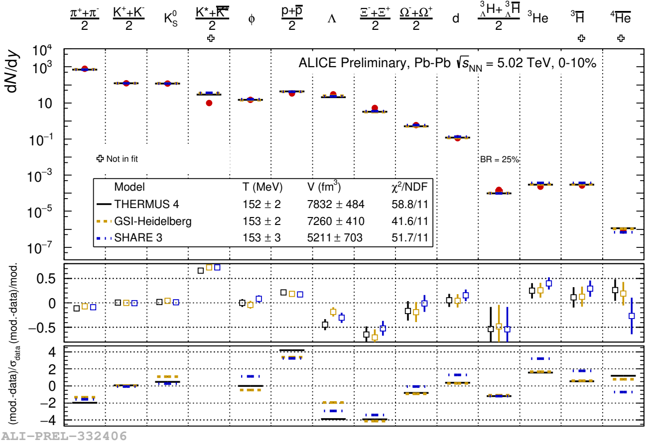
Figure 1.11: Statistical hadronization model fits (THERMUS 4 [84], GSI-Heidelberg [52], SHARE 3 [85]) to integrated particles yields at mid rapidity measured with ALICE in central Pb-Pb collisions. The chemical freeze-out temperatures in all three implementations agree within uncertainties. The middle panel shows the difference between the model and the measurement divided by the model expectation. The lowest panel shows the same difference expressed in terms of uncertainties of the measured ALICE data.
