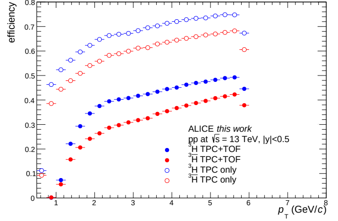
Figure 3.28: (Anti)triton tracking efficiency ( \epsilon ) averaged over all periods in the years 2016, 2017, and 2018. The full symbols represent the efficiency obtained requiring a signal in the TPC and TOF detectors while the open symbols do not require a TOF signal.
