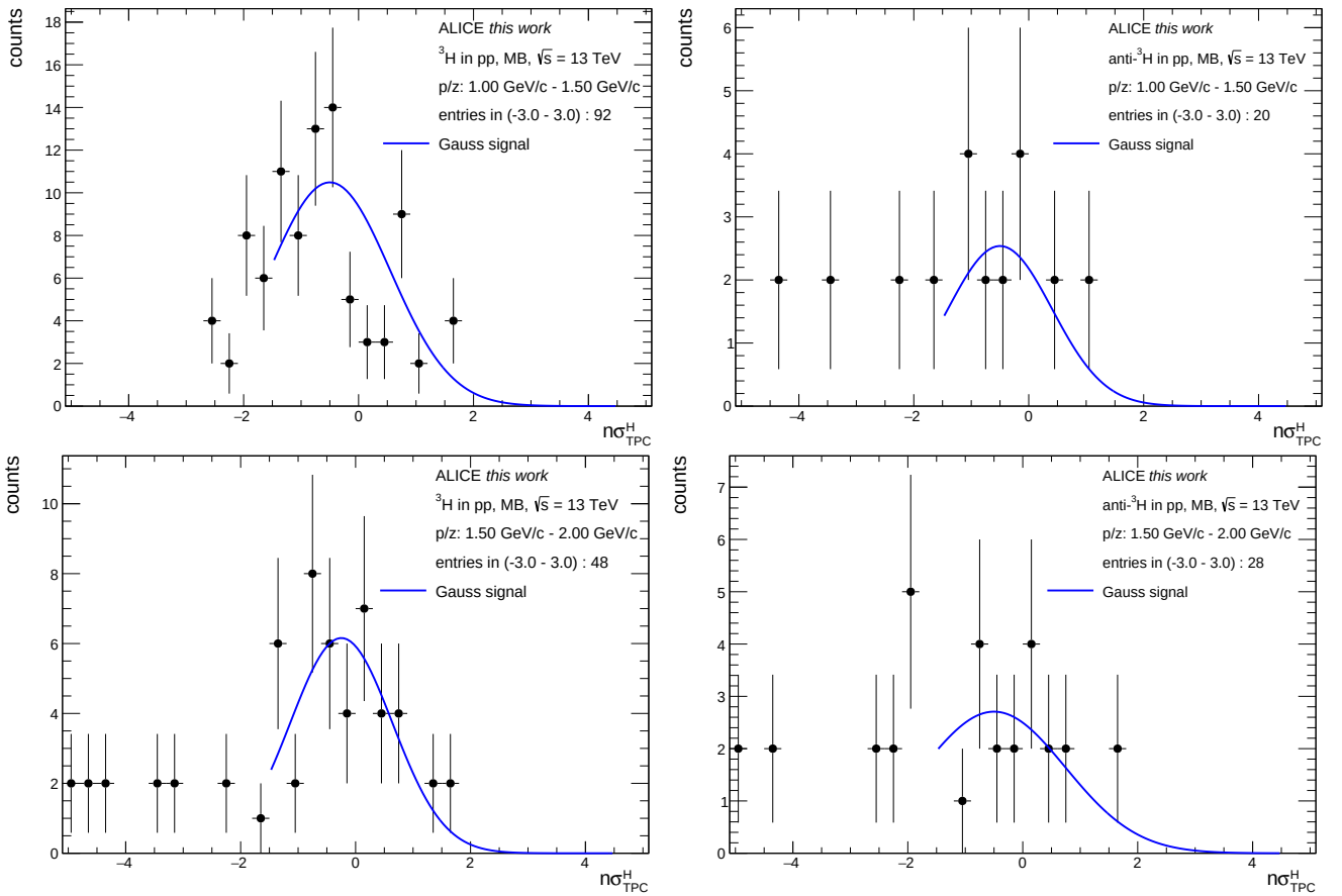
Figure 3.15: TPC-only signal extraction for triton candidates with low momentum ( p \leq 2 GeV/c) in the minimum bias event class. The left side shows particle while the right one shows antiparticle.
