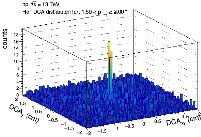
Figure 3.21: The correlation between DCA_{xy} and DCA_z for ^3\text{He} candidates.
