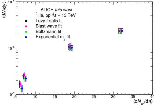
Figure 4.3: Integrated yield of (anti-) 3 He nuclei obtained with the different models for extrapolation. The data points are slightly shifted along the x-axis for better visibility.
