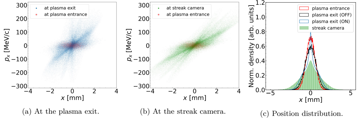
Figure 6.14: Phase space and position distribution of a simulated p^+ bunch with \epsilon_n = 9.5 mm mrad and \sigma_{y,i} = 560\text{ }\mu\text{m} undergoing SSM in a 10 m long plasma or travelling the same distance in a drift space. Parameter set defined in S-Set2 is used.
