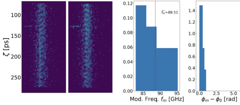
Figure 6.10: From left to right: Time-resolved (y, \zeta) images of micro-bunch trains; histogram of the frequency distribution over eleven events; histogram of the corresponding phase distribution. The RIF is at \simeq -0.75\sigma_t .
