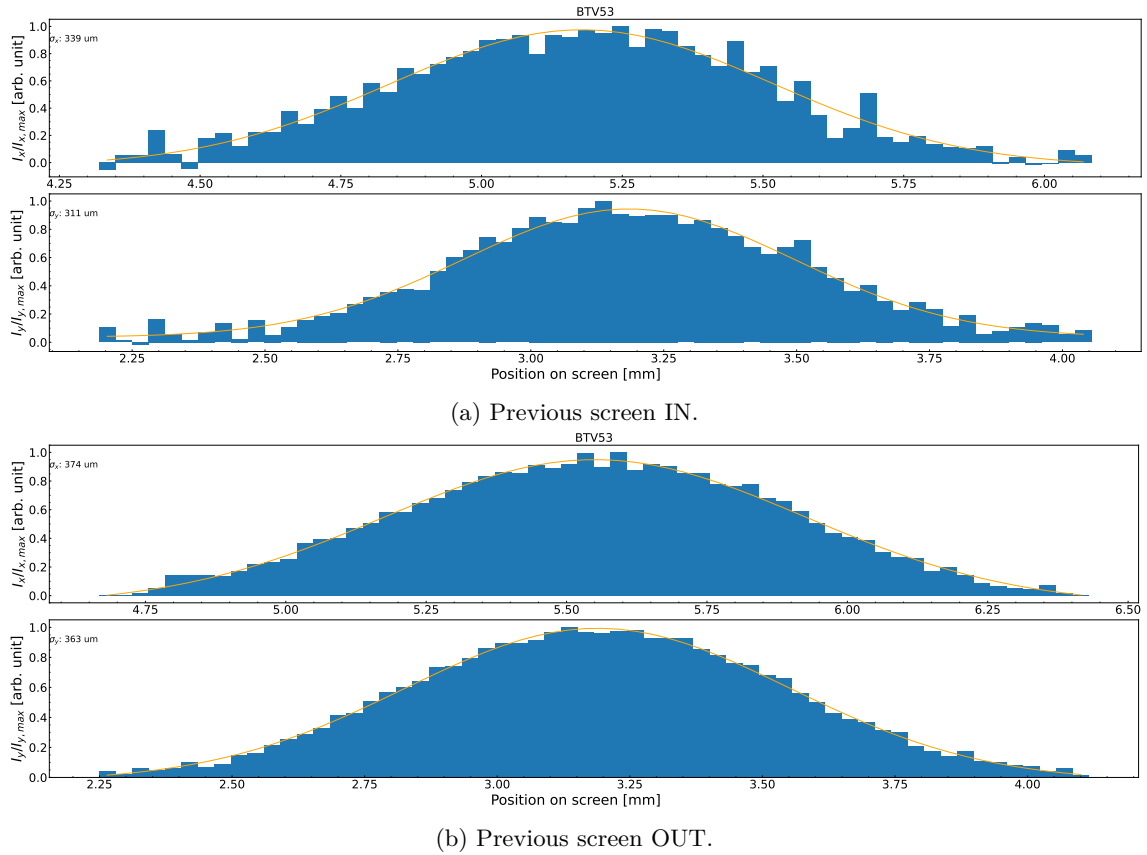
Figure A.1: Example of data quality. Data for a beam size measurement at BTV53. Projections along both transverse axes when the next upstream screen is present (a) or not (b). Sources of noise are secondary particles produced when the beam crosses the previous screen.
