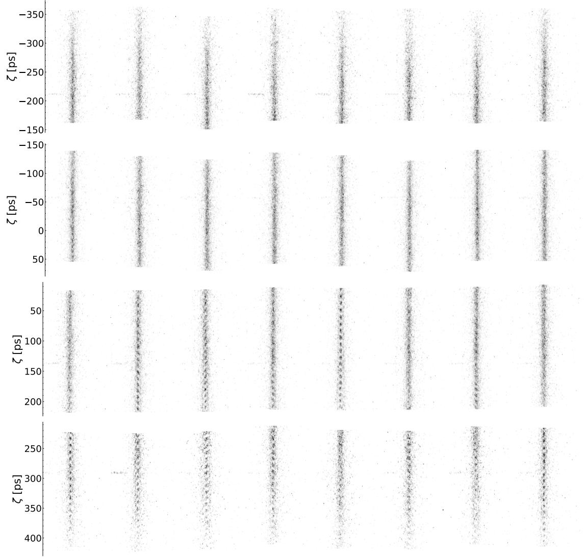
Figure 6.7: Time-resolved (y, \zeta) images of p^+ bunches of \sigma_{y,i} \sim 560 \mu\text{m} transverse size at the iris. The RIF is positioned at -2.6\sigma_t . Horizontal rows present eight individual events. First row: range \sim(-1.6 \text{ to } -0.68)\sigma_t . Second row range \sim(-0.68 \text{ to } 0.23)\sigma_t . Third row: range \sim(0.11 \text{ to } 0.92)\sigma_t . Fourth row: range \sim(1.94 \text{ to } 2.03)\sigma_t . The bunch duration is \sigma_t \sim 219 \text{ ps} . The colour-scale is logarithmic. Note that images along one column are all from different events.
