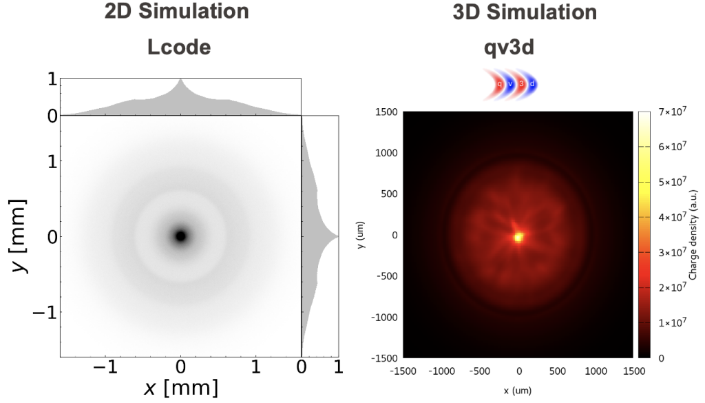
Figure A.6: Additional results after submitting this thesis. Result of a 3D simulation with the code qv3d by Dr John Farmer. Post-processing and parameters space similar to the 2D case. Presented is a beam of \sigma_{\perp,i} = 600 \mu\text{m} with parameters according to S-Set 3 . A spoke like structure appears in the 3D simulations. The outer-end of the spokes show some sort of ring also visible in the 2D simulations.
