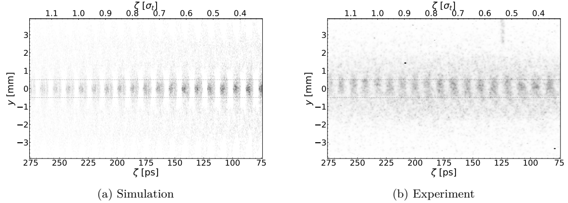
Figure 6.12: Time-resolved (\zeta, y) images of p^+ bunches of \sim 560 \mu\text{m} transverse size at the iris. The RIF is positioned at -0.75\sigma_t . For simulations the S-Set2 parameters are used.
