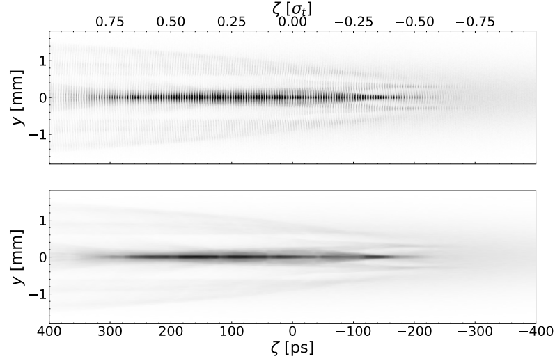
Figure 6.21: Cut through the bunch centre: y\zeta – plane of two different resolutions. The initial transverse beam size is \sigma_{\perp,i} = 600 \mu\text{m} . The parameter set S-Set3 was used.
