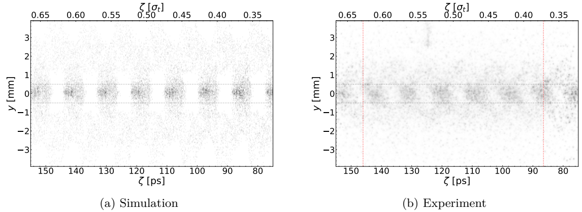
Figure 6.13: Time-resolved images of p^+ bunch of \sim 560 \mu\text{m} transverse size at the iris. The RIF is positioned at -0.75\sigma_t . 80 % image density is indicated by red lines. For simulations the S-Set2 parameters are used.
