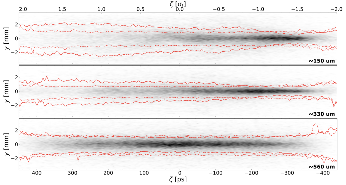
Figure 6.3: Time-resolved (\zeta, y) images of p^+ bunches of beam sizes at iris (top to bottom) of \sim 150 \mu\text{m} , \sim 330 \mu\text{m} and \sim 560 \mu\text{m} . The RIF is positioned at (-2.72 \text{ to } -2.61) \sigma_t . The solid red lines show the 80 % bunch envelope of a plasma ON and the red dashed lines the 80 % bunch envelope of a plasma OFF bunch. The bunch spread in the front is non-physical and due to a low signal-to-noise ratio. Each image has its own colour-scale.
