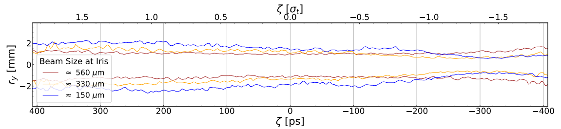
Figure 6.4: Condensed 80 % bunch envelope results of Fig. 6.3. The bunch centre is at \zeta = 0 , the RIF is (-2.72 \text{ to } -2.61) \sigma_t ahead the centre.
