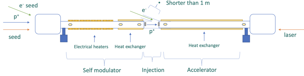
Figure 1.2: Schematic representation of experimental setup for Run 2c. Image taken from [34].
