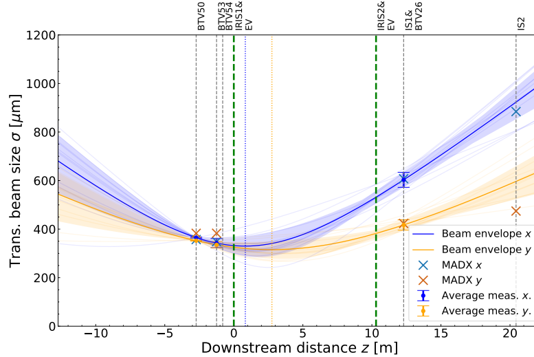
Figure 2.4: Transverse envelope of a beam with target \sigma_{x,y} = 330\text{ }\mu\text{m} at the iris. See page 23 for further explanations.
