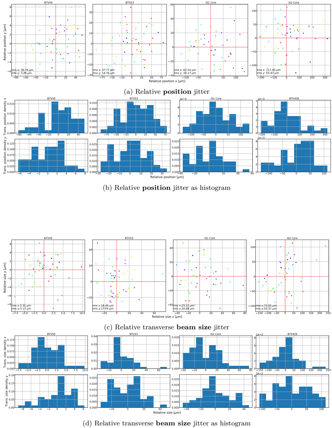
Figure 2.3: Summarised p^+ beam event-to-event jitter results of a beam with target transverse beam size at the plasma entrance of 200\mu\text{m} . The origin is found by taking the average (red cross) of the absolute position or transverse size of the events. The points are sequentially rainbow colour-coded (red to violet), i.e., points of similar colour were time-wise close to each other.
