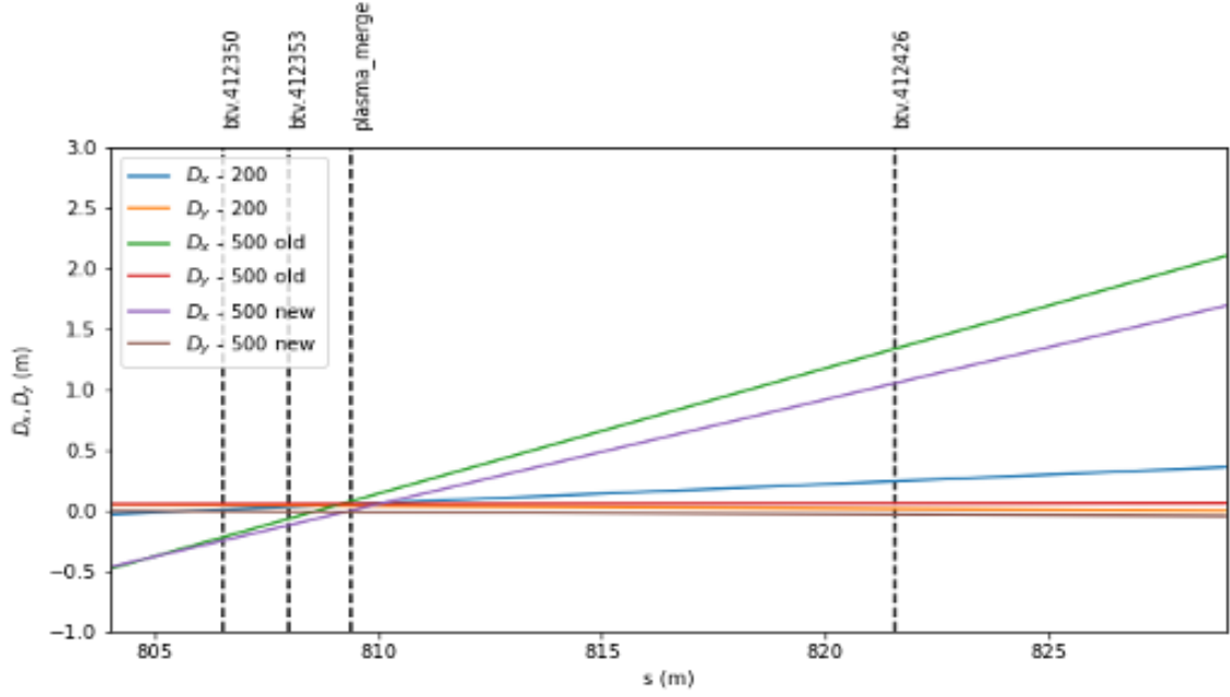
Figure A.4: Dispersion along the x - and y -axis for the baseline design beam ( 200 ), for the 330\text{ }\mu\text{m} large beam ( 500\text{ old} ) and the largest beam with 560\text{ }\mu\text{m} transverse size ( 500\text{ new} ). Figure provided by Dr Vittorio Bencini in private communication, 3 rd Aug 2022.
