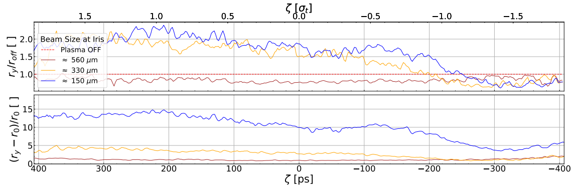
Figure 6.5: Top plot: bunch envelope dynamically normalised to the time-slice corresponding bunch envelope of the plasma OFF bunch. For all beam sizes \sigma_{y,i} , r_y/r_{off} = 1 correspond to the relative extent of a plasma OFF bunch. Bottom plot: bunch envelope normalised to the beam size \sigma_{y,i} at the plasma entrance (iris).
