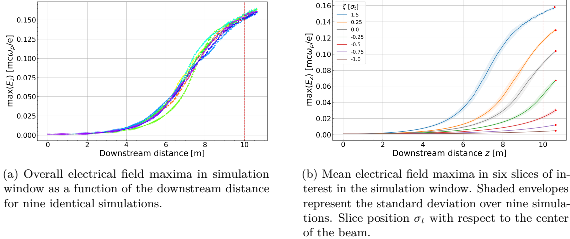
Figure A.5: Extended reproducibility study for a S-Set 2 beam with 700\text{ }\mu\text{m} transverse beam size at iris and number of macro-particles N = 1 \times 10^8 .
