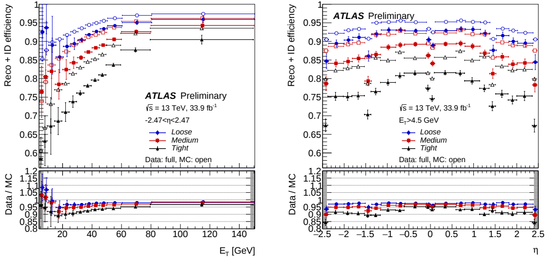
Figure 4.1.: Electron reconstruction and identification efficiencies in data and MC as a function of transverse energy E_T (left) and pseudo-rapidity \eta (right) of the electron. The uncertainty displayed includes both statistical and systematic uncertainties [143].
