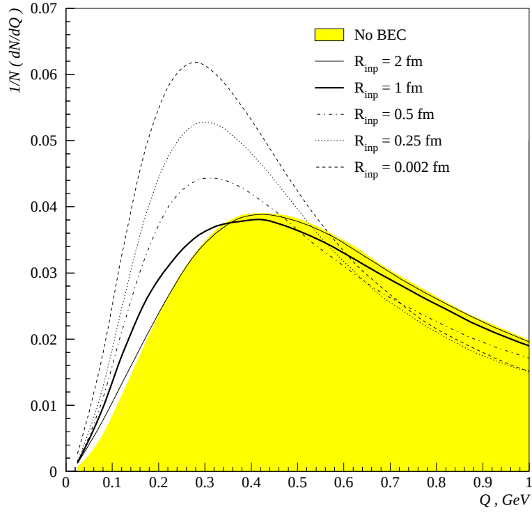
Figure 4.7: Distribution of Q as a function of the input source radii R_{\text{inp}} . The shaded area shows this distribution in absence of BEC.
