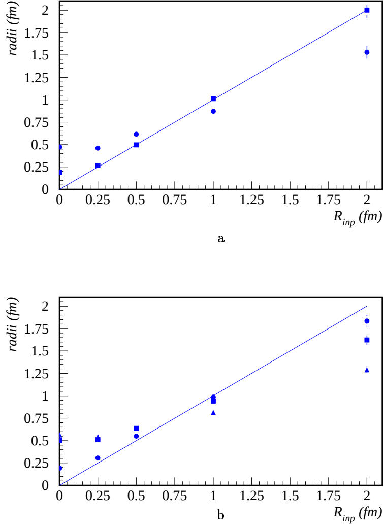
Figure 4.8: Components of the correlation width as a function of the input source radii R_{inp} : a) R_{\parallel} (■), R_{\perp} (●) and b) R_{t,out} (▲), R_{t,side} (■), R_{long} (●).
