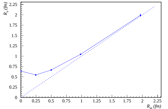
Fig. 6. Fitted values of output radii R_o for different input radii R_{in}
