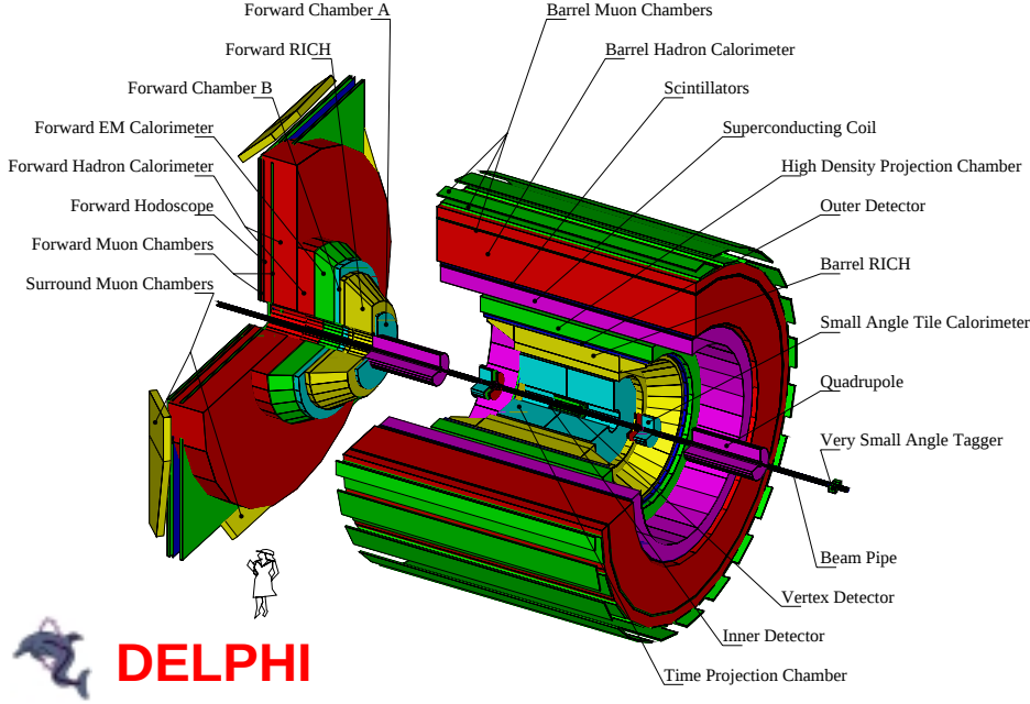
Figure 2.2: DELPHI detector
