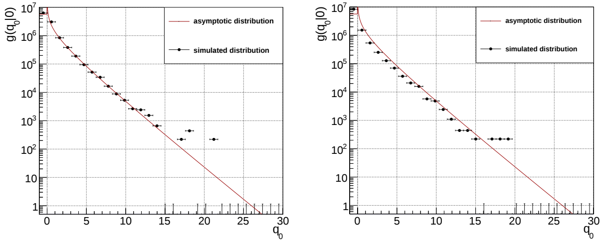
(a) PDF of q_0 for the same setting as in figure (3.3(a)), (b) PDF of q_0 obtained by a simulation that avoided the simulated with Gaussians replacing the Poisson terms. fit process.
