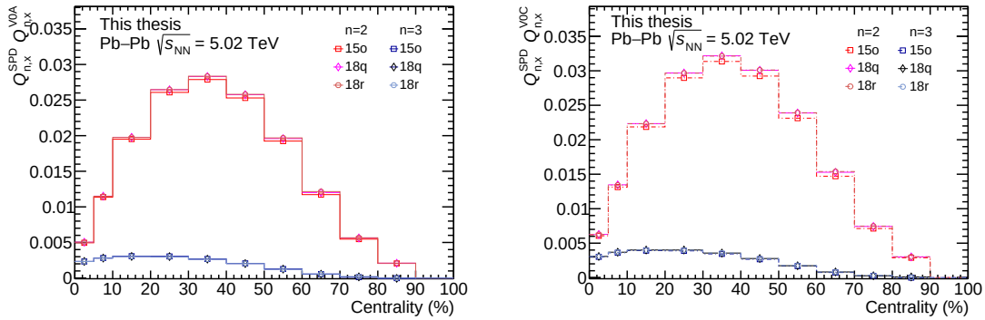
Figure 3.14: Raw Q_{n,x}^{\text{SPD}} Q_{n,x}^{\text{V0A}} and Q_{n,x}^{\text{SPD}} Q_{n,x}^{\text{V0C}} distributions as function of centrality, for the second and third harmonics ( n = 2, 3 ).
