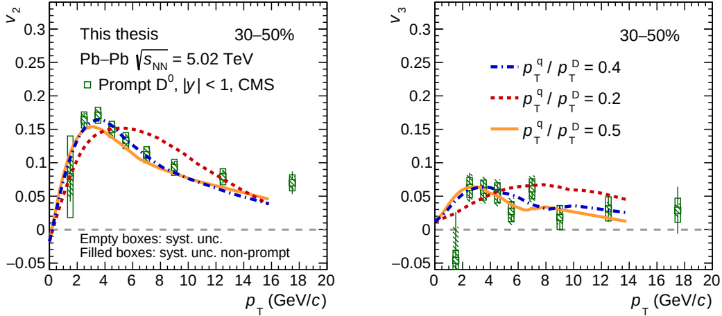
Figure 5.28: Scaled D meson v_2 (left) and v_3 (right) distribution as a function of p_T , constructed from \pi^\pm and J/\psi v_n , for the 30–50% centrality interval.
