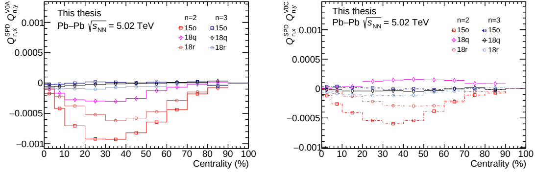
Figure 3.15: Raw Q_{n,x}^{\text{SPD}} Q_{n,y}^{\text{V0A}} and Q_{n,x}^{\text{SPD}} Q_{n,y}^{\text{V0C}} distributions as function of centrality, for the second and third harmonics ( n = 2, 3 ).
