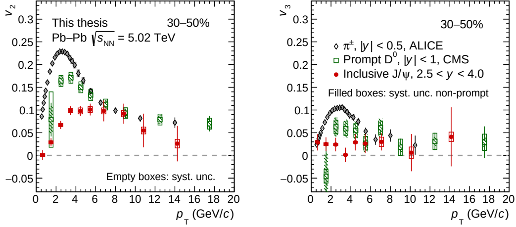
Figure 5.5: Comparison of J/\psi v_2 and v_3 to \pi^\pm and prompt D^0 (published data), as a function of p_T for the 30–50% centrality interval.
