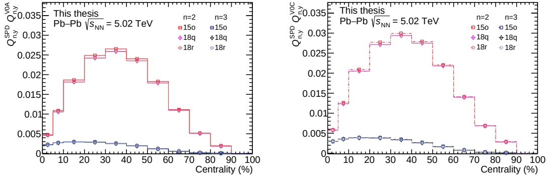
Figure 3.16: Raw Q_{n,y}^{\text{SPD}} Q_{n,y}^{\text{V0A}} and Q_{n,y}^{\text{SPD}} Q_{n,y}^{\text{V0C}} distributions as function of centrality, for the second and third harmonics ( n = 2, 3 ).
