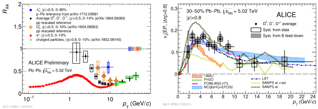
Figure 1.21: Left: R_{AA}(p_T) for \pi^\pm , D mesons, \Lambda_c^+ , and high- p_T charged particles. Right: v_2(p_T) of D mesons measured in Pb–Pb collision. Figures taken from [67]
