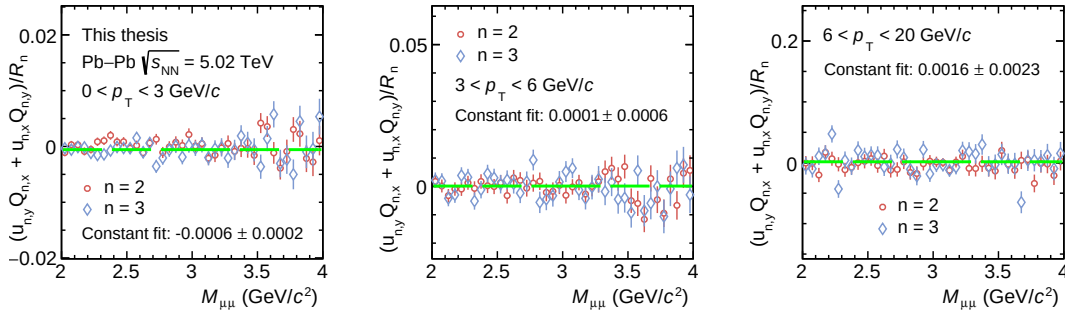
Figure 4.31: M_{\mu\mu} dependence of the cross-term products \mathbf{u}_{n,x} and \mathbf{Q}_{n,y} (using SPD as reference flow detector) for different p_T ranges, in the J/\psi mass region.
