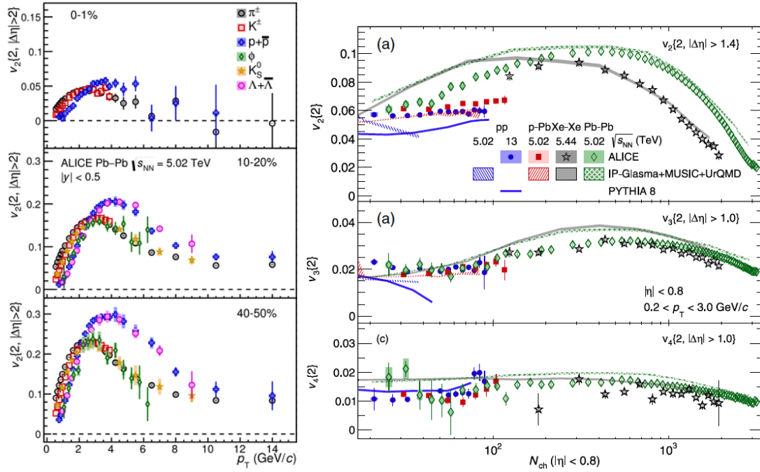
Figure 1.12: Left: p_T -differential v_2 of identified particles in Pb–Pb collisions for various centrality classes. Right: Anisotropic flow measurements ( v_2 , v_3 and v_4 ) of charged particles in different collision systems (p–p, p–Pb, Pb–Pb, and Xe–Xe) as a function of the multiplicity N_{ch} (number of charged particles produced per event). Figures taken from [34] and [35], respectively.
