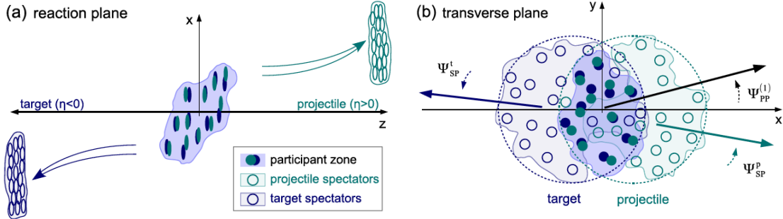
Figure 3.1: Sketch of a non-central heavy-ion collision. \Psi_{\text{RP}} is corresponding to the x axis in (b). Figure taken from [123].
