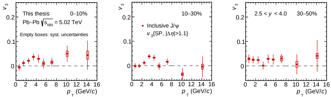
Figure 5.2: p_T -differential J/\psi v_3 for different centrality ranges. Empty boxes are the uncorrelated uncertainties, while the error bars show the statistical uncertainties.
