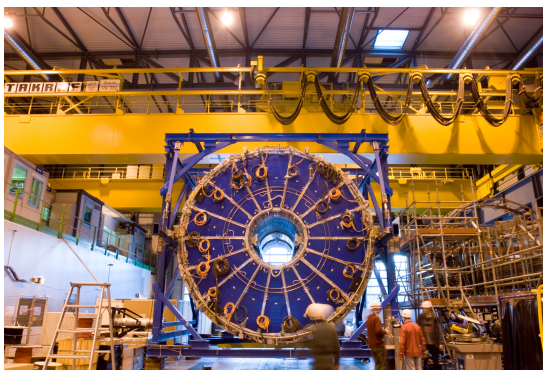
Figure 2.4: TPC installations and its schematics (Figures from [99, 100]).
