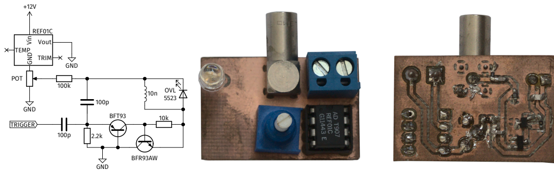
Figure 11.4: Schematic for the first prototype of a LED driver with adjustable bias voltage and the fabricated board.
