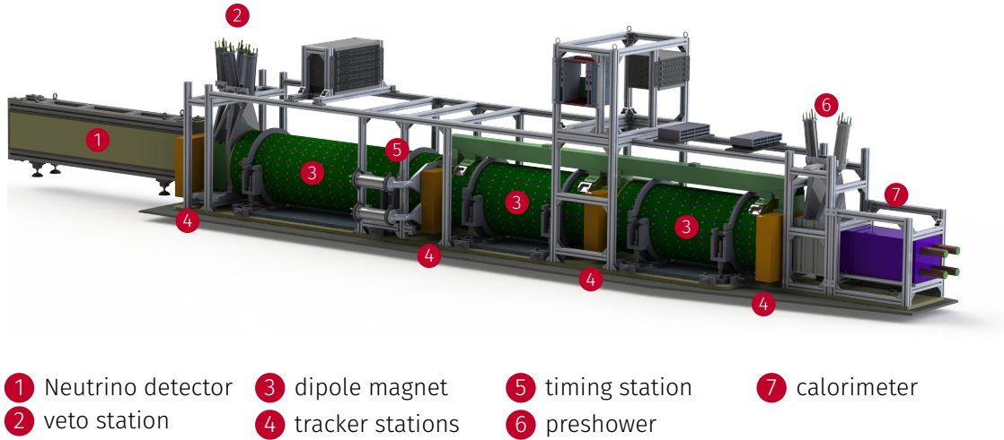
Figure 8.1: Computer rendering of the FASER detector showing all sub-detectors with the front of the detector on the left. For better visibility the cables are hidden in the render.
