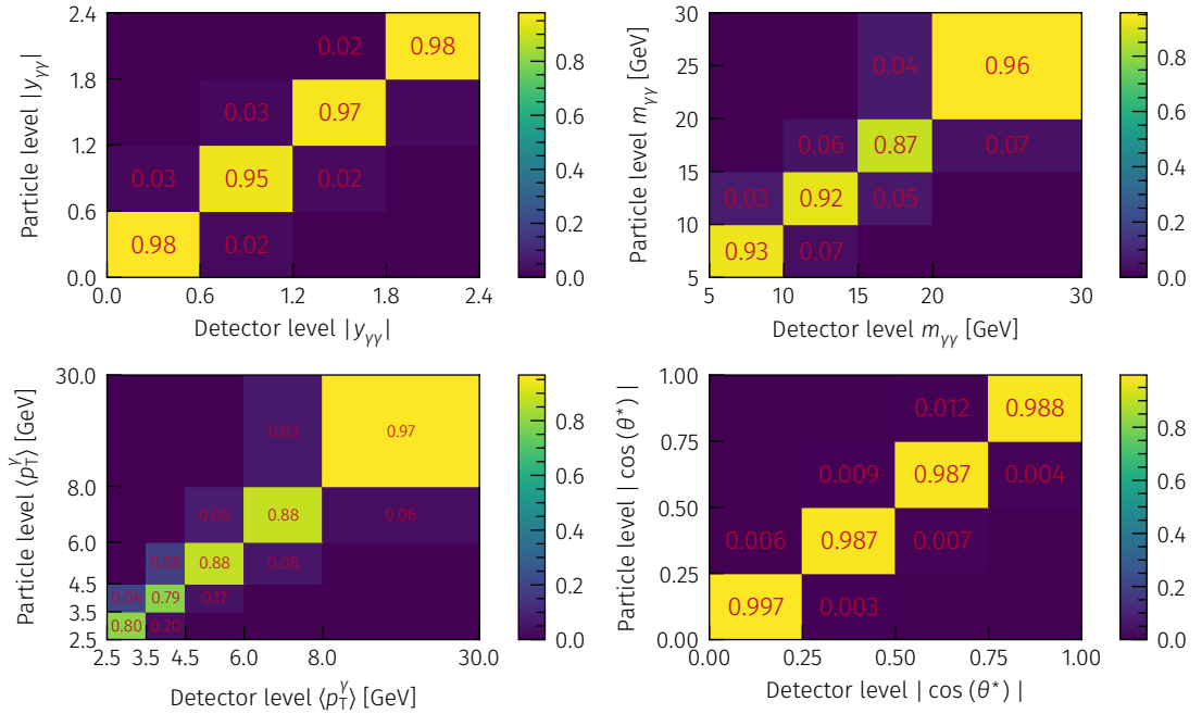
Figure 6.23: Detector response matrices as a function of di-photon rapidity (upper left), di-photon invariant mass (upper right), average photon transverse momentum (lower left) and |\cos \theta^*| (lower right). The numbers represent the corresponding bin values.
