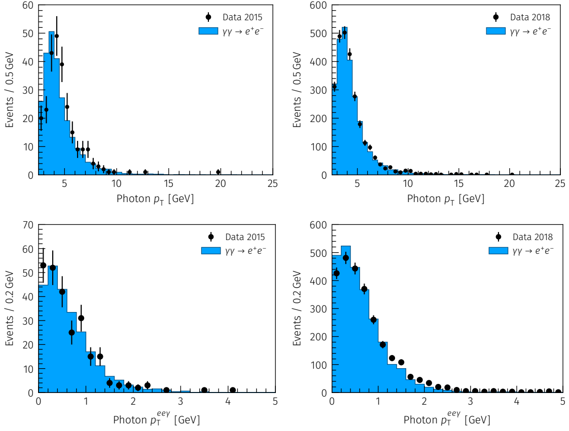
Figure 6.4: Transverse momentum of the hard-bremsstrahlung photons (top) and of the electron, track and photon system (bottom) for the 2015 (left) and 2018 (right) data taking periods compared to simulated events.
