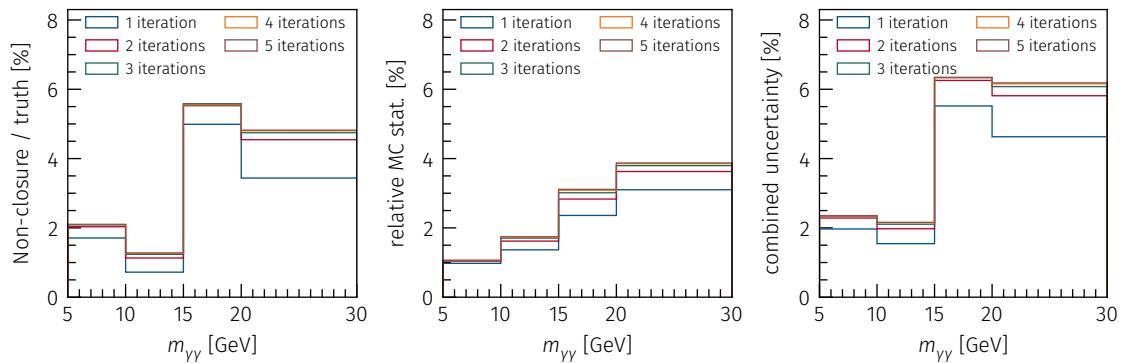
Figure 6.24: Relative non-closure, statistical and combined uncertainty from the MC non-closure test for the di-photon invariant mass for different numbers of iterations.
