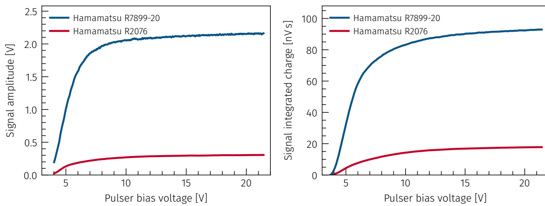
Figure B.1: Measured signal amplitude (left) and integrated charge (right) for both PMTs at different pulser bias voltages.
