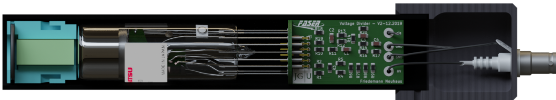
Figure 10.5: Rendering of the readout assembly for the calorimeter. The tube and the end-plug are cut open to allow visibility of all components. The components from left to right are: the filter holder (light blue) with both the filter (black) and the light mixer (light green), the photomultiplier connected to the voltage divider via the adapter PCB and the end-plug with the electrical connections.
