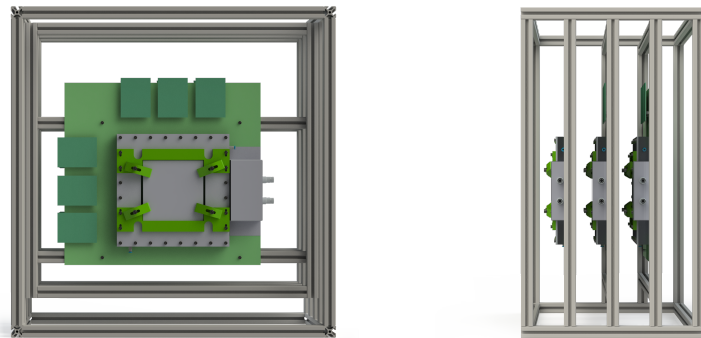
Figure 12.1: Rendering of the preshower prototype used for the test beam as seen from the front (left) and the side (right). The 3D-printed holder and clamps for the absorber plates are shown in green in the front view.
