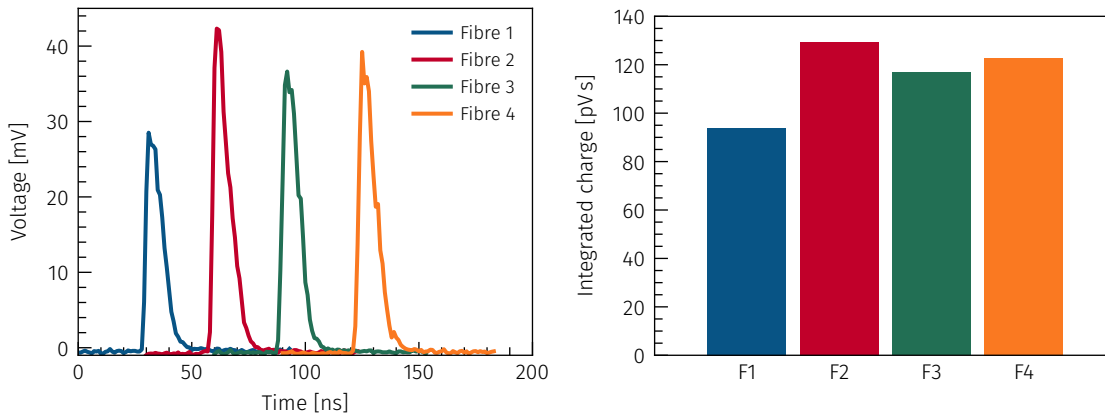
Figure 11.15: Measured waveforms (left) and integrated charges (right) for each fibre in the same PMT one at a time. The waveforms are shifted in time to fit them in a common plot.
