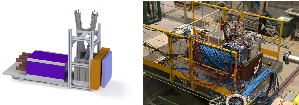
Figure 11.17: Rendering (left) and photograph (right) of the detector setup used for the combined calorimeter and tracker test beam.
