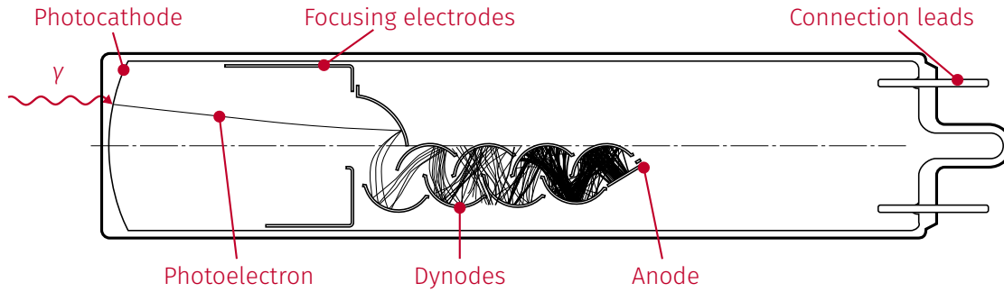
Figure 10.2: Schematic drawing showing the main components and the working principle of a photomultiplier. The electrical connections from the base to the components are left out for clarity (based on a graphic from [131]).
