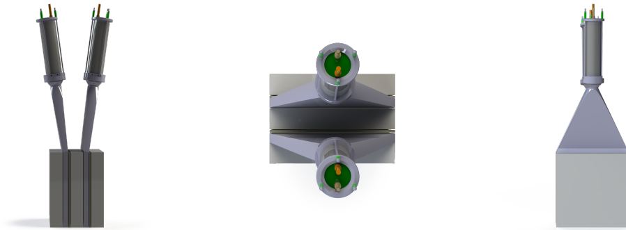
Figure 8.4: Rendering of the preshower station assembly from different views without any of the support structure. It shows the two scintillator plates with light guides and PMTs, the graphite blocks (light grey) and the tungsten plates (dark grey).
