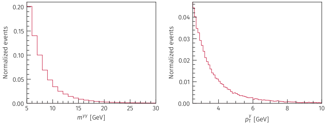
Figure 6.2: Normalized particle level distribution from MC simulation for the di-photon invariant mass m_{\gamma\gamma} (left) and the single photon transverse momentum p_{T,\gamma}^Y (right) without any fiducial selection except for cuts applied on generator level.
