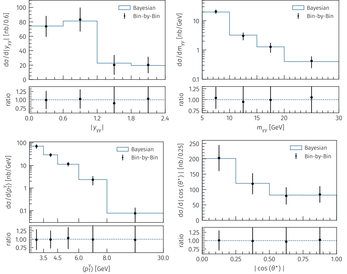
Figure 6.27: Comparison of the differential cross-sections as a function of absolute di-photon rapidity (upper left), di-photon invariant mass (upper right), average photon transverse momentum (lower left) and absolute di-photon |\cos \theta^*| (lower right) as determined by Bayesian (line) and bin-by-bin (points) unfolding. The ratio in the bottom of each plot shows the ratio of the values for bin-by-bin over Bayesian. In this comparison only statistical uncertainties are shown. It should be noted, that the statistical uncertainties are highly correlated.
