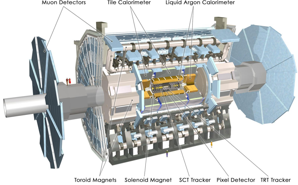
FIG. 13: Computer generated image of the ATLAS detector layout identifying the sub-detector components 61 .
