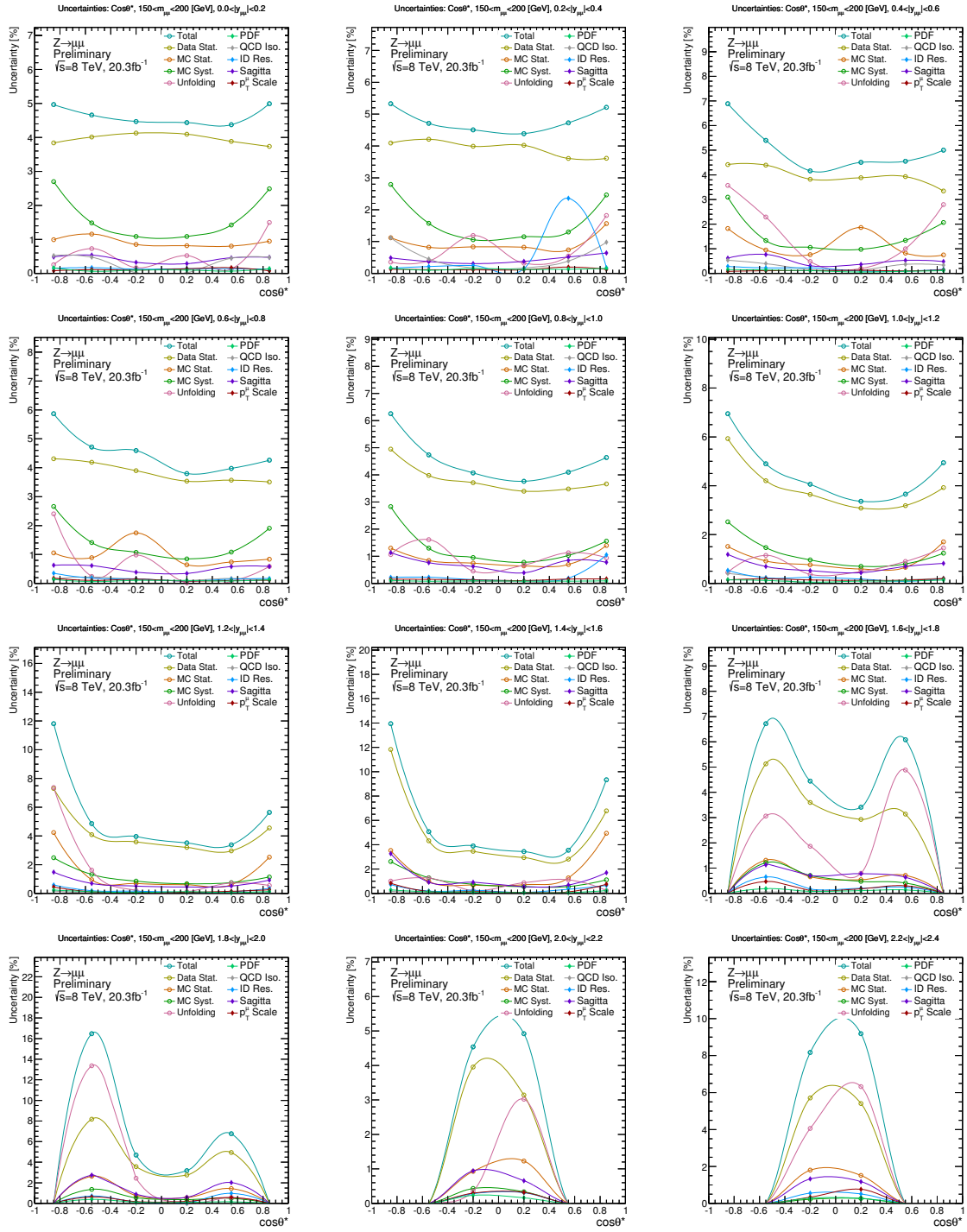
FIG. 66: Largest sources of uncertainty across each rapidity bin within the 150 < m_{\ell\ell} < 200 GeV mass regime.
