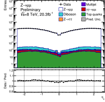
(e) Muon \eta_\mu for |y_{\mu\mu}| > 1.0 and 80 < m_{\mu\mu} < 91 GeV.
