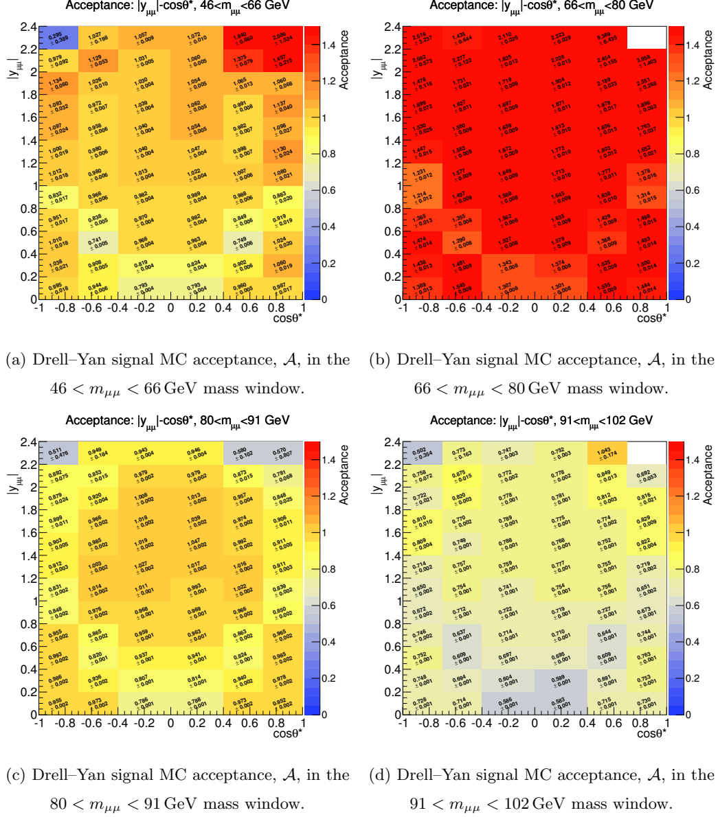
FIG. 29: Two dimensional ( |y_{\mu\mu}|, \cos\theta^* ) plots of the Drell-Yan signal acceptance in the first four invariant mass windows of the measurement. Uncertainties on the values show statistical uncertainties only.
