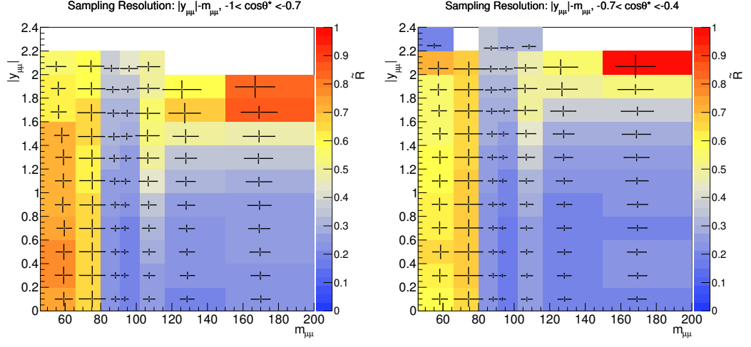
(a) Drell-Yan signal MC sampling resolution in the -1.0 < \cos \theta^* < -0.7 region. (b) Drell-Yan signal MC sampling resolution in the -0.7 < \cos \theta^* < -0.4 region.
