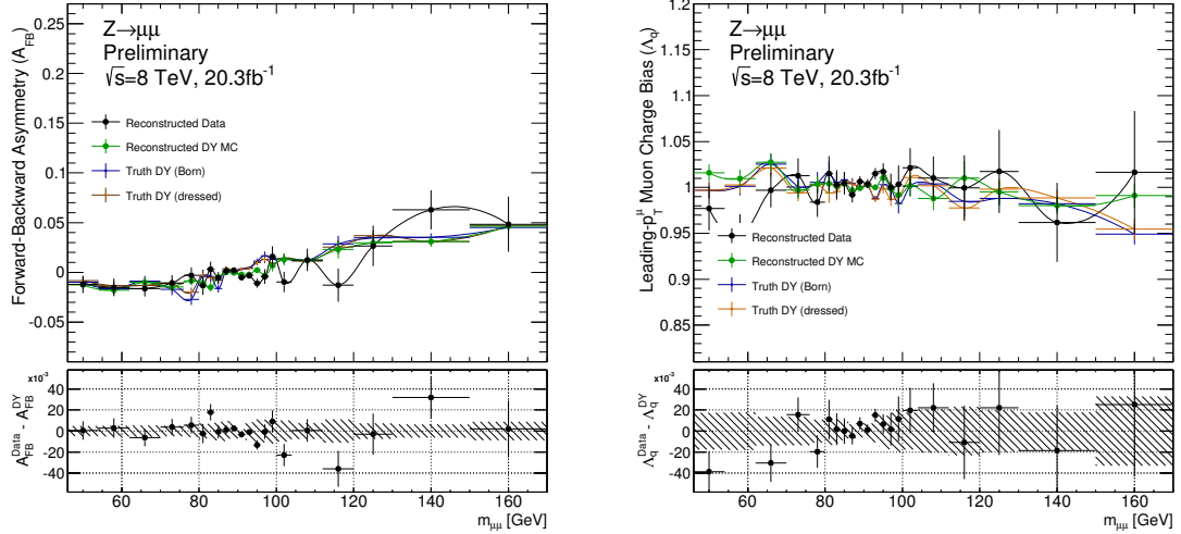
(c) A_{FB} distributions, in the -\eta barrel hemisphere, -1.05 < \eta < 0.0 , using inner detector (ID) sagitta bias corrected p_T^\mu .
