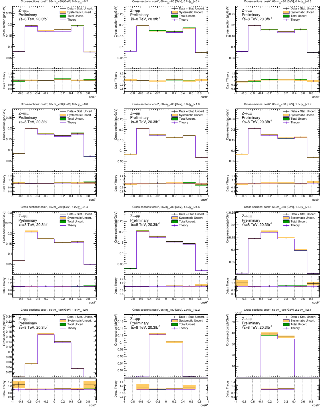
FIG. 75: Cross-section central values and uncertainty bands across each rapidity bin within the 66 < m_{ll} < 80 GeV mass regime unfolded to the Born truth-level with one Bayesian iteration. Theory predictions are taken from powheg-pythia8 Drell-Yan MC. The luminosity uncertainty of 1.9% is not included.
