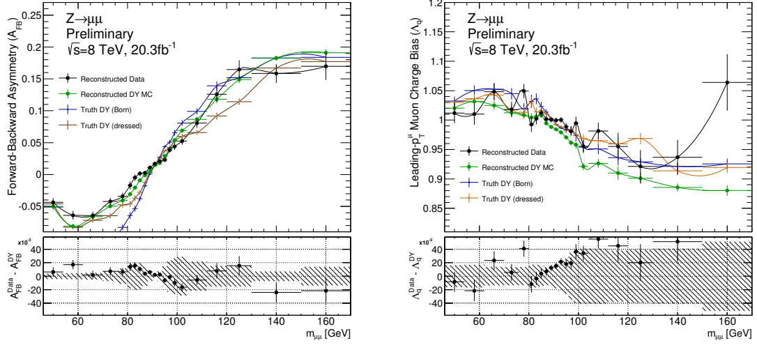
(a) A_{FB} distributions, in the -\eta hemisphere end-cap, -2.4 < \eta < -1.05 , using inner detector (ID) sagitta bias corrected p_T^\mu .
