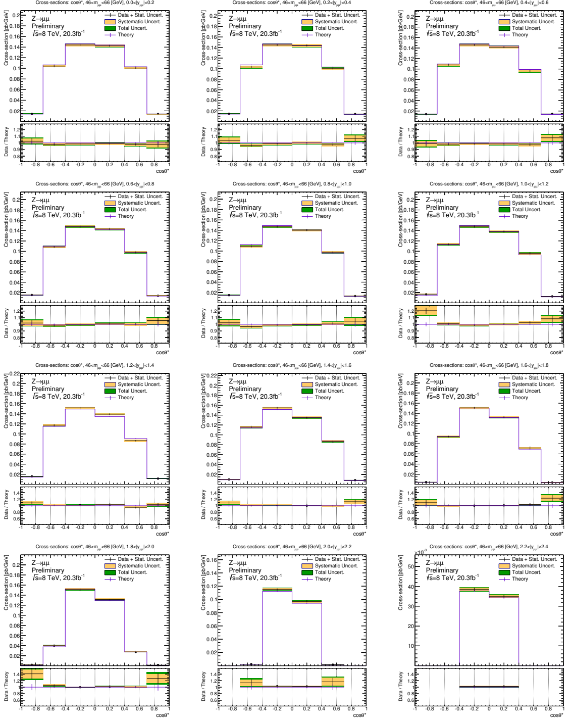
FIG. 74: Cross-section central values and uncertainty bands across each rapidity bin within the 46 < m_{\mu\mu} < 66 GeV mass regime unfolded to the Born truth-level with one Bayesian iteration. Theory predictions are taken from powheg-pythia8 Drell-Yan MC. The luminosity uncertainty of 1.9% is not included.
