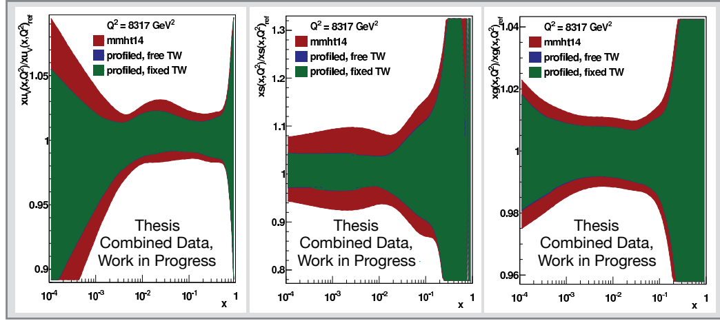
FIG. 90: Uncertainty bands for different PDF components at Q^2 = m_Z^2 = 8317 \text{ GeV}^2 as a function of x . The displayed uncertainty bands are MMHT2014nnlo (outer red band), profiled MMHT2014nnlo with free \sin^2 \theta_W^{\text{eff.}} (blue middle band), and profiled MMHT2014nnlo with fixed \sin^2 \theta_W^{\text{eff.}} (inner green band). The PDF components (left to right) are: xu_v ( u -valence); xs (strange); xg (gluon);
