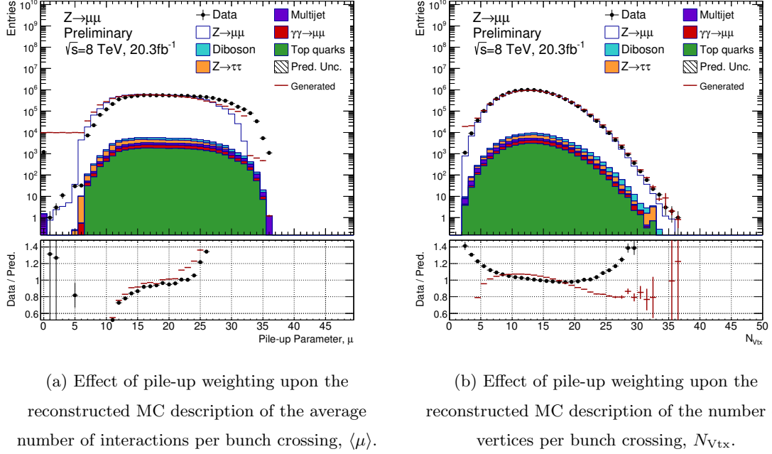
FIG. 37: Reconstruction effects of the pile-up reweighting correction and global \langle\mu\rangle scaling applied at the truth-level to MC simulation. Reconstructed MC and data are shown after applying the full event selection criteria. The uncorrected MC is given by the red line while the corrected is given by the stacked MC histograms and data points are in black. Histogram error bars in the figures include statistical uncertainties only. The bottom panels show the agreements between data and MC with uncorrected and corrected MC.
