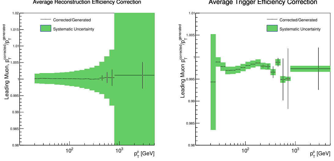
(a) The average leading-muon reconstruction efficiency correction as a function of leading-muon transverse momentum.
