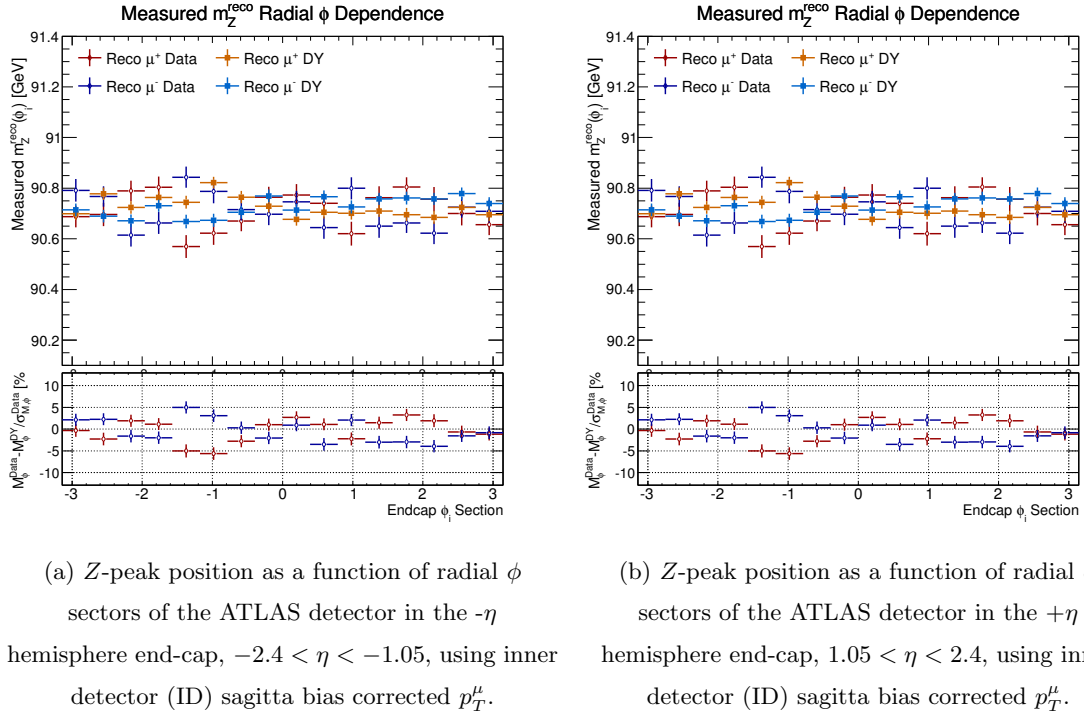
FIG. 47: The leading- p_T^\mu radial \phi dependence of the Z -peak position reconstructed in the ATLAS ID end-caps. The reconstructed DY signal MC prediction ( \mu^+ leading-muons in orange, \mu^- leading-muons in light-blue) is shown along with the measured data ( \mu^+ leading-muons in red, \mu^- leading-muons in dark-blue). The bottom panels show the relative positively- and negatively-charged leading- p_T^\mu muon agreement between data and MC. The agreement is shown as a percentage of the measured Z -peak width in data. Error bars show statistical uncertainties only.
