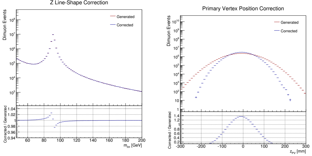
(a) The invariant mass, m_{\mu\mu} , dependent lineshape correction for the Z-boson modelling applied to the Drell-Yan signal MC. The top panel shows the nominal lineshape generated in MC and the corrected running-width lineshape. The bottom panel shows the ratio of the corrected and generated lineshapes.
