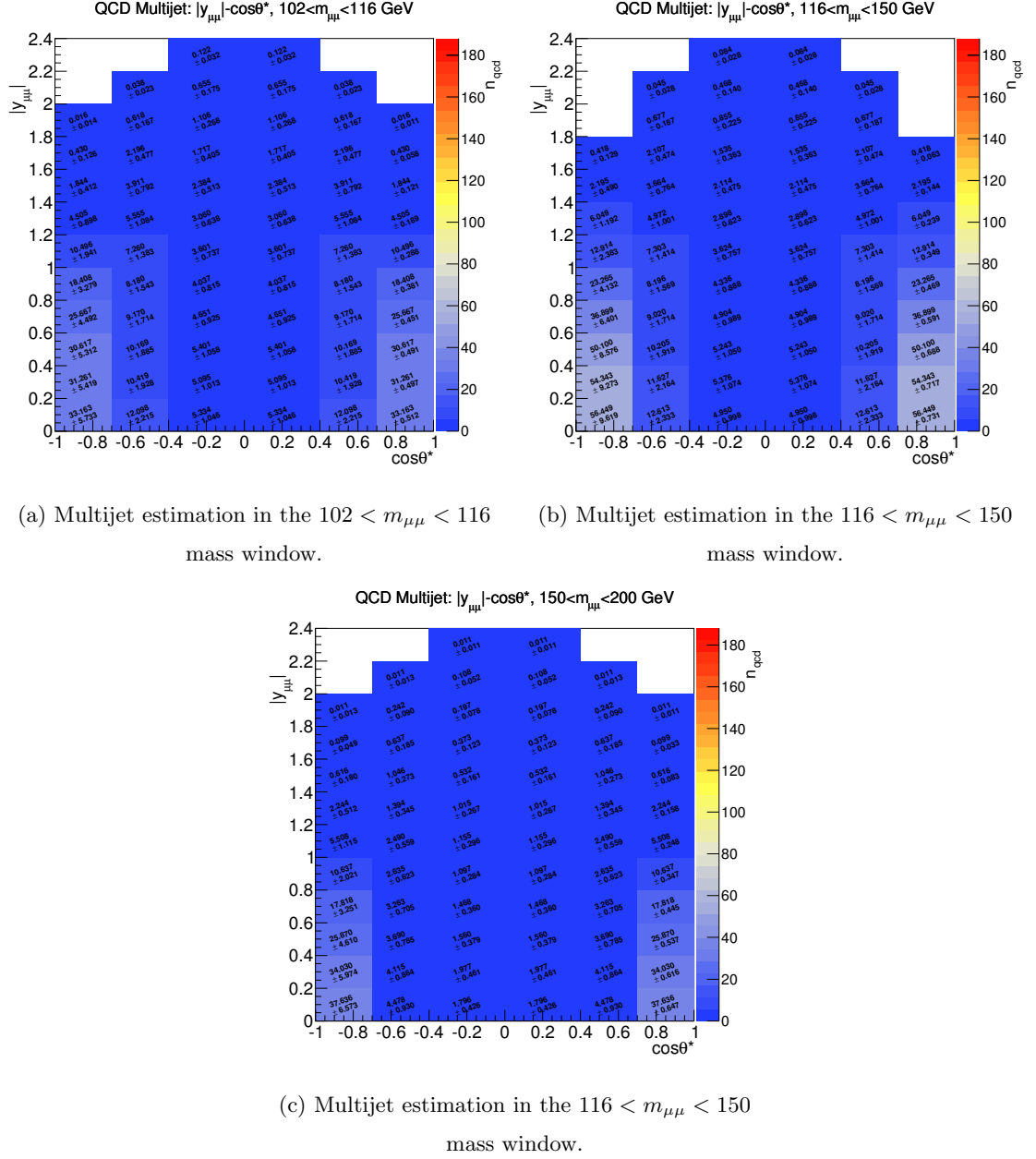
FIG. 54: Two dimensional ( y - \cos\theta^* ) plots of the dimuon QCD multijet background estimation in the last three invariant mass windows of the measurement. Uncertainties on the values include multijet systematic uncertainties, as described in Section 11, only.
