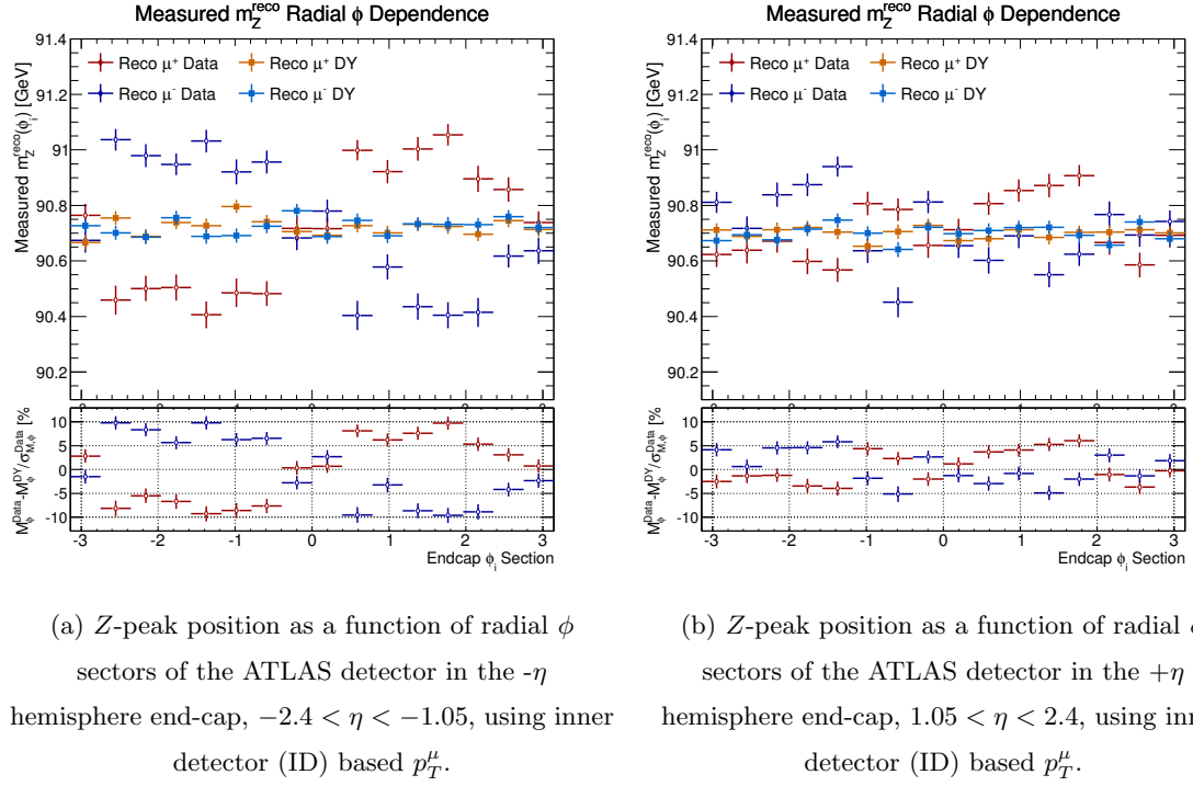
FIG. 46: The leading- p_T^\mu radial \phi dependence of the Z -peak position reconstructed in the ATLAS ID end-caps. The reconstructed DY signal MC prediction ( \mu^+ leading-muons in orange, \mu^- leading-muons in light-blue) is shown along with the measured data ( \mu^+ leading-muons in red, \mu^- leading-muons in dark-blue). The bottom panels show the relative positively- and negatively-charged leading- p_T^\mu muon agreement between data and MC. The agreement is shown as a percentage of the measured Z -peak width in data. Error bars show statistical uncertainties only.
