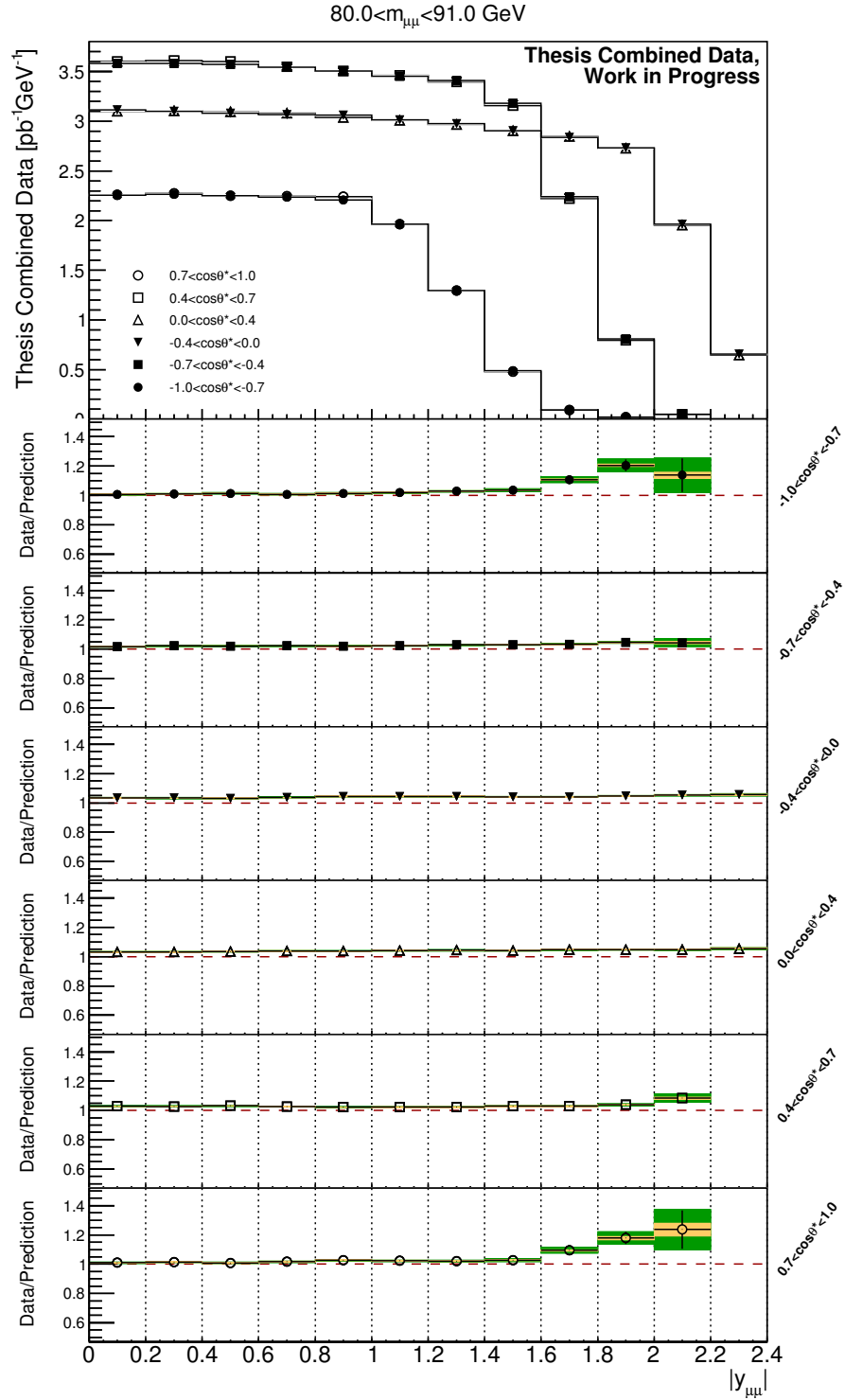
FIG. 85: Combined cross-section central values and uncertainty bands as a function of rapidity within the 80 < m_{\mu\mu} < 91 GeV mass regime. Each set of points corresponds to a different \cos \theta^* bin in the measurement. The ratios of data and MC predictions for each \cos \theta^* bin are provided in the sub-panels. The luminosity uncertainty of 1.9% is not included.
