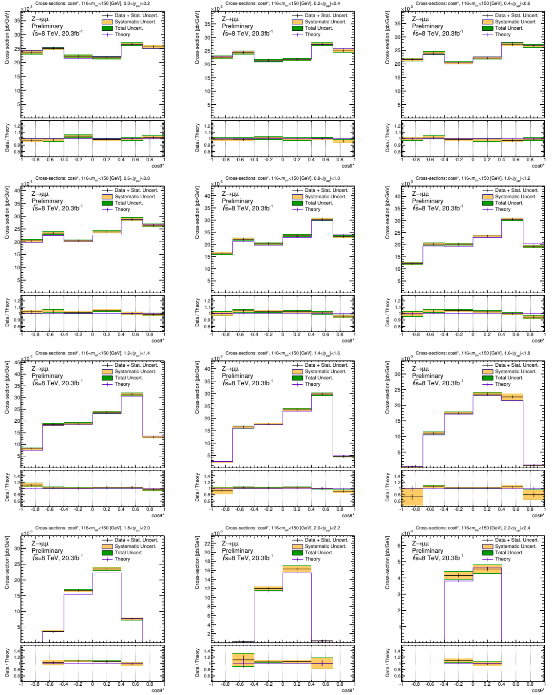
FIG. 79: Cross-section central values and uncertainty bands across each rapidity bin within the 116 < m_{ll} < 150 GeV mass regime unfolded to the Born truth-level with one Bayesian iteration. Theory predictions are taken from powheg-pythia8 Drell-Yan MC. The luminosity uncertainty of 1.9% is not included.
