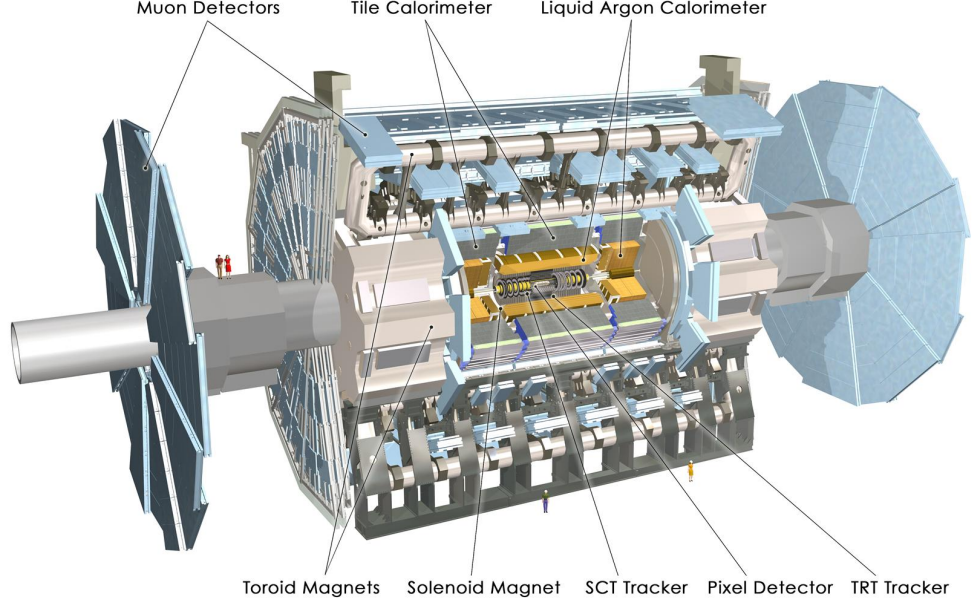
FIG. 13: Computer generated image of the ATLAS detector layout identifying the sub-detector components 61 .
