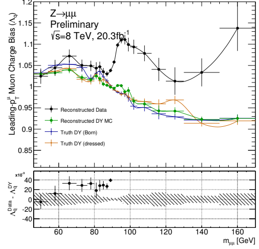
(b) \Lambda_q distributions, in the -\eta hemisphere end-cap, -2.4 < \eta < -1.05 , using combined muon (ID & MS) p_T^\mu .
