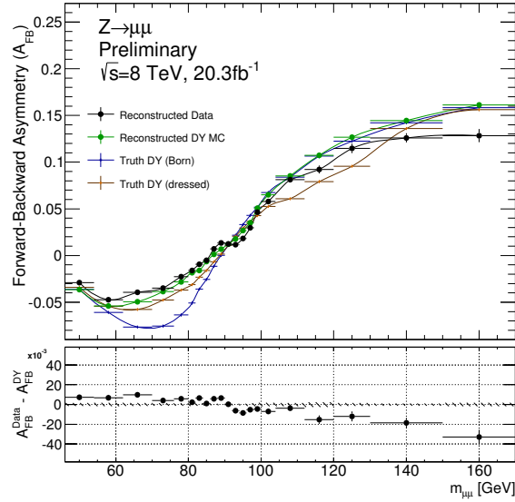
FIG. 40: Forward-backward asymmetry as a function of m_{\mu\mu} for the predictions of two truth-levels (Born and dressed) calculated from the signal MC, and non-unfolded results from reconstructed signal MC and background-subtracted data. The bottom panel displays the difference between reconstructed MC DY signal, A_{FB}^{DY} , and reconstructed background-subtracted data, A_{FB}^{data} . A smooth curve is displayed between points for clarity. Error bars show statistical uncertainties only.
