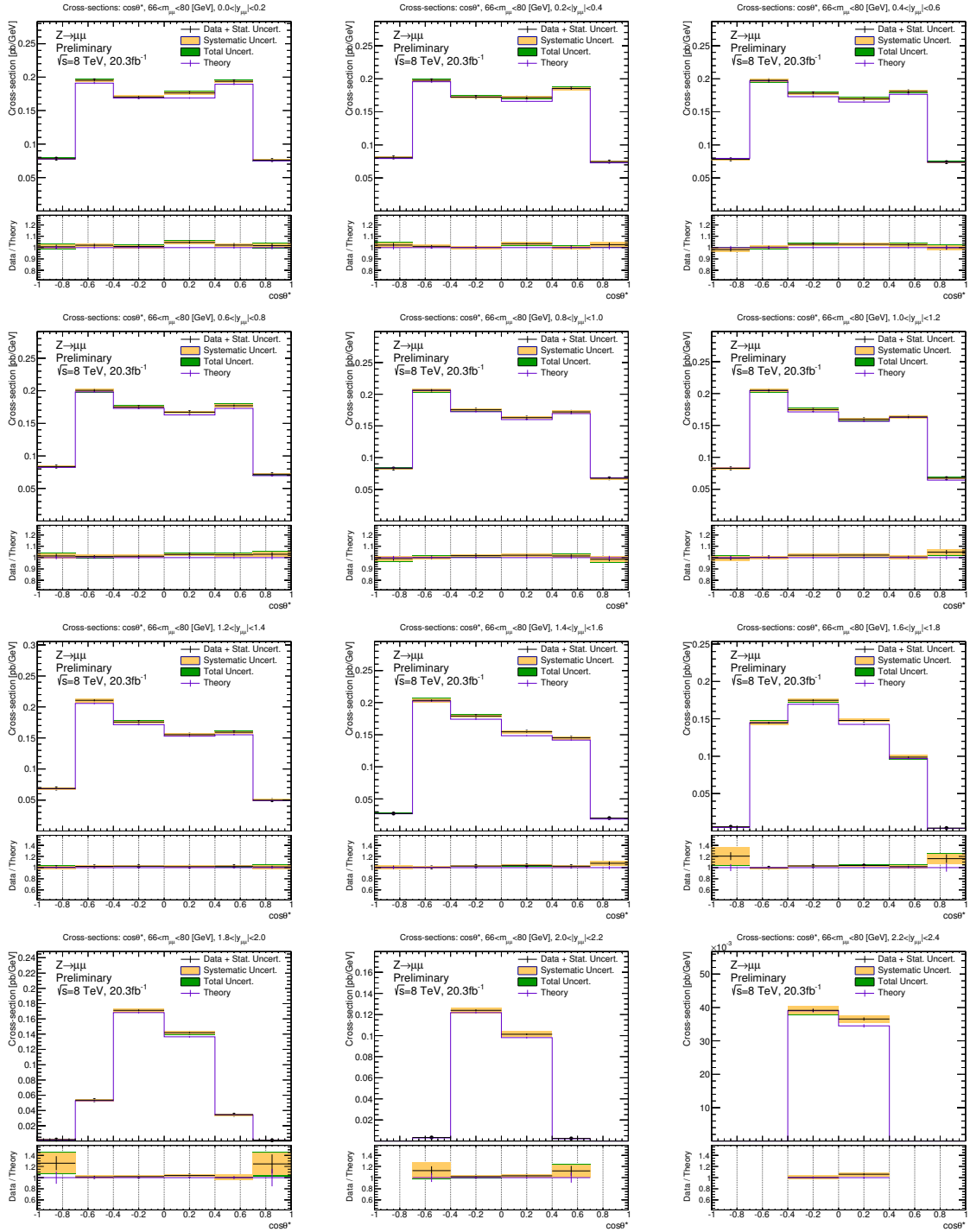
FIG. 75: Cross-section central values and uncertainty bands across each rapidity bin within the 66 < m_{\mu\mu} < 80 GeV mass regime unfolded to the Born truth-level with one Bayesian iteration. Theory predictions are taken from powheg-pythia8 Drell-Yan MC. The luminosity uncertainty of 1.9% is not included.
