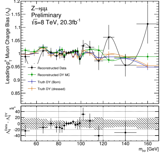
(d) \Lambda_q distributions, in the -\eta barrel hemisphere, -1.05 < \eta < 0.0 , using combined muon (ID & MS) p_T^\mu .
