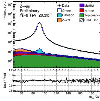
(h) Dimuon m_{\mu\mu} for |y_{\mu\mu}| < 1.0 .
