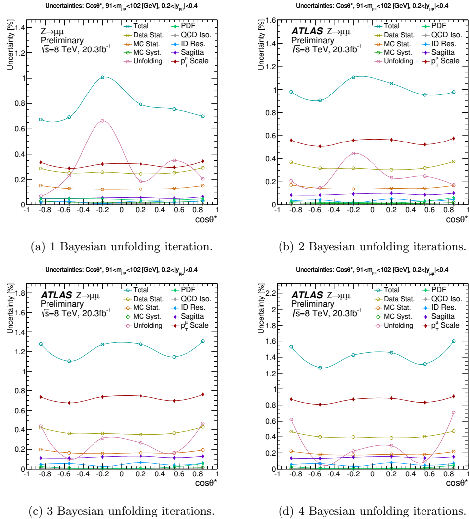
FIG. 67: Leading muon channel uncertainties for the 91 < m_{\mu\mu} < 102 \text{ GeV} and 0.2 < |y_{\mu\mu}| < 0.4 cross-section bin for different numbers of Bayesian unfolding iterations.
