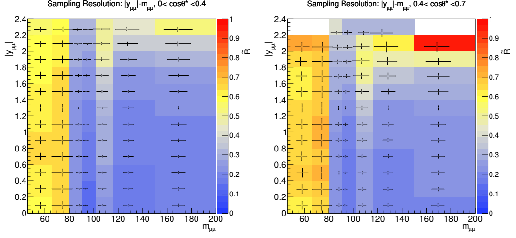
(a) Drell-Yan signal MC sampling resolution in the 0.0 < \cos\theta^* < 0.4 region. (b) Drell-Yan signal MC sampling resolution in the 0.4 < \cos\theta^* < 0.7 region.
