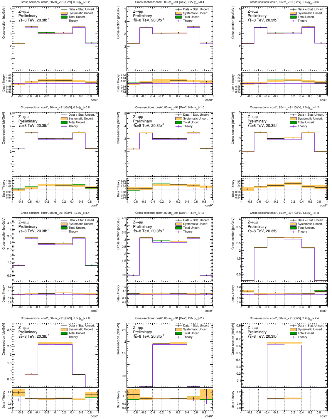
FIG. 76: Cross-section central values and uncertainty bands across each rapidity bin within the 80 < m_{ll} < 91 GeV mass regime unfolded to the Born truth-level with one Bayesian iteration. Theory predictions are taken from powheg-pythia8 Drell-Yan MC. The luminosity uncertainty of 1.9% is not included.
