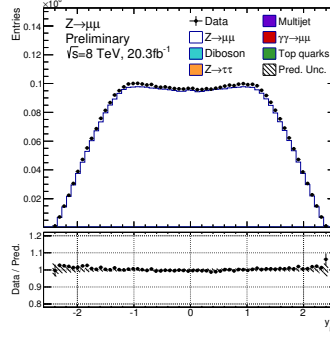
(b) Dimuon y_{\mu\mu} for all |y_{\mu\mu}| and 80 < m_{\mu\mu} < 91 GeV.
