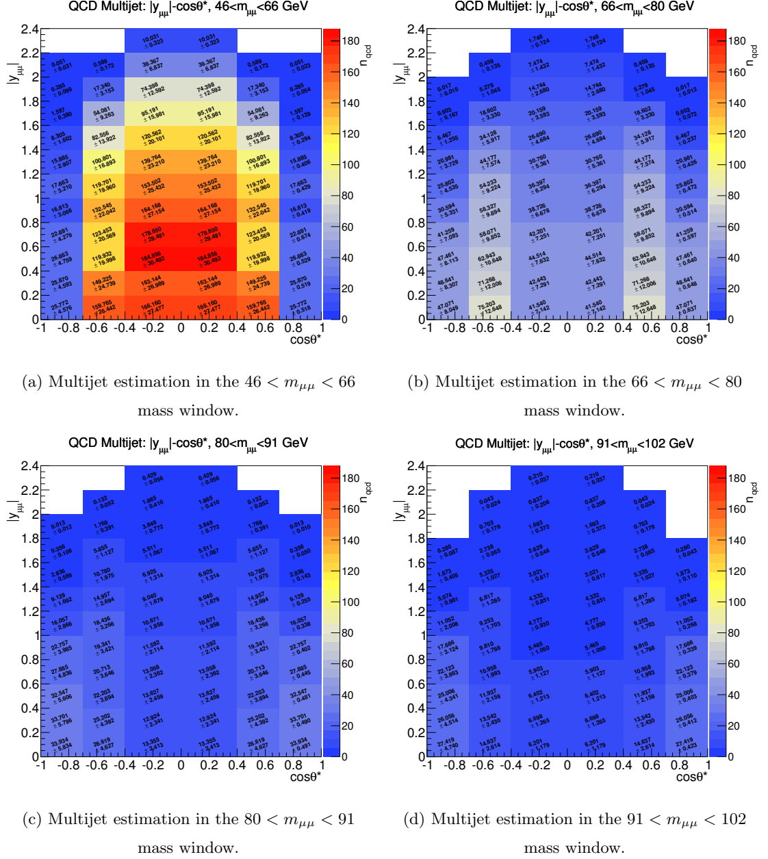
FIG. 53: Two dimensional ( y - \cos\theta^* ) plots of the dimuon QCD multijet background estimation in the first four invariant mass windows of the measurement. Uncertainties on the values include multijet systematic uncertainties, as described in Section 11, only.
