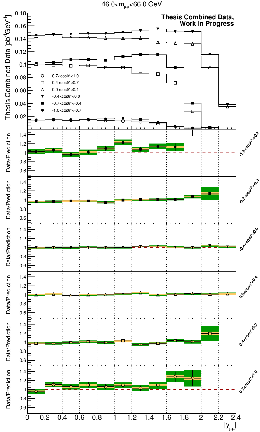
FIG. 83: Combined cross-section central values and uncertainty bands as a function of rapidity within the 46 < m_{ll} < 66 \text{ GeV} mass regime. Each set of points corresponds to a different \cos\theta^* bin in the measurement. The ratios of data and MC predictions for each \cos\theta^* bin are provided in the sub-panels. The luminosity uncertainty of 1.9% is not included.
