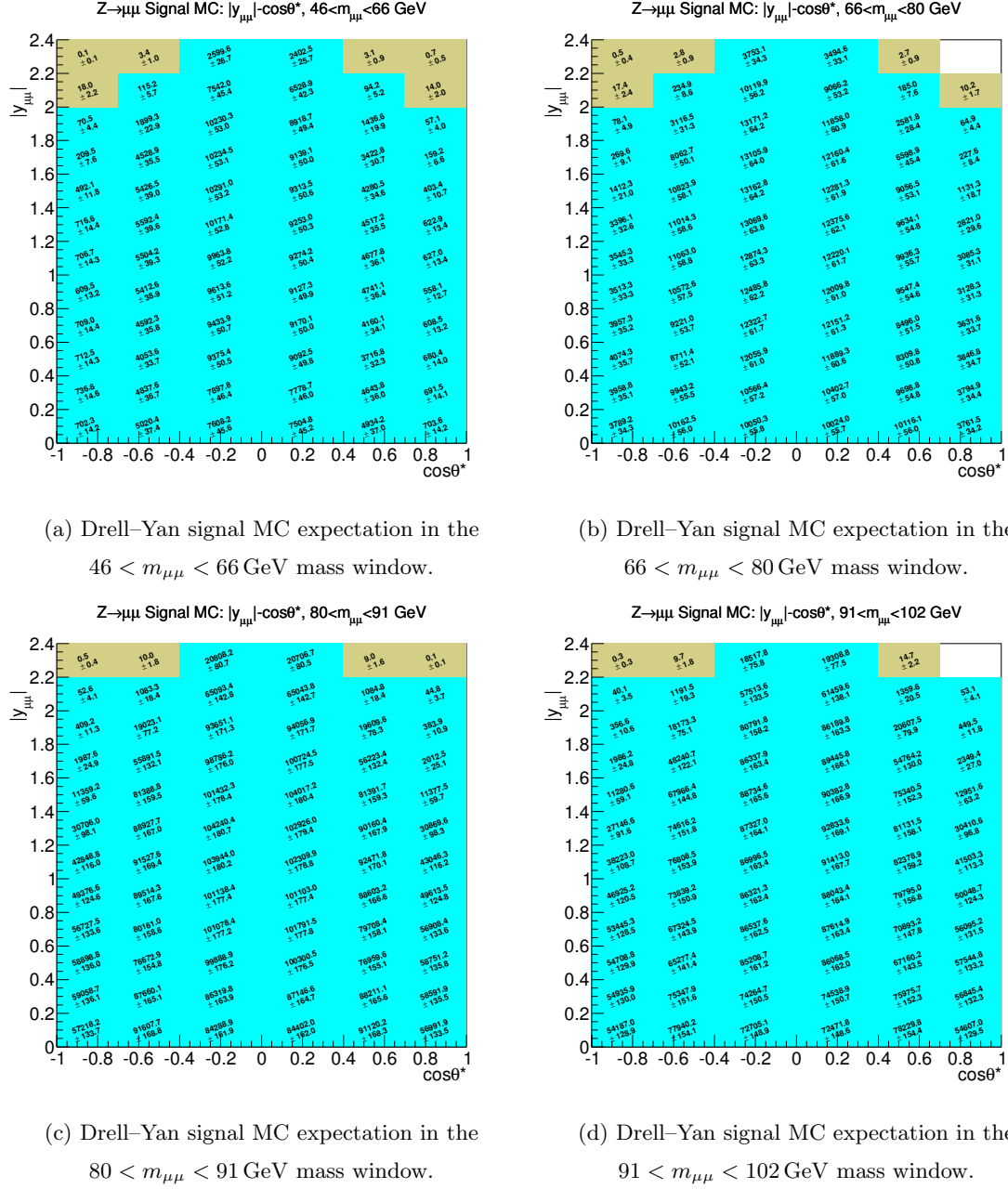
FIG. 72: Two dimensional ( |y_{\mu\mu}|, \cos\theta^* ) plots of the reconstructed DY signal expectation in the first four invariant mass windows of the measurement. Bins that are shown in blue pass the low statistics bin vetoing, bins in light brown are vetoed by the requirement and blank bins without a value are also vetoed. Only statistical uncertainties are shown on the values in each bin.
