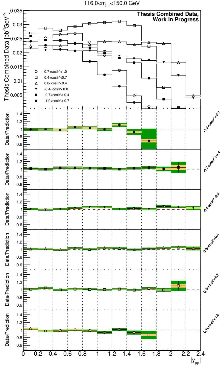
FIG. 88: Combined cross-section central values and uncertainty bands as a function of rapidity within the 116 < m_{ll} < 150 GeV mass regime. Each set of points corresponds to a different \cos \theta^* bin in the measurement. The ratios of data and MC predictions for each \cos \theta^* bin are provided in the sub-panels. The luminosity uncertainty of 1.9% is not included.
