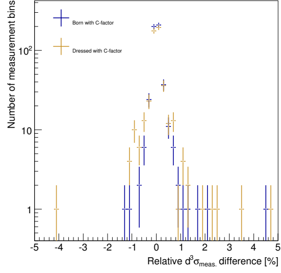
FIG. 93: Comparison of directly unfolded to the bare truth-level cross-section values with Born and dressed cross-section values with applied C -factors.
