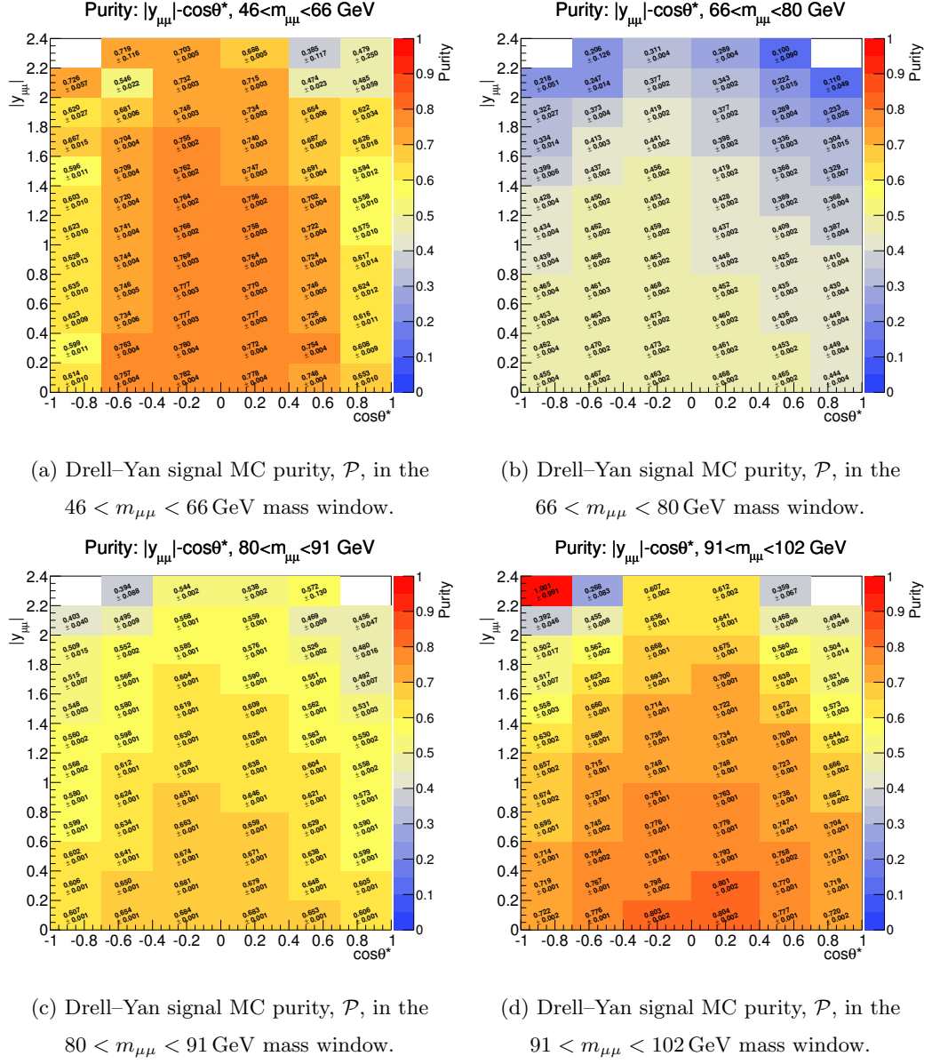
FIG. 31: Two dimensional (|y_{\mu\mu}|, \cos\theta^*) plots of the Drell-Yan signal purity in the first four invariant mass windows of the measurement. Uncertainties on the values show statistical uncertainties only.
