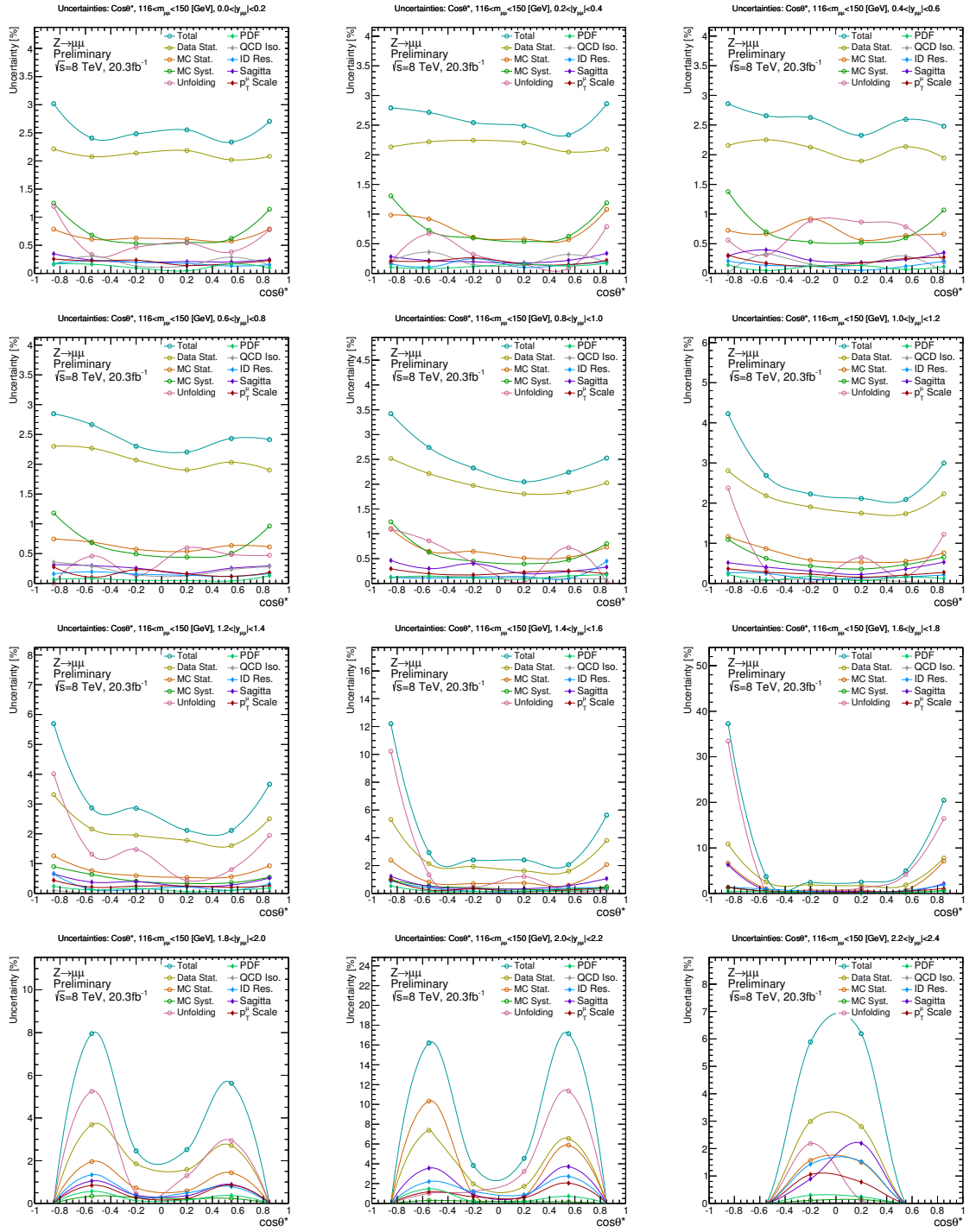
FIG. 65: Largest sources of uncertainty across each rapidity bin within the 116 < m_{\ell\ell} < 150 GeV mass regime.
