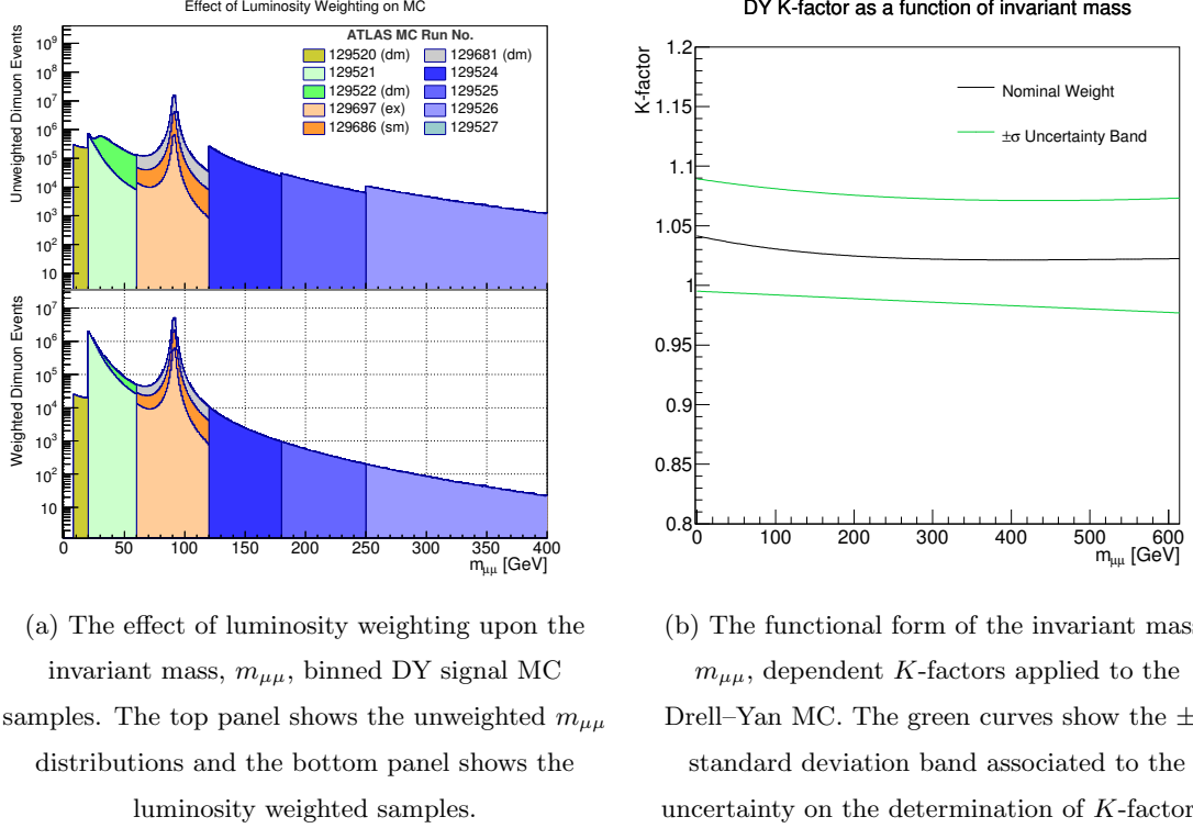
FIG. 35: Luminosity weighting and K -factor cross-section correction applied at the truth-level to MC simulation. Histogram error bars are statistical.
