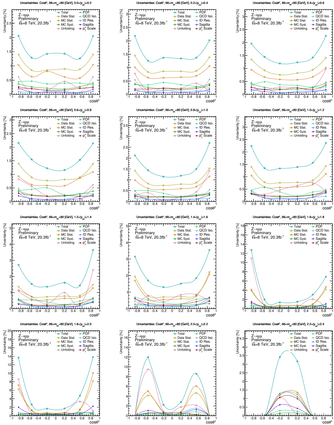
FIG. 61: Largest sources of uncertainty across each rapidity bin within the 66 < m_{\mu\mu} < 80 GeV mass regime.
