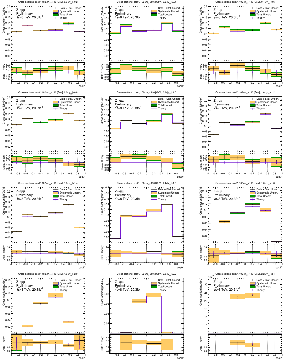
FIG. 78: Cross-section central values and uncertainty bands across each rapidity bin within the 102 < m_{\mu\mu} < 116 GeV mass regime unfolded to the Born truth-level with one Bayesian iteration. Theory predictions are taken from powheg-pythia8 Drell-Yan MC. The luminosity uncertainty of 1.9% is not included.
