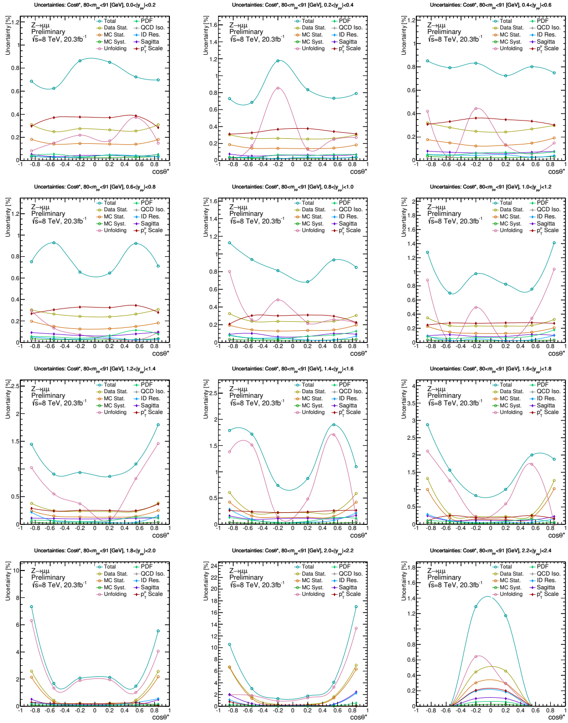
FIG. 62: Largest sources of uncertainty across each rapidity bin within the 80 < m_{\mu\mu} < 91 GeV mass regime.
