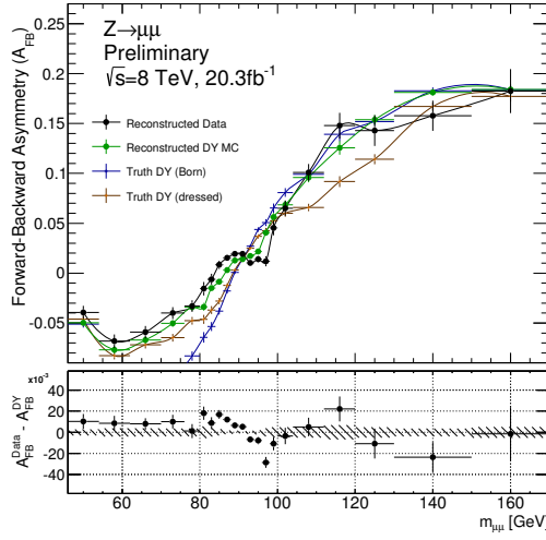
(a) A_{FB} distributions, in the -\eta hemisphere end-cap, -2.4 < \eta < -1.05 , using combined muon (ID & MS) p_T^\mu .
