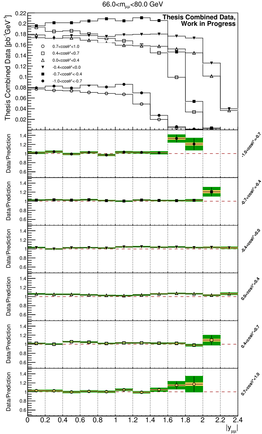
FIG. 84: Combined cross-section central values and uncertainty bands as a function of rapidity within the 66 < m_{\mu\mu} < 80 GeV mass regime. Each set of points corresponds to a different \cos \theta^* bin in the measurement. The ratios of data and MC predictions for each \cos \theta^* bin are provided in the sub-panels. The luminosity uncertainty of 1.9% is not included.
