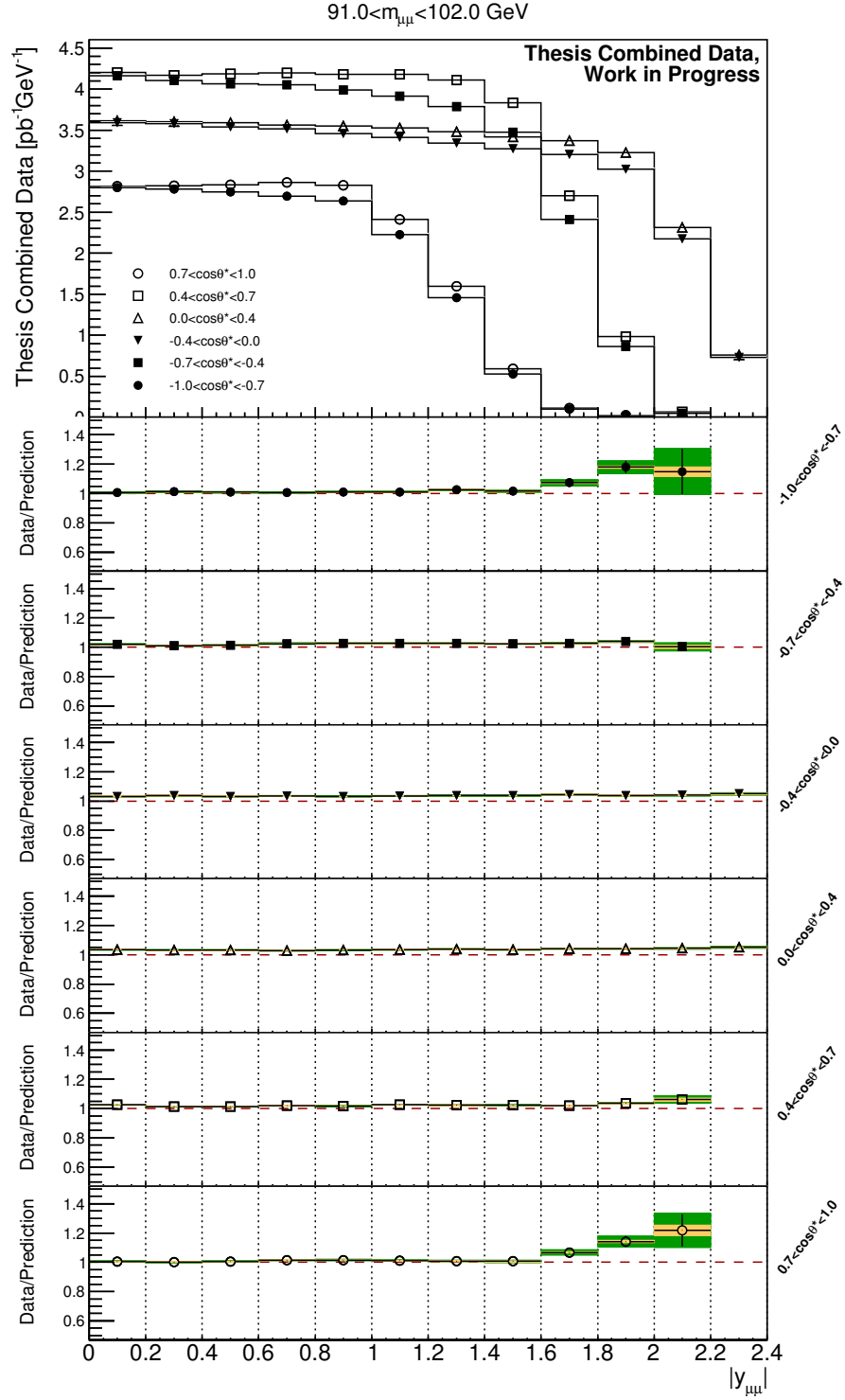
FIG. 86: Combined cross-section central values and uncertainty bands as a function of rapidity within the 91 < m_{ll} < 102 \text{ GeV} mass regime. Each set of points corresponds to a different \cos\theta^* bin in the measurement. The ratios of data and MC predictions for each \cos\theta^* bin are provided in the sub-panels. The luminosity uncertainty of 1.9% is not included.
