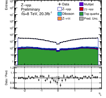
(f) Muon \eta_\mu for |y_{\mu\mu}| > 1.0 and 116 < m_{\mu\mu} < 150 GeV.
