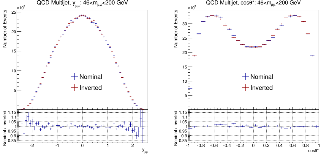
(a) Anti-isolated data y_{\mu\mu} distribution integrated in \cos\theta^* . The sign invariance is shown by the inverted distribution.
