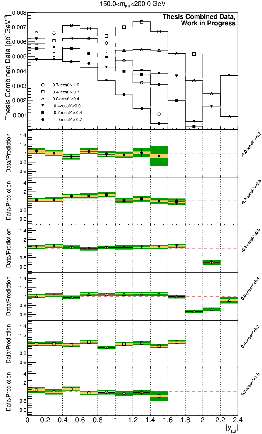
FIG. 89: Combined cross-section central values and uncertainty bands as a function of rapidity within the 150 < m_{ll} < 200 \text{ GeV} mass regime. Each set of points corresponds to a different \cos \theta^* bin in the measurement. The ratios of data and MC predictions for each \cos \theta^* bin are provided in the sub-panels. The luminosity uncertainty of 1.9% is not included.
