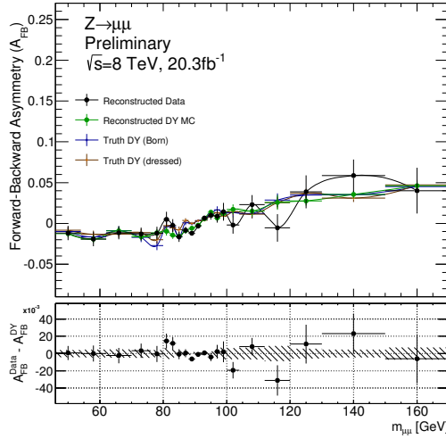
(c) A_{FB} distributions, in the -\eta barrel hemisphere, -1.05 < \eta < 0.0 , using combined muon (ID & MS) p_T^\mu .
