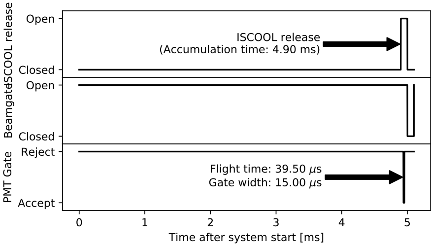
Figure 5.3: For bunching ^{40}\text{Ar} , the ions were accumulated in ISCOOL for 4.9 ms and then released. The gate on the signal of the PMTs starts 39.5 μs after release of the bunch and is 15 μs long. After ISCOOL closes, the beamgate briefly closes and the cycle repeats continuously. ^{36,38}\text{Ar} used different flight times only.
