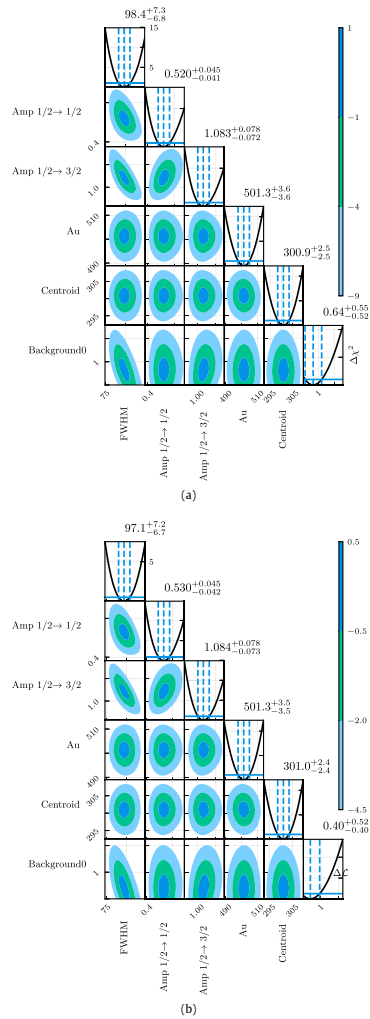
Fig. 3. Output of generate_correlation_map for (a) \chi^2 (Listing 1 line 24) and (b) likelihood (Listing 1 line 28) for the toy dataset. The diagonals show the resulting change in \chi^2 or likelihood after fixing one parameter and refitting. The 1\sigma boundaries are also indicated. The 2D contourplot is achieved in the same way with 2 parameters fixed.
