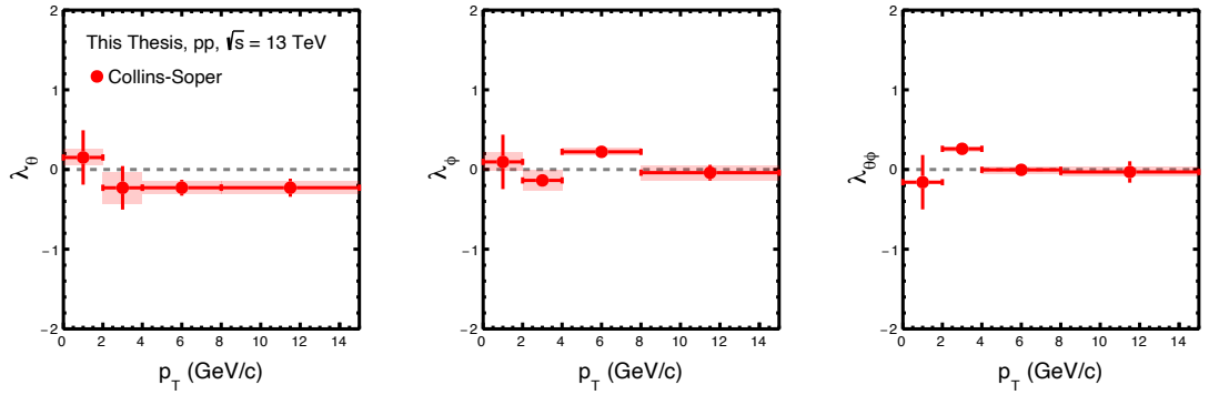
Figure 4.24: Polarization parameters \lambda_\theta , \lambda_\phi and \lambda_{\theta\phi} as a function of transverse momentum for Collins-Soper frame with systematic uncertainties [123].
