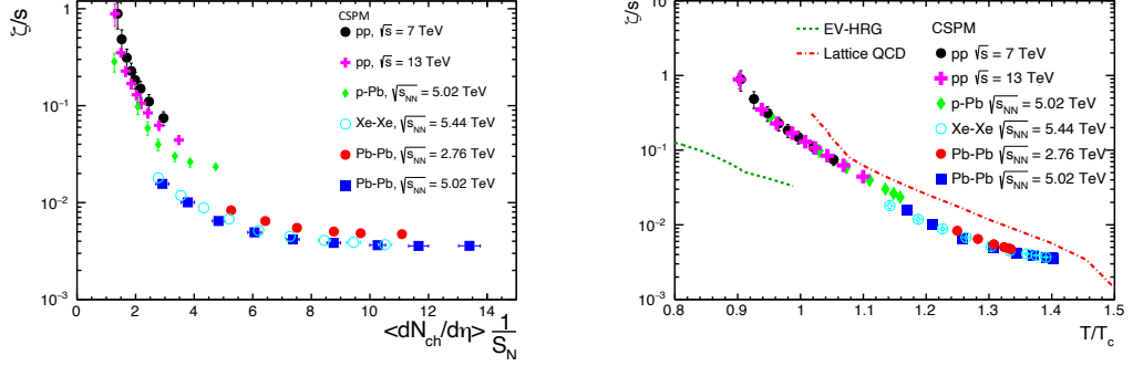
Figure 2.9: The ratio of bulk viscosity to entropy density as a function of charged particle multiplicity density (left panel) and initial percolation temperature scaled with critical temperature (right panel) for pp collisions at \sqrt{s} = 7 and 13 TeV, p -Pb collisions at \sqrt{s_{NN}} = 5.02 TeV, Xe-Xe collisions at \sqrt{s_{NN}} = 5.44 TeV, Pb-Pb collisions at \sqrt{s_{NN}} = 2.76 and 5.02 TeV [50] estimated from the CSPM.
