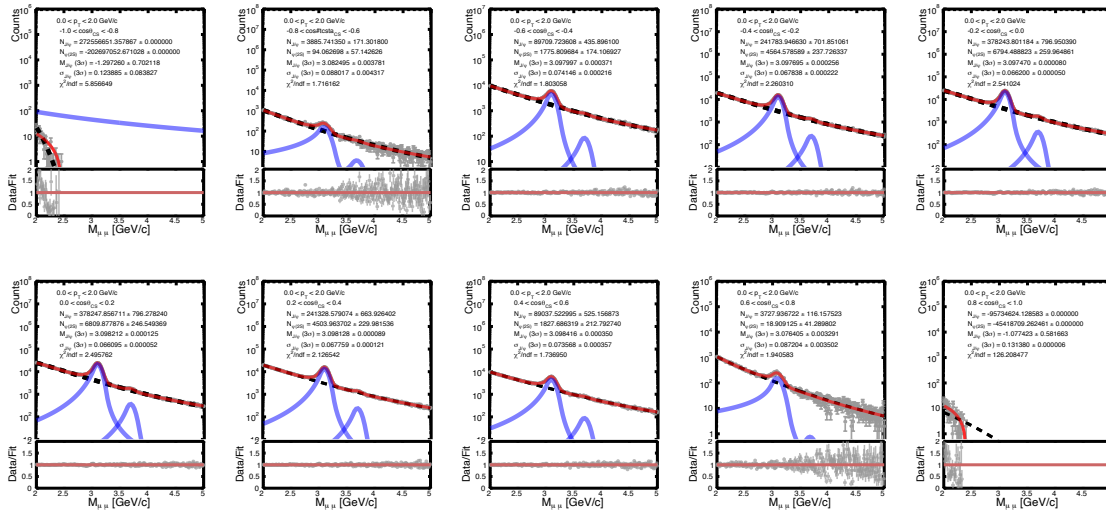
Figure 6.9: Double Crystal Ball + variable width Gaussian function fit to the invariant mass spectra for various \cos\theta ranges for 0.0 < p_T < 2.0 GeV/c in the Collin-Soper frame [123].
