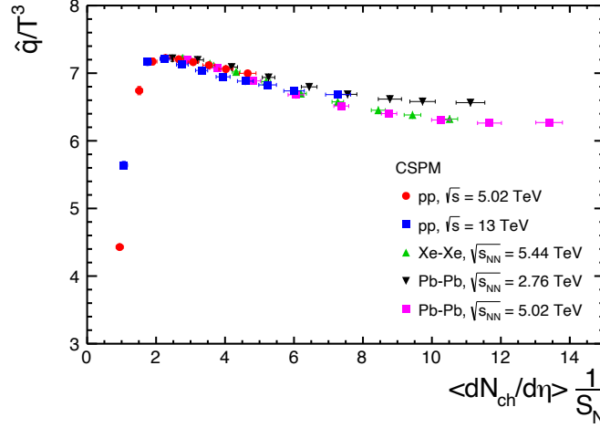
Figure 2.14: \hat{q}/T^3 vs charged particle multiplicity scaled by S_{\perp} for pp collisions at \sqrt{s} = 5.02 and 13 TeV, Xe–Xe collisions at \sqrt{s_{NN}} = 5.44 TeV and Pb–Pb collisions at \sqrt{s_{NN}} = 2.76 and 5.02 TeV [81] estimated from the CSPM.
