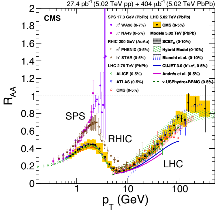
Figure 1.4: Nuclear modification factor, R_{AA} , for neutral pions, charged hadrons, and charged particles in central heavy-ion collisions at SPS, RHIC and the LHC [5].
