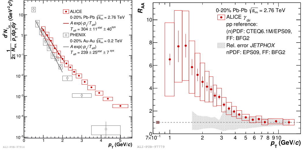
Figure 1.7: Initial photon spectra (left panel) and nuclear modification factor of direct photons for 0 – 20% centrality Pb–Pb collisions at \sqrt{s_{\text{NN}}} = 2.76 TeV [8] (right panel).
