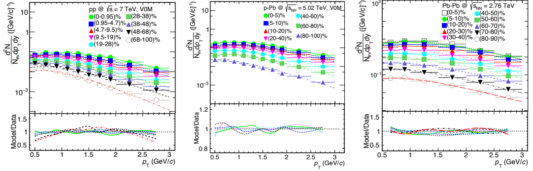
Figure 3.7: Blastwave fits to the transverse momentum spectra of \phi meson for pp collision at \sqrt{s} = 7 TeV, p-Pb collision at \sqrt{s_{\text{NN}}} = 5.02 TeV and Pb-Pb collision at \sqrt{s_{\text{NN}}} = 2.76 TeV for various multiplicity classes [95].
