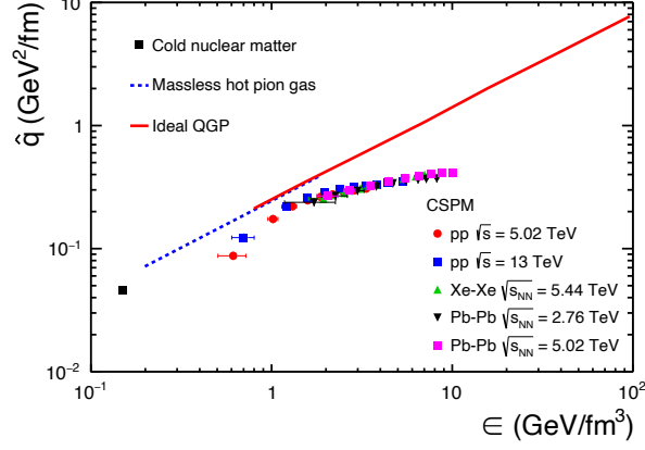
Figure 2.15: Jet quenching parameter \hat{q} as a function of initial energy density for pp collisions at \sqrt{s} = 5.02 and 13 TeV, Xe–Xe collisions at \sqrt{s_{\text{NN}}} = 5.44 TeV and Pb–Pb collisions at \sqrt{s_{\text{NN}}} = 2.76 and 5.02 TeV [81]. The blue dotted line is for massless pion gas, the solid red curve is for ideal QGP, and the black square is for cold nuclear matter [82] estimated from the CSPM.
