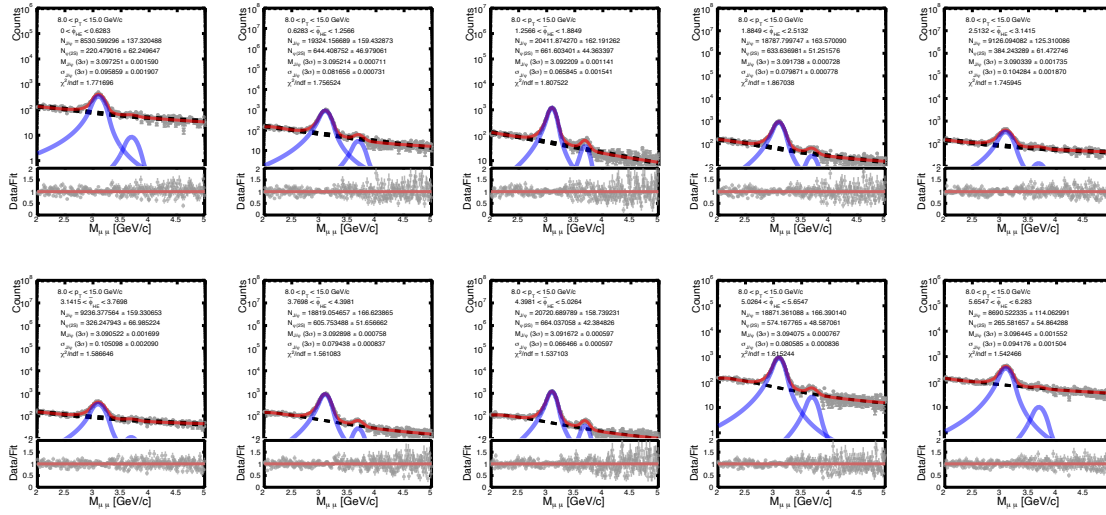
Figure 6.32: Double Crystal Ball + variable width Gaussian function fit to the invariant mass spectra for various \tilde{\phi} ranges for 8.0 < p_T < 15.0 GeV/c in the helicity frame [123].
