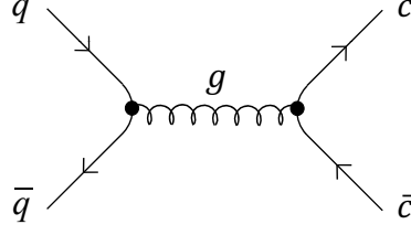
Figure 4.4: Charmoina production from quark anti-quark annihilation.
