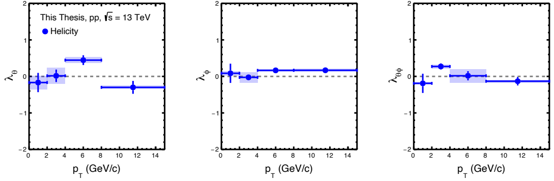
Figure 4.23: Polarization parameters \lambda_\theta , \lambda_\phi and \lambda_{\theta\phi} as functions of transverse momentum for helicity frame with systematic uncertainties [123].
