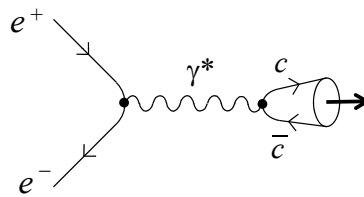
Figure 4.3: Charmoina production through electron-positron annihilation.
