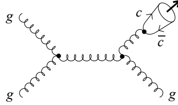
Figure 4.5: Charmoina production through gluon fragmentation.
