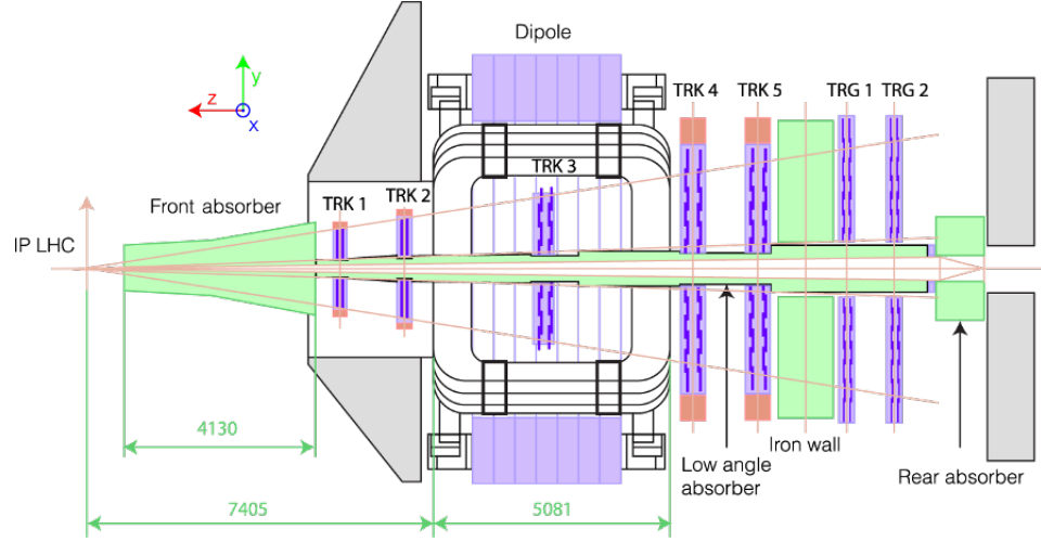
Figure 4.2: A schematic diagram of the muon spectrometer.
