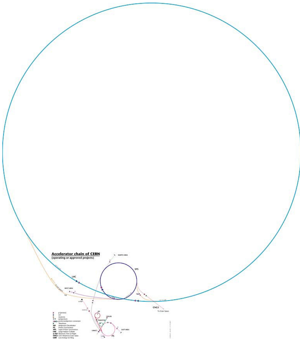
FIGURE 56 The true scale cartoon of the CERN accelerator complex. LHC dominates the view with its 27 km circumference [178].
