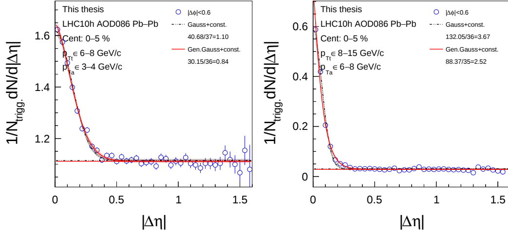
FIGURE 36 Example per-trigger yields with the two fit functions of the analysis for the lowest (left) and highest (right) p_{Tt} - p_{Ta} combinations, respectively.
