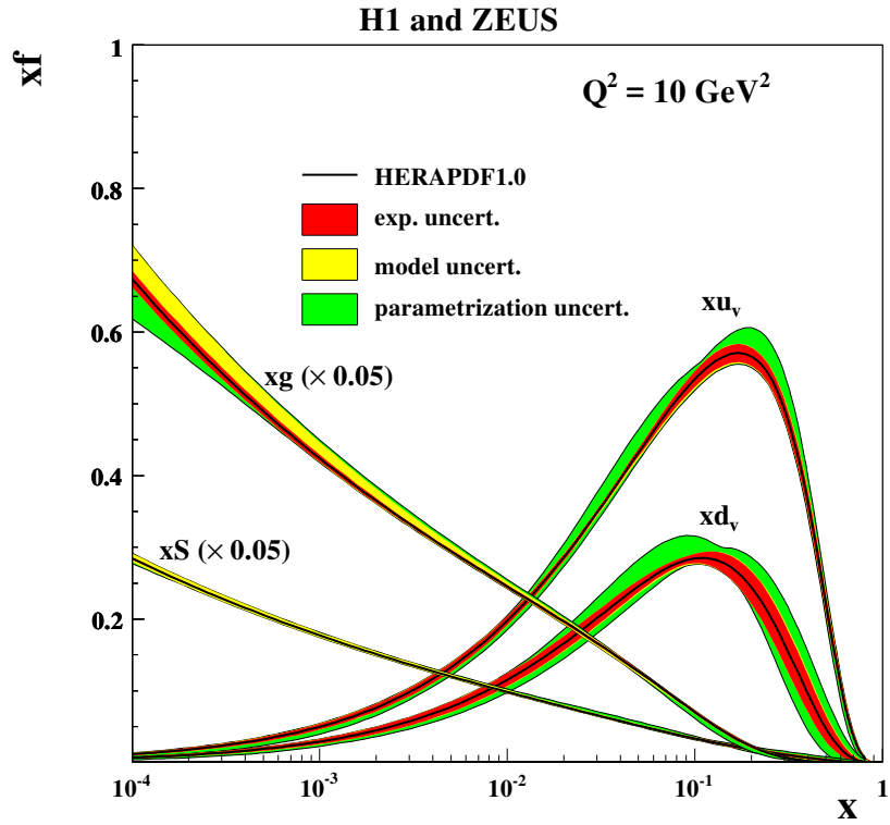
FIGURE 6 The parton distribution functions from combined data of HERA and ZEUS [53].
