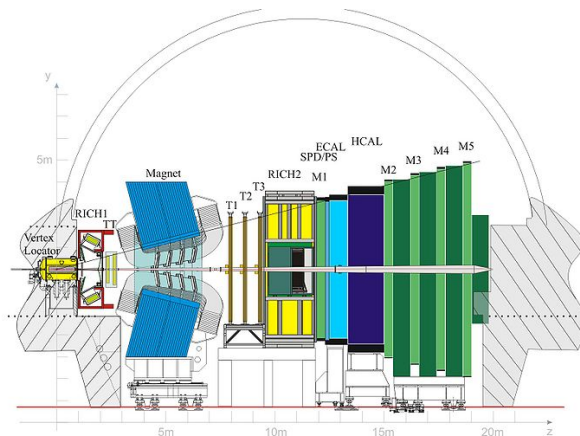
(a) LHCb Schematic view [5].
