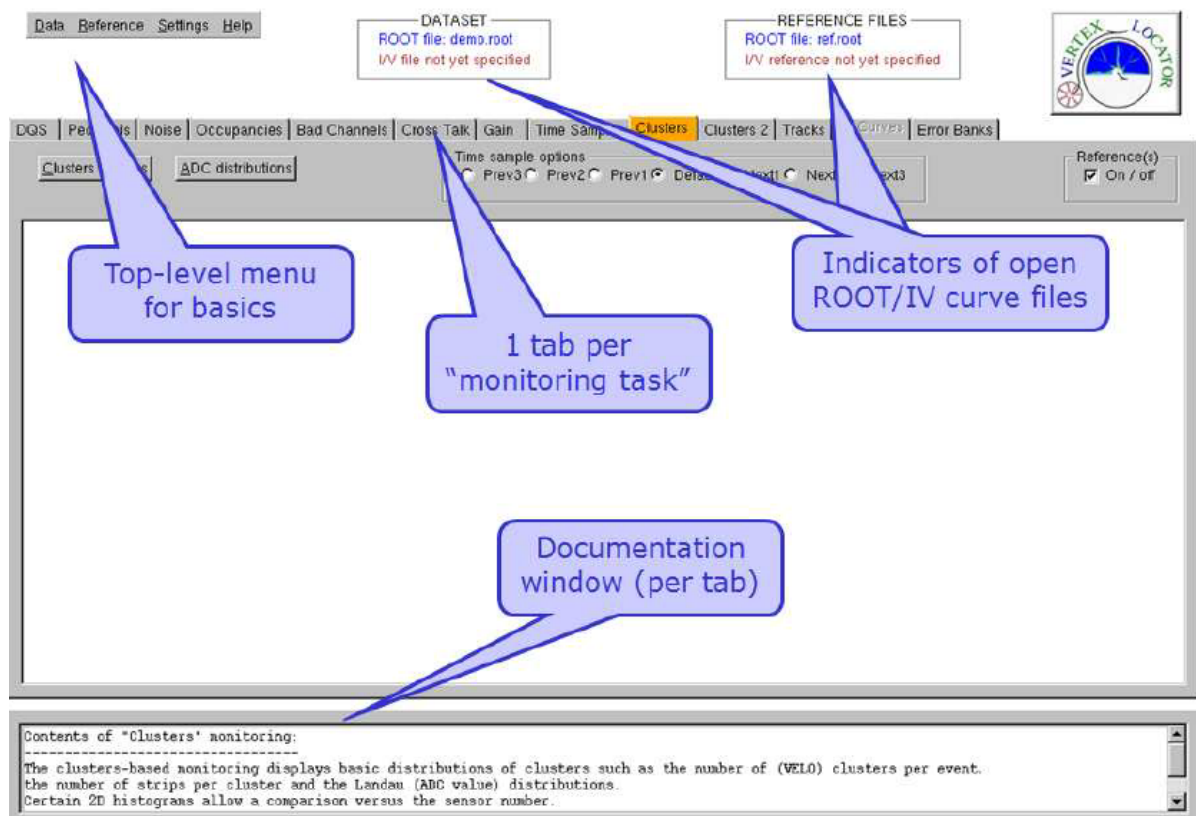
Figure 3.6: Overview of the VeloMoniGUI [18].
