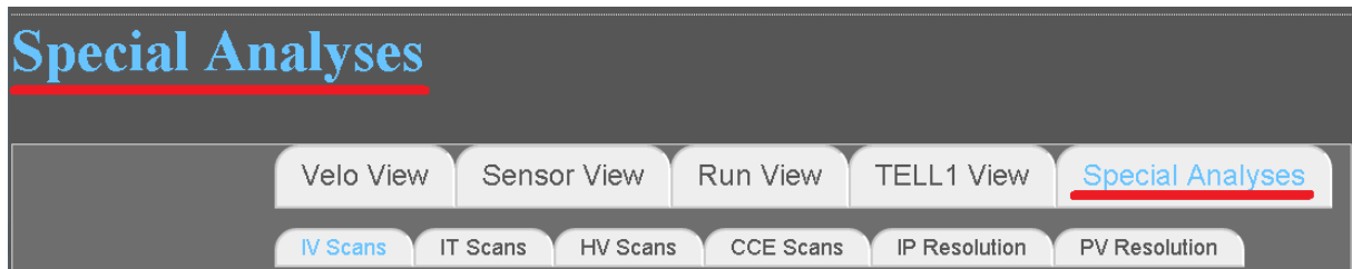
Figure 4.3: Tabs highlighting.
