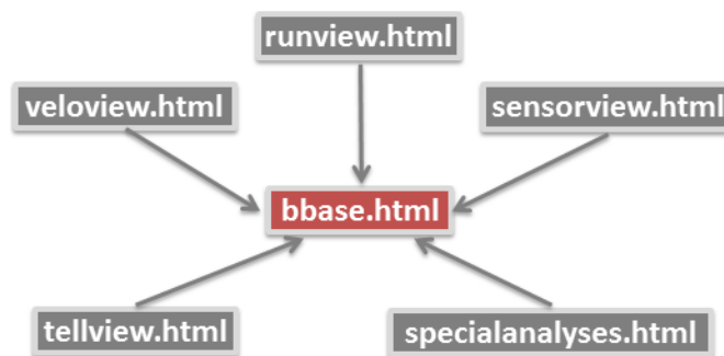
Figure 5.7: bbase.html inheritance diagram.
