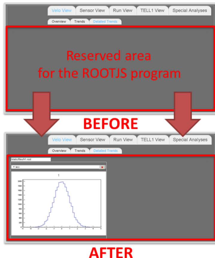
Figure 5.20: Integration overview.
