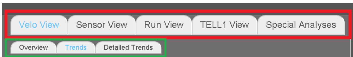
Figure 4.4: Navigation bars.
