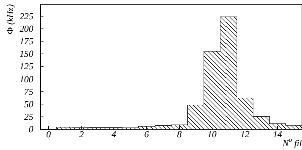
Figure 4.14: Flux incident per wire of the prototype DC1 for different values of cathode plane voltage. The muon beam is shifted 35 mm horizontally from the center of the detector.
