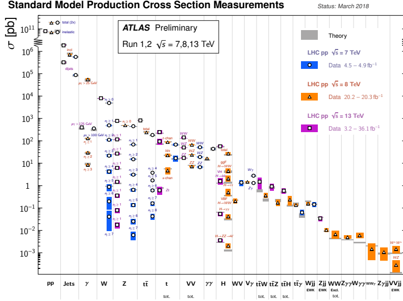
Figure 1.2: Summary of several SM total and fiducial production cross section measurements, corrected for leptonic branching fractions, compared to the corresponding theoretical expectations. All theoretical expectations were calculated at NLO or higher. The measurements have been performed with the ATLAS detector at \sqrt{s} = 7, 8 and 13 TeV. The luminosity used for each measurement is indicated close to the data point.
