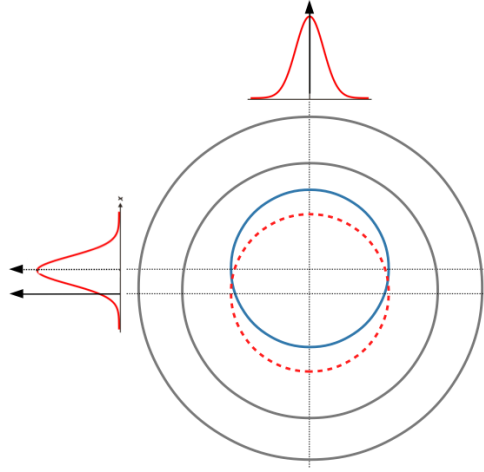
Figure 3.4: Schematic representation of how a vertical displacement of a barrel layer will reflect on the residual distributions. The real position of the inner layer is painted with a blue circle. If the detector is not aligned, it is assumed that the layer is at its nominal position (red dashed circle) for the track reconstruction, what introduces a shift of the residuals distributions in the direction transverse to the displacement.
