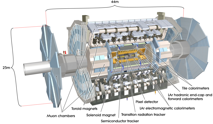
Figure 2.5: A cut-away view of the ATLAS detector, displaying its major subsystems. Some people are drawn together with the detector to show the real scale of the detector [29].
