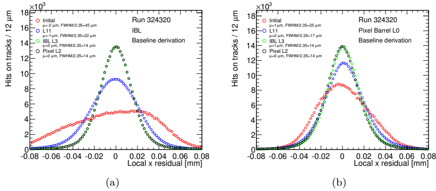
Figure 7.1: IBL (a) and Pixel first layer (b) local- x residual distributions for four different alignment constants: from last 2016 alignment constants, after the IBL bowing was extrapolated to -20 °C (in red); after a L11 alignment (in blue); after a L3 alignment of the IBL (in green); and after a L2 alignment of the Pixel (in black).
