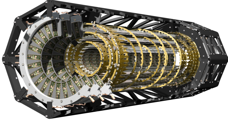
Figure 2.8: Schematic drawing of the ATLAS Pixel Detector [28].
