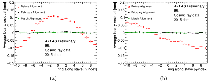
Figure 5.4: The IBL mean of the local- x (a) and local- y (b) residual distributions as a function of the \eta position of the module, before alignment (red) and with February (black) and March (green) alignments [60].
