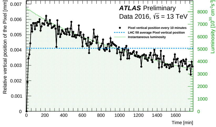
Figure 4.10: Short time scale movements of the Pixel detector during a fill. Every time the Pixel detector is switched on it rises fast during a transitory regime until it reaches a maximum. Afterwards (in a high luminosity LHC fill) the Pixel detector goes down following closely the behaviour of the luminosity of the beams. The black points correspond to the vertical position of the Pixel detector as a function of time (every 10 min) and relative to the initial measurement, whereas the instantaneous luminosity is plotted in the green area histogram. The relative normalisation of both histograms allows a straight comparison. The dashed blue line corresponds to the average vertical position that would be computed from the entire range [59].
