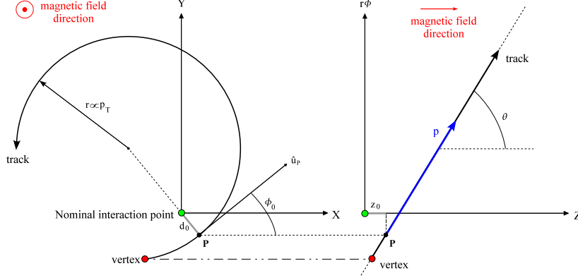
Figure 3.2: Graphical interpretation of track parameters at perigee, P .
