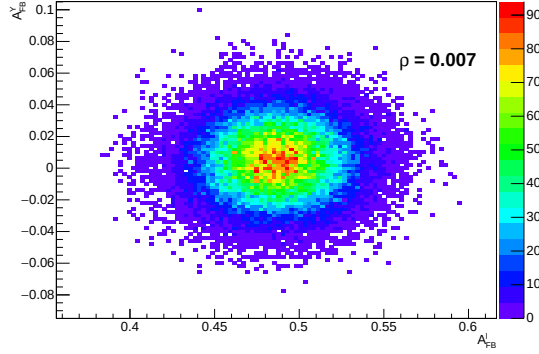
Figure 15.2: Statistical correlation between the measured asymmetries A_{\text{FB}}^Y and A_{\text{FB}}^L evaluated from data using the bootstrapping method. The derived correlation coefficient, computed from the ratio between the covariance of the two asymmetries and the product of their standard deviations, is quoted.
