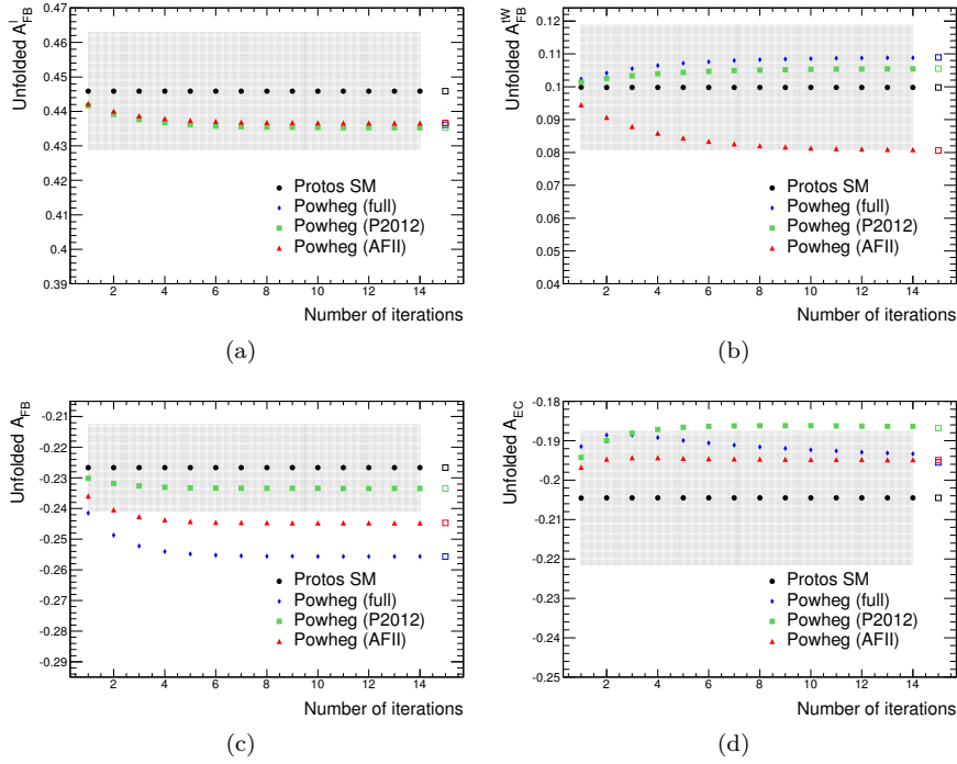
Figure 13.3: Unfolded values of the asymmetries as a function of the number of iterations of the bayesian unfolding algorithm: (a) A_{\text{FB}}^{\ell} , (b) A_{\text{FB}}^{tW} , (c) A_{\text{FB}} , and (d) A_{\text{EC}} . The SM PROTOS (black points), the nominal POWHEG-BOX (blue diamonds), the POWHEG-BOX with the P2012 tune (green boxes), and the ATLFAS-II POWHEG-BOX (red triangles) event samples are used. A grey band around the PROTOS sample points is drawn with a width equal to the statistical uncertainty due to the limited size of the simulated sample. The results given by a simple inversion of the migration matrix are also shown for comparison (empty squares at the last bin).
