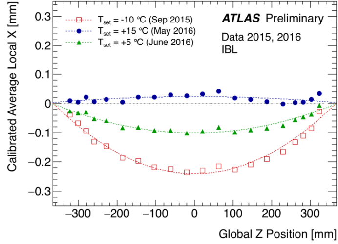
Figure 5.14: IBL local-x correction in the transverse plane averaged over all 14 IBL staves for 2015 data (red open squares), and for 2016 data using different T_{\text{set}} (+15 ^{\circ}\text{C} , solid blue circles; +5 ^{\circ}\text{C} , solid green triangles) [66].
