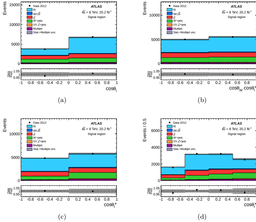
Figure 12.1: Angular distributions in the signal region for the combined electron and muon channels (a) \cos\theta_\ell , (b) \cos\theta_W \cos\theta_\ell^* , (c) \cos\theta_\ell^* with 2 bins, and (d) \cos\theta_\ell^* with 4 bins. The predicted distributions are re-scaled using the values given in table 10.1. The uncertainty bands correspond to the errors due to the limited size of the simulation samples added in quadrature with the data-driven normalisation uncertainty estimated for the multijet contribution.
