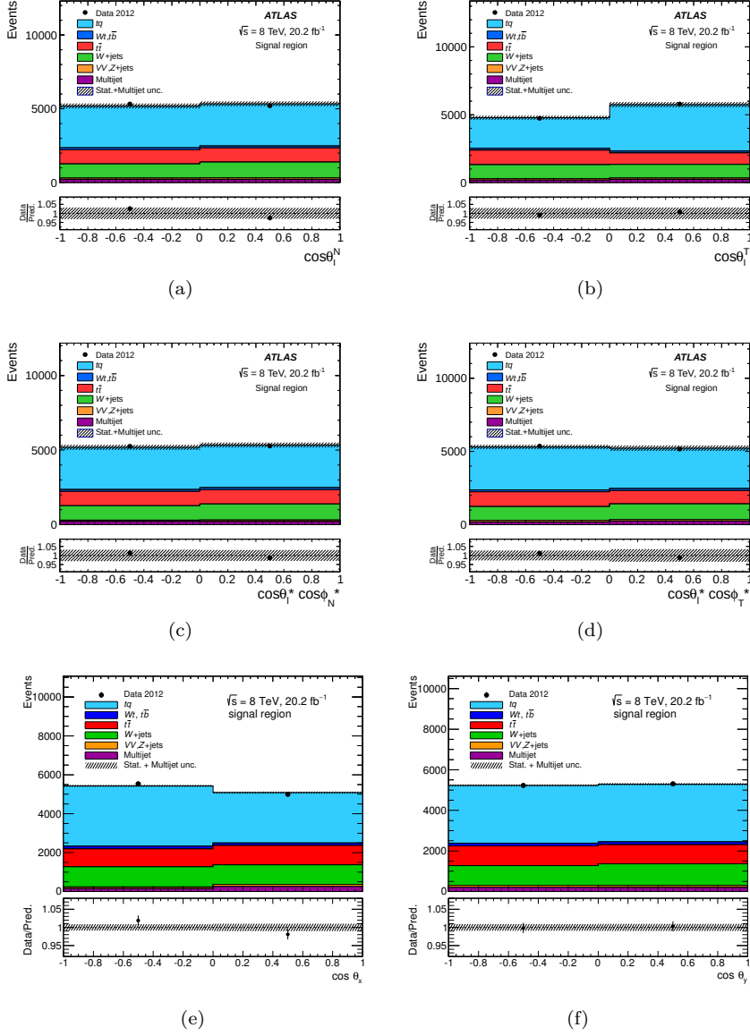
Figure 12.2: Angular distributions in the signal region for the combined electron and muon channels (a) \cos\theta_\ell^N , (b) \cos\theta_\ell^T , (c) \cos\theta_\ell^* \cos\phi_N^* , (d) \cos\theta_\ell^* \cos\phi_T^* , (e) \cos\theta_x and (f) \cos\theta_y . The predicted distributions are re-scaled using the values given in table 10.1. The uncertainty bands correspond to the errors due to the limited size of the simulation samples added in quadrature with the data-driven normalisation uncertainty estimated for the multijet contribution.
