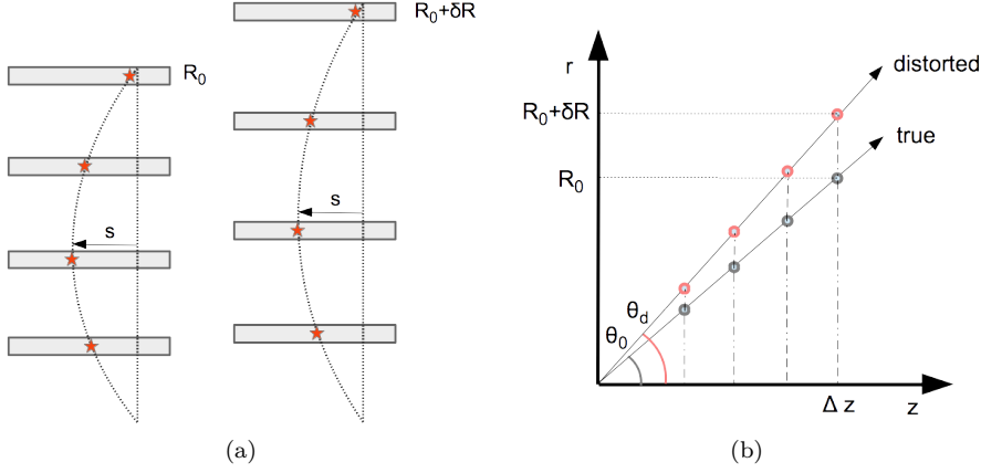
Figure 3.6: Schematic representation of how the radial distortion leaves invariant the sagitta of the track, left, while modifying the \cot \theta of the track, right. In the left figure, the reconstructed points are located at different radii, but at the same transverse distance than the true ones. In the right diagram, true points are given in grey, while the reconstructed points with the distorted geometry are shown in red. In this model, the z coordinate of the points is preserved and the r coordinate is changed proportionally to the true radius.
