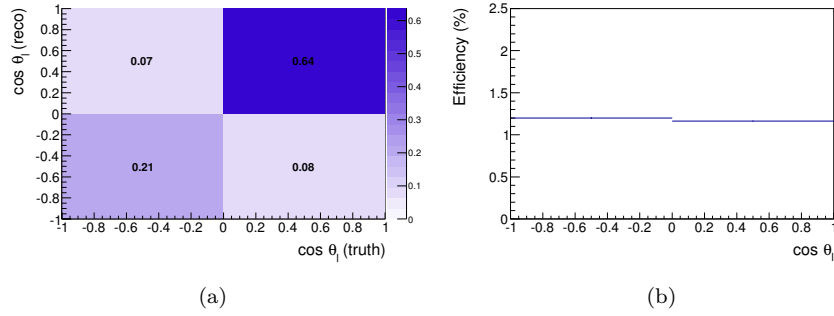
Figure 13.2: (a) Migration matrix and (b) efficiency curve for the \cos\theta_l distribution.
