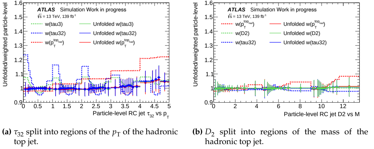
Figure 6.25: Particle-level distributions for substructure observables, further divided into regions of the top jet kinematics. The lines represent a ratio to the re-weighted particle-level distribution. The dashed lines are for the nominal particle-level prediction, whilst the solid lines are for the re-weighted detector-level MC which has been unfolded. The ratio for the unfolded distribution should be compatible with unity in order for the test to have achieved closure.
