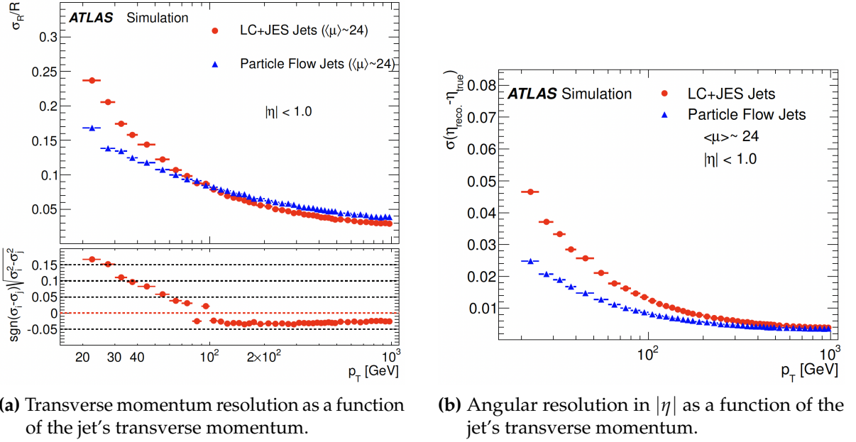
Figure 3.5: Resolution comparison between jets clustered from calorimeter clusters and particle flow jets, simulated in MC for dijet events. Plots from Ref. [112].
