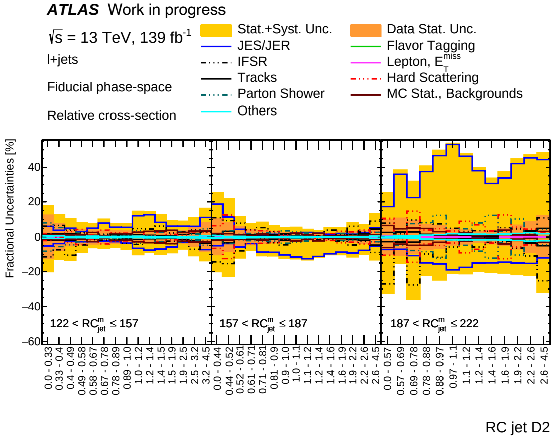
Figure 7.7: Uncertainties on the distribution of the t\bar{t} \ell + \text{jets} production cross-section as a function of the D_2 substructure observable for the large- R reclustered jet which is the hadronic top jet candidate, split into three regions of the mass of the jet. Statistical uncertainties are shown in an orange band, while the yellow band shows the sum of statistical and systematic uncertainties.
