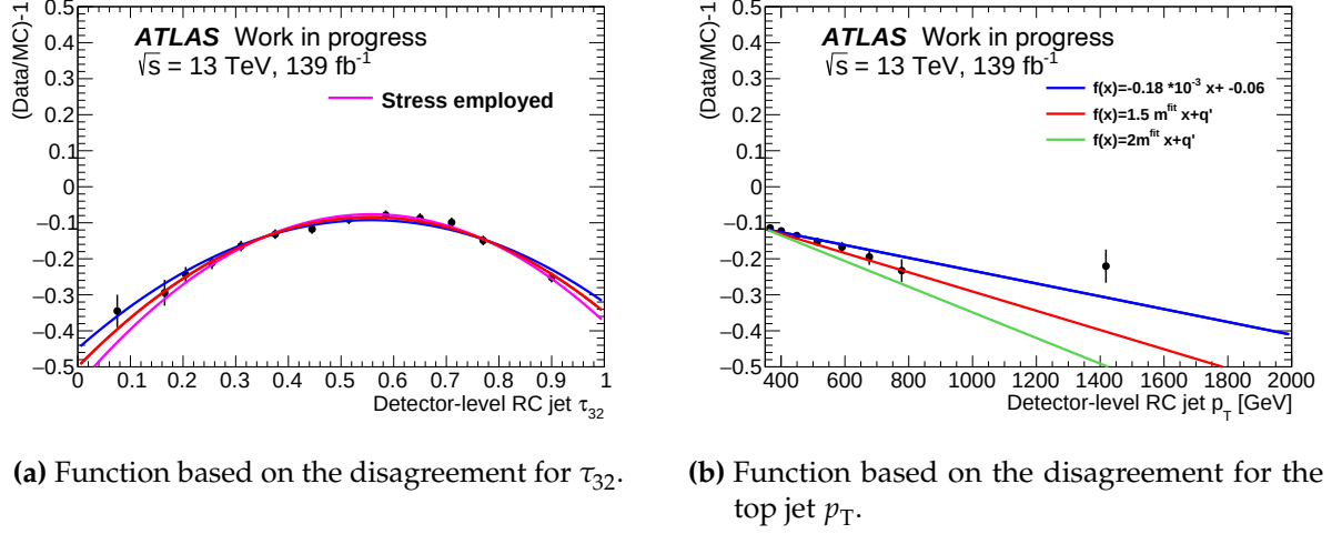
Figure 6.23: Stress functions applied in the stress test for all measured observables.
