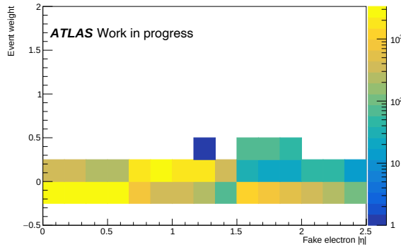
(a) Electrons
