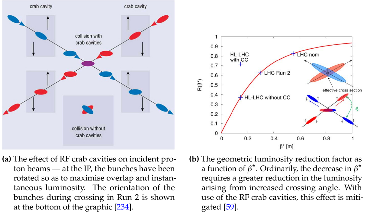
Figure 9.4: Effect of the RF crab cavities on \beta^* at the HL-LHC.
