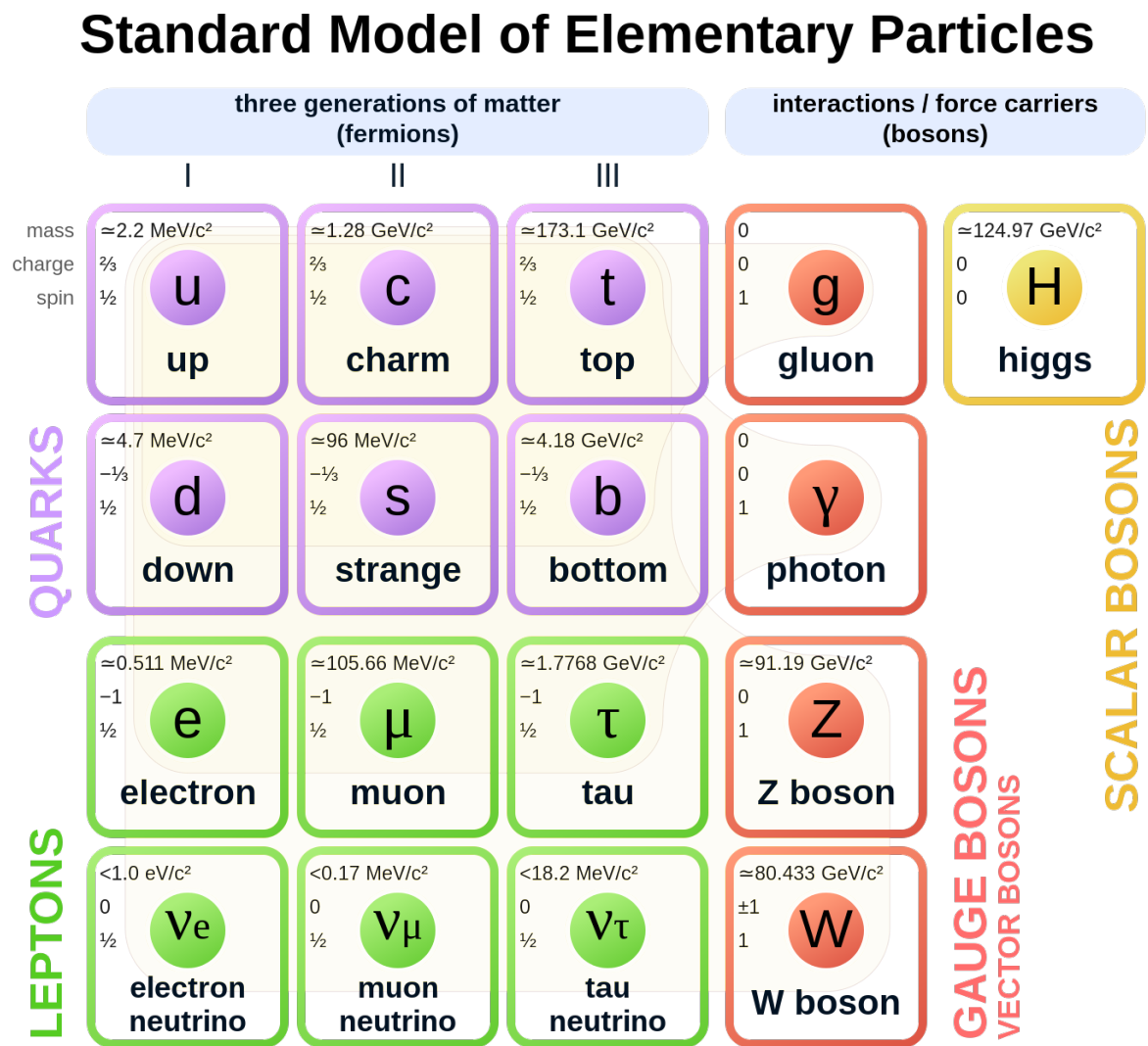
Figure 1.1: The Standard Model of particle physics. Each particle is shown with its mass, electrical charge, and spin. The shaded regions denote which forces are felt by which particles. Image from Ref. [13].
