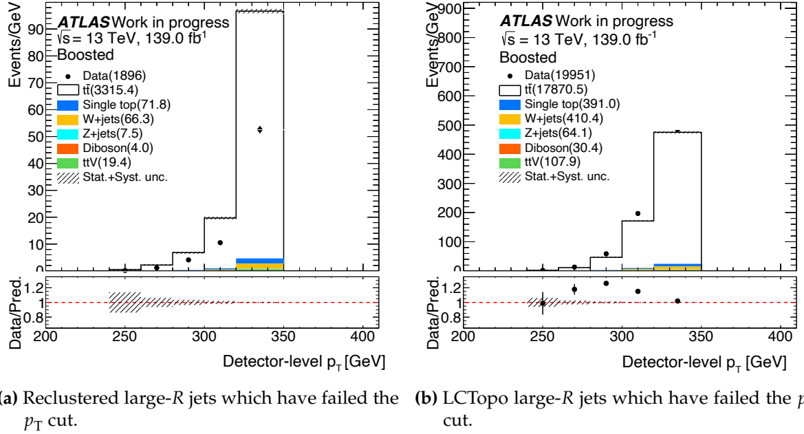
Figure 4.6: Detector-level p_T distribution for the hadronic top candidate jet. Each distribution shows the jets which failed the 350 GeV p_T cut when that cut was passed by the \Delta R -matched jet from the other jet collection.
