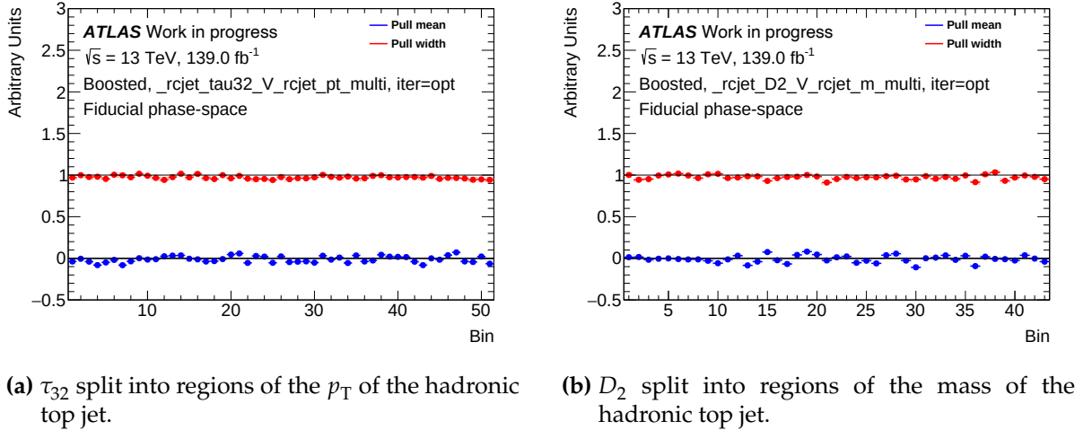
Figure 6.22: Unfolding pull test for substructure observables, showing the mean and standard deviation of the Gaussian fit to the distribution of the pull variable across 1000 pseudo-experiments. The error bands represent the uncertainties from the fit on the pull distribution.
