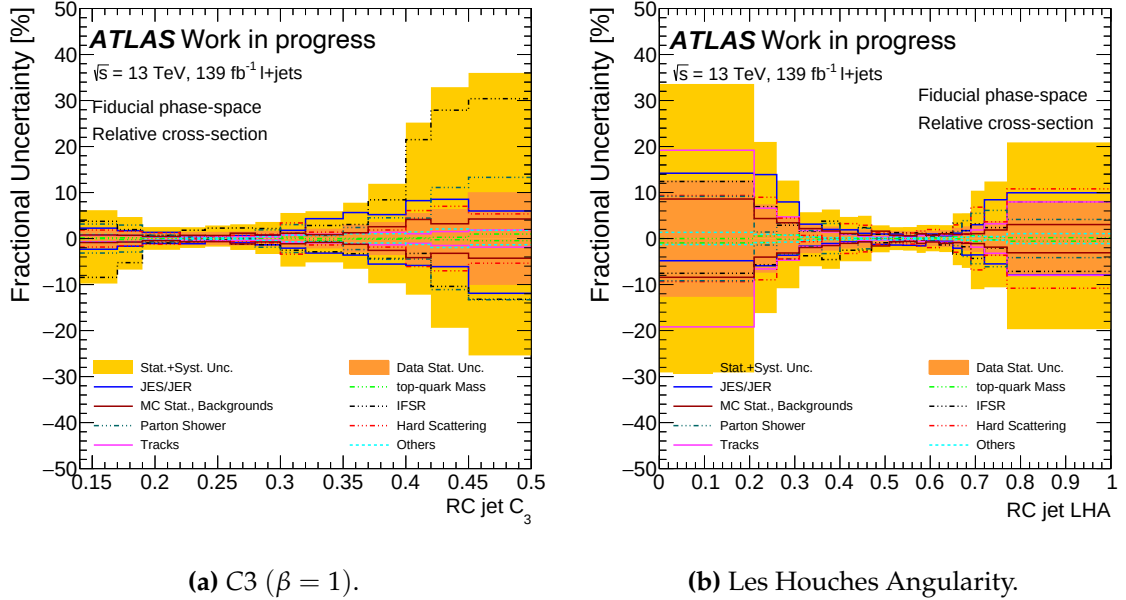
Figure 7.3: Distribution of uncertainties as a function of the substructure of the large- R reclustered jet which is the hadronic top candidate, unfolded to particle-level. Statistical uncertainties are shown in an orange band, while the yellow band shows the sum of statistical and systematic uncertainties. Sources of systematic uncertainties are further separated out by the various coloured lines shown.
