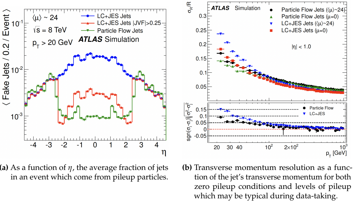
Figure 3.6: Effects of pileup compared for particle flow jets and jets clustered from calorimeter clusters. Plots from Ref. [112].
