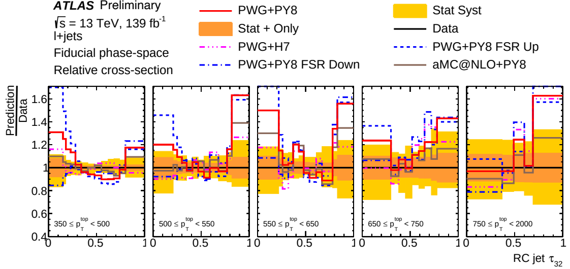
Figure 8.8: Distribution of the t\bar{t}\ell +jets production cross-section as a function of the \tau_{32} substructure observable for the large- R reclustered jet which is the hadronic top jet candidate, unfolded to particle level and split into five regions of the p_T of the jet. Shown is the ratio between NLO predictions and the data. Statistical uncertainties are shown in an orange band, while the yellow band shows the sum of statistical and systematic uncertainties.
