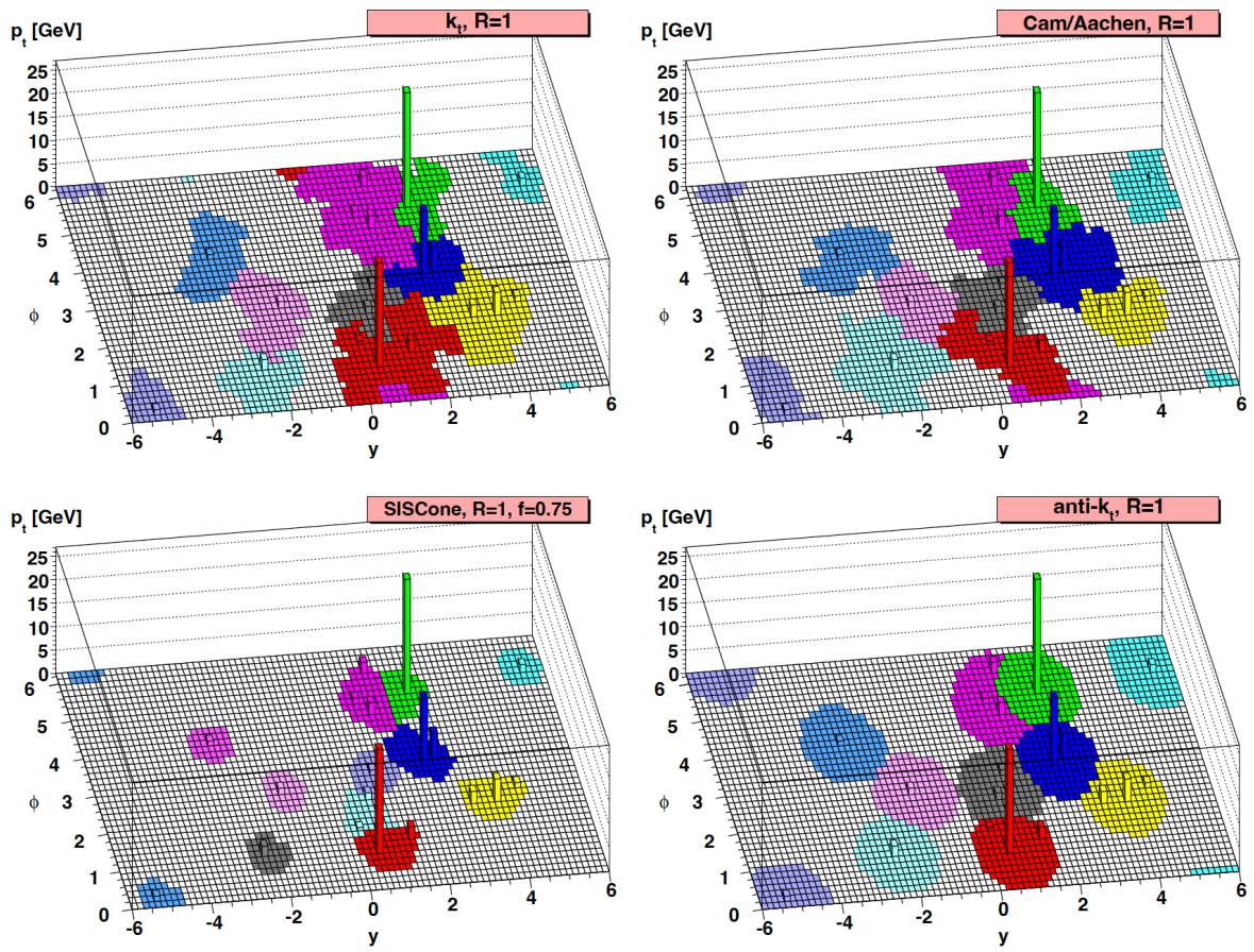
Figure 3.4: This diagram from Ref. [94] provides a comparison between four jet algorithms — the three k_t sequential recombination algorithms, and the SIScone algorithm.
