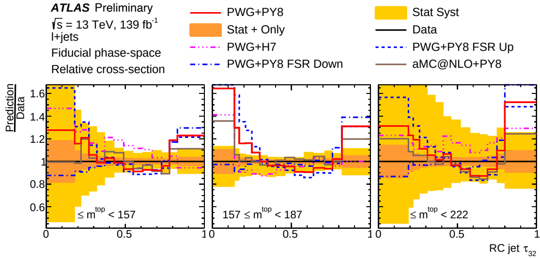
Figure 8.7: Distribution of the t\bar{t} \ell + \text{jets} production cross-section as a function of the \tau_{32} substructure observable for the large- R reclustered jet which is the hadronic top jet candidate, unfolded to particle level and split into three regions of the mass of the jet. Shown is the ratio between NLO predictions and the data. Statistical uncertainties are shown in an orange band, while the yellow band shows the sum of statistical and systematic uncertainties.
