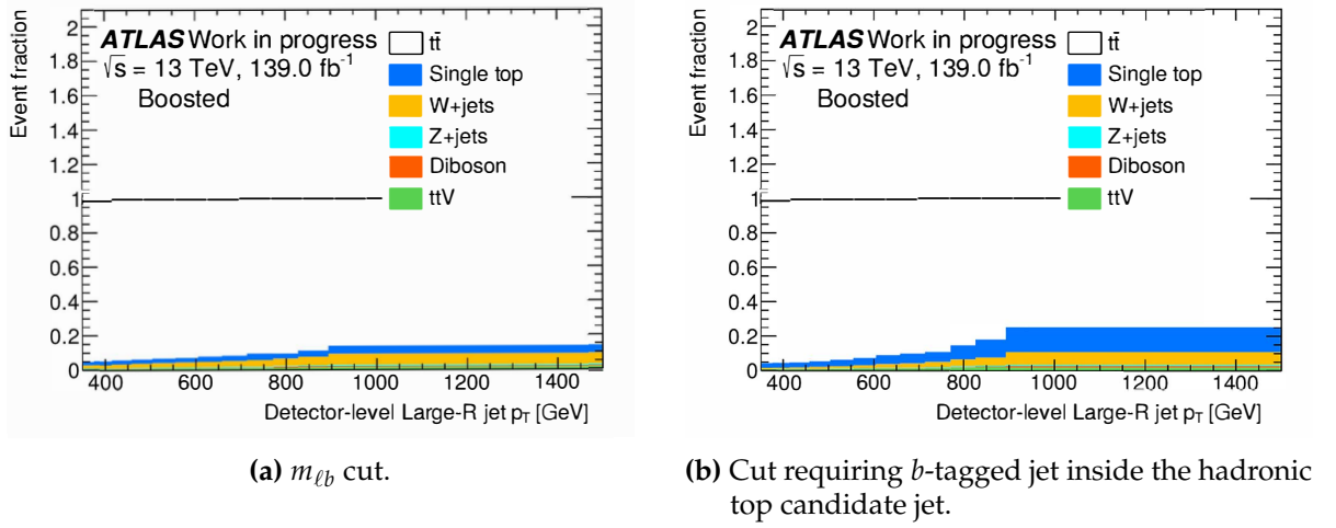
Figure 5.11: The fraction of events coming from each Monte Carlo sample at detector-level.
