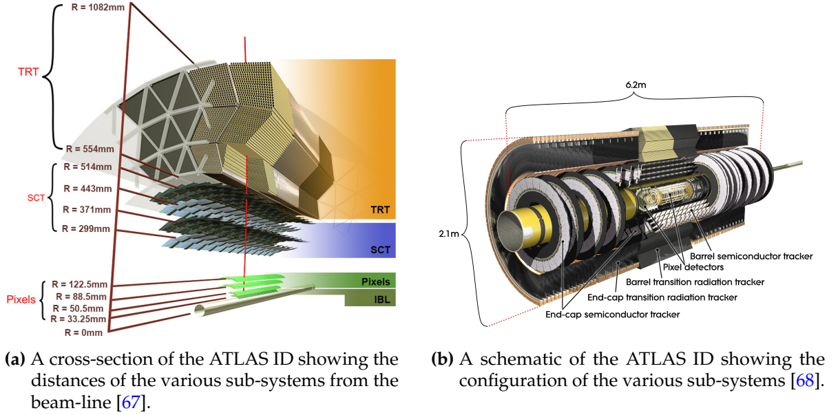
Figure 2.6: The ATLAS Inner Detector.
