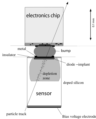
(a) A single pixel in a hybrid pixel detector. Charge is liberated as an ionising particle traverses the depletion zone. By means of the applied electric field, this charge is collected and then read out by the electronics.
