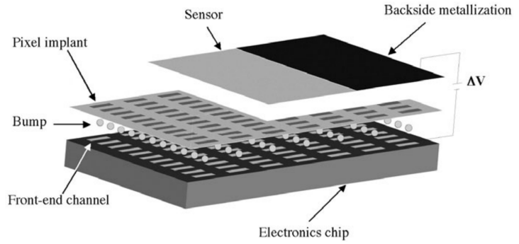
(b) Exploded view of a general hybrid pixel detector. The FE chip is bump-bonded to the sensor, with a read out channel for each pixel.
