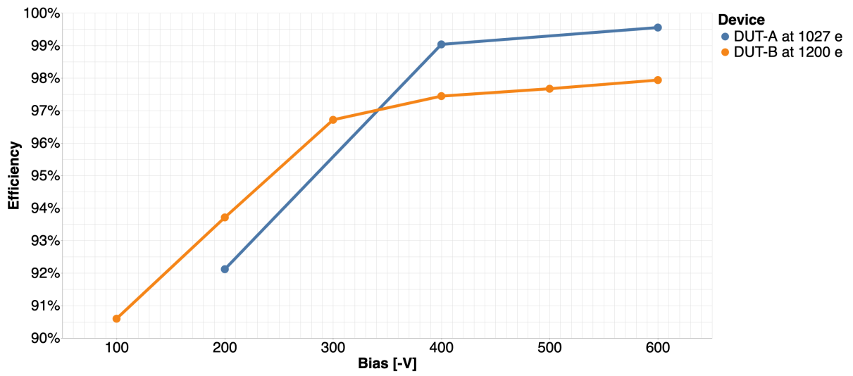
Figure 10.18: Device efficiency as a function of V_{\text{bias}} . Shown are both the device with no PTB at \text{THL} = 1027 \text{ e}^- and with zigzag PTB at \text{THL} = 1200 \text{ e}^- .
