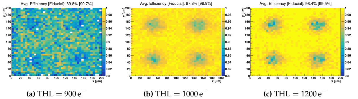
Figure 10.17: In-pixel efficiency map representing the average efficiency of a 4 \times 4 pixel array scanned across the full sensor. Shown here is the module with zigzag PTB structure and using the linear front-end, at V_{\text{bias}} = 600 \text{ V} , with different thresholds.
