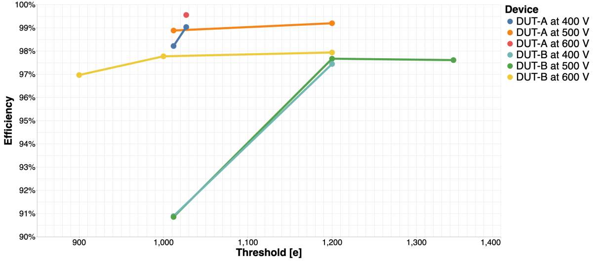
Figure 10.16: Device efficiency as a function of threshold. Shown are both the device with zigzag PTB, and the device with no PTB structure, each at V_{\text{bias}} = 400 \text{ V} , V_{\text{bias}} = 500 \text{ V} , and V_{\text{bias}} = 600 \text{ V} . All measurements are with the linear front-end.
