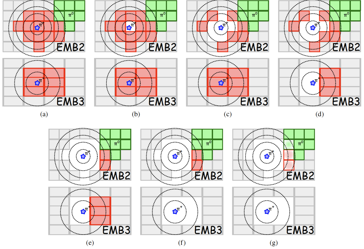
Figure 3.7: Idealised view of the particle flow cell subtraction procedure. The extrapolated position of a track from a \pi^+ is shown by the blue star for two ECAL layers, with EMB2 representing the LHED. Calorimeter cells are red for the cluster belonging to the \pi^+ and green for those belonging to a \pi^0 . Starting from the innermost ring of the LHED in (a), rings are removed from those with highest energy density to those with lowest, as long as the removed energy remains less than that expected to be deposited. Once the procedure reaches (g), this final ring contains enough energy to take the total removed over the expected deposited energy, so is scaled until the energy removed matches that expected to have been deposited. Image from Ref. [112]
