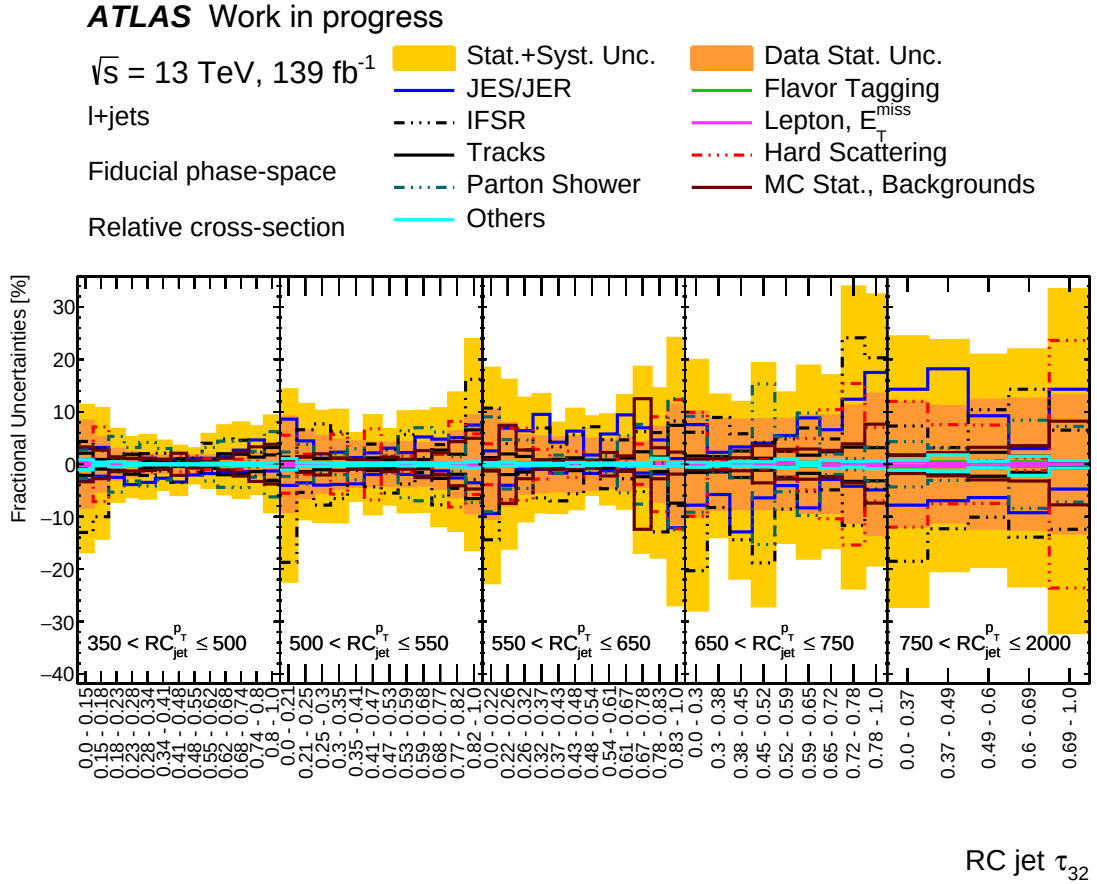
Figure 7.6: Uncertainties on the distribution of the t\bar{t} \ell + \text{jets} production cross-section as a function of the \tau_{32} substructure observable for the large- R reclustered jet which is the hadronic top jet candidate, split into five regions of the p_T of the jet. Statistical uncertainties are shown in an orange band, while the yellow band shows the sum of statistical and systematic uncertainties.
