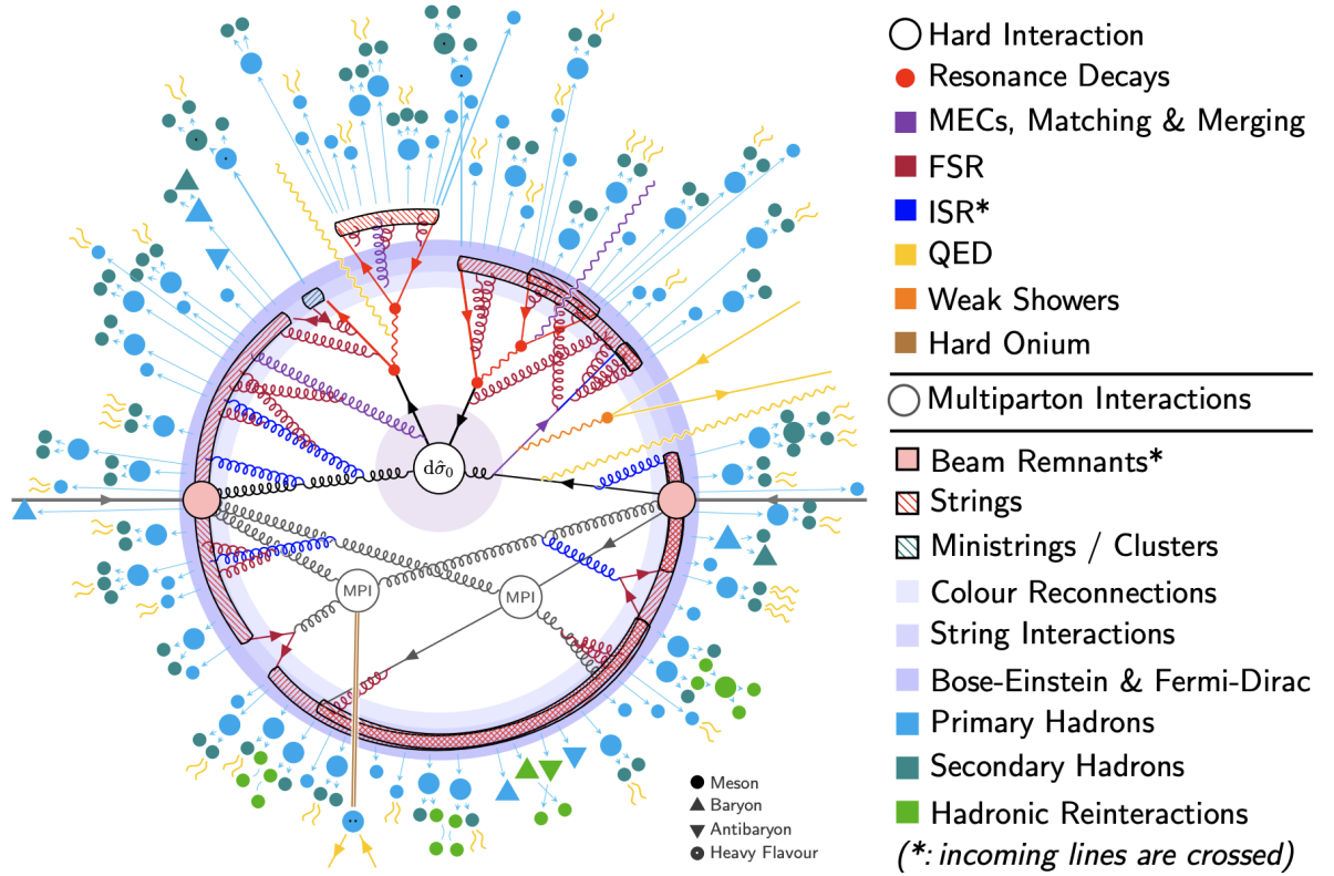
Figure 1.7: Shown are the numerous components which must be simulated for a t\bar{t} event, as performed using PYTHIA [40]. From the incoming protons, shown in the pink circles either side of the diagram, the hard scatter process can be seen in the centre, producing a t\bar{t} pair which subsequently decays. Also present are multi-parton interactions (MPI), the parton shower (PS), and the hadronisation process resulting in stable hadrons present in the final-state. Image from Ref. [41, 42].
