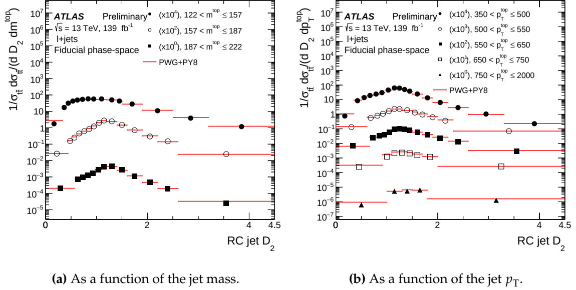
Figure 8.6: Distribution of the t\bar{t} \ell + \text{jets} production cross-section as a function of the D_2 substructure observable for the large- R reclustered jet which is the hadronic top jet candidate, unfolded to particle level. Shown is a comparison between the data and the nominal prediction, with results divided into regions of the jet kinematics.
