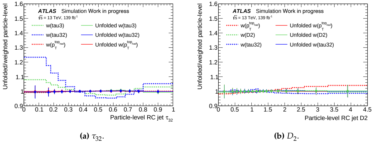
Figure 6.24: Particle-level distributions for substructure observables. The lines represent a ratio to the re-weighted particle-level distribution. The dashed lines are for the nominal particle-level prediction, whilst the solid lines are for the re-weighted detector-level MC which has been unfolded. The ratio for the unfolded distribution should be compatible with unity in order for the test to have achieved closure.
