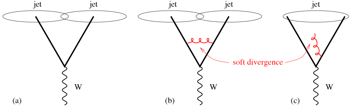
Figure 3.2: This diagram from Ref. [97] shows the effect of an infrared-unsafe algorithm. In a) and b), the result is the same. Two jets, the same two jets, are returned. In c), however, the soft radiation introduced has skewed the algorithm such that the two jets are merged into one and a different jet collection is returned.
