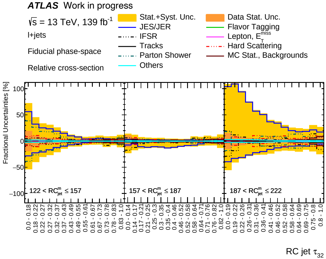
Figure 7.5: Uncertainties on the distribution of the t\bar{t} \ell + \text{jets} production cross-section as a function of the \tau_{32} substructure observable for the large- R reclustered jet which is the hadronic top jet candidate, split into three regions of the mass of the jet. Statistical uncertainties are shown in an orange band, while the yellow band shows the sum of statistical and systematic uncertainties.
