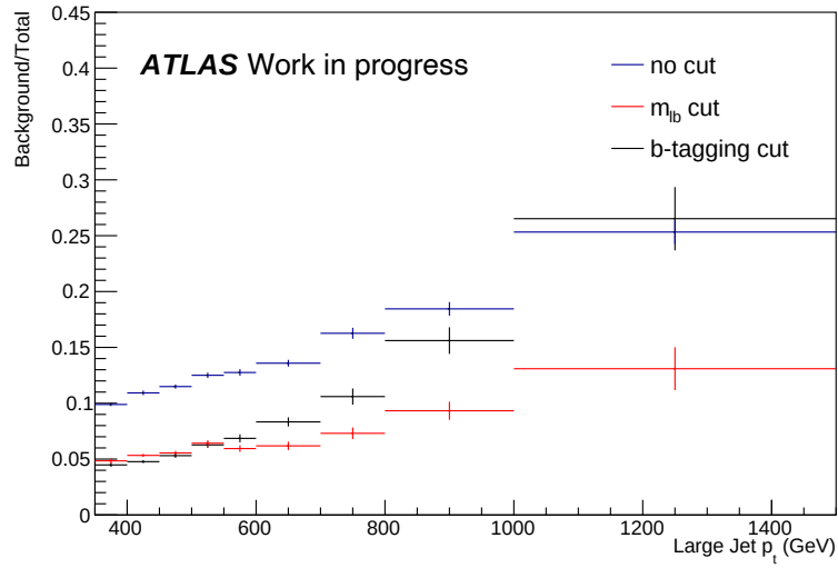
Figure 5.7: The proportion of accepted events which are background, as a function of p_T , for the m_{lb} cut, the b -tagging cut, and when no final cut is applied.
