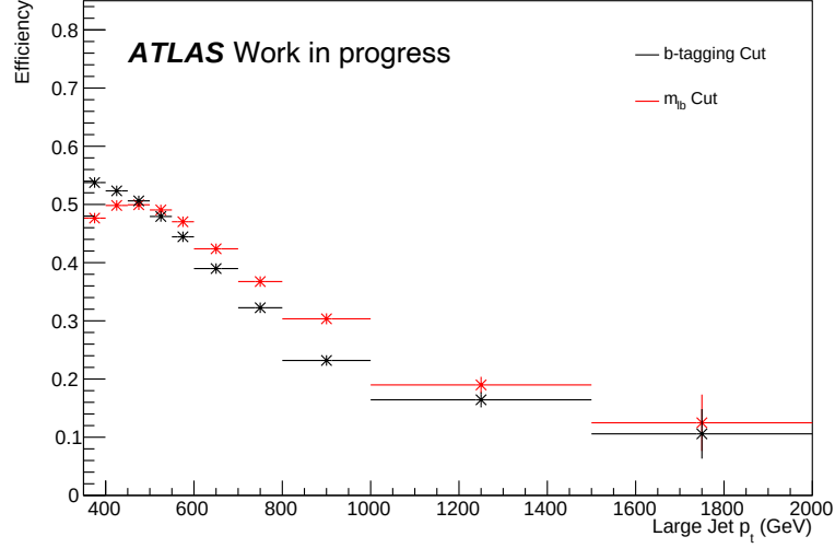
Figure 5.6: The proportion of signal events passing selection, as a function of p_T , for the m_{lb} cut and the b -tagging cut.
