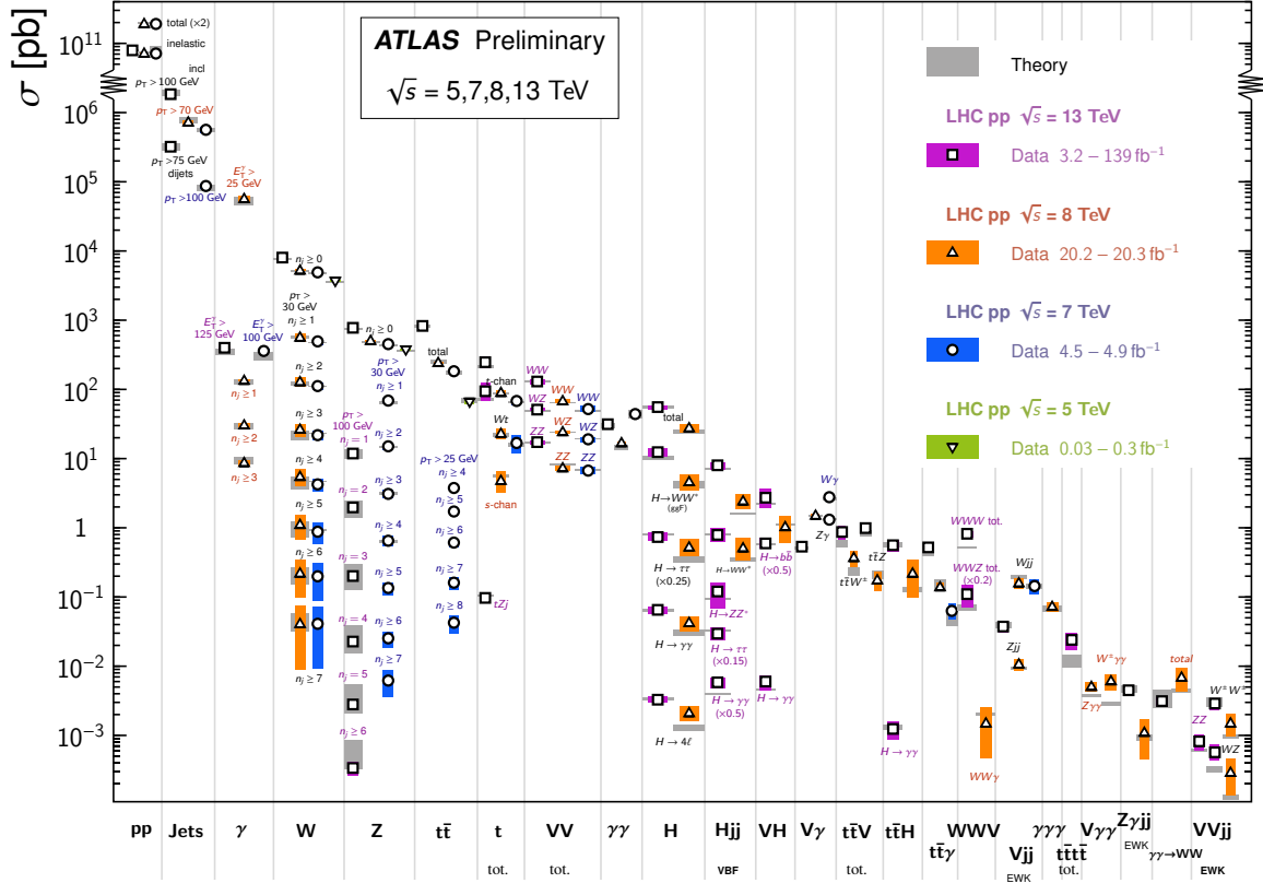
Figure 9.2: Cross-sections for many SM processes accessible to ATLAS [30]. Measurements from all data-taking periods are included as well as theoretical predictions. Measurements are corrected for branching fraction.
