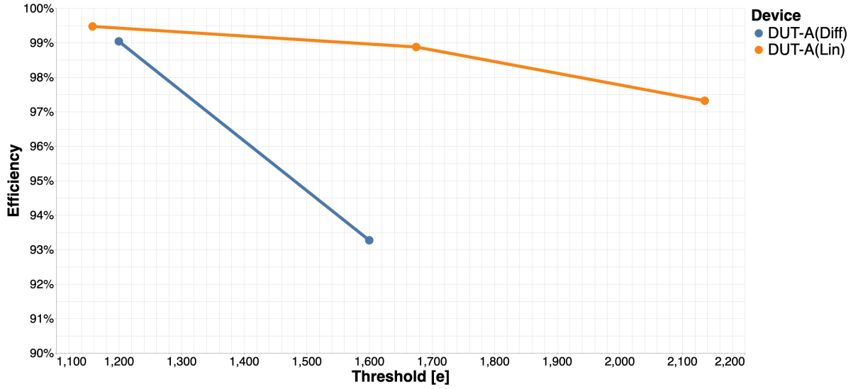
Figure 10.13: Device efficiency as a function of threshold, in number of electrons. Shown here are linear and differential front-ends, at V_{\text{bias}} = 600 V, for the module with no PTB structure.
