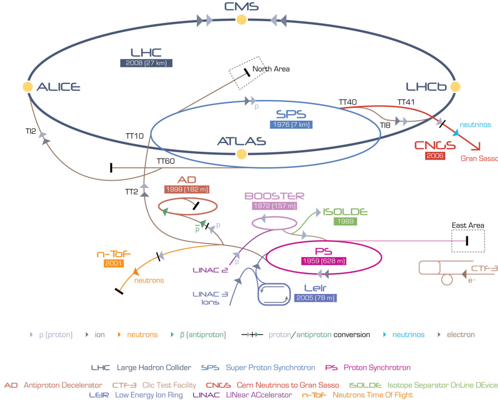
FIGURE 3.1: Schema of the LHC injection chain
