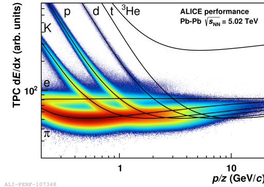
FIGURE 3.10: Distribution of dE/dx for charged particles in function of particle momentum, measured by the TPC in Pb-Pb collisions.
