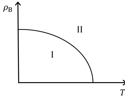
FIGURE 1.4: First phase diagram of hadronic matter [33]: \rho_B is the baryonic density, T is the temperature, I the confined phase and II the deconfined phase.
