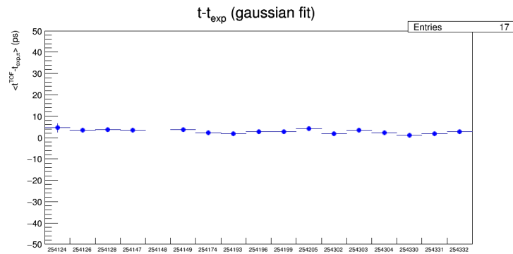
FIGURE 4.20: Trending distribution of the (t_{\text{TOF}} - t_{\text{exp}}) alignment for a set of 2016 pp runs at \sqrt{s} = 13 TeV is shown, obtained by the QA offline analysis. Each value per run is the mean value from the gaussian fit of the (t_{\text{TOF}} - t_{\text{exp}}) distribution.
