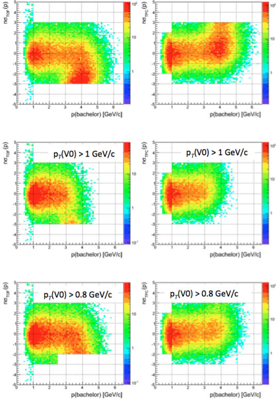
FIGURE 5.13: Effects of different PID cuts on TOF (left) and TPC (right) variables for the bachelor track in the bin 4 < p_T < 5 GeV/c bin with different cuts on V0 p_T . Top: no cut on V0 p_T applied and contamination from pions and kaons visible; middle: strong cut on V0 p_T but reduction of statistics at larger momentum; bottom: relaxation of the cut on V0 p_T and strengthening of the cut on TOF PID.
