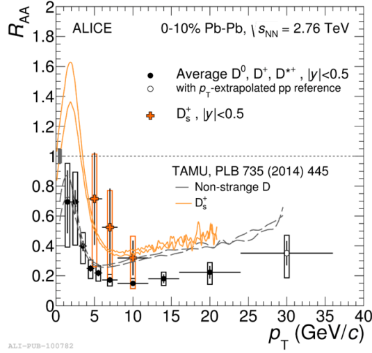
FIGURE 2.14: Nuclear modification factor R_{AA} of D_s^+ mesons [118], compared with the averaged R_{AA} for D^0 , D^+ and D^{*+} [117], measured by ALICE.
