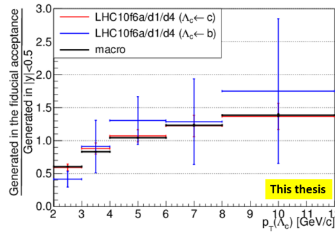
FIGURE 6.7: Acceptance estimated with the toy model, in black. Superimposed in red and blue colors, the results on minimum bias MC productions, for comparison.
