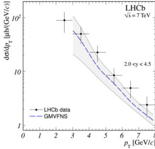
FIGURE 2.5: p_T -differential cross sections for charmed baryon \Lambda_c^+ in pp collisions at \sqrt{s} = 7 TeV, measured by LHCb [14], compared with GM-VFNS calculations [89] [90].
