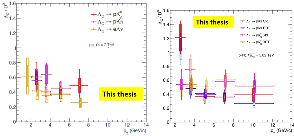
FIGURE 6.42: Comparison between all the \Lambda_c/D^0 ratios in pp collisions (Left plot) and p-Pb collisions (Right plot).
