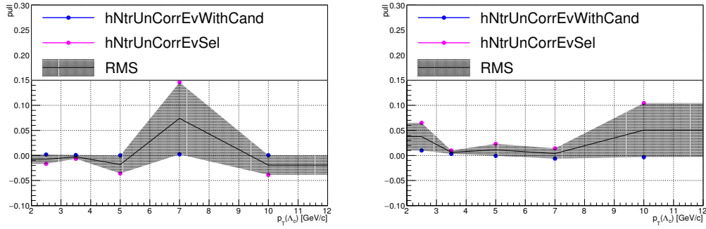
FIGURE 6.37: Relative discrepancy of the efficiency estimated with different multiplicity weights with respect to that one used in our analysis. On the left, for \Lambda_c from b; on the right the prompt ones.
