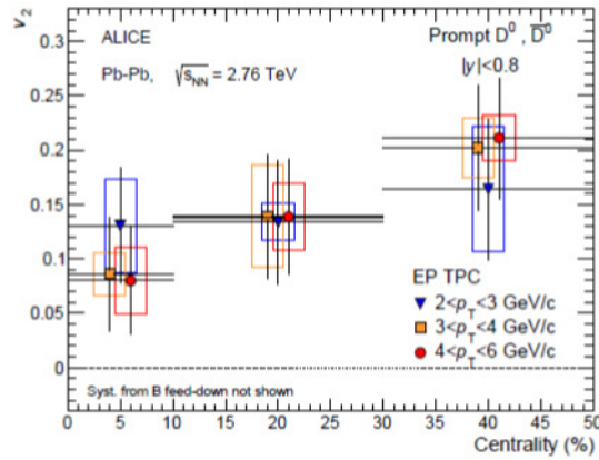
FIGURE 2.19: Centrality dependence of the D^0 meson \nu_2 measured by ALICE for three different p_T intervals [137].
