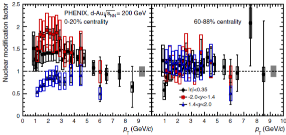
FIGURE 2.7: Nuclear modification factor of leptons from heavy-flavour decays in d-Au collisions. Measurement performed with the PHENIX detector at \sqrt{s_{\text{NN}}} = 200 GeV, as a function of p_T in two different centrality classes [97].
