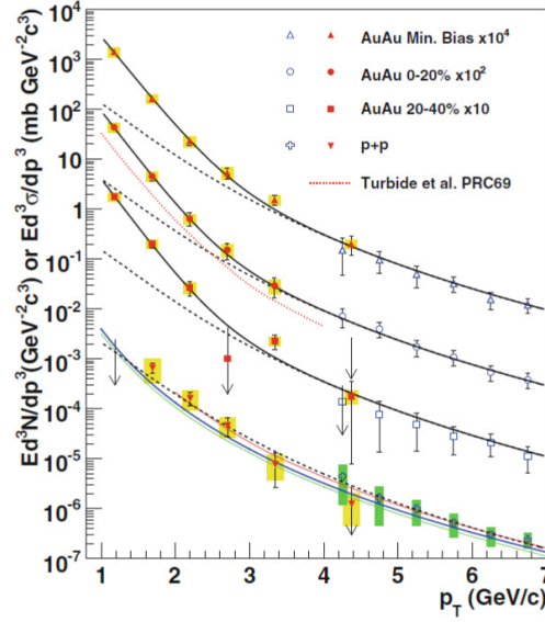
FIGURE 1.15: Transverse momentum dependence of direct photon particle spectra in Au - Au minimum bias collisions at RHIC in 0-20% and 20-40% centrality classes, shown together with pp results [53]. The dashed lines are the scaled pp data; the three lines on the pp results are next-to-leading order pQCD calculations. The dotted line on the Au - Au results is also a result from theoretical calculations.
