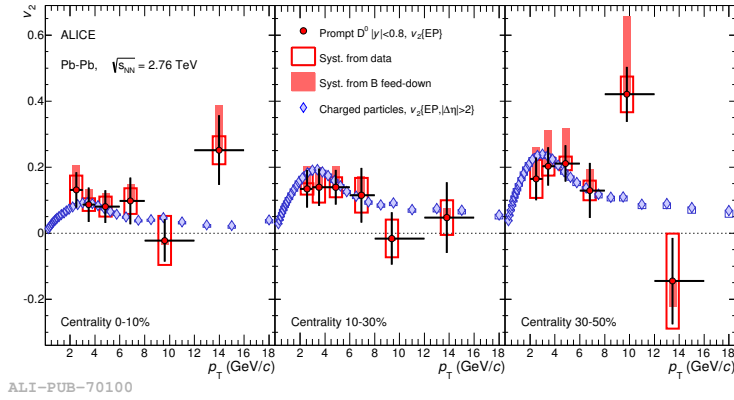
FIGURE 2.18: D-mesons \nu_2 measured by the ALICE Collaboration [135] [137]. Comparison of prompt D^0 meson and charged-particle \nu_2 measured by ALICE Collaboration [114] [136] in three centrality classes as a function of p_T .
