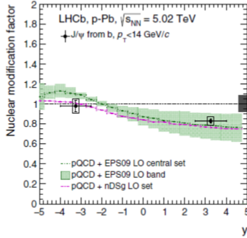
FIGURE 2.10: LHCb measurements of non-prompt J/\Psi in p-Pb collisions [104]: the nuclear modification factor is shown as a function of the rapidity and compared to nPDF-based calculations [106].
