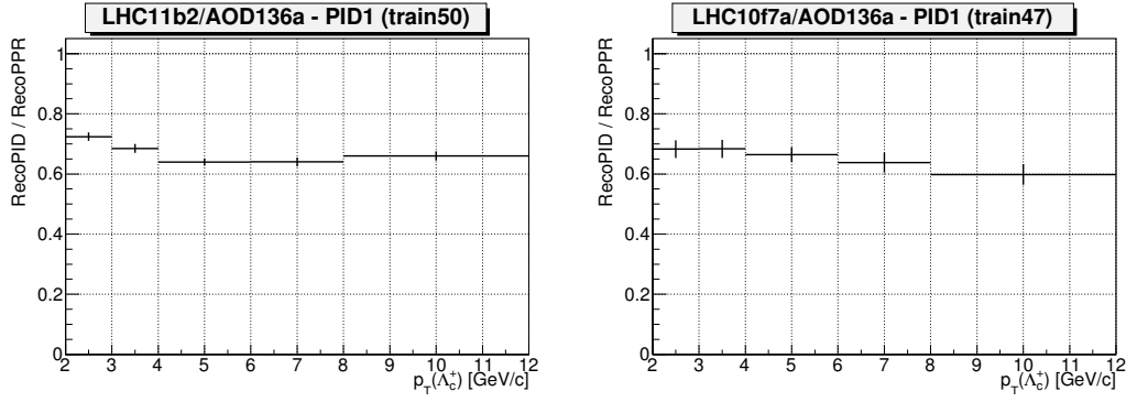
FIGURE 6.12: Bachelors identification efficiency vs p_T of \Lambda_c in pp collisions.
