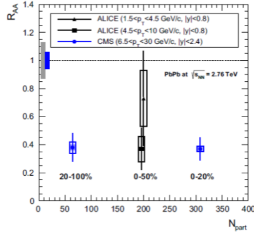
FIGURE 2.15: Non-prompt J/\Psi R_{AA} measured in two centrality bins from CMS [123] and in one centrality bin for two p_T ranges from ALICE [124]. The ALICE points are slightly shifted horizontally for better visibility. The correlated uncertainties are shown as filled box at R_{AA} = 1 .
