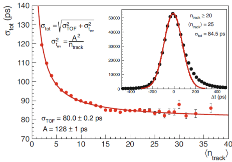
FIGURE 4.21: TOF total time resolution versus number of tracks per event.
