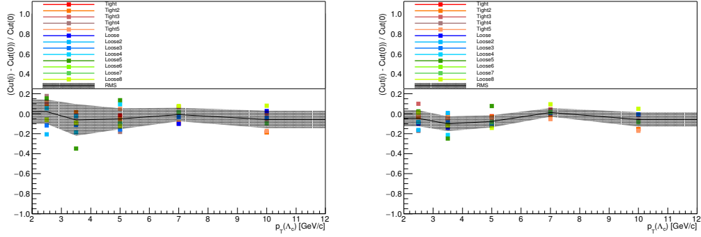
FIGURE 6.26: Systematics on cut variation in pp. Relative discrepancy of the p_T -differential cross section in five p_T intervals estimated for each set of cuts with respect to that one estimated on the central cuts set. In the left plot, the signal extraction was performed without any restriction on the fit parameter. In the right plot, sigmas are fixed to the values obtained from signal extraction on the central set of cuts.
