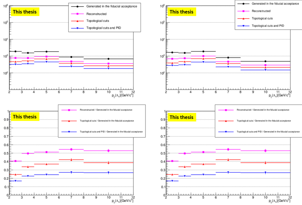
FIGURE 6.10: LHC13d3 production: on the top, \Lambda_c \rightarrow p K_S^0 generated in the acceptance (black), reconstructed in the acceptance (magenta), selected according to the cut optimization (red) and bachelor PID (blue); on the bottom: ratios with respect to the \Lambda_c \rightarrow p K_S^0 generated in the acceptance. On the left, prompt \Lambda_c and on the right b-induced \Lambda_c . The efficiency is the blue fraction on the bottom.
