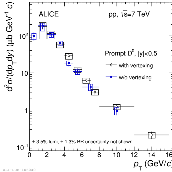
FIGURE 2.3: p_T -differential production cross section of D^0 mesons with |y| < 0.5 in pp collisions at \sqrt{s} = 7 TeV [80]. The comparison between the prompt D^0 cross sections measured with and without decay-vertex reconstruction is shown.
