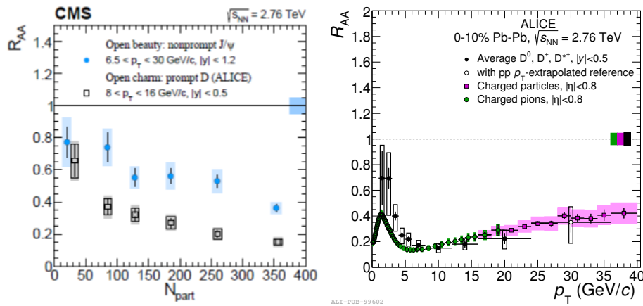
FIGURE 2.16: Comparison of R_{AA} for charm, beauty and light-flavour. Left: R_{AA} of D mesons in 8 < p_T < 16 GeV/c from ALICE [125] and preliminary non-prompt J/\Psi mesons from CMS in 6.5 < p_T < 30 GeV/c [126]; Right: Prompt D-meson R_{AA} (average of D^0 , D^+ and D^{*+} ) as a function of p_T compared to the nuclear modification factor of pions and charged particles in the 0-10% centrality range [128].
