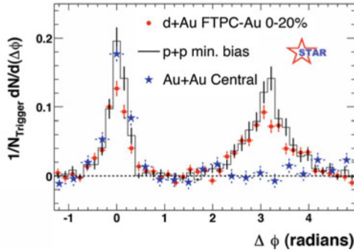
FIGURE 1.16: Correlation of near-side and away-side jets ( p_T in [4-6] GeV) [59]. It is clearly visible for pp and d - Au collisions, whereas it is lost for Au - Au collisions ( \sqrt{s_{NN}} = 200 \text{ GeV} )
