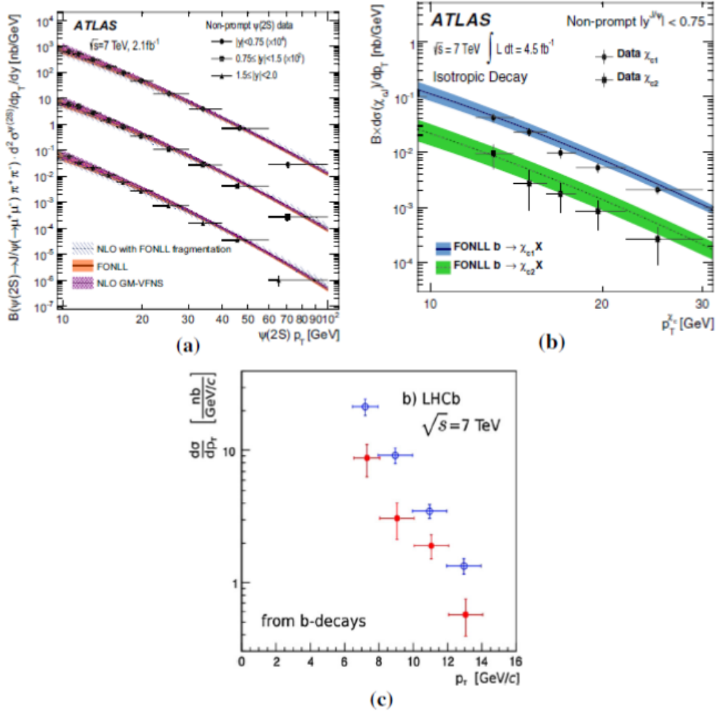
FIGURE 2.6: p_T -differential cross sections for non-prompt charmonia (assumed to come from beauty decays: a) \Psi(2S) by ATLAS [92], compared with FONLL [74] and GM-VFNS [89] [90]; b) \chi_{c1} and \chi_{c2} by ATLAS [93], compared with FONLL [74]; c) J/\psi and \eta_c by LHCb [91].
