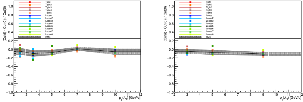
FIGURE 6.27: pp analysis: Relative discrepancy of the p_T - differential cross section in five, on the left, and three, on the right, p_T intervals estimated for each set of cuts with respect to that one estimated on the central cuts set. Sigmas are fixed to the values obtained from signal extraction on the central set of cuts.
