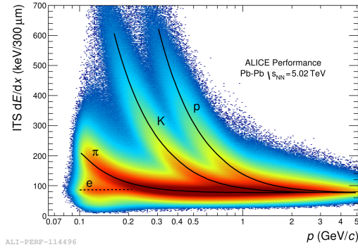
FIGURE 3.8: Distribution of dE/dx for charged particles in function of particle momentum, measured by the ITS in Pb-Pb collisions.
