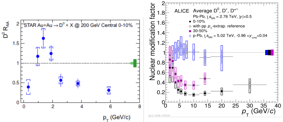
FIGURE 2.13: Left: Transverse momentum dependence of the nuclear modification factor R_{AA} of D^0 mesons in the 10% most central Au-Au collisions at \sqrt{s_{NN}} = 200 GeV [116]. Right: R_{AA} of prompt D mesons (average of D^0 , D^+ and D^{*+} ) versus p_T for 0-10% and 30-50% centrality classes in Pb-Pb collisions at \sqrt{s_{NN}} = 2.76 TeV [117] and p-Pb collisions at \sqrt{s_{NN}} = 5.02 TeV [99]. Theoretical calculations for D_s^+ mesons, using the TAMU model [120] [121] are superimposed.
