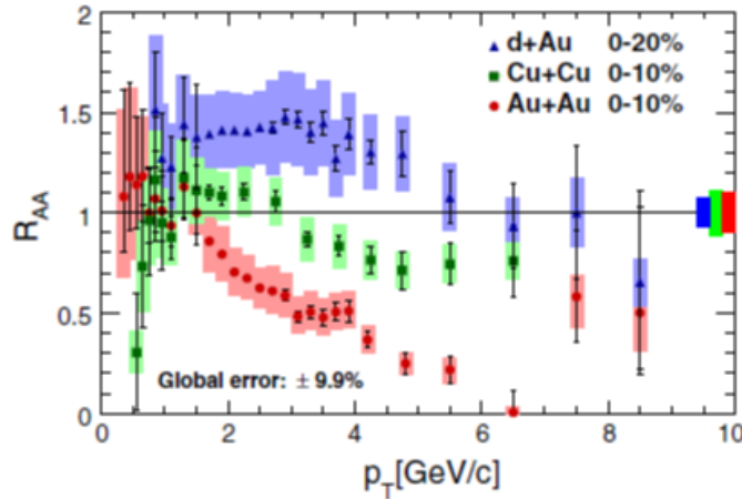
FIGURE 2.11: Transverse momentum dependence of the R_{AA} of heavy-flavour decay electrons at mid-rapidity measured in central d-Au [111], Cu-Cu [112] and Au-Au [110] collisions.
