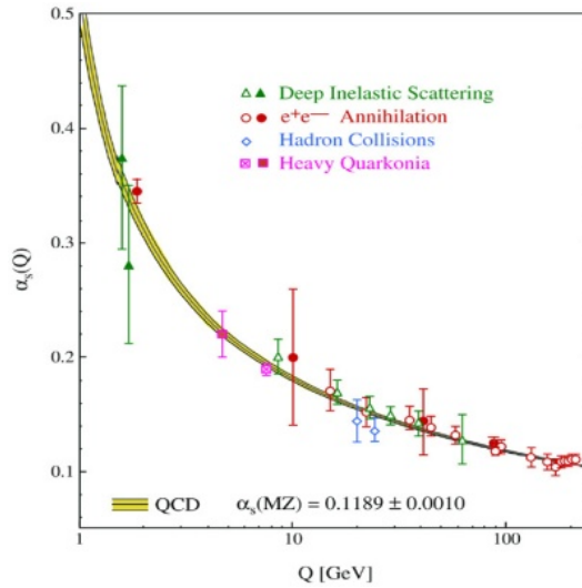
FIGURE 1.1: Coupling coefficient \alpha_s for QCD, as a function of transfert momentum Q , measured using different colliding systems.
