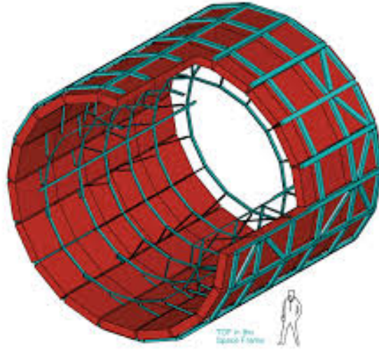
FIGURE 4.2: ALICE TOF layout.
