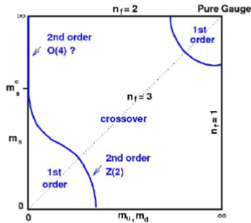
FIGURE 1.7: Lattice QCD calculations of the criticalness of the hadronic matter phase transition for \mu_B = 0 and for three quark flavours assuming the mass of u and d identical and a strange quark mass with mass m_s [37].
