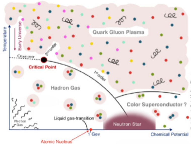
FIGURE 1.9: Hadronic matter phase diagram, according the most recent lattice QCD results and hypothesis.
