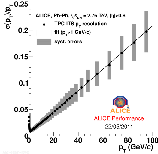
FIGURE 3.9: TPC track momentum resolutions.
