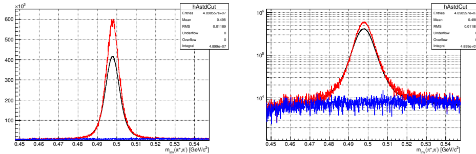
FIGURE 5.12: \pi^+ - \pi^- invariant mass distributions for true (red) and fake (blue) K_S^0 ; superimposed in black the same distribution for data with the additional selections on p - \pi^- , \pi^+ - \bar{p} and e^+ - e^- invariant masses. Left: linear scale; right: logarithmic scale.
