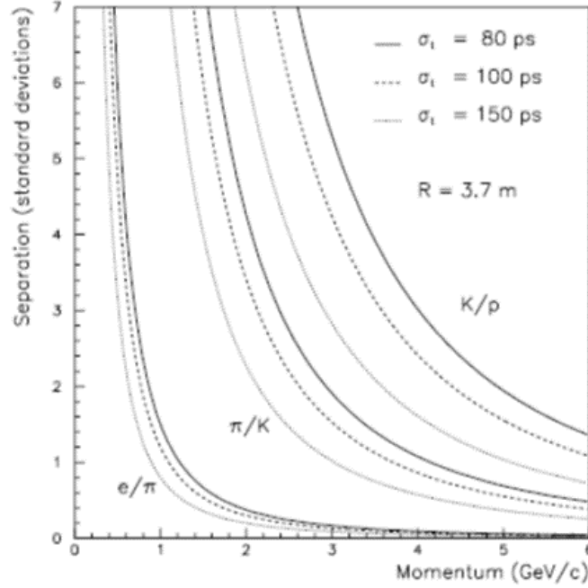
FIGURE 4.1: Predicted separation of particles emitted at \theta = 90^\circ for TOF. The separation is shown in correspondence of three different TOF resolutions.
