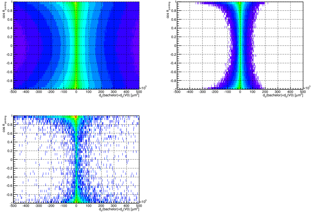
FIGURE 5.4: d_0(\text{bachelor}) \times d_0(V0) vs cosine of \Lambda_c pointing angle. On the top left: data; on the top right: MC background; on the bottom left, MC signal.
