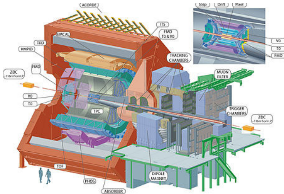
FIGURE 3.6: Schematic view of the ALICE detector. Here AD [142] and DCAL [143] are not visible, since they were added only recently, during the Long Shutdown 1 of the LHC.
