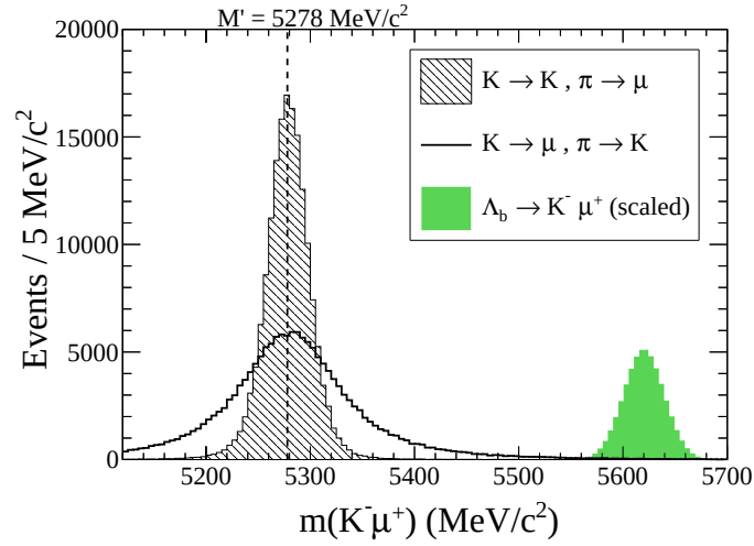
Figure 3.3: Mass distribution of the B^0 \rightarrow K^+\pi^- reflection after selections.
