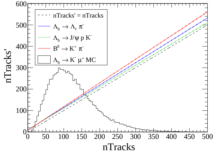
Figure 4.11: Calibration curves for the track multiplicity. The histogram shows the n\text{Tracks} distribution from simulated \Lambda_b \rightarrow K^- \mu^+ events in arbitrary units.
