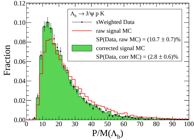
Figure 4.14: Comparison of the boost distribution from MC to data before and after the correction.
