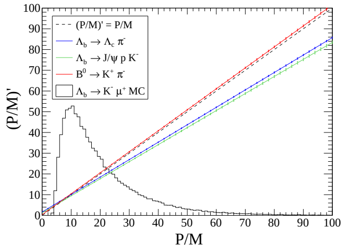
Figure 4.20: Calibration curves for the \Lambda_b boost from 2011 data. The histogram shows the P/M distribution from simulated \Lambda_b \rightarrow K^-\mu^+ events in arbitrary units.
