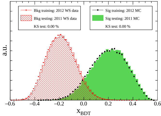
Figure 5.8: BDT response comparison using 2012 data for training and 2011 data for testing.
