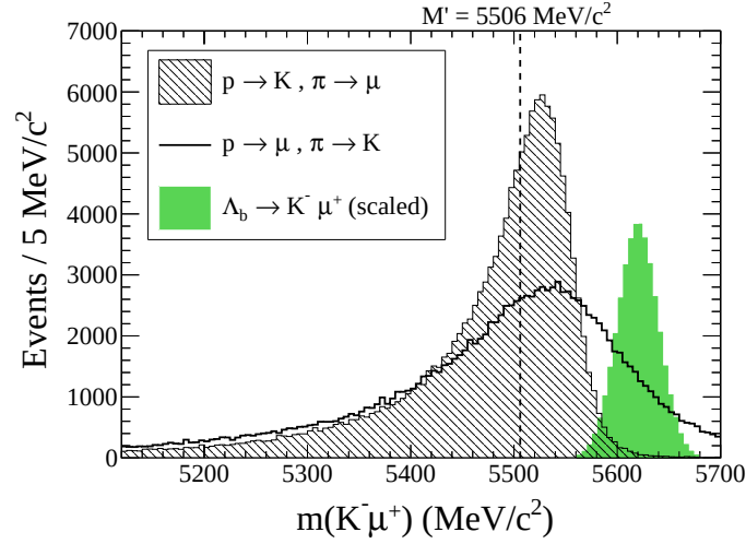
Figure 3.4: Mass distribution of the \Lambda_b \rightarrow p\pi^- reflection after selections.
