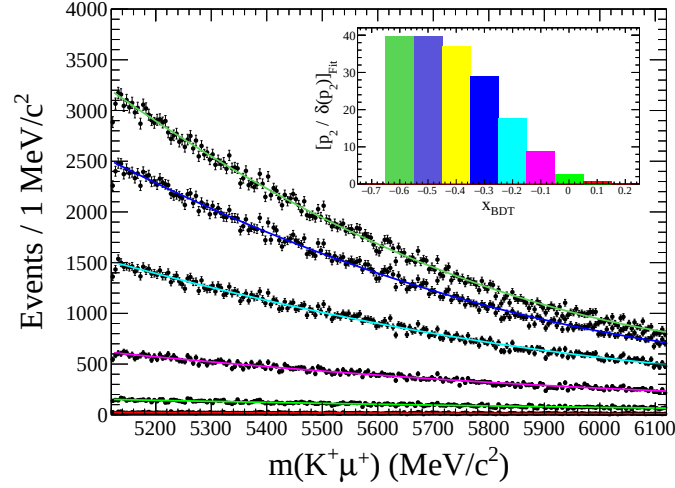
Figure 5.7: Influence of the BDT classifier on the K^+\mu^+ mass spectrum.
