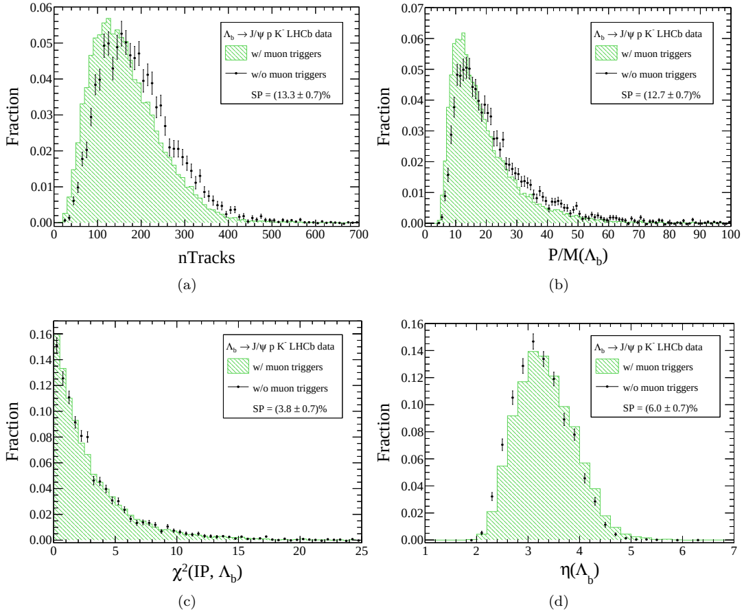
Figure 4.10: sPlot 'ed distributions from \Lambda_b \rightarrow J/\psi p K^- events using different trigger conditions.
